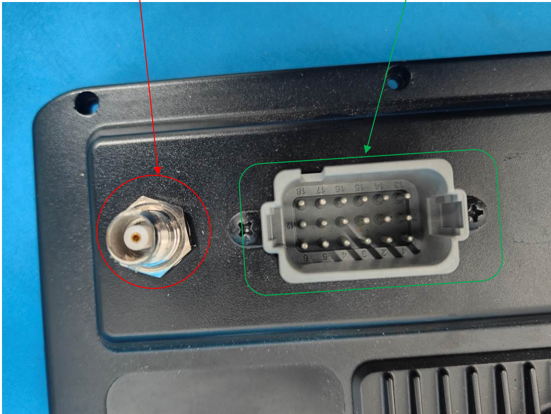
Main Harness Interface
