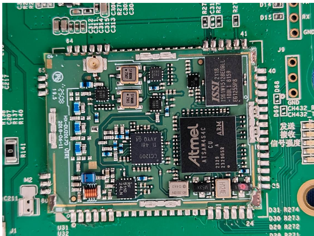
PMR Module Unshielded (only RX)
