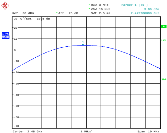
BLE 2Mbps_High_Channel
