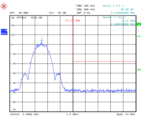
BLE 2Mbps_High_Channel
