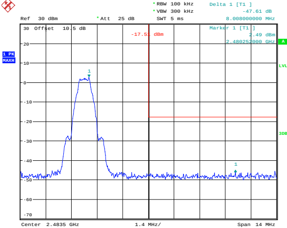
BLE 1Mbps_High_Channel
