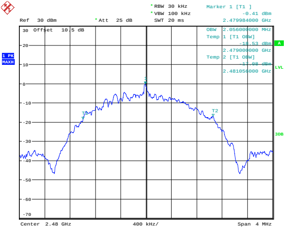
BLE 2Mbps_High_Channel
