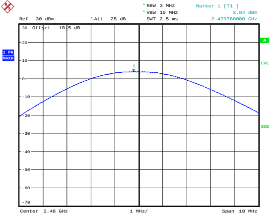
BLE 1Mbps_High_Channel
