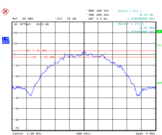
BLE 2Mbps_High_Channel
