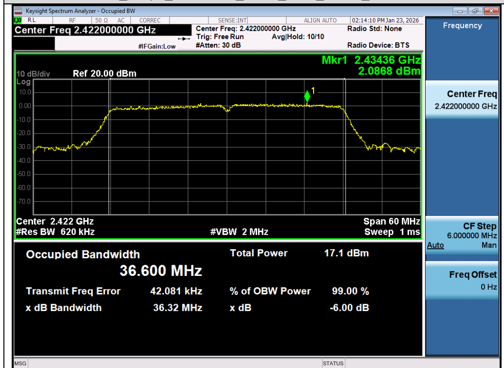
Test_Graph_802.11n40_ANT1_2422_MCS0_DTSBW
