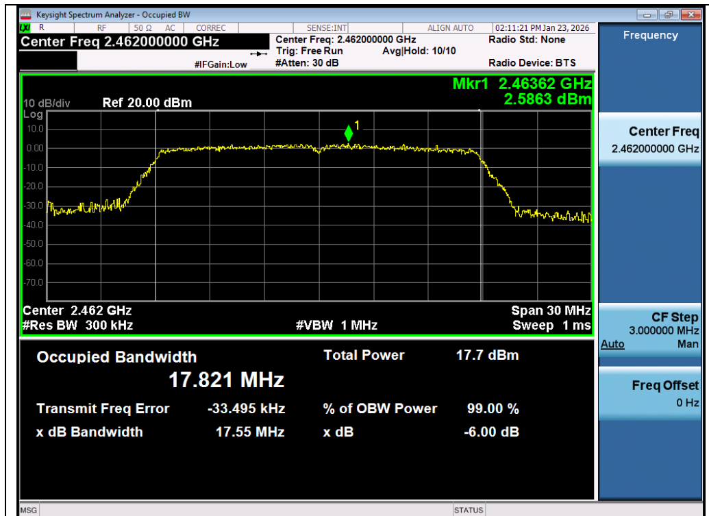
Test_Graph_802.11n20_ANT1_2462_MCS0_DTSBW
