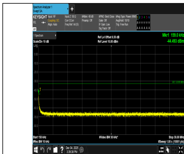
EGPRS1900-661-2-0.15~30MHz-PASS
