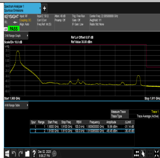
Band2-10MHz-16QAM-19150-1RB#0-PASS
