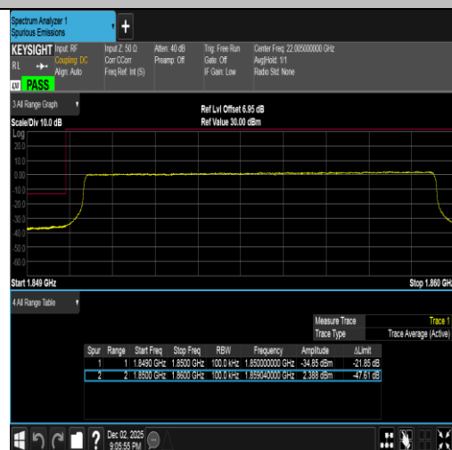
Band2-10MHz-16QAM-18650-50RB#0-PASS
