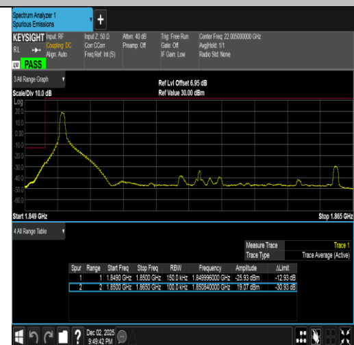
Band2-15MHz-16QAM-18675-1RB#0-PASS
