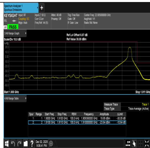
Band2-10MHz-QPSK-19150-1RB#49-PASS
