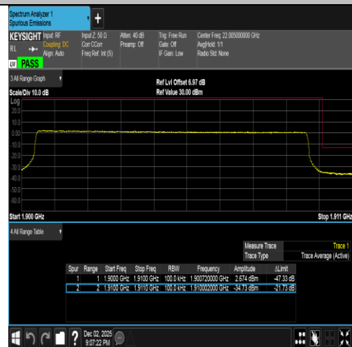
Band2-10MHz-16QAM-19150-50RB#0-PASS
