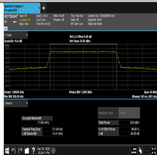
Band2-20MHz-16QAM-18900-100RB#0-PASS
