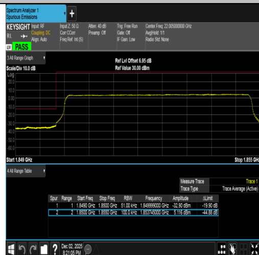
Band2-5MHz-16QAM-18625-25RB#0-PASS
