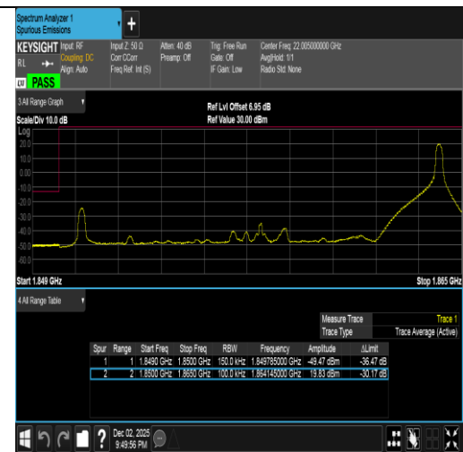
Band2-15MHz-QPSK-18675-1RB#74-PASS
