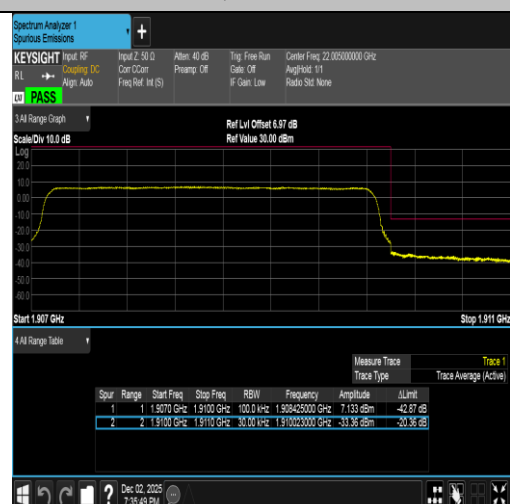
Band2-3MHz-16QAM-19185-15RB#0-PASS
