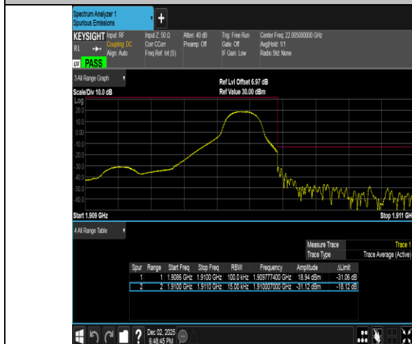
Band2-1.4MHz-16QAM-19193-1RB#5-PASS
