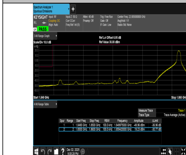
Band2-10MHz-16QAM-18650-1RB#49-PASS
