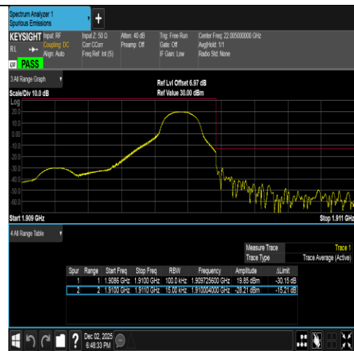
Band2-1.4MHz-QPSK-19193-1RB#5-PASS
