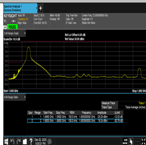
Band2-10MHz-16QAM-18650-1RB#0-PASS
