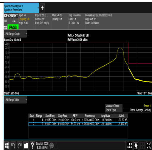
Band2-5MHz-QPSK-19175-1RB#24-PASS
