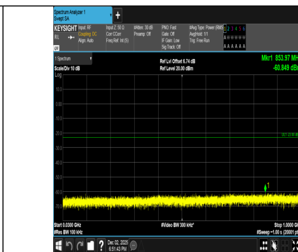
Band2-1.4MHz-QPSK-18607-1RB#5-30~1000-PASS
