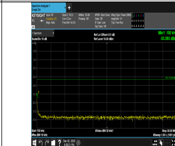
Band2-1.4MHz-QPSK-18900-6RB#0-0.15~30-PASS
