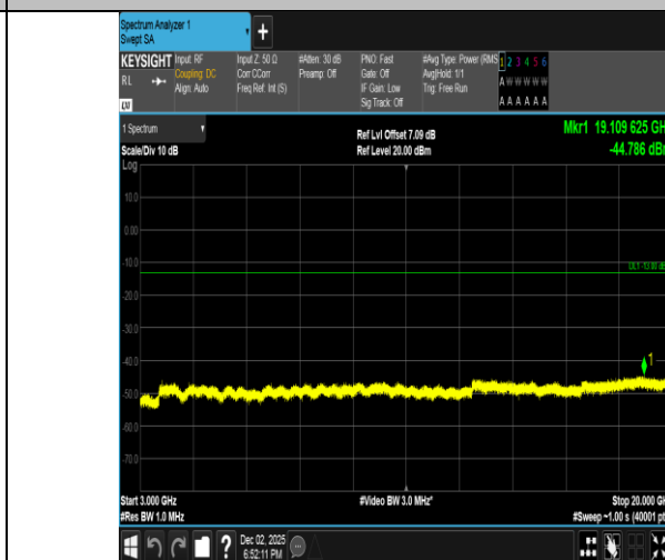
Band2-1.4MHz-QPSK-18607-1RB#5-3000~20000-PASS
