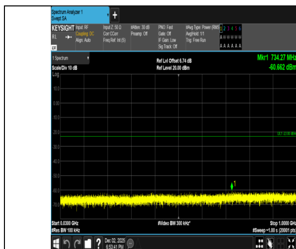
Band2-1.4MHz-QPSK-18607-6RB#0-30~1000-PASS
