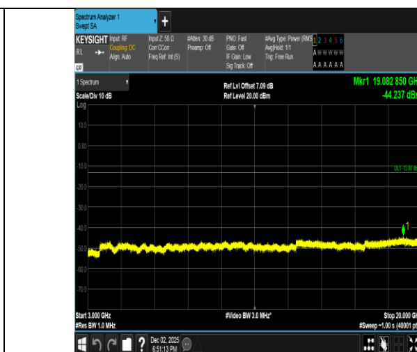
Band2-1.4MHz-16QAM-18607-1RB#0-3000~20000-PASS
