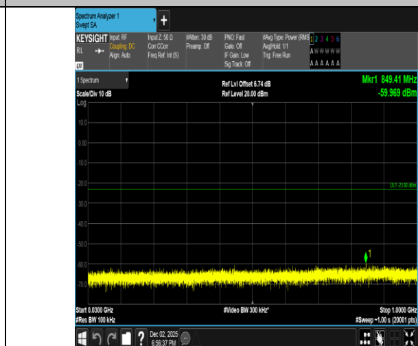
Band2-1.4MHz-16QAM-18900-1RB#0-30~1000-PASS
