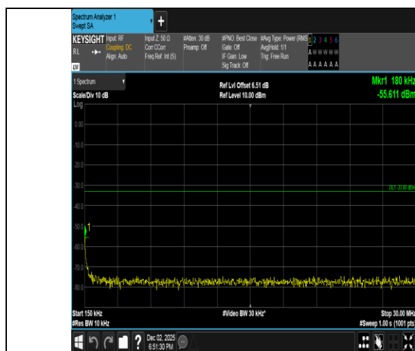
Band2-1.4MHz-QPSK-18607-1RB#5-0.15~30-PASS
