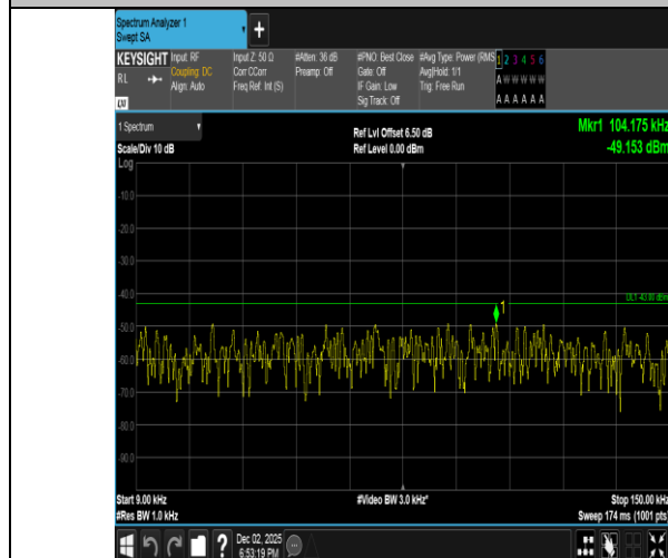
Band2-1.4MHz-QPSK-18607-6RB#0-0.009~0.15-PASS
