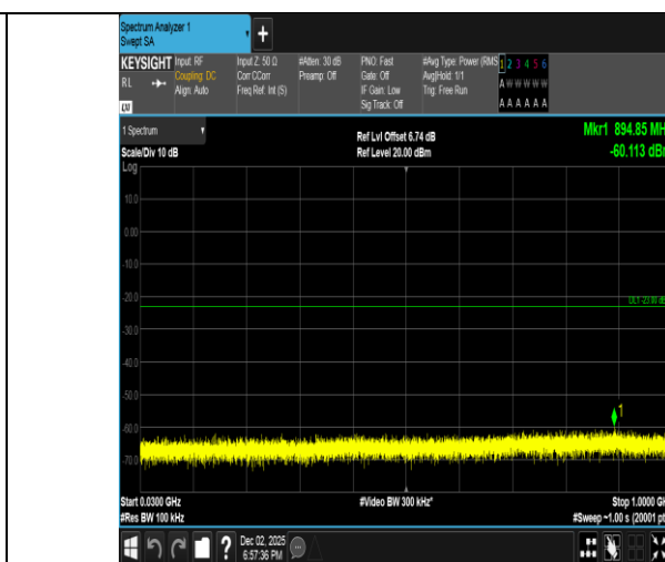
Band2-1.4MHz-QPSK-18900-1RB#5-30~1000-PASS
