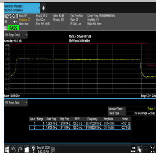
Band2-15MHz-16QAM-19125-75RB#0-PASS
