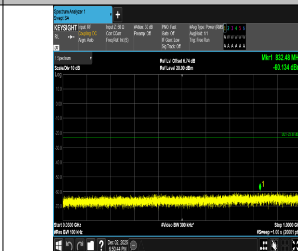
Band2-1.4MHz-16QAM-18607-1RB#0-30~1000-PASS
