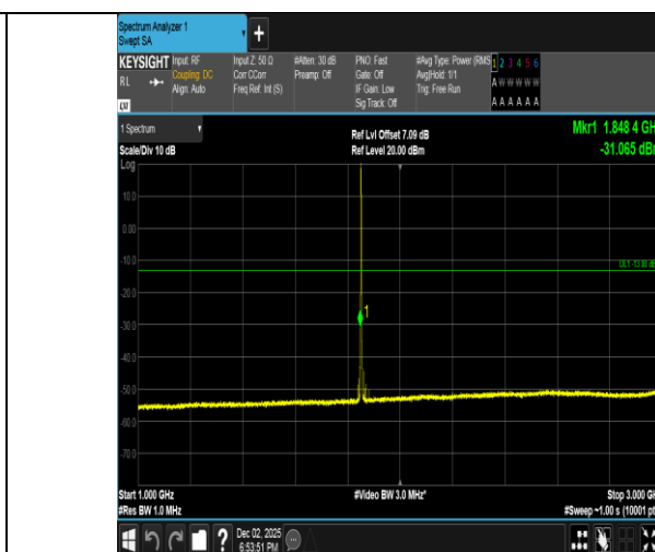
Band2-1.4MHz-QPSK-18607-6RB#0-1000~3000-PASS
