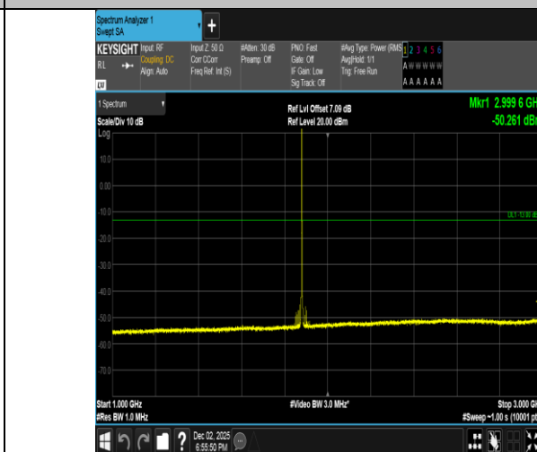
Band2-1.4MHz-QPSK-18900-1RB#0-1000~3000-PASS
