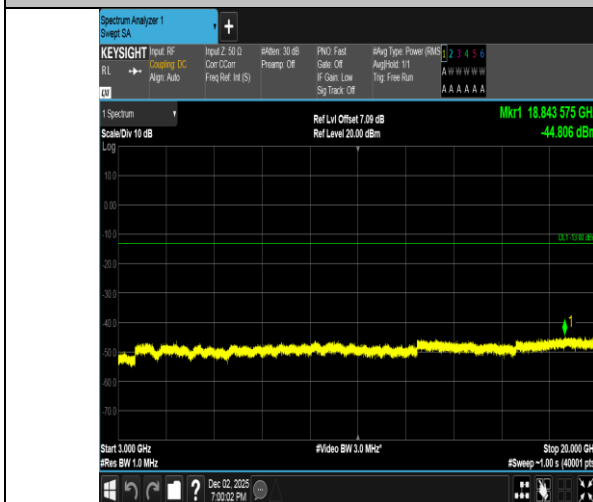
Band2-1.4MHz-QPSK-18900-6RB#0-3000~20000-PASS
