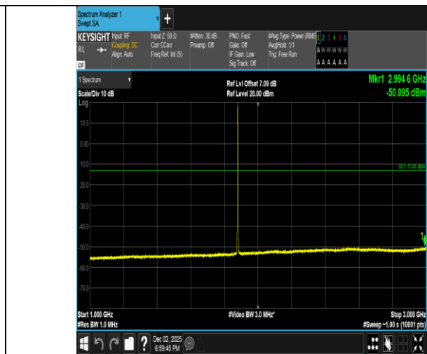
Band2-1.4MHz-QPSK-18900-6RB#0-1000~3000-PASS
