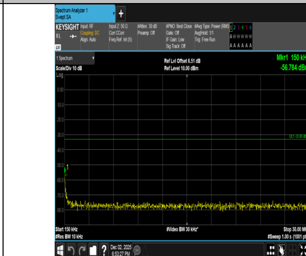
Band2-1.4MHz-QPSK-18607-6RB#0-0.15~30-PASS
