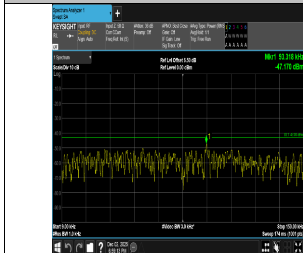
Band2-1.4MHz-QPSK-18900-6RB#0-0.009~0.15-PASS
