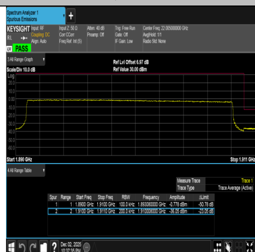
Band2-20MHz-16QAM-19100-100RB#0-PASS
