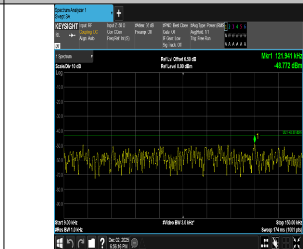
Band2-1.4MHz-16QAM-18900-1RB#0-0.009~0.15-PASS
