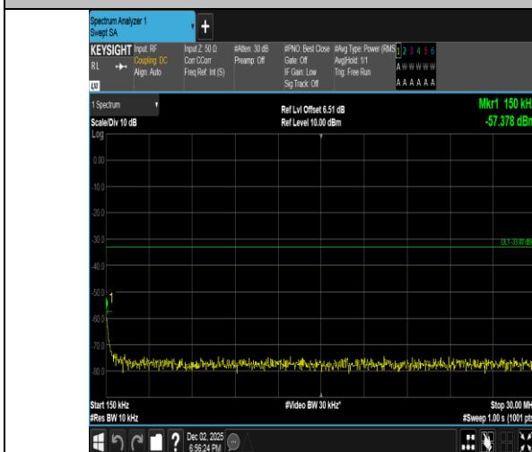
Band2-1.4MHz-16QAM-18900-1RB#0-0.15~30-PASS
