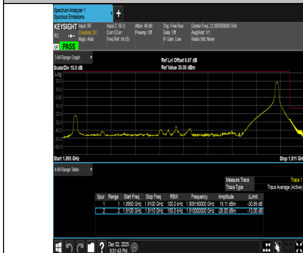
Band2-15MHz-16QAM-19125-1RB#74-PASS
