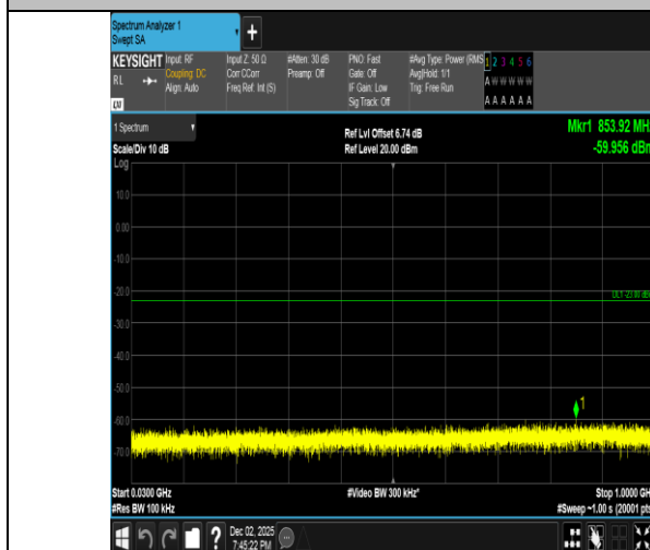
Band2-3MHz-16QAM-18900-1RB#14-30~1000-PASS
