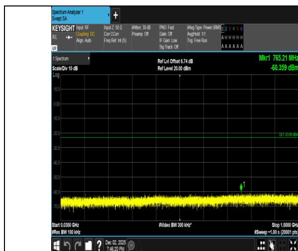
Band2-3MHz-QPSK-18900-15RB#0-30~1000-PASS
