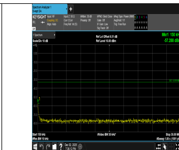
Band2-3MHz-QPSK-18615-1RB#0-0.15~30-PASS
