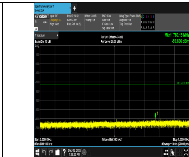
Band2-3MHz-QPSK-18615-1RB#14-30~1000-PASS
