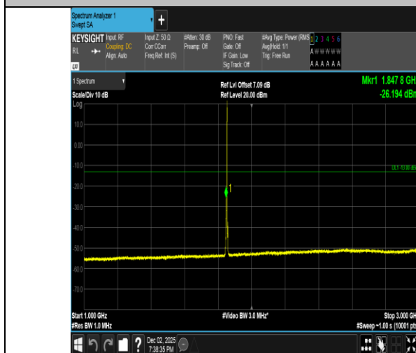
Band2-3MHz-QPSK-18615-1RB#14-1000~3000-PASS
