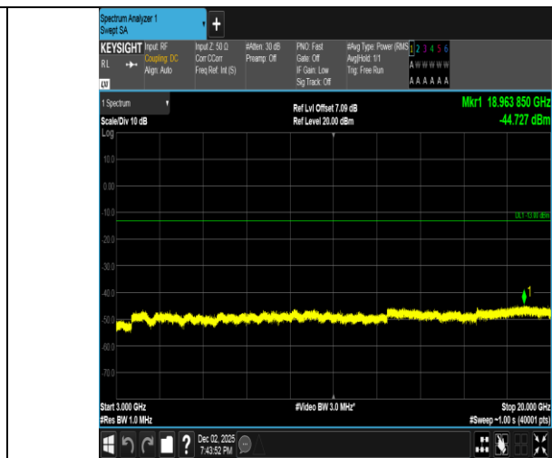
Band2-3MHz-16QAM-18900-1RB#0-3000~20000-PASS
