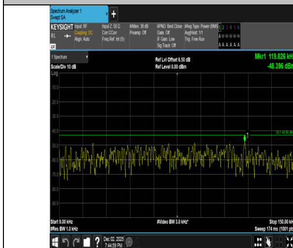
Band2-3MHz-16QAM-18900-1RB#14-0.009~0.15-PASS
