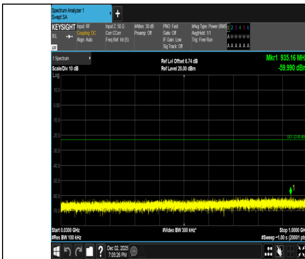
Band2-1.4MHz-QPSK-19193-6RB#0-30~1000-PASS
