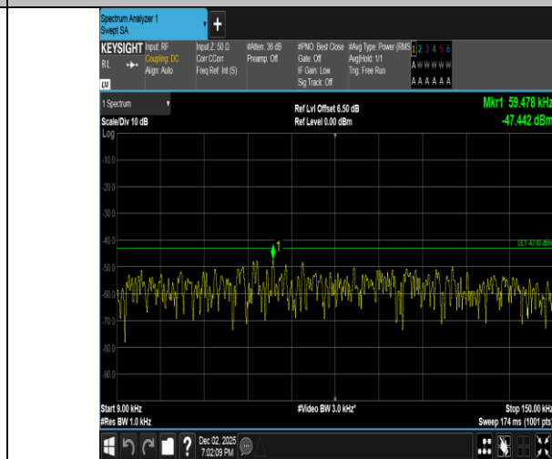
Band2-1.4MHz-16QAM-19193-1RB#0-0.009~0.15-PASS
