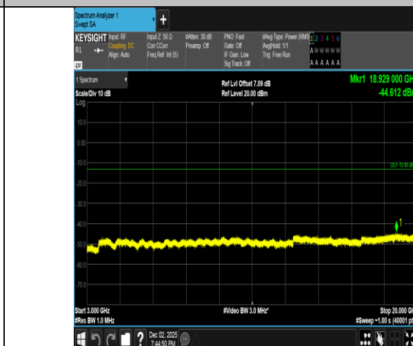
Band2-3MHz-QPSK-18900-1RB#14-3000~20000-PASS
