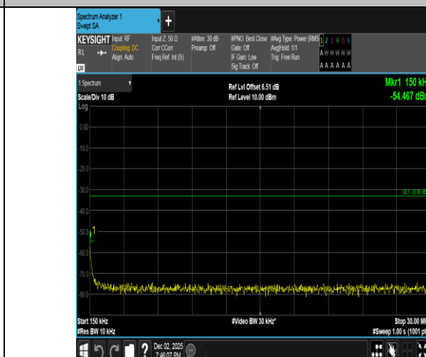
Band2-3MHz-QPSK-18900-15RB#0-0.15~30-PASS
