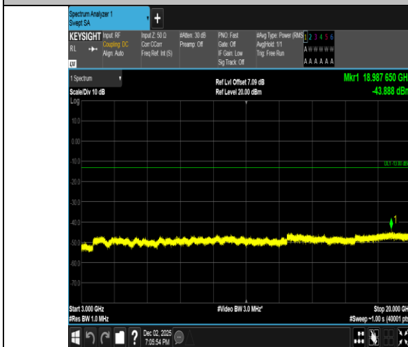
Band2-1.4MHz-QPSK-19193-6RB#0-3000~20000-PASS
