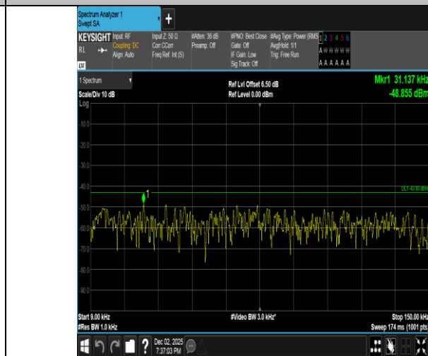
Band2-3MHz-16QAM-18615-1RB#0-0.009~0.15-PASS
