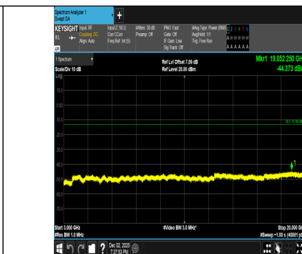
Band2-3MHz-16QAM-18615-1RB#0-3000~20000-PASS
