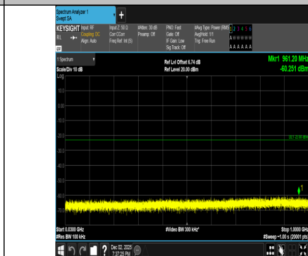
Band2-3MHz-16QAM-18615-1RB#0-30~1000-PASS
