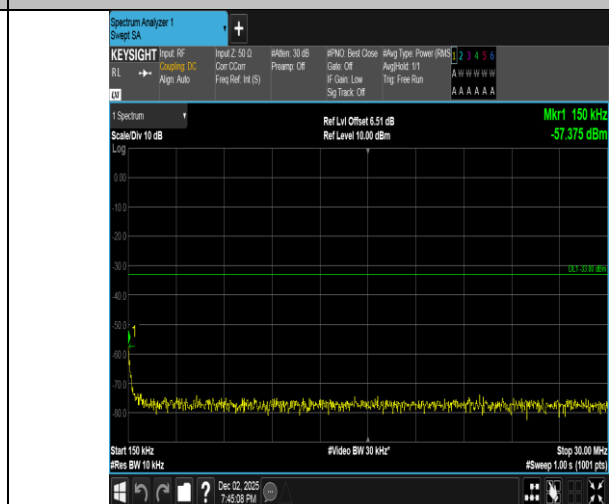
Band2-3MHz-16QAM-18900-1RB#14-0.15~30-PASS
