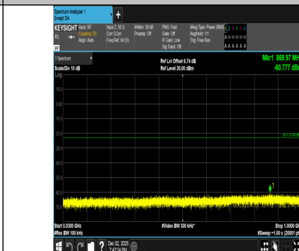
Band2-3MHz-16QAM-18900-1RB#0-30~1000-PASS
