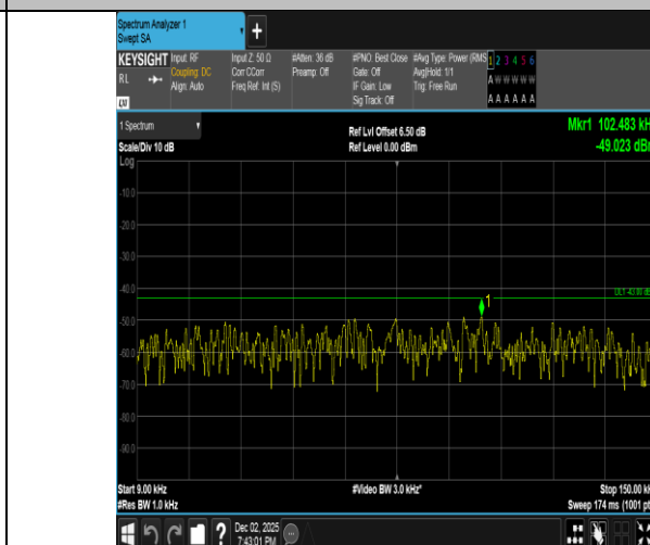
Band2-3MHz-16QAM-18900-1RB#0-0.009~0.15-PASS
