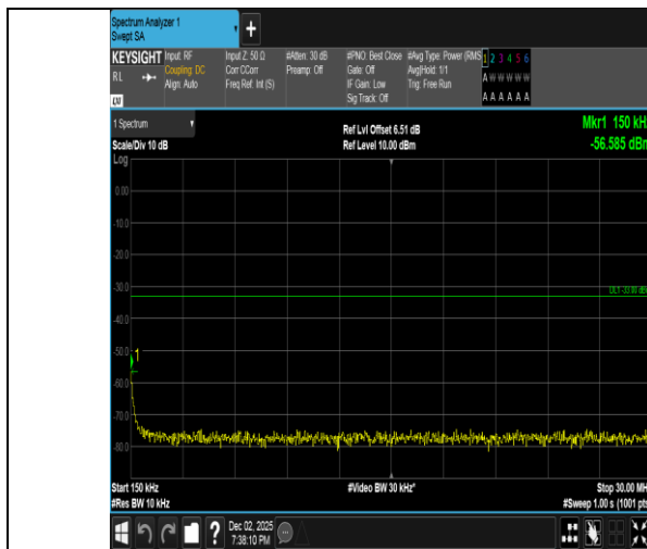
Band2-3MHz-QPSK-18615-1RB#14-0.15~30-PASS
