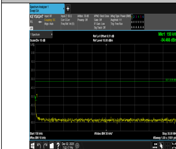
Band2-1.4MHz-16QAM-19193-1RB#0-0.15~30-PASS
