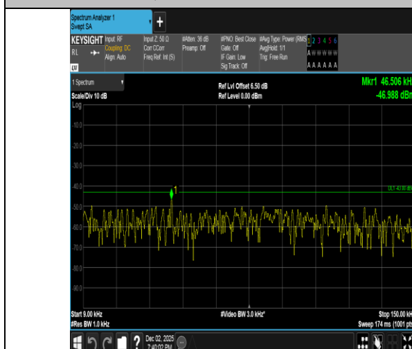
Band2-3MHz-QPSK-18615-15RB#0-0.009~0.15-PASS
