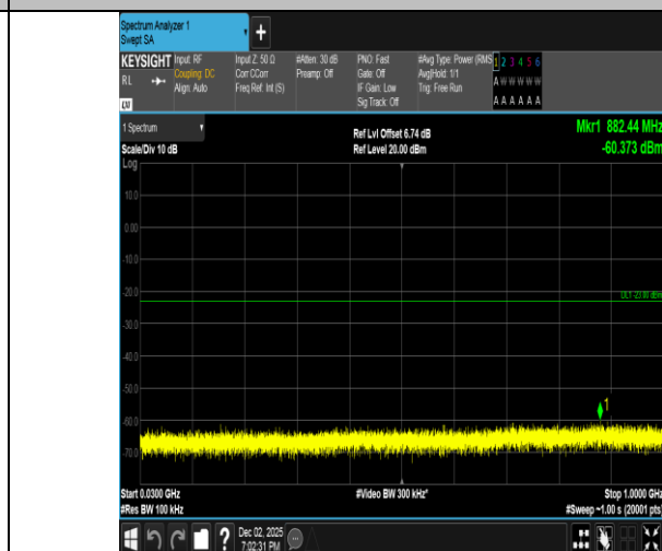
Band2-1.4MHz-16QAM-19193-1RB#0-30~1000-PASS
