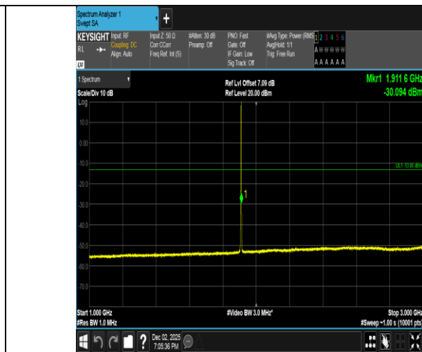
Band2-1.4MHz-QPSK-19193-6RB#0-1000~3000-PASS
