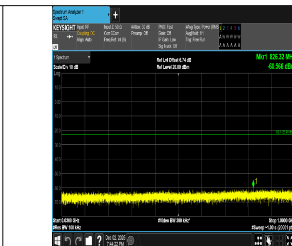
Band2-3MHz-QPSK-18900-1RB#14-30~1000-PASS
