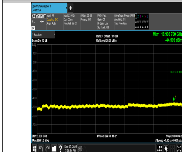
Band2-3MHz-QPSK-18615-1RB#0-3000~20000-PASS
