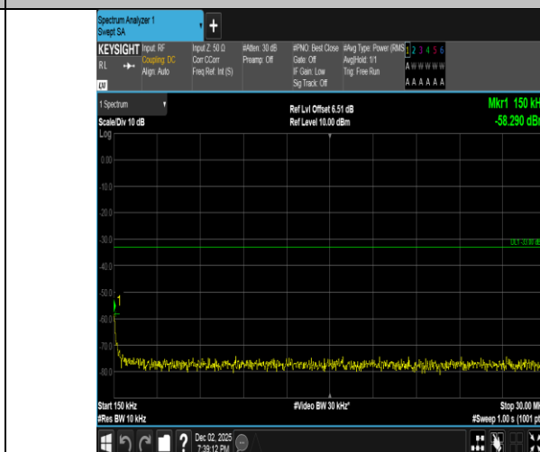
Band2-3MHz-16QAM-18615-1RB#14-0.15~30-PASS
