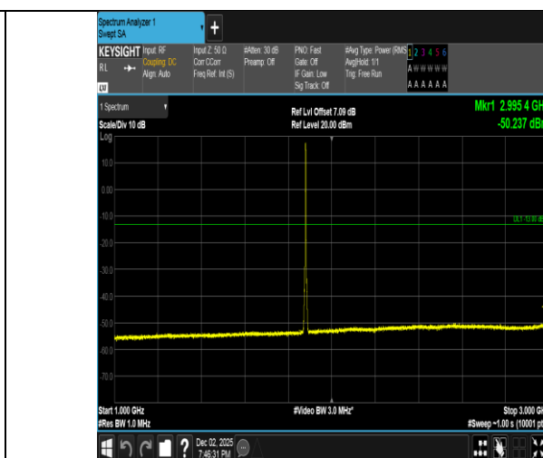
Band2-3MHz-QPSK-18900-15RB#0-1000~3000-PASS
