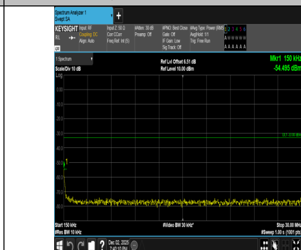
Band2-3MHz-QPSK-18615-15RB#0-0.15~30-PASS
