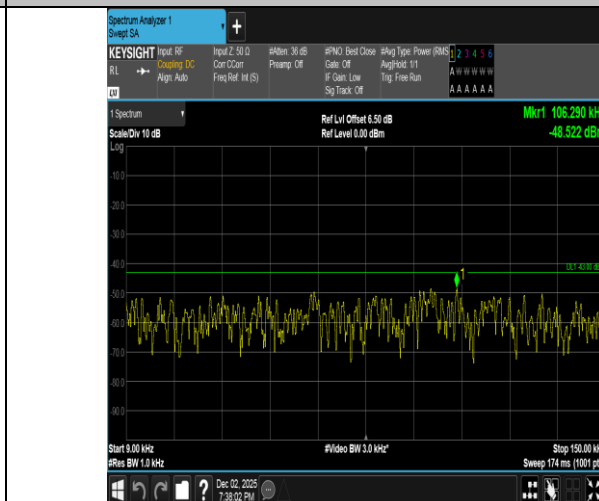
Band2-3MHz-QPSK-18615-1RB#14-0.009~0.15-PASS
