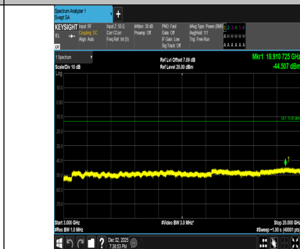
Band2-3MHz-QPSK-18615-1RB#14-3000~20000-PASS
