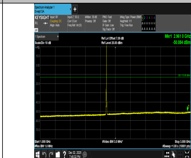
Band2-3MHz-16QAM-18900-1RB#14-1000~3000-PASS
