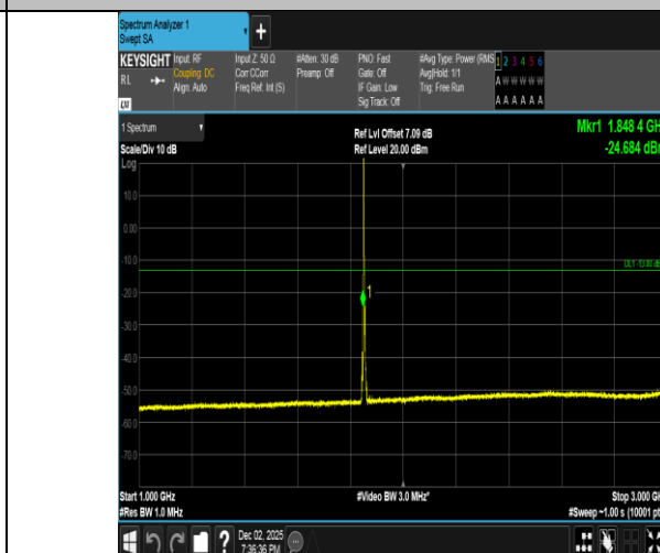
Band2-3MHz-QPSK-18615-1RB#0-1000~3000-PASS
