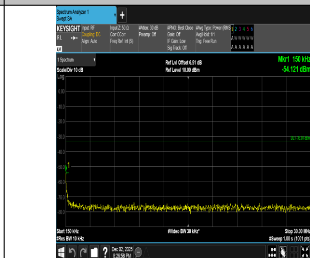
Band2-5MHz-QPSK-18625-25RB#0-0.15~30-PASS
