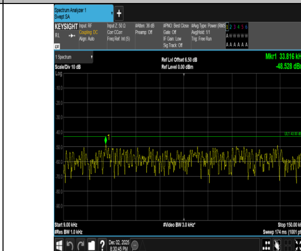
Band2-5MHz-QPSK-18900-1RB#24-0.009~0.15-PASS
