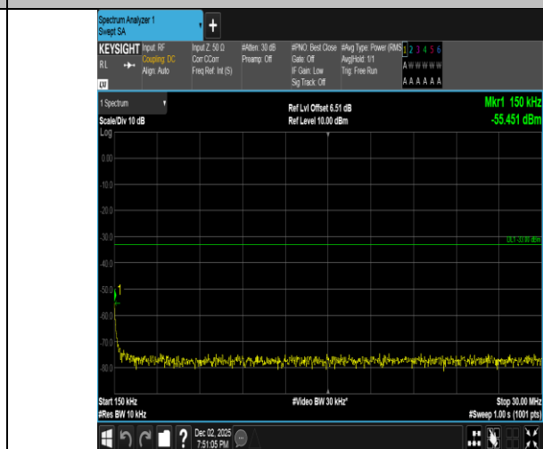
Band2-3MHz-16QAM-19185-1RB#14-0.15~30-PASS
