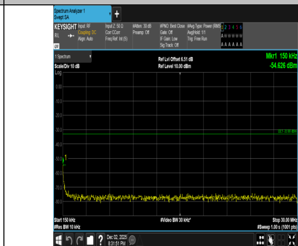
Band2-5MHz-16QAM-18900-1RB#24-0.15~30-PASS
