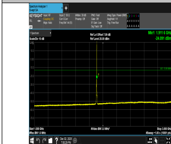
Band2-3MHz-QPSK-19185-1RB#14-1000~3000-PASS
