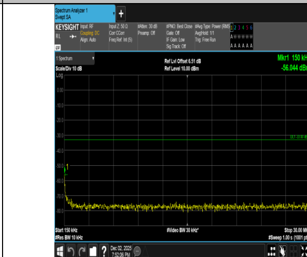
Band2-3MHz-QPSK-19185-15RB#0-0.15~30-PASS
