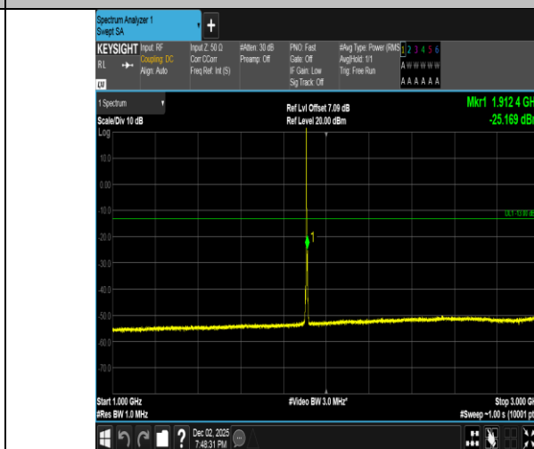
Band2-3MHz-QPSK-19185-1RB#0-1000~3000-PASS
