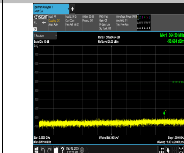
Band2-5MHz-16QAM-18900-1RB#0-30~1000-PASS
