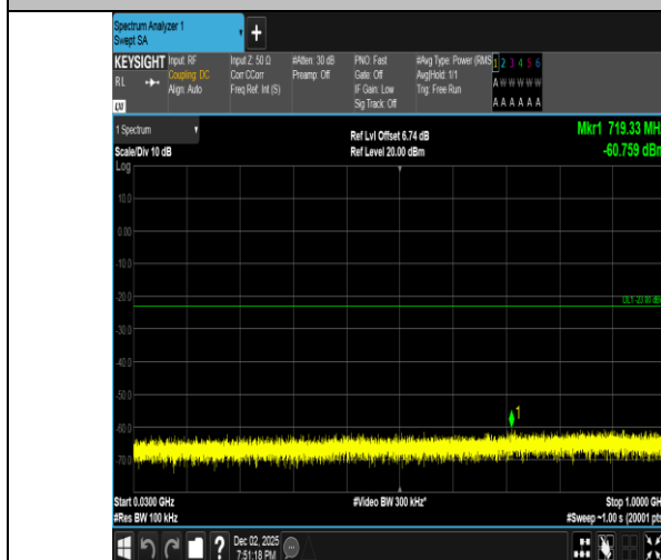
Band2-3MHz-16QAM-19185-1RB#14-30~1000-PASS
