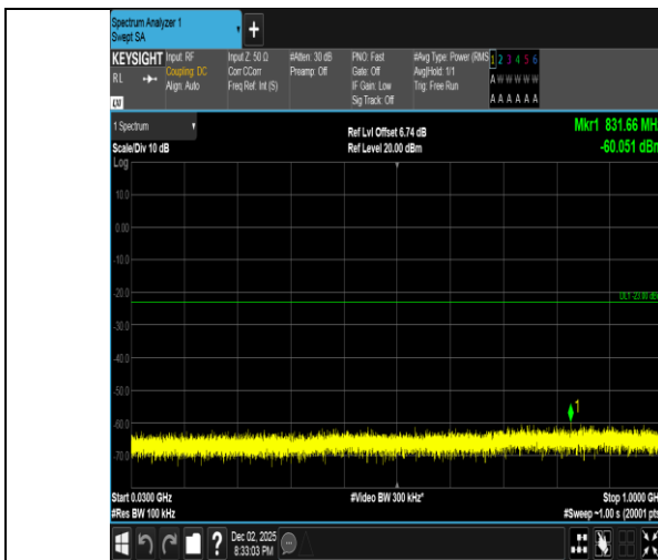
Band2-5MHz-QPSK-18900-25RB#0-30~1000-PASS
