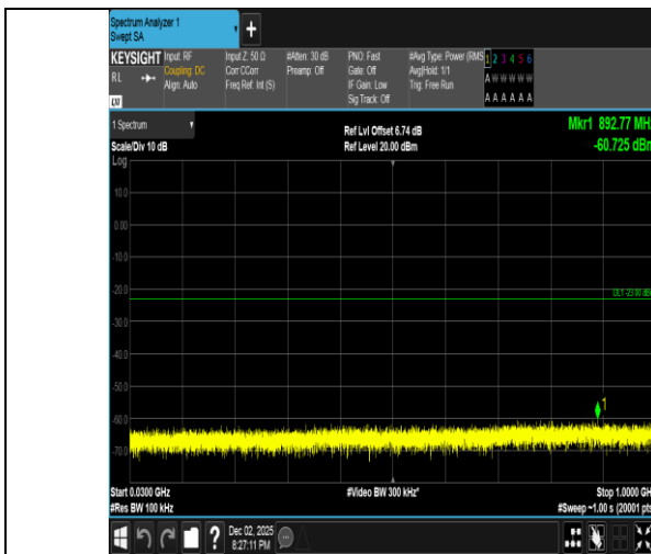
Band2-5MHz-QPSK-18625-25RB#0-30~1000-PASS
