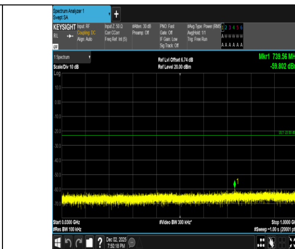
Band2-3MHz-QPSK-19185-1RB#14-30~1000-PASS
