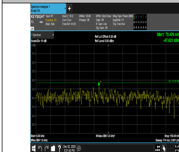
Band2-5MHz-16QAM-18900-1RB#24-0.009~0.15-PASS
