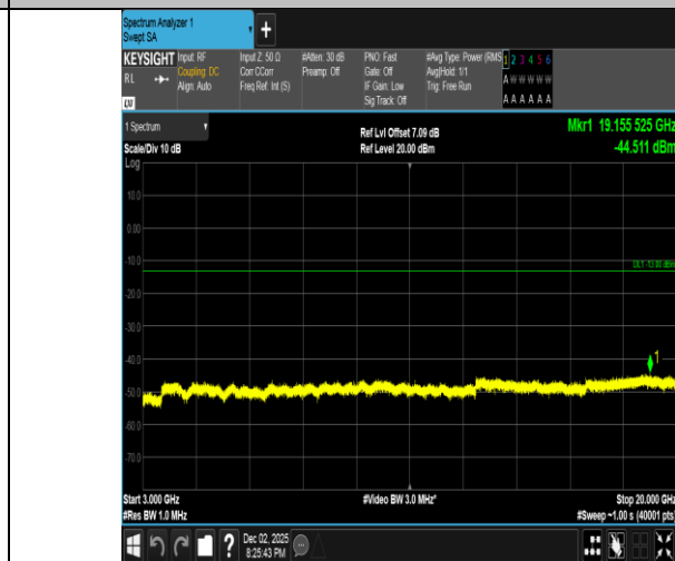
Band2-5MHz-QPSK-18625-1RB#24-3000~20000-PASS
