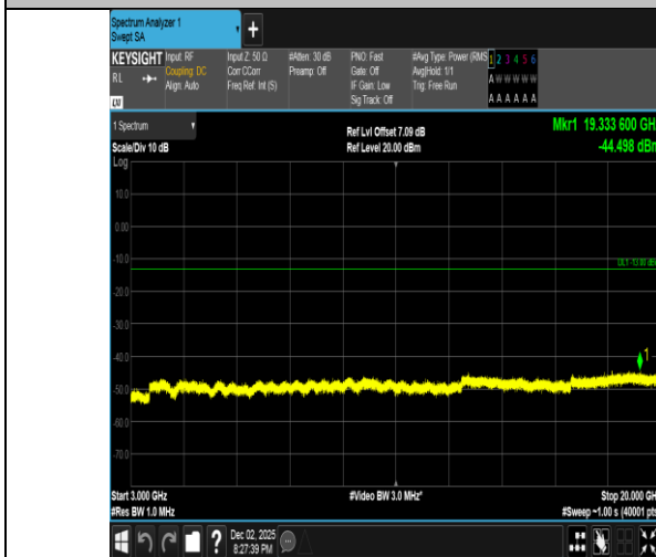
Band2-5MHz-QPSK-18625-25RB#0-3000~20000-PASS
