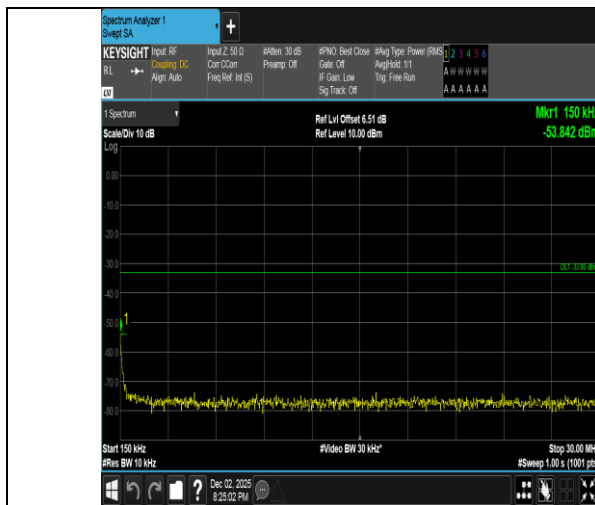
Band2-5MHz-QPSK-18625-1RB#24-0.15~30-PASS
