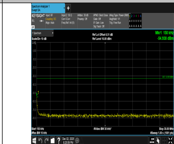
Band2-5MHz-16QAM-18625-1RB#24-0.15~30-PASS
