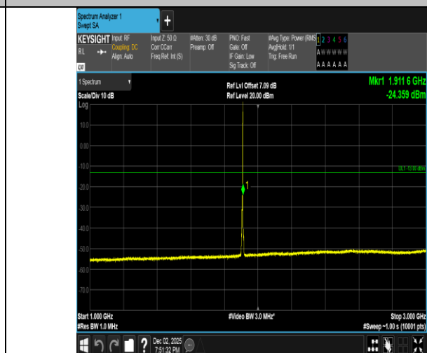
Band2-3MHz-16QAM-19185-1RB#14-1000~3000-PASS
