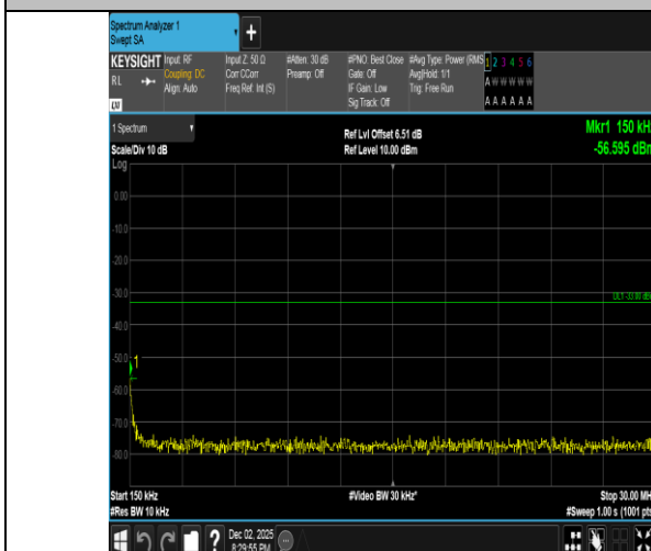
Band2-5MHz-16QAM-18900-1RB#0-0.15~30-PASS
