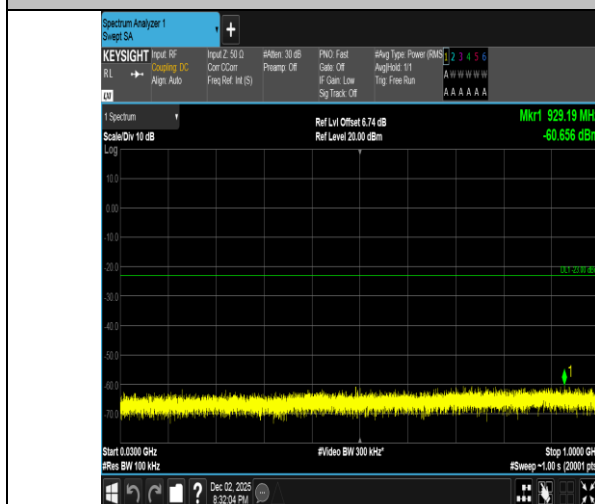
Band2-5MHz-16QAM-18900-1RB#24-30~1000-PASS
