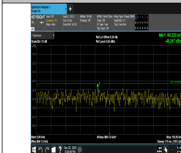
Band2-5MHz-QPSK-18625-25RB#0-0.009~0.15-PASS
