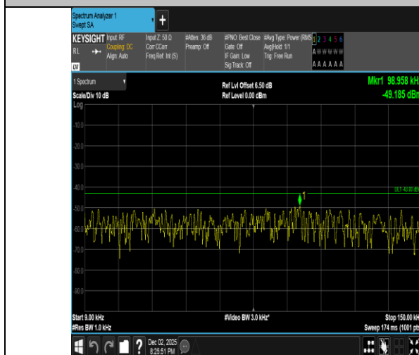
Band2-5MHz-16QAM-18625-1RB#24-0.009~0.15-PASS
