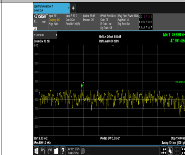
Band2-3MHz-QPSK-19185-1RB#14-0.009~0.15-PASS
