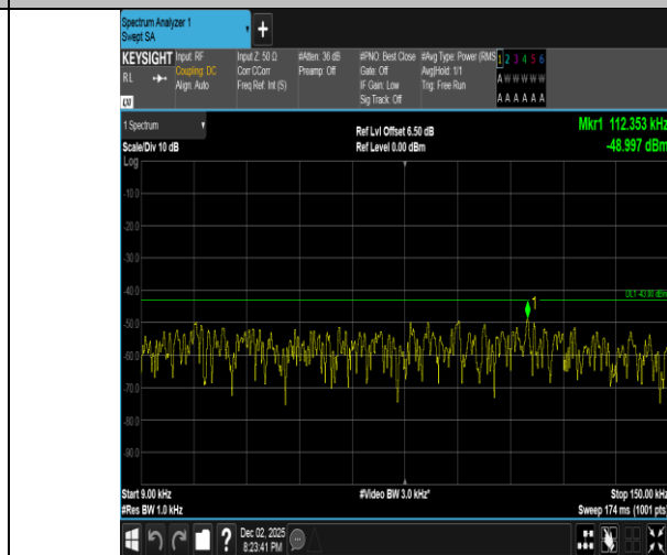
Band2-5MHz-16QAM-18625-1RB#0-0.009~0.15-PASS
