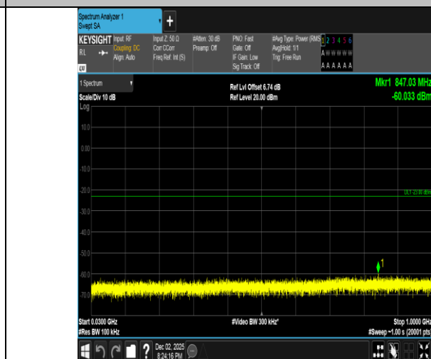
Band2-5MHz-16QAM-18625-1RB#0-30~1000-PASS
