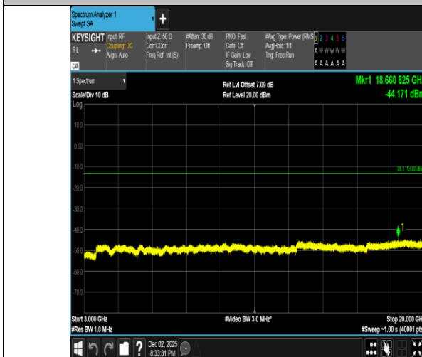
Band2-5MHz-QPSK-18900-25RB#0-3000~20000-PASS
