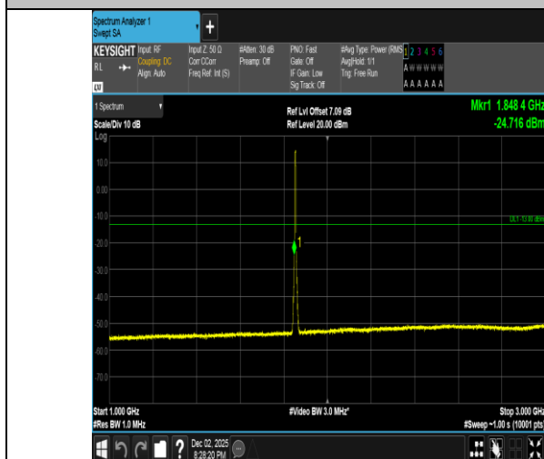
Band2-5MHz-16QAM-18625-25RB#0-1000~3000-PASS
