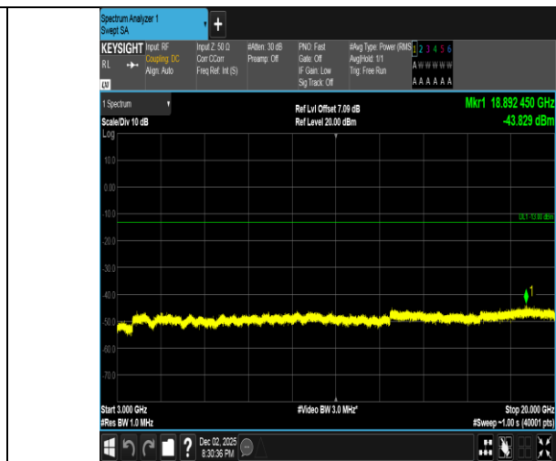
Band2-5MHz-16QAM-18900-1RB#0-3000~20000-PASS
