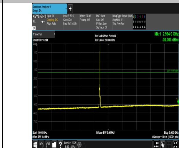
Band2-5MHz-16QAM-18900-1RB#24-1000~3000-PASS
