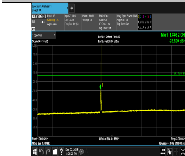
Band2-5MHz-QPSK-18625-1RB#24-1000~3000-PASS
