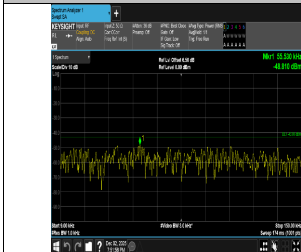
Band2-3MHz-QPSK-19185-15RB#0-0.009~0.15-PASS
