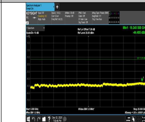
Band2-3MHz-QPSK-19185-1RB#14-3000~20000-PASS
