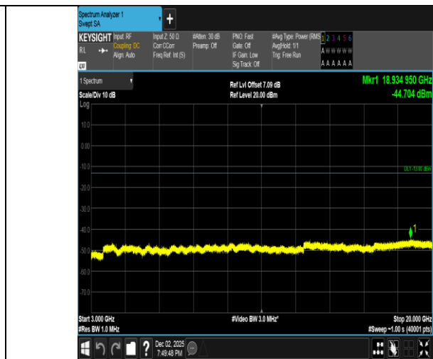
Band2-3MHz-16QAM-19185-1RB#0-3000~20000-PASS
