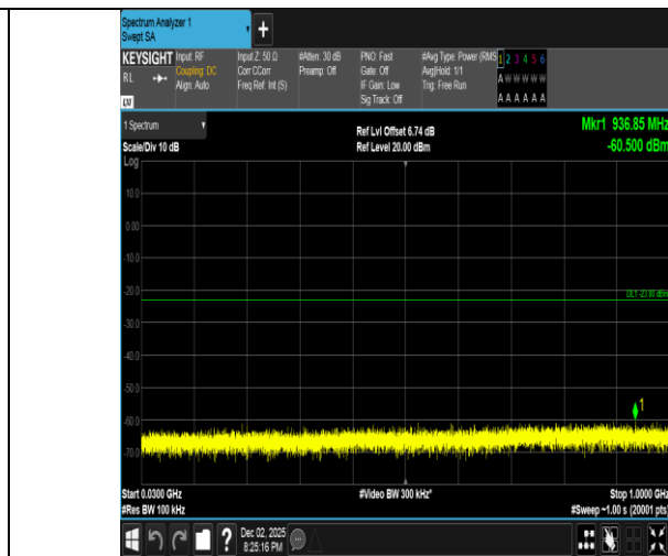
Band2-5MHz-QPSK-18625-1RB#24-30~1000-PASS
