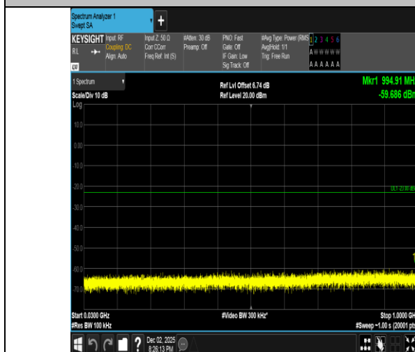
Band2-5MHz-16QAM-18625-1RB#24-30~1000-PASS
