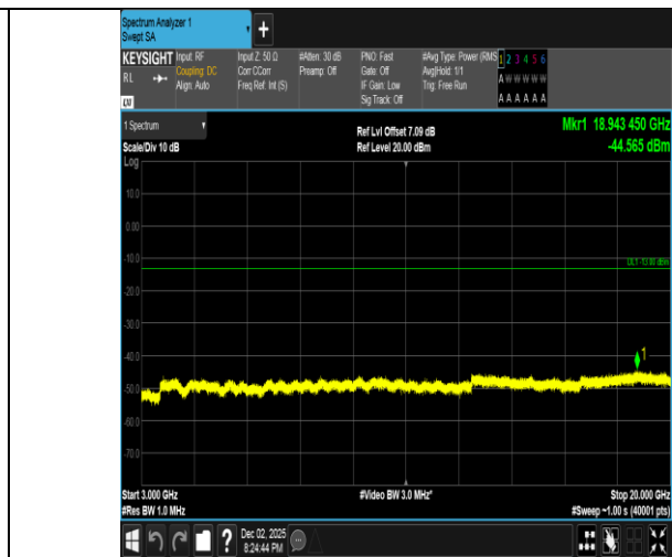
Band2-5MHz-16QAM-18625-1RB#0-3000~20000-PASS
