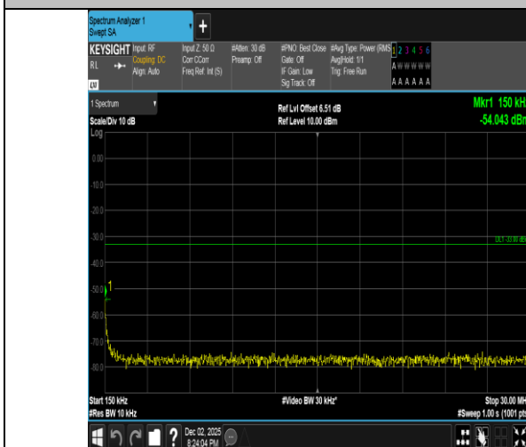
Band2-5MHz-16QAM-18625-1RB#0-0.15~30-PASS
