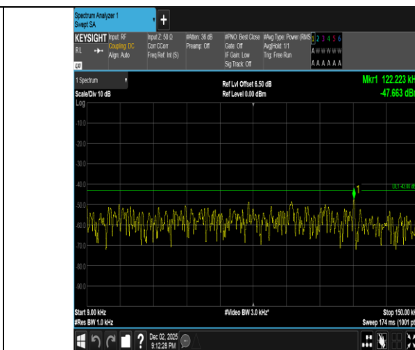
Band2-10MHz-16QAM-18650-50RB#0-0.009~0.15-PASS
