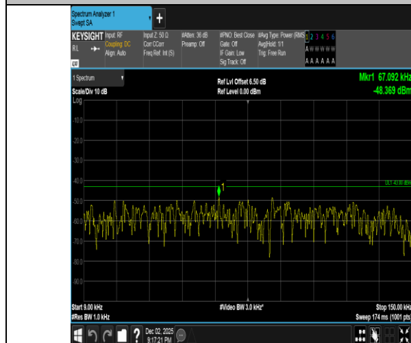
Band2-10MHz-QPSK-18900-50RB#0-0.009~0.15-PASS
