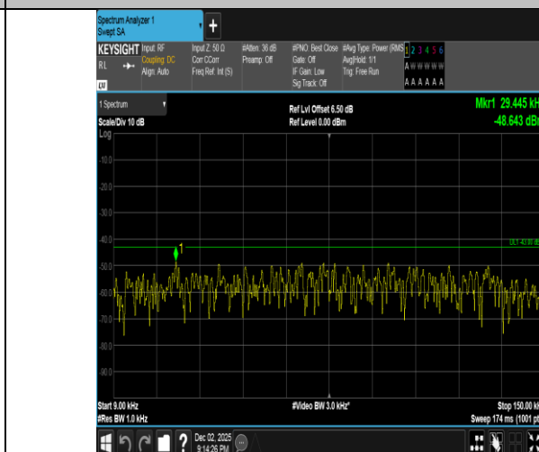
Band2-10MHz-16QAM-18900-1RB#0-0.009~0.15-PASS
