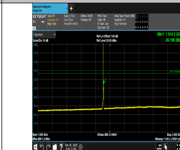
Band2-5MHz-QPSK-19175-1RB#0-1000~3000-PASS
