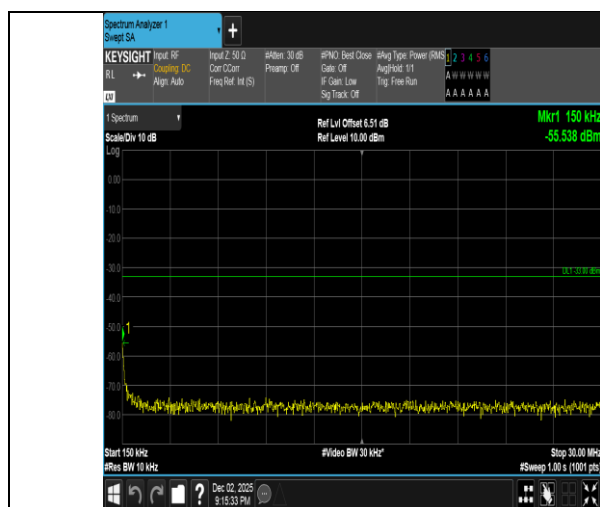
Band2-10MHz-QPSK-18900-1RB#49-0.15~30-PASS
