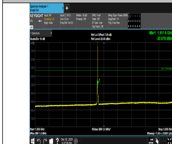
Band2-5MHz-QPSK-19175-1RB#24-1000~3000-PASS
