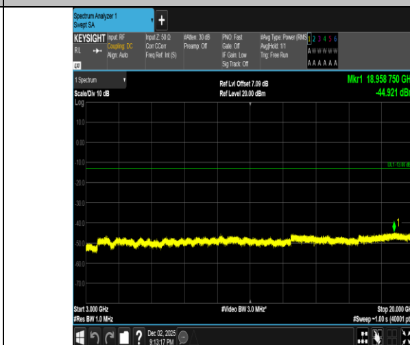
Band2-10MHz-16QAM-18650-50RB#0-3000~20000-PASS
