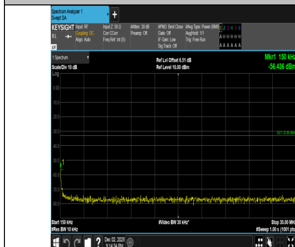
Band2-10MHz-16QAM-18900-1RB#0-0.15~30-PASS
