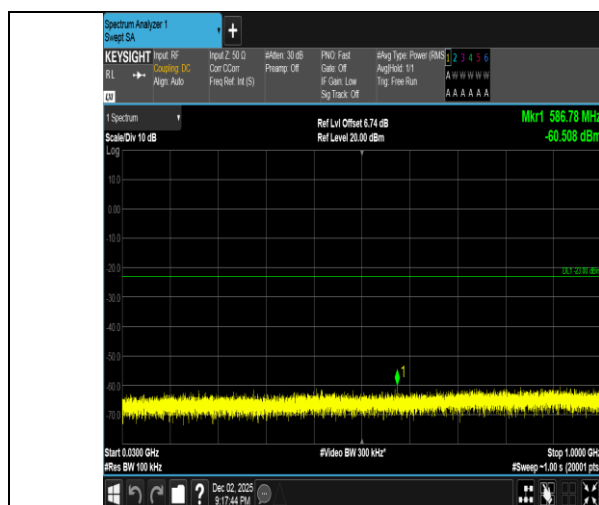
Band2-10MHz-QPSK-18900-50RB#0-30~1000-PASS
