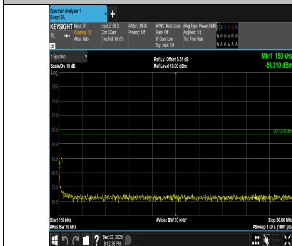
Band2-10MHz-16QAM-18650-50RB#0-0.15~30-PASS
