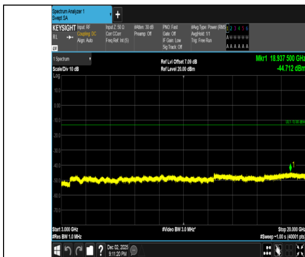
Band2-10MHz-16QAM-18650-1RB#49-3000~20000-PASS
