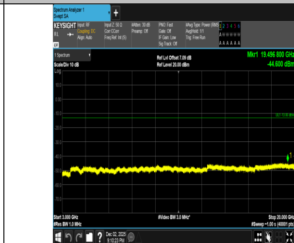
Band2-10MHz-QPSK-18650-1RB#49-3000~20000-PASS
