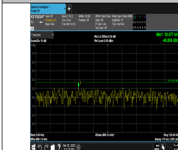
Band2-10MHz-QPSK-18650-50RB#0-0.009~0.15-PASS
