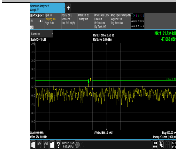
Band2-5MHz-16QAM-19175-1RB#24-0.009~0.15-PASS
