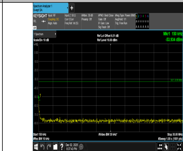
Band2-5MHz-16QAM-19175-1RB#24-0.15~30-PASS
