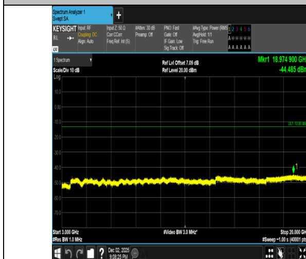
Band2-10MHz-QPSK-18650-1RB#0-3000~20000-PASS
