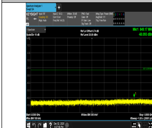
Band2-5MHz-16QAM-19175-1RB#24-30~1000-PASS
