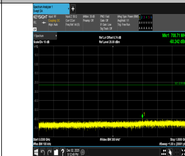
Band2-10MHz-16QAM-18650-50RB#0-30~1000-PASS
