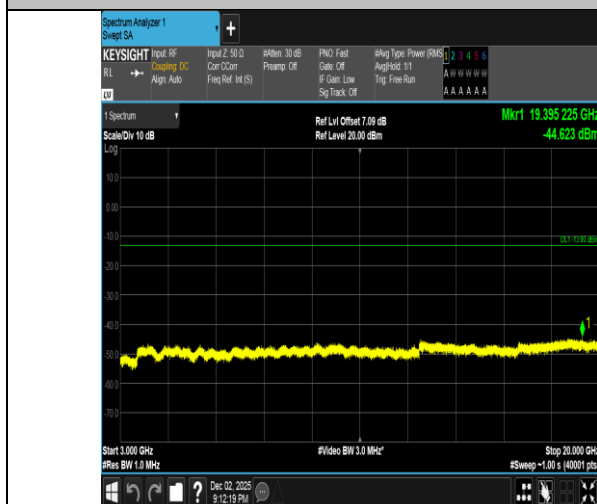
Band2-10MHz-QPSK-18650-50RB#0-3000~20000-PASS
