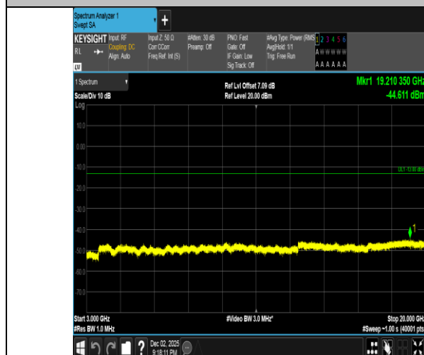
Band2-10MHz-QPSK-18900-50RB#0-3000~20000-PASS
