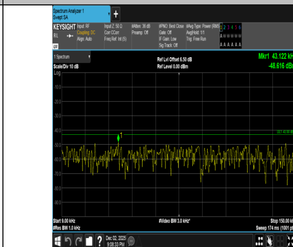
Band2-10MHz-16QAM-18650-1RB#0-0.009~0.15-PASS
