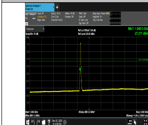
Band2-10MHz-16QAM-18650-50RB#0-1000~3000-PASS
