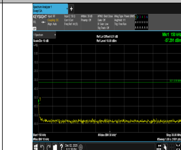
Band2-10MHz-QPSK-18650-50RB#0-0.15~30-PASS
