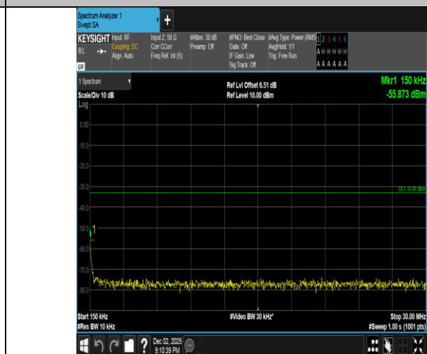
Band2-10MHz-16QAM-18650-1RB#49-0.15~30-PASS
