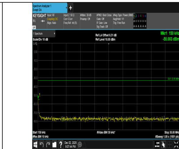
Band2-10MHz-QPSK-18650-1RB#0-0.15~30-PASS
