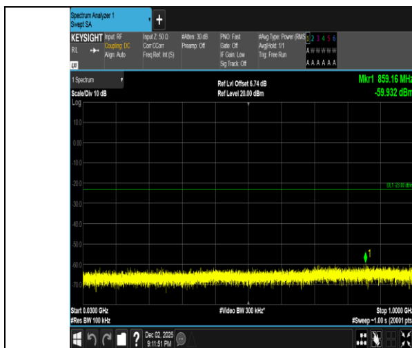
Band2-10MHz-QPSK-18650-50RB#0-30~1000-PASS
