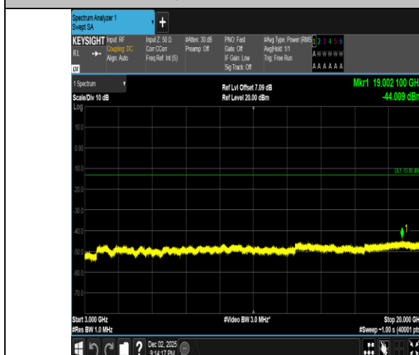
Band2-10MHz-QPSK-18900-1RB#0-3000~20000-PASS
