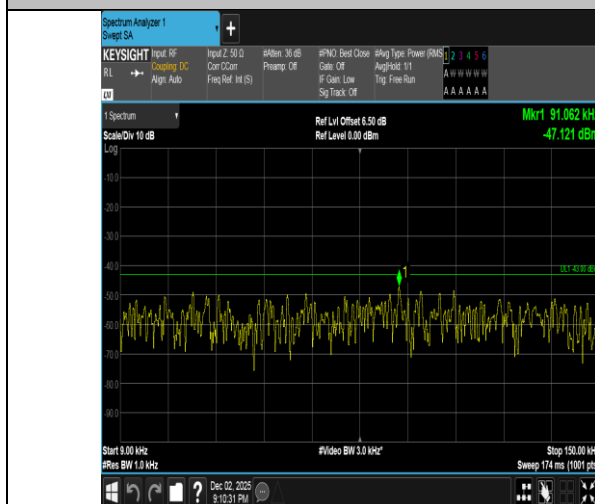
Band2-10MHz-16QAM-18650-1RB#49-0.009~0.15-PASS
