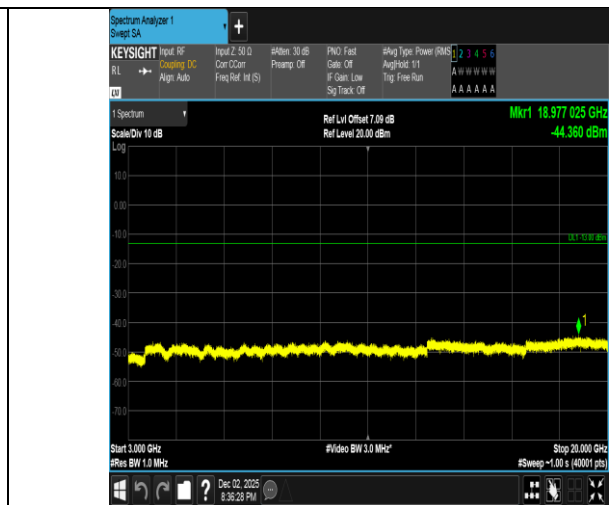
Band2-5MHz-16QAM-19175-1RB#0-3000~20000-PASS
