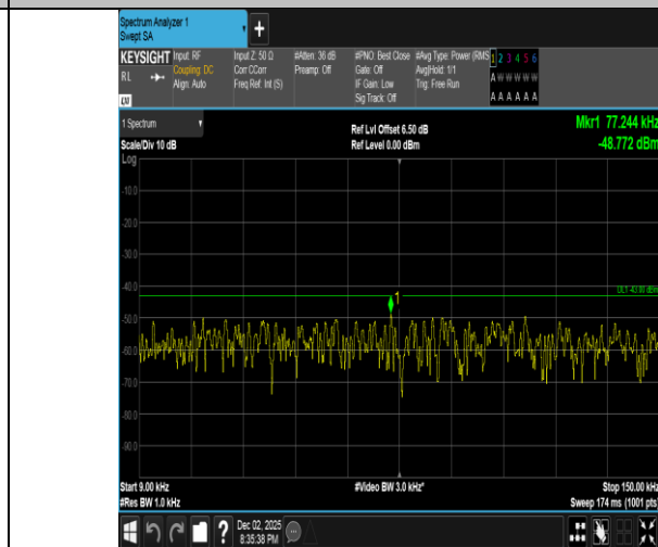
Band2-5MHz-16QAM-19175-1RB#0-0.009~0.15-PASS
