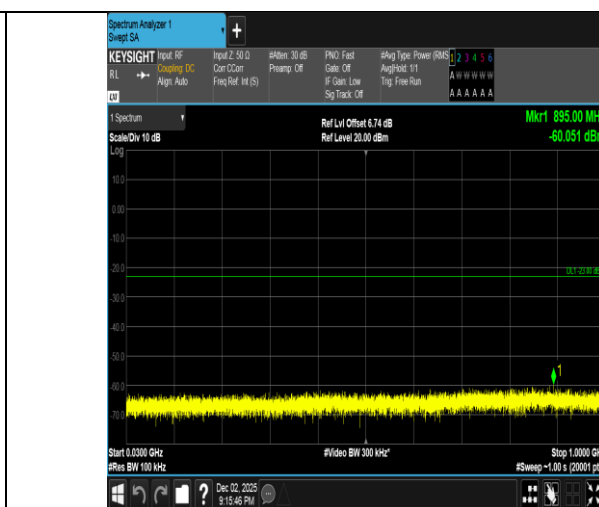
Band2-10MHz-QPSK-18900-1RB#49-30~1000-PASS
