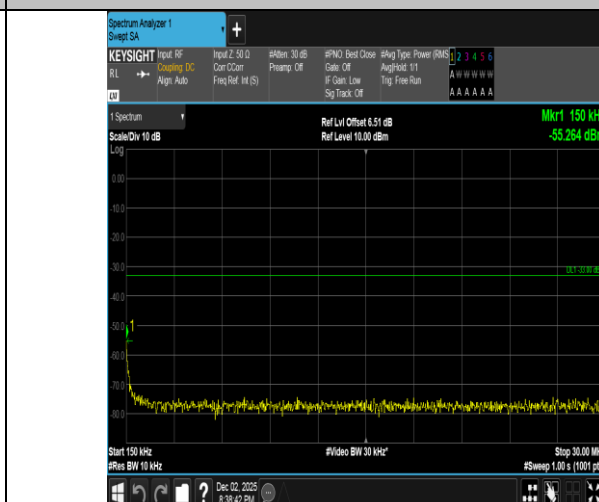
Band2-5MHz-QPSK-19175-25RB#0-0.15~30-PASS
