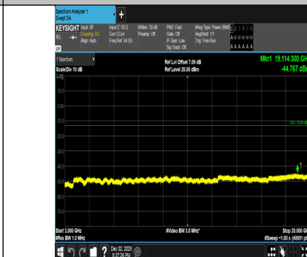
Band2-5MHz-QPSK-19175-1RB#24-3000~20000-PASS
