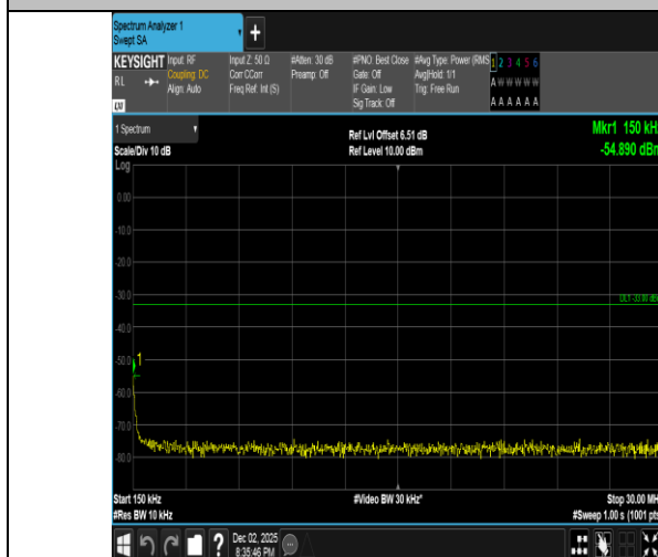
Band2-5MHz-16QAM-19175-1RB#0-0.15~30-PASS
