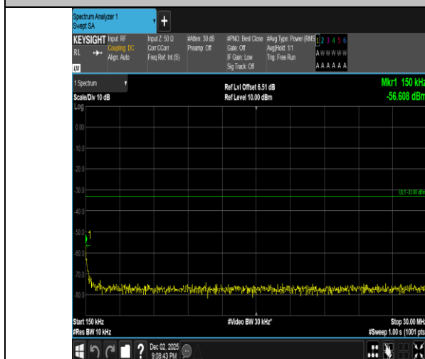
Band2-10MHz-16QAM-18650-1RB#0-0.15~30-PASS
