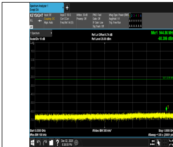
Band2-5MHz-QPSK-19175-25RB#0-30~1000-PASS
