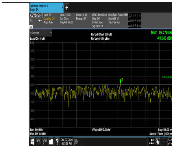
Band2-10MHz-QPSK-18650-1RB#0-0.009~0.15-PASS
