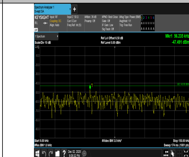
Band2-10MHz-QPSK-18650-1RB#49-0.009~0.15-PASS
