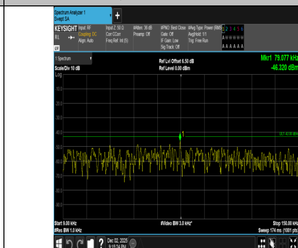
Band2-10MHz-QPSK-18900-1RB#49-0.009~0.15-PASS
