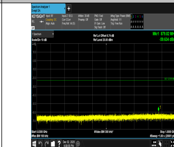
Band2-10MHz-16QAM-18650-1RB#0-30~1000-PASS
