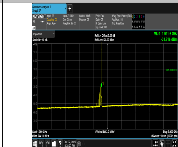
Band2-5MHz-16QAM-19175-1RB#24-1000~3000-PASS
