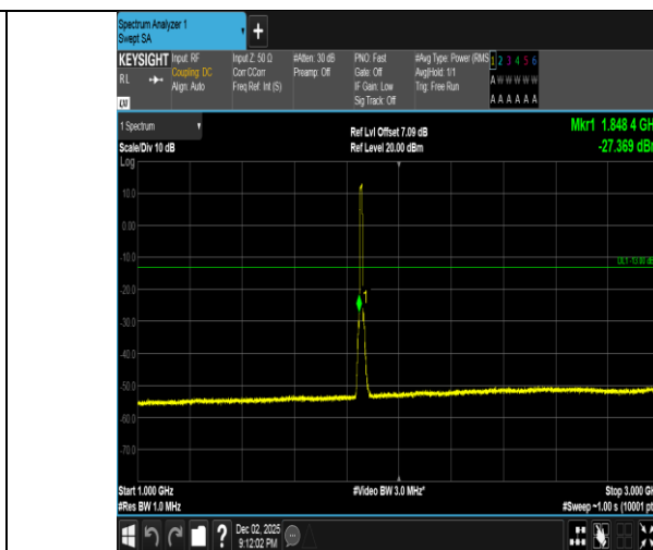
Band2-10MHz-QPSK-18650-50RB#0-1000~3000-PASS
