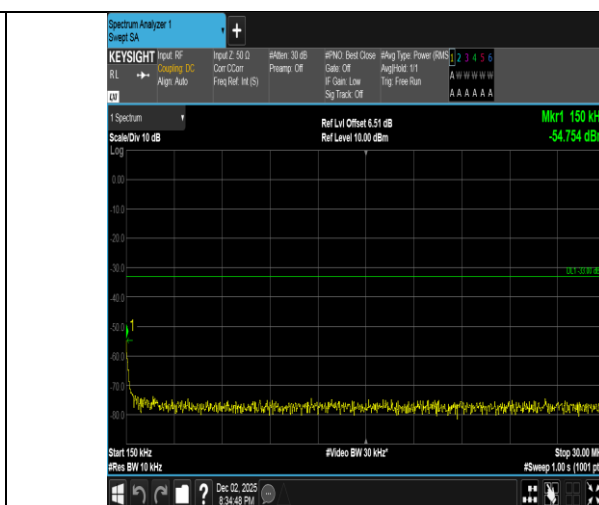
Band2-5MHz-QPSK-19175-1RB#0-0.15~30-PASS
