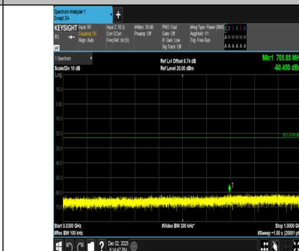
Band2-10MHz-16QAM-18900-1RB#0-30~1000-PASS
