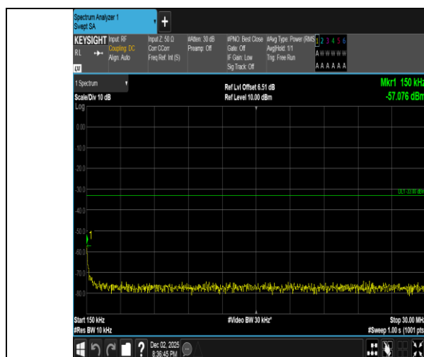
Band2-5MHz-QPSK-19175-1RB#24-0.15~30-PASS
