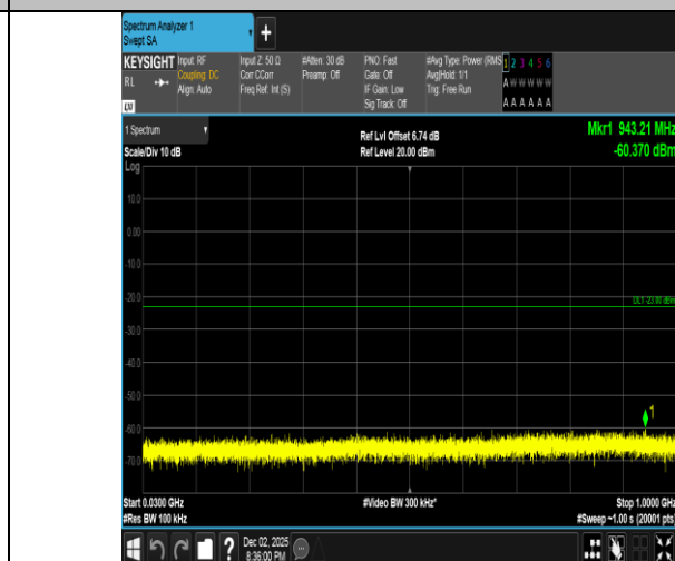
Band2-5MHz-16QAM-19175-1RB#0-30~1000-PASS
