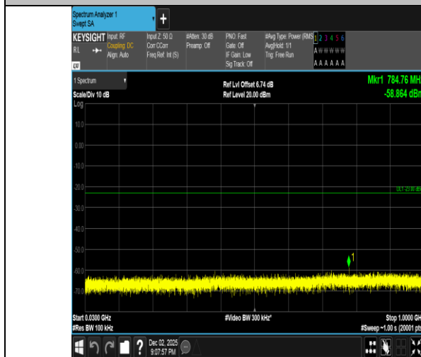
Band2-10MHz-QPSK-18650-1RB#0-30~1000-PASS
