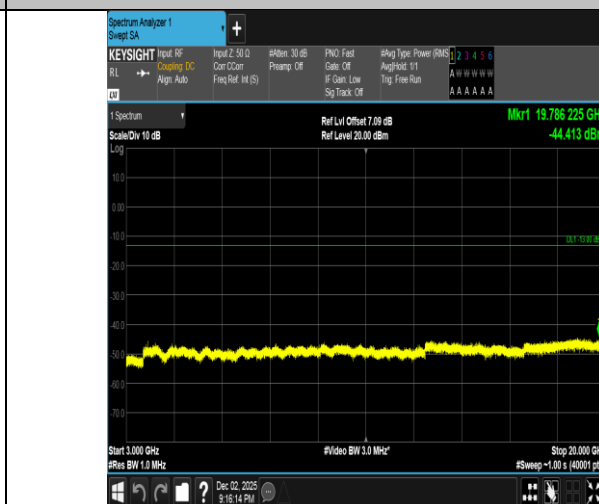
Band2-10MHz-QPSK-18900-1RB#49-3000~20000-PASS
