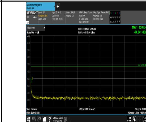
Band2-10MHz-QPSK-18900-50RB#0-0.15~30-PASS
