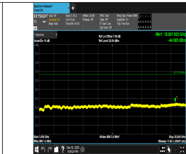
Band2-10MHz-16QAM-18650-1RB#0-3000~20000-PASS
