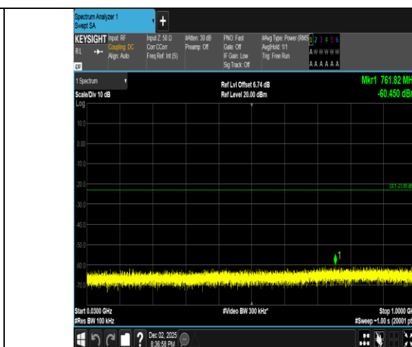
Band2-5MHz-QPSK-19175-1RB#24-30~1000-PASS
