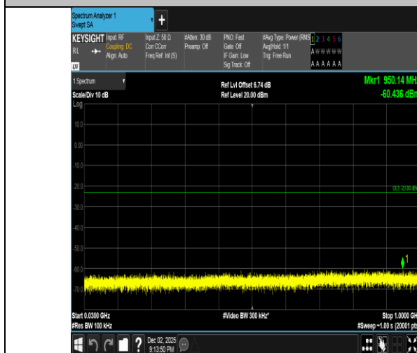
Band2-10MHz-QPSK-18900-1RB#0-30~1000-PASS
