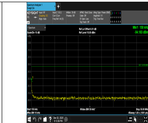
Band2-10MHz-QPSK-18900-1RB#0-0.15~30-PASS
