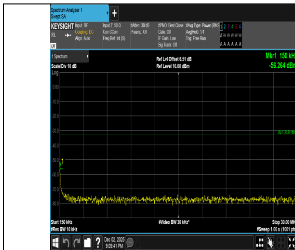
Band2-10MHz-QPSK-18650-1RB#49-0.15~30-PASS
