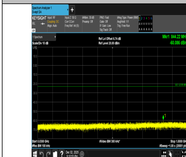
Band2-10MHz-16QAM-18650-1RB#49-30~1000-PASS
