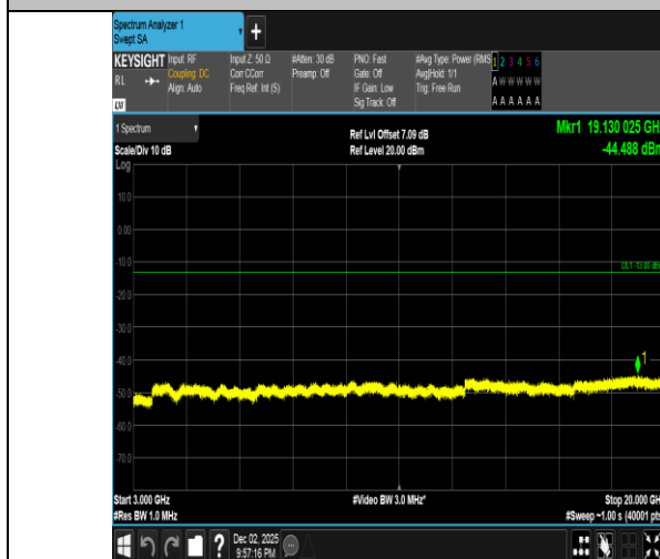
Band2-15MHz-QPSK-18675-75RB#0-3000~20000-PASS
