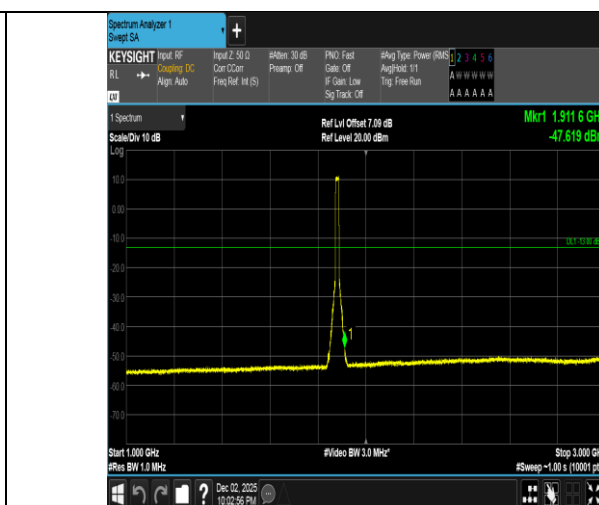
Band2-15MHz-QPSK-18900-75RB#0-1000~3000-PASS
