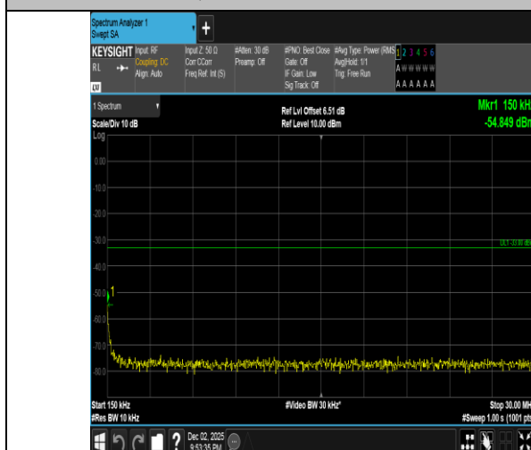
Band2-15MHz-16QAM-18675-1RB#0-0.15~30-PASS
