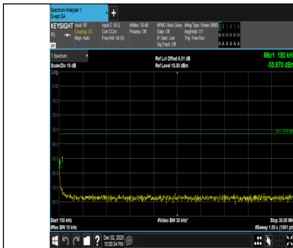
Band2-15MHz-QPSK-18900-1RB#74-0.15~30-PASS
