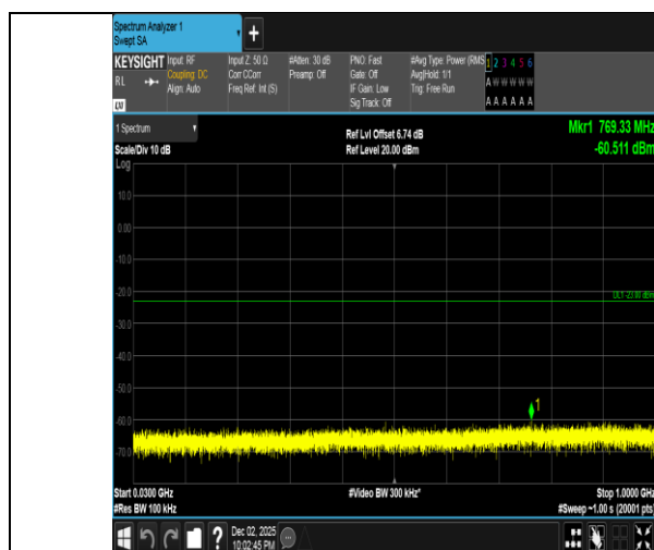
Band2-15MHz-QPSK-18900-75RB#0-30~1000-PASS
