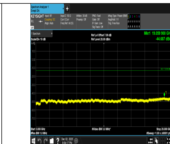
Band2-15MHz-16QAM-18675-1RB#0-3000~20000-PASS
