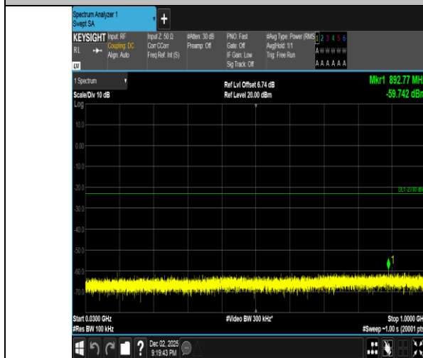
Band2-10MHz-QPSK-19150-1RB#0-30~1000-PASS
