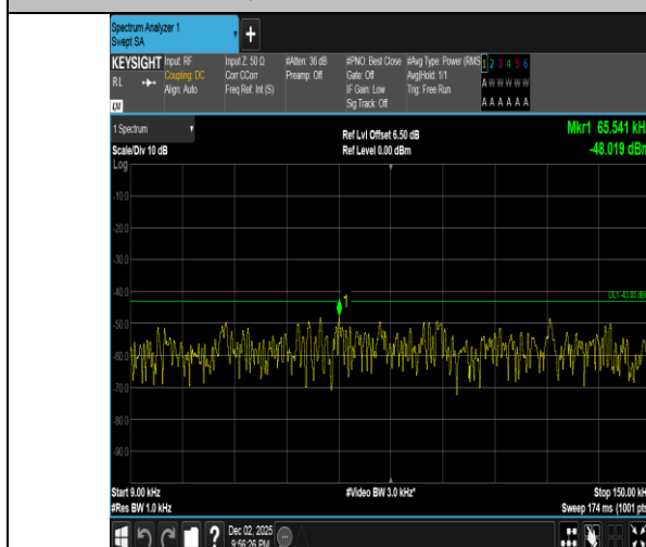
Band2-15MHz-QPSK-18675-75RB#0-0.009~0.15-PASS
