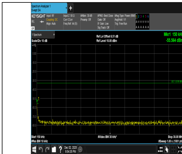
Band2-15MHz-QPSK-18675-1RB#74-0.15~30-PASS
