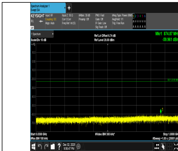
Band2-15MHz-QPSK-18675-75RB#0-30~1000-PASS
