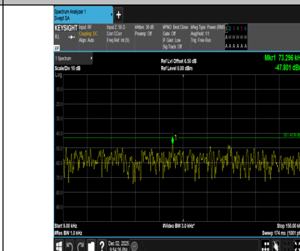
Band2-15MHz-QPSK-18675-1RB#74-0.009~0.15-PASS
