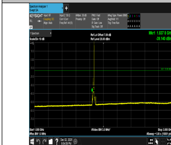
Band2-15MHz-QPSK-18675-1RB#74-1000~3000-PASS
