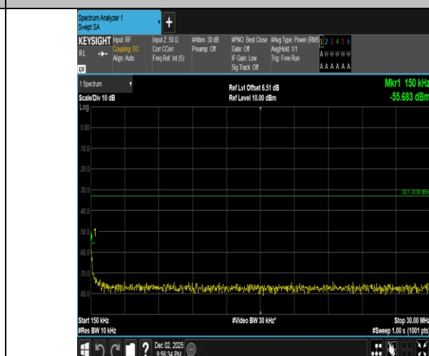
Band2-15MHz-QPSK-18675-75RB#0-0.15~30-PASS
