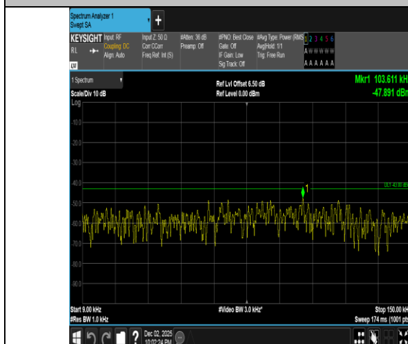
Band2-15MHz-QPSK-18900-75RB#0-0.009~0.15-PASS
