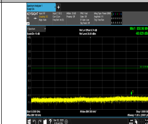
Band2-15MHz-16QAM-18900-1RB#0-30~1000-PASS
