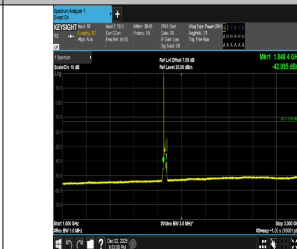
Band2-15MHz-QPSK-18675-1RB#0-1000~3000-PASS
