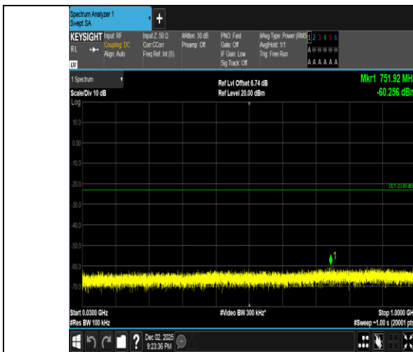
Band2-10MHz-QPSK-19150-50RB#0-30~1000-PASS
