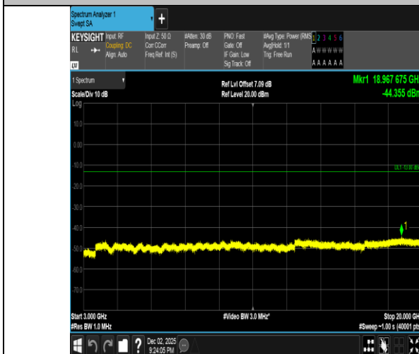
Band2-10MHz-QPSK-19150-50RB#0-3000~20000-PASS
