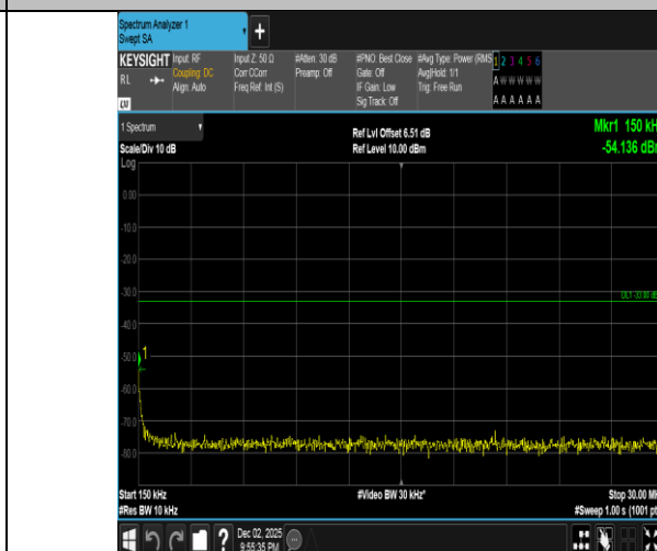
Band2-15MHz-16QAM-18675-1RB#74-0.15~30-PASS
