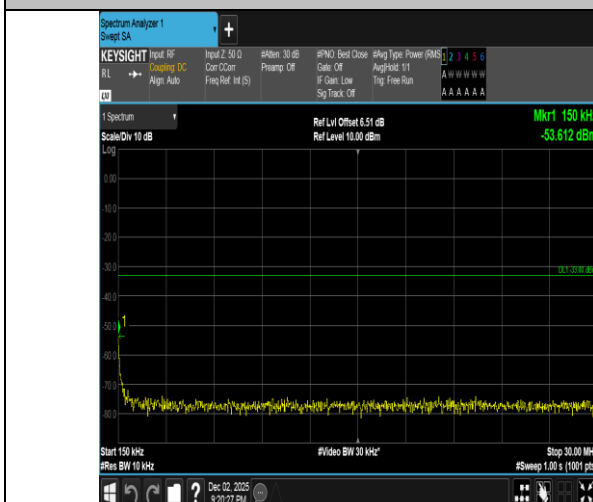
Band2-10MHz-16QAM-19150-1RB#0-0.15~30-PASS
