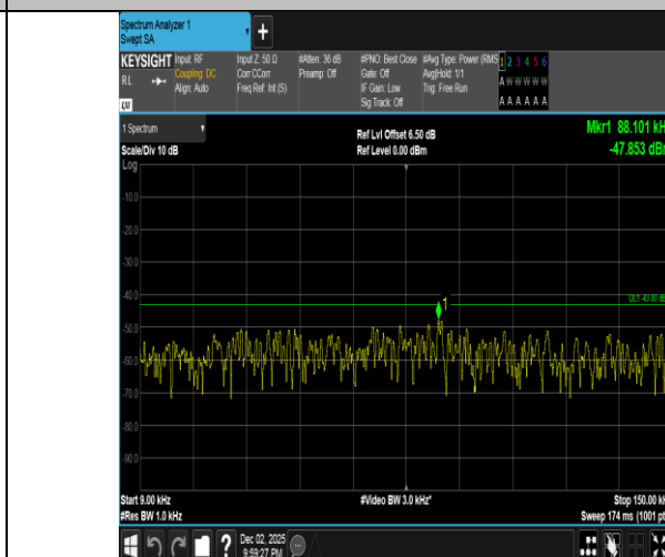
Band2-15MHz-16QAM-18900-1RB#0-0.009~0.15-PASS
