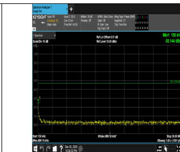
Band2-15MHz-QPSK-19125-1RB#0-0.15~30-PASS
