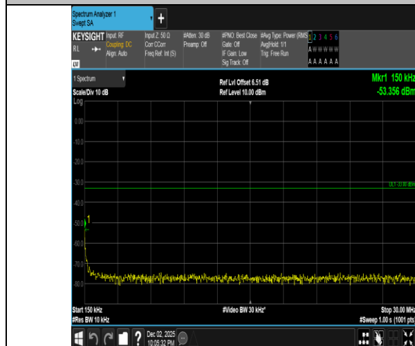
Band2-15MHz-16QAM-19125-1RB#0-0.15~30-PASS
