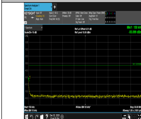
Band2-20MHz-16QAM-18900-1RB#0-0.15~30-PASS
