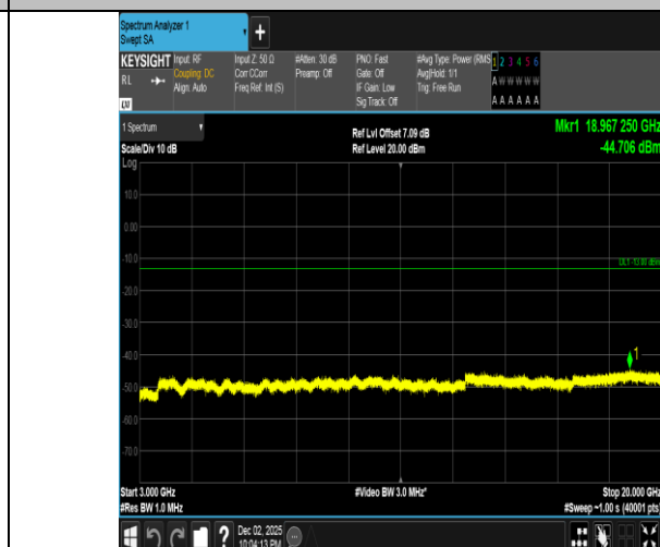
Band2-15MHz-16QAM-18900-75RB#0-3000~20000-PASS
