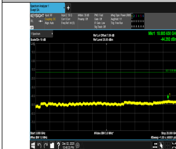
Band2-20MHz-QPSK-18900-100RB#0-3000~20000-PASS
