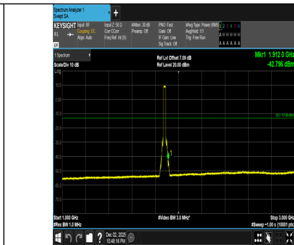
Band2-20MHz-QPSK-18900-100RB#0-1000~3000-PASS
