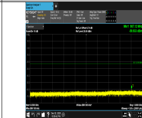
Band2-15MHz-16QAM-19125-75RB#0-30~1000-PASS
