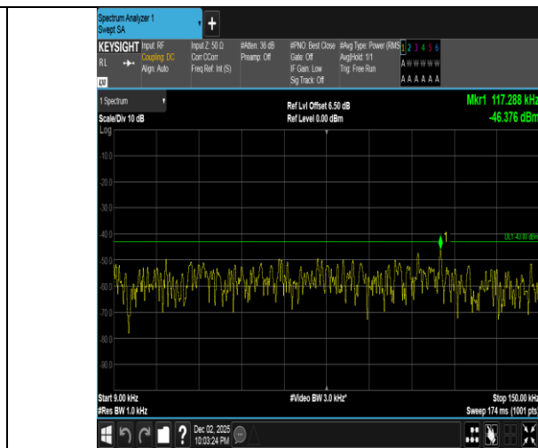
Band2-15MHz-16QAM-18900-75RB#0-0.009~0.15-PASS
