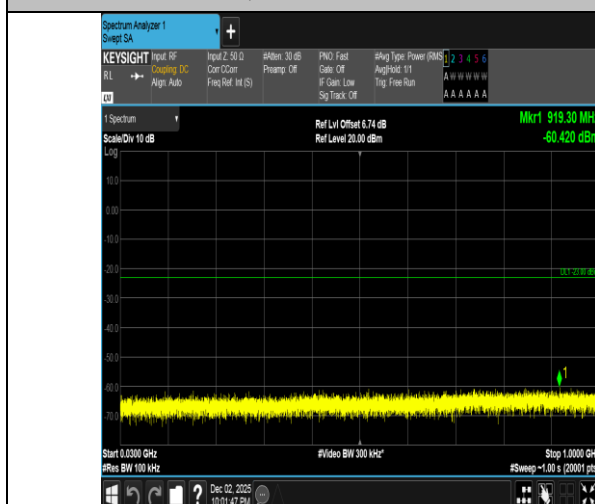
Band2-15MHz-16QAM-18900-1RB#74-30~1000-PASS
