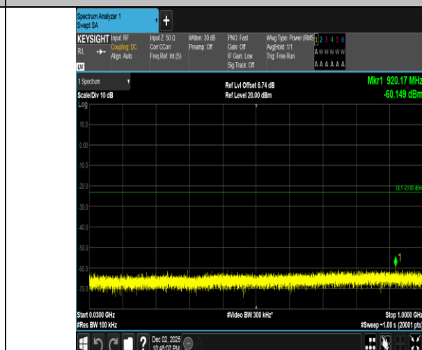
Band2-20MHz-16QAM-18900-1RB#0-30~1000-PASS
