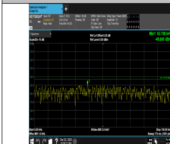
Band2-15MHz-QPSK-19125-75RB#0-0.009~0.15-PASS
