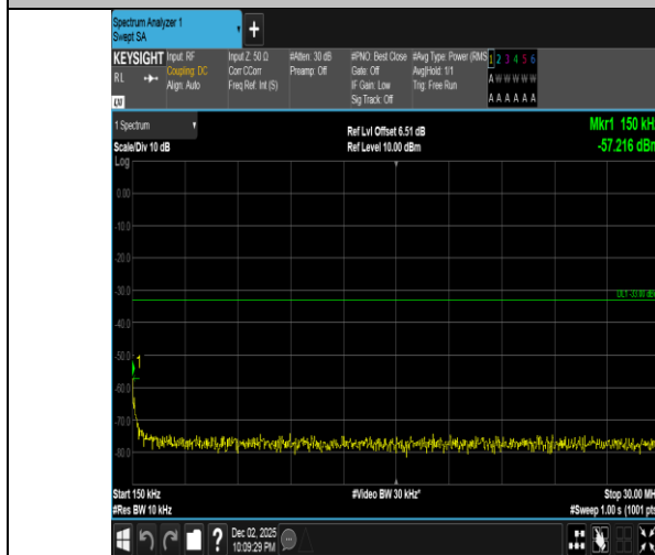
Band2-15MHz-16QAM-19125-75RB#0-0.15~30-PASS
