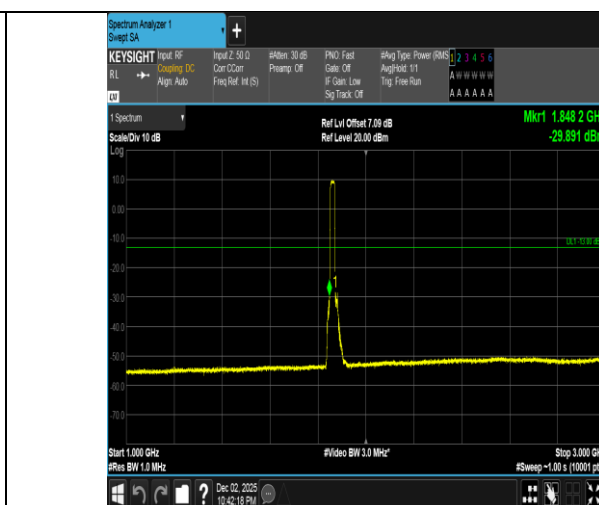
Band2-20MHz-QPSK-18700-100RB#0-1000~3000-PASS
