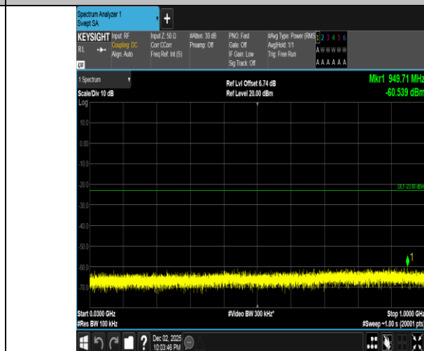
Band2-15MHz-16QAM-18900-75RB#0-30~1000-PASS
