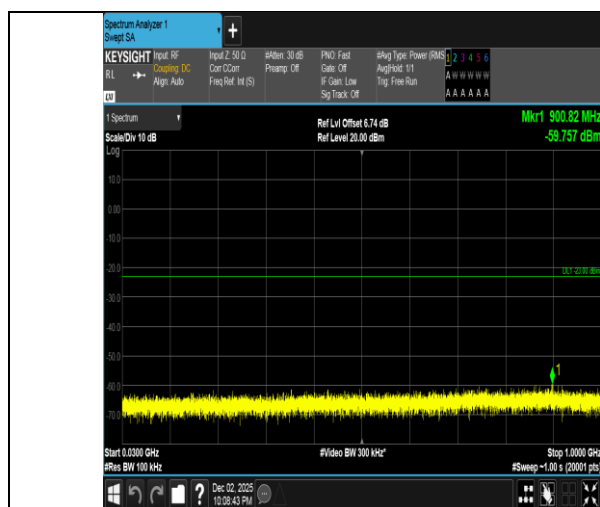
Band2-15MHz-QPSK-19125-75RB#0-30~1000-PASS
