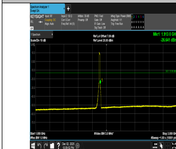
Band2-15MHz-16QAM-19125-75RB#0-1000~3000-PASS
