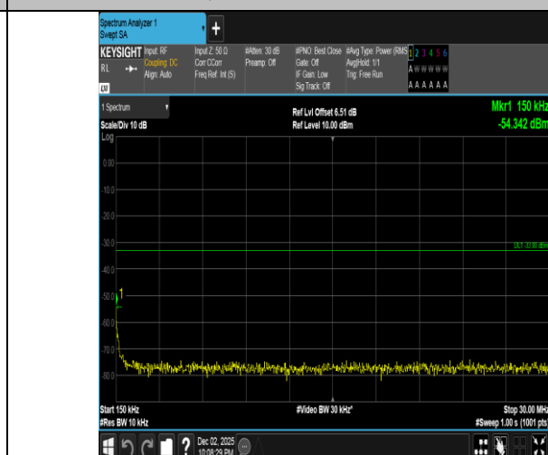
Band2-15MHz-QPSK-19125-75RB#0-0.15~30-PASS
