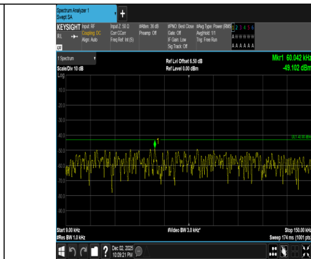
Band2-15MHz-16QAM-19125-75RB#0-0.009~0.15-PASS
