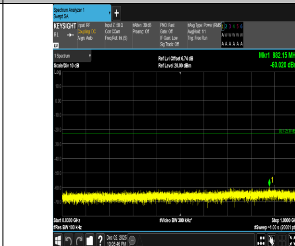
Band2-15MHz-16QAM-19125-1RB#0-30~1000-PASS
