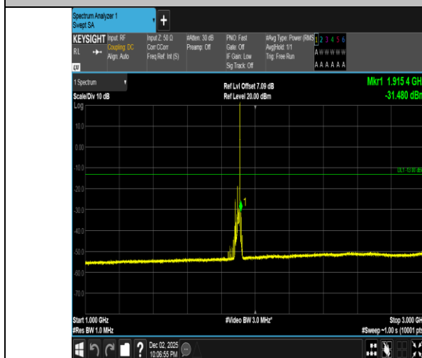
Band2-15MHz-QPSK-19125-1RB#74-1000~3000-PASS
