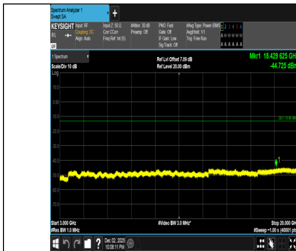
Band2-15MHz-16QAM-19125-1RB#74-3000~20000-PASS
