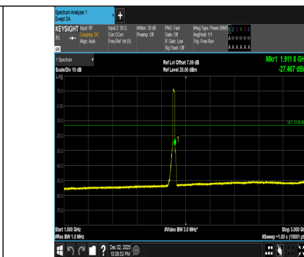
Band2-15MHz-QPSK-19125-75RB#0-1000~3000-PASS
