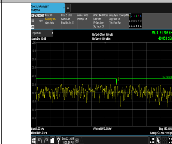
Band2-15MHz-16QAM-19125-1RB#0-0.009~0.15-PASS
