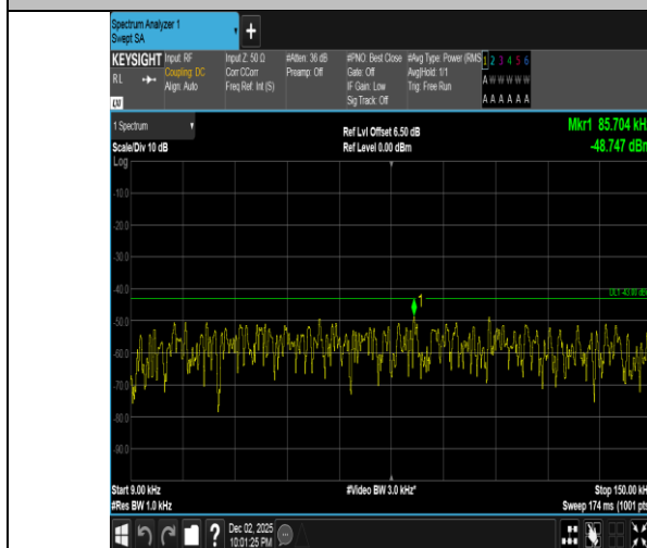
Band2-15MHz-16QAM-18900-1RB#74-0.009~0.15-PASS
