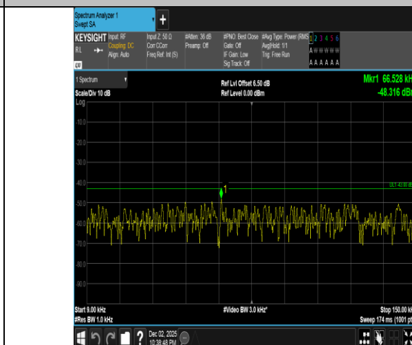
Band2-20MHz-16QAM-18700-1RB#0-0.009~0.15-PASS
