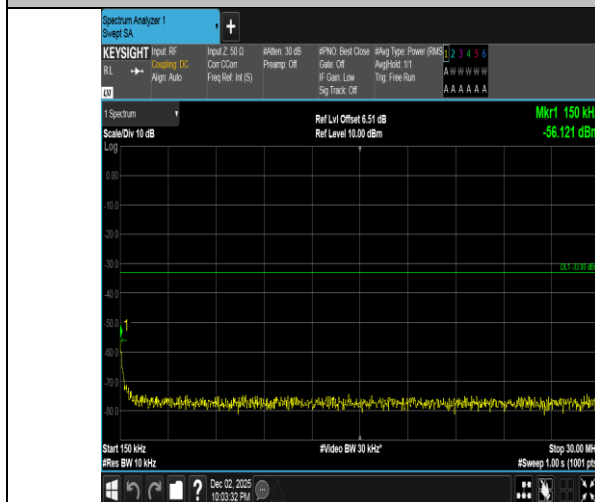
Band2-15MHz-16QAM-18900-75RB#0-0.15~30-PASS
