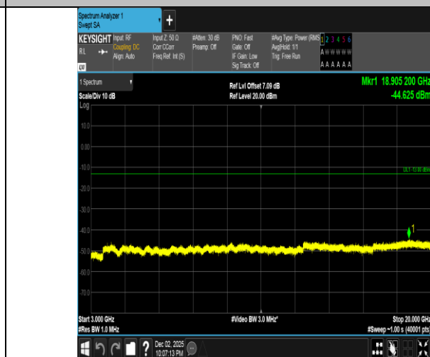
Band2-15MHz-QPSK-19125-1RB#74-3000~20000-PASS
