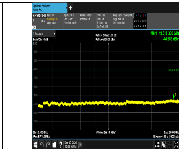
Band2-15MHz-16QAM-18900-1RB#0-3000~20000-PASS
