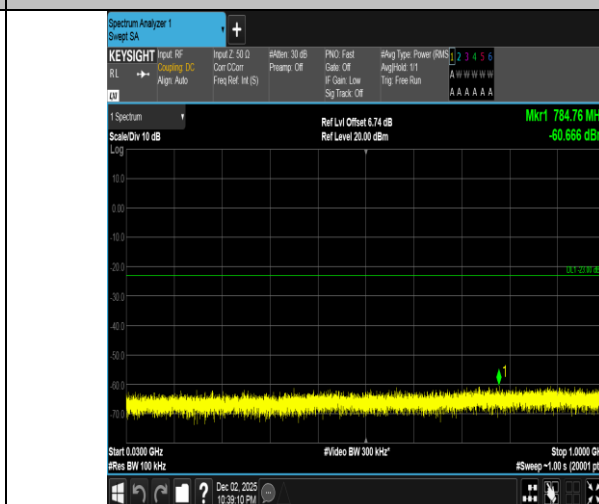
Band2-20MHz-16QAM-18700-1RB#0-30~1000-PASS
