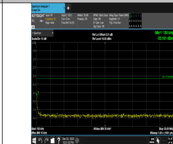
Band2-15MHz-16QAM-18900-1RB#74-0.15~30-PASS
