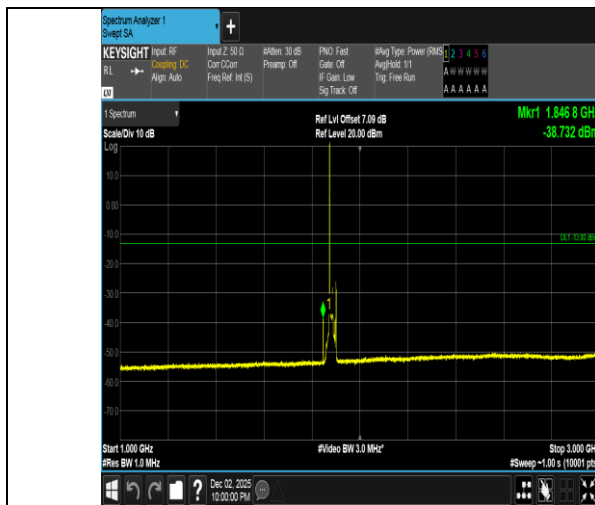
Band2-15MHz-16QAM-18900-1RB#0-1000~3000-PASS
