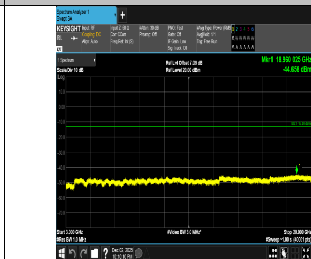
Band2-15MHz-16QAM-19125-75RB#0-3000~20000-PASS
