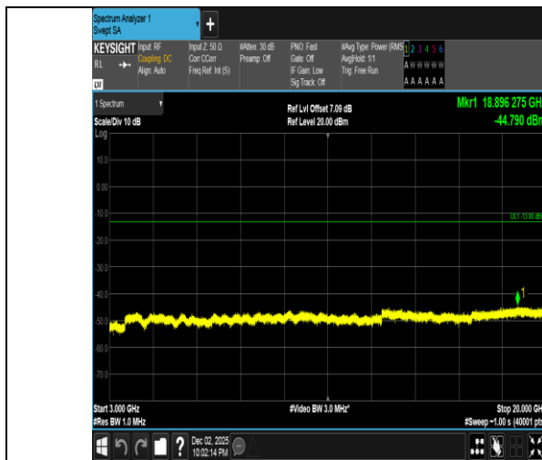
Band2-15MHz-16QAM-18900-1RB#74-3000~20000-PASS
