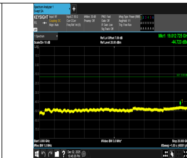
Band2-20MHz-16QAM-18900-1RB#0-3000~20000-PASS
