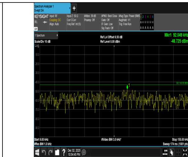
Band2-20MHz-16QAM-19100-100RB#0-0.009~0.15-PASS
