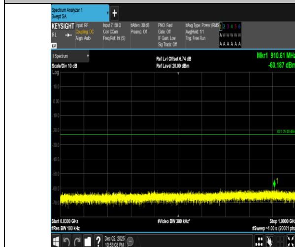
Band2-20MHz-16QAM-19100-1RB#99-30~1000-PASS
