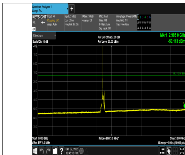
Band2-20MHz-16QAM-18900-1RB#0-1000~3000-PASS
