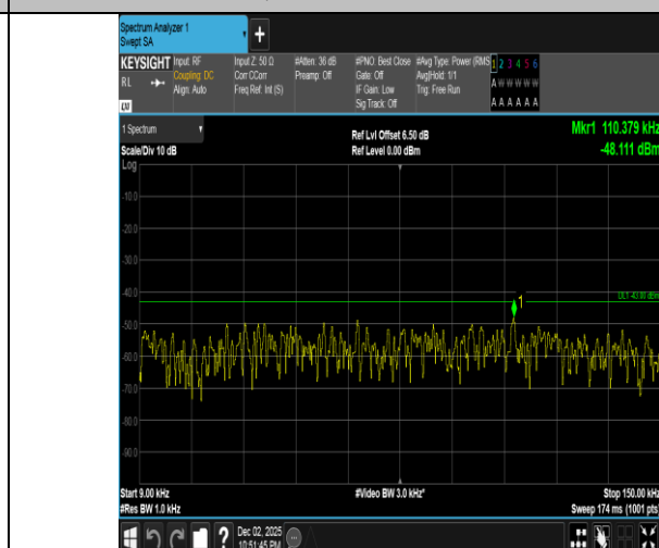
Band2-20MHz-QPSK-19100-1RB#99-0.009~0.15-PASS
