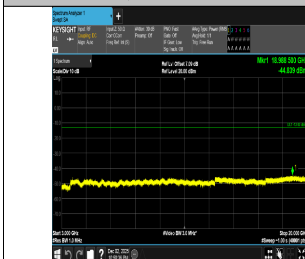
Band2-20MHz-QPSK-19100-1RB#0-3000~20000-PASS
