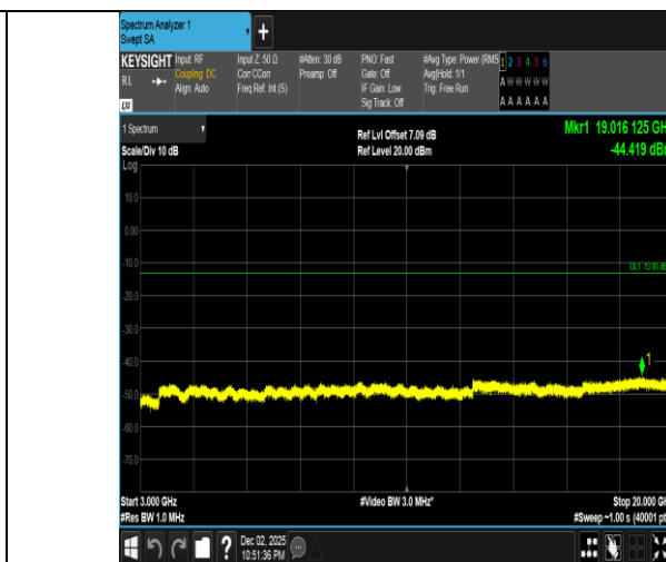
Band2-20MHz-16QAM-19100-1RB#0-3000~20000-PASS
