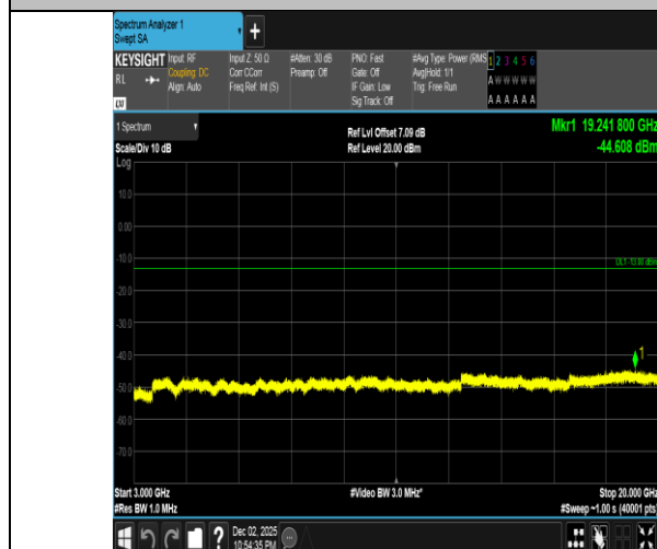
Band2-20MHz-QPSK-19100-100RB#0-3000~20000-PASS
