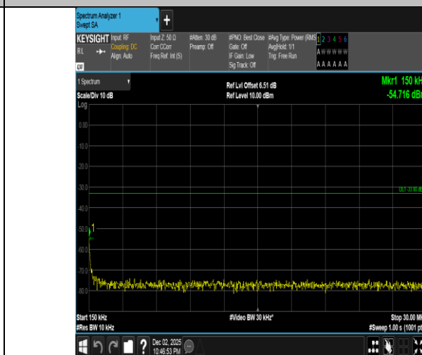
Band2-20MHz-16QAM-18900-1RB#99-0.15~30-PASS
