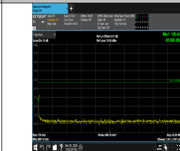
Band2-20MHz-16QAM-19100-1RB#99-0.15~30-PASS
