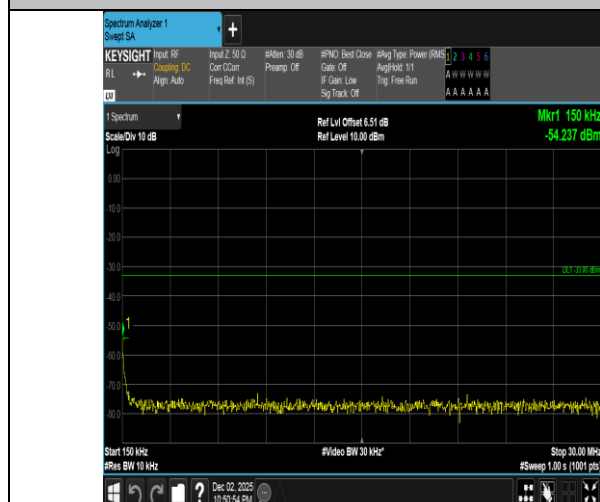
Band2-20MHz-16QAM-19100-1RB#0-0.15~30-PASS
