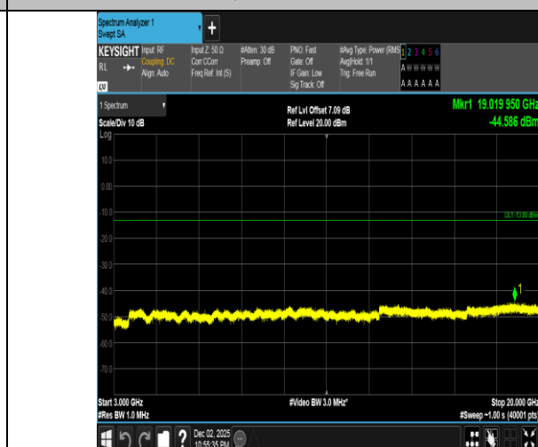
Band2-20MHz-16QAM-19100-100RB#0-3000~20000-PASS
