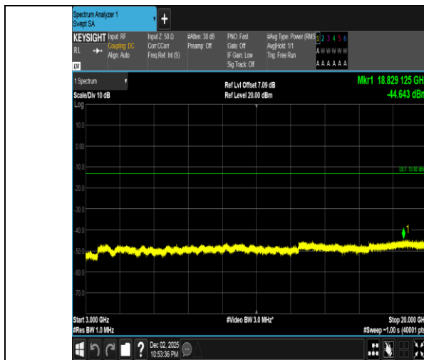
Band2-20MHz-16QAM-19100-1RB#99-3000~20000-PASS
