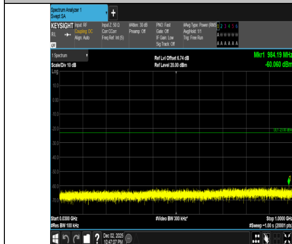
Band2-20MHz-16QAM-18900-1RB#99-30~1000-PASS
