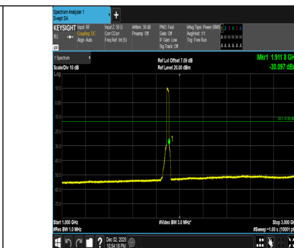
Band2-20MHz-QPSK-19100-100RB#0-1000~3000-PASS
