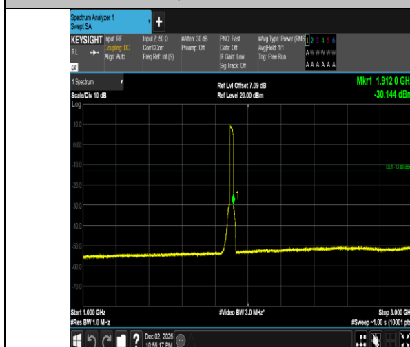
Band2-20MHz-16QAM-19100-100RB#0-1000~3000-PASS
