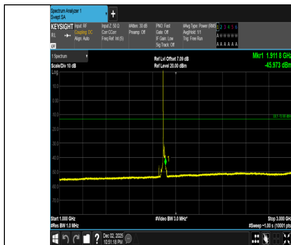
Band2-20MHz-16QAM-19100-1RB#0-1000~3000-PASS
