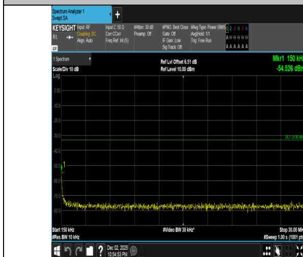
Band2-20MHz-16QAM-19100-100RB#0-0.15~30-PASS
