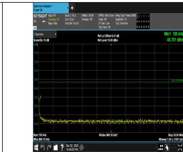
Band2-20MHz-QPSK-19100-1RB#0-0.15~30-PASS
