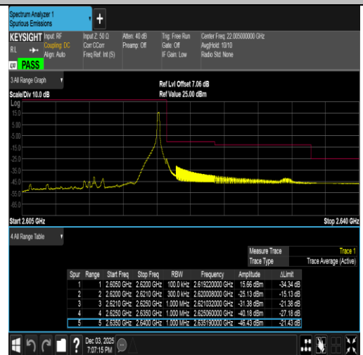
Band38-15MHz-QPSK-38175-1RB#74-PASS
