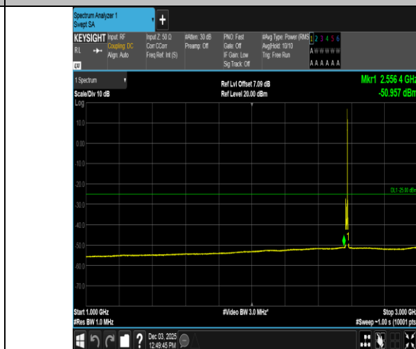
Band38-5MHz-QPSK-37775-1RB#24-1000~3000-PASS
