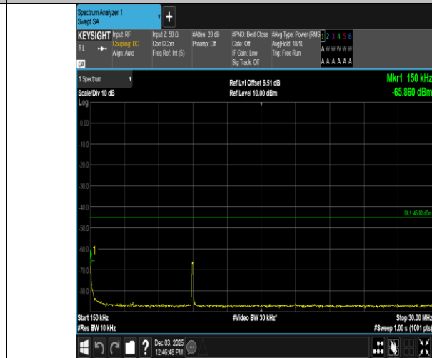
Band38-5MHz-16QAM-37775-1RB#0-0.15~30-PASS
