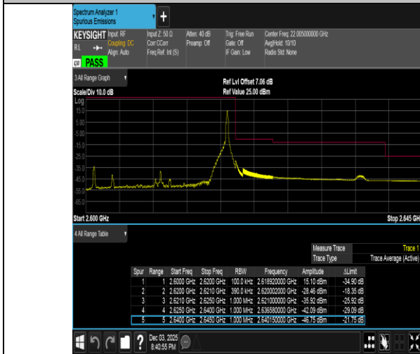
Band38-20MHz-16QAM-38150-1RB#99-PASS
