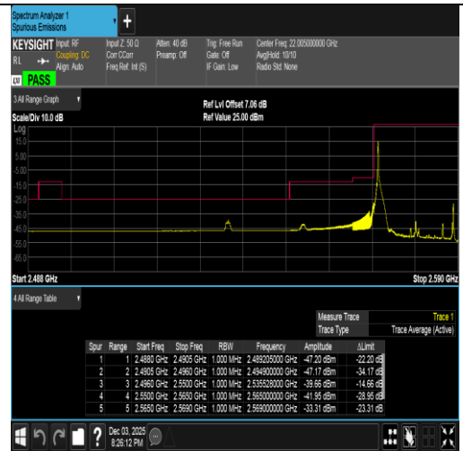
Band38-20MHz-16QAM-37850-1RB#0-PASS
