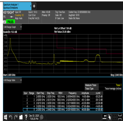
Band38-15MHz-16QAM-38175-1RB#0-PASS
