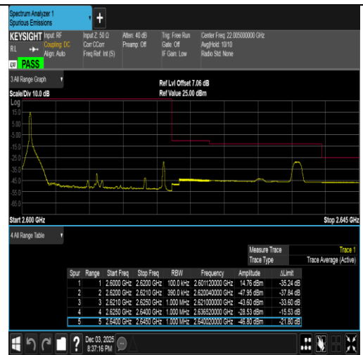
Band38-20MHz-16QAM-38150-1RB#0-PASS
