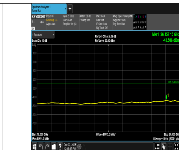
Band38-5MHz-QPSK-37775-1RB#0-18000~27000-PASS
