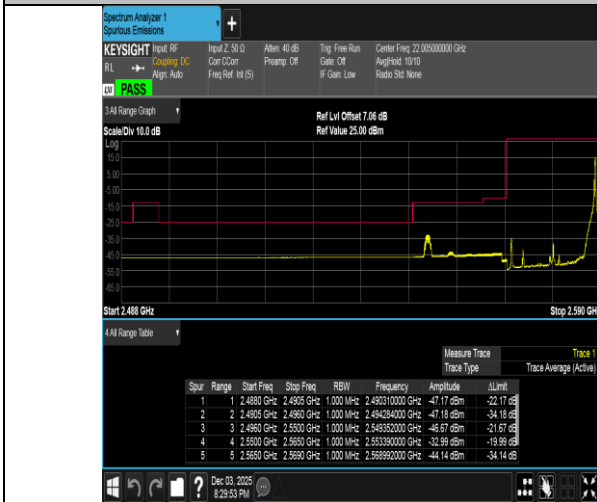
Band38-20MHz-16QAM-37850-1RB#99-PASS
