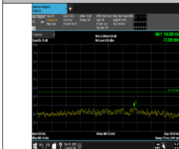
Band38-5MHz-QPSK-37775-1RB#24-0.009~0.15-PASS
