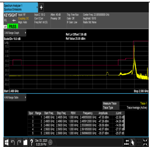
Band38-10MHz-16QAM-37800-1RB#0-PASS
