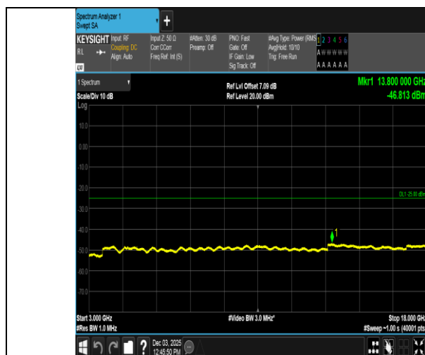
Band38-5MHz-QPSK-37775-1RB#0-3000~18000-PASS
