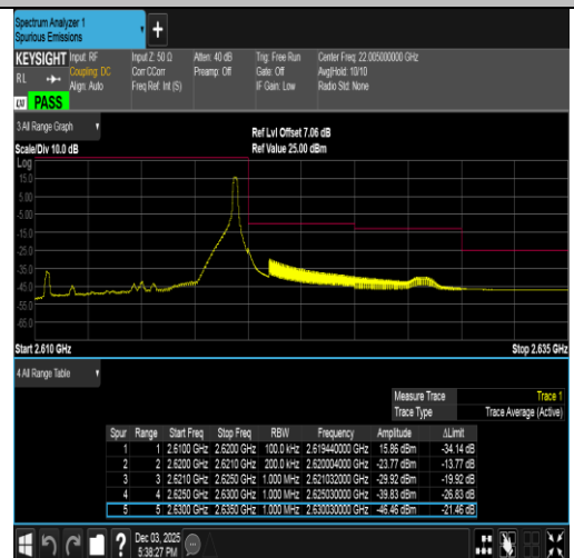
Band38-10MHz-QPSK-38200-1RB#49-PASS
