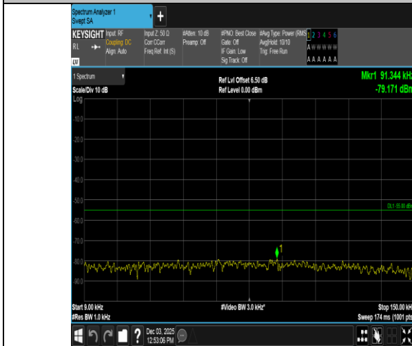
Band38-5MHz-QPSK-37775-25RB#0-0.009~0.15-PASS
