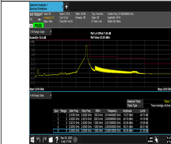
Band38-10MHz-16QAM-38200-1RB#49-PASS
