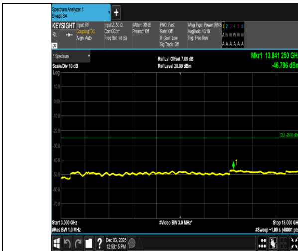
Band38-5MHz-QPSK-37775-1RB#24-3000~18000-PASS
