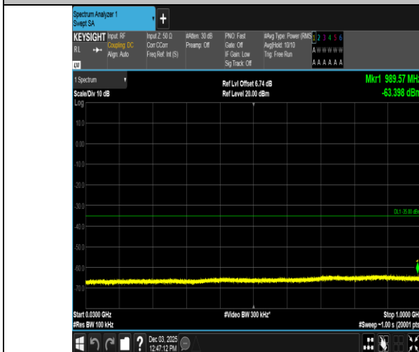
Band38-5MHz-16QAM-37775-1RB#0-30~1000-PASS
