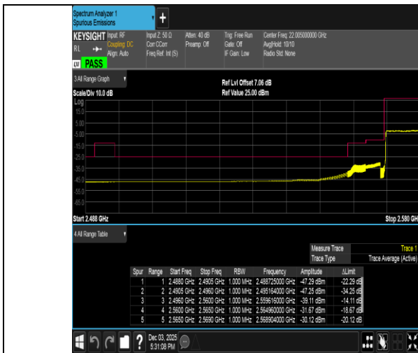
Band38-10MHz-QPSK-37800-50RB#0-PASS
