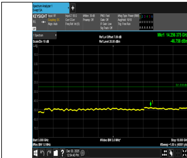
Band38-5MHz-QPSK-37775-25RB#0-3000~18000-PASS
