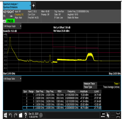
Band38-10MHz-16QAM-38200-1RB#0-PASS
