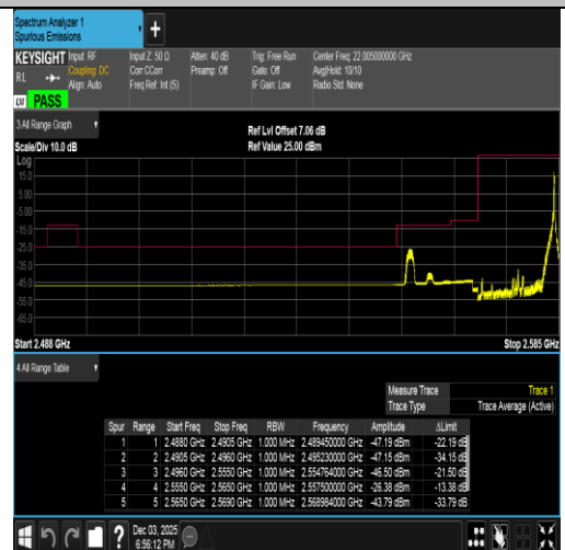
Band38-15MHz-QPSK-37825-1RB#74-PASS
