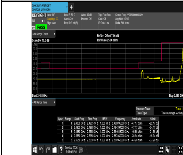
Band38-15MHz-16QAM-37825-1RB#74-PASS
