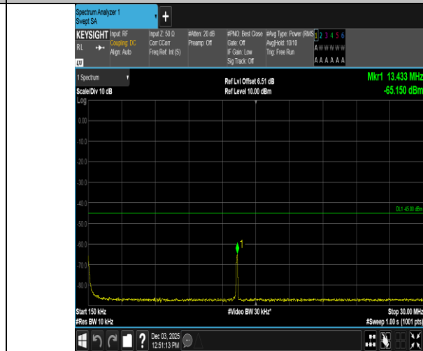
Band38-5MHz-16QAM-37775-1RB#24-0.15~30-PASS
