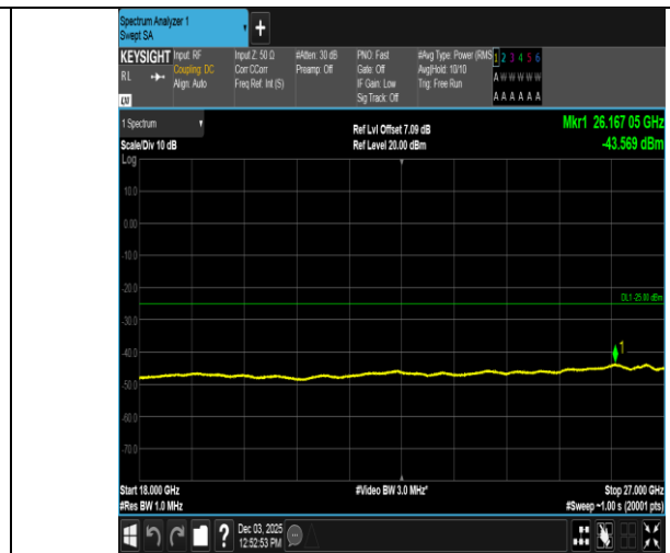
Band38-5MHz-16QAM-37775-1RB#24-18000~27000-PASS
