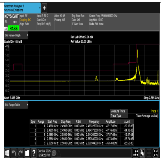
Band38-15MHz-16QAM-37825-1RB#0-PASS
