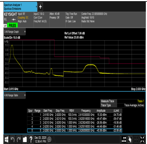
Band38-5MHz-16QAM-38225-1RB#0-PASS
