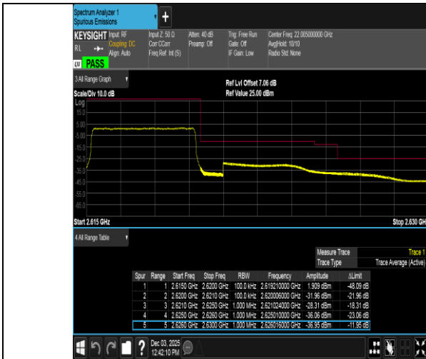
Band38-5MHz-QPSK-38225-25RB#0-PASS
