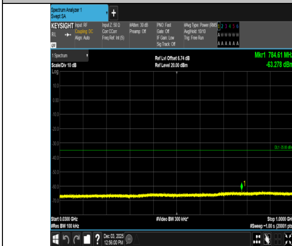
Band38-5MHz-16QAM-37775-25RB#0-30~1000-PASS
