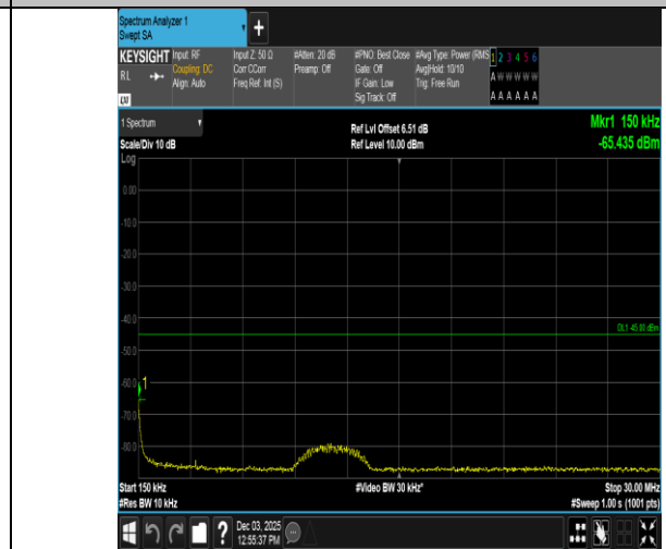
Band38-5MHz-16QAM-37775-25RB#0-0.15~30-PASS
