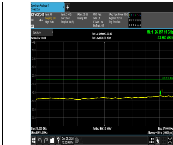
Band38-5MHz-QPSK-37775-25RB#0-18000~27000-PASS
