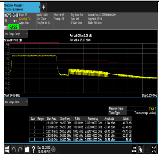
Band38-5MHz-16QAM-38225-25RB#0-PASS
