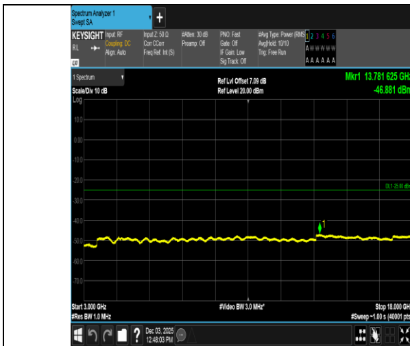
Band38-5MHz-16QAM-37775-1RB#0-3000~18000-PASS
