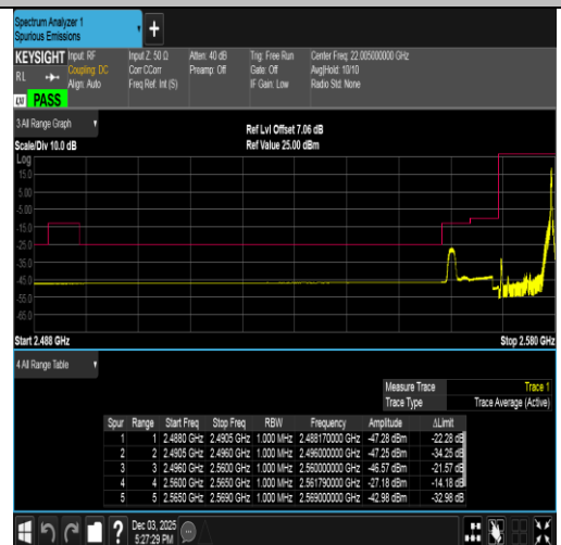
Band38-10MHz-QPSK-37800-1RB#49-PASS
