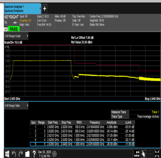
Band38-15MHz-16QAM-38175-75RB#0-PASS
