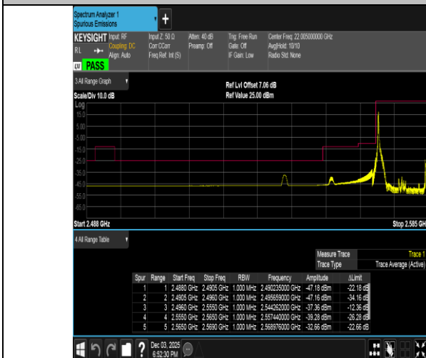
Band38-15MHz-QPSK-37825-1RB#0-PASS
