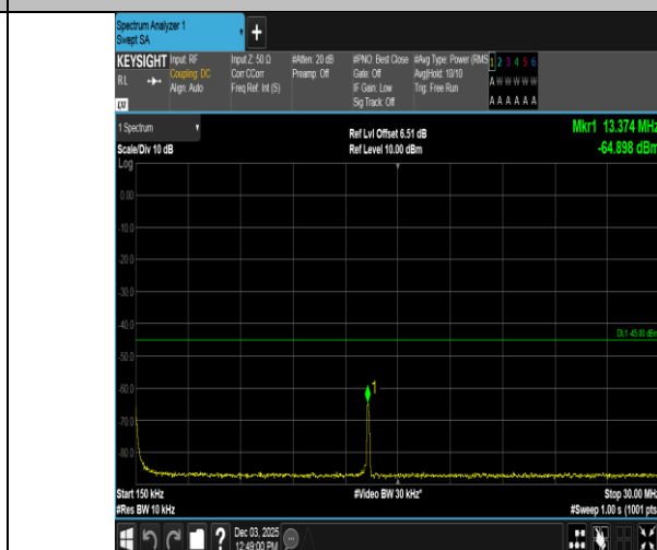
Band38-5MHz-QPSK-37775-1RB#24-0.15~30-PASS
