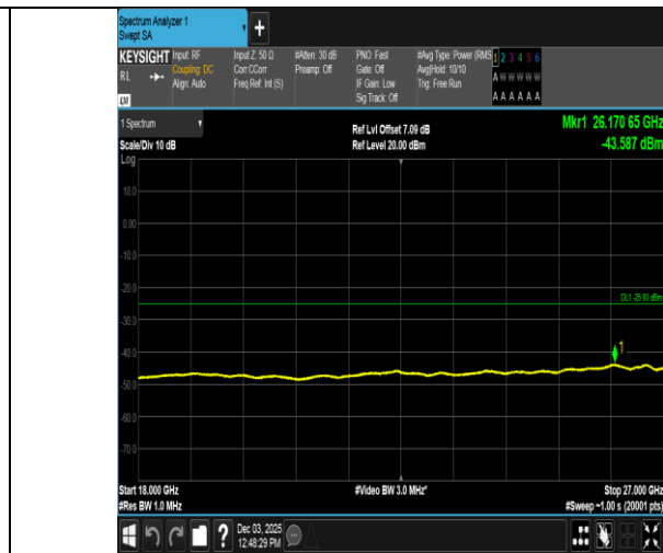
Band38-5MHz-16QAM-37775-1RB#0-18000~27000-PASS
