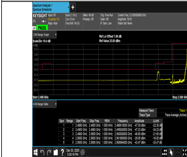
Band38-10MHz-16QAM-37800-1RB#49-PASS
