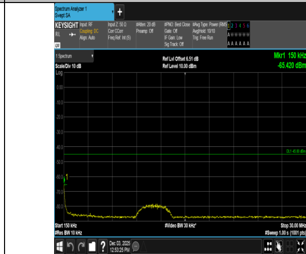
Band38-5MHz-QPSK-37775-25RB#0-0.15~30-PASS
