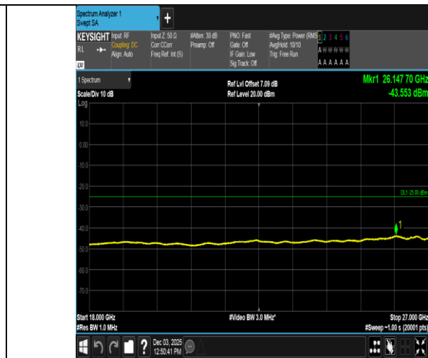
Band38-5MHz-QPSK-37775-1RB#24-18000~27000-PASS
