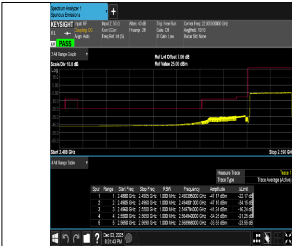
Band38-20MHz-QPSK-37850-100RB#0-PASS
