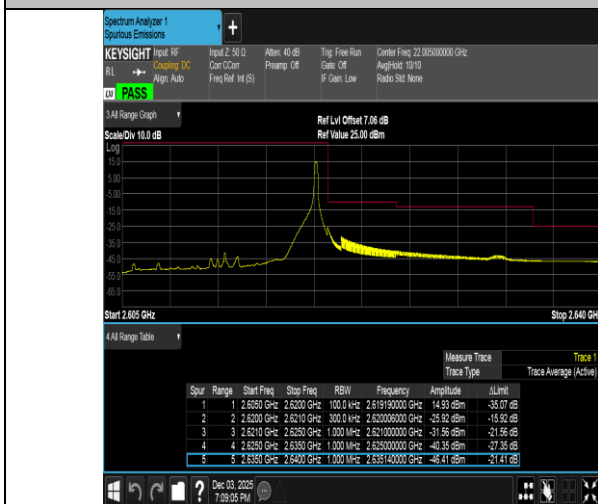
Band38-15MHz-16QAM-38175-1RB#74-PASS
