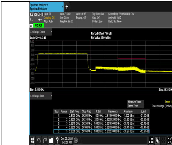
Band38-10MHz-QPSK-38200-50RB#0-PASS
