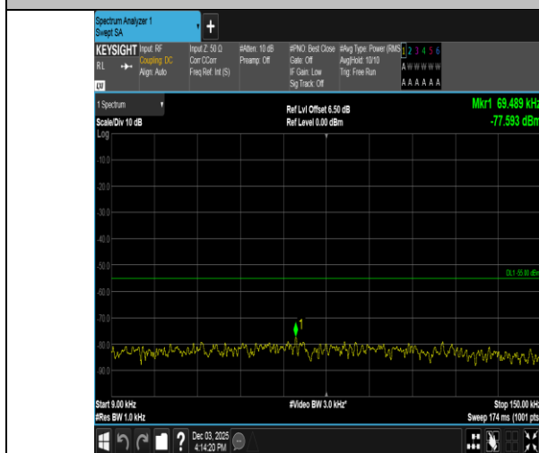
Band38-5MHz-16QAM-38000-25RB#0-0.009~0.15-PASS
