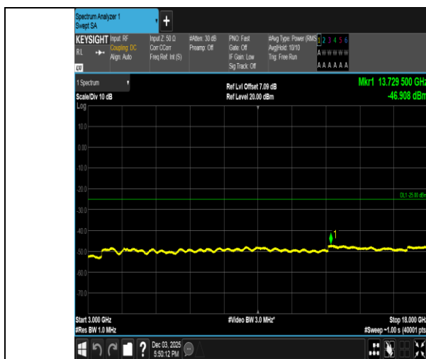
Band38-10MHz-QPSK-37800-1RB#49-3000~18000-PASS
