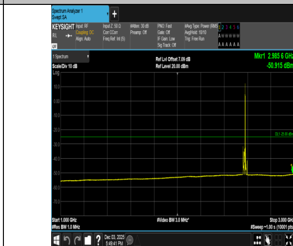
Band38-10MHz-QPSK-37800-1RB#49-1000~3000-PASS
