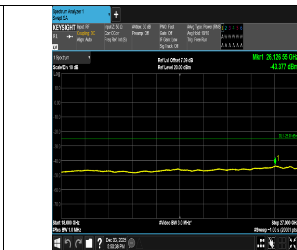
Band38-10MHz-QPSK-37800-1RB#49-18000~27000-PASS
