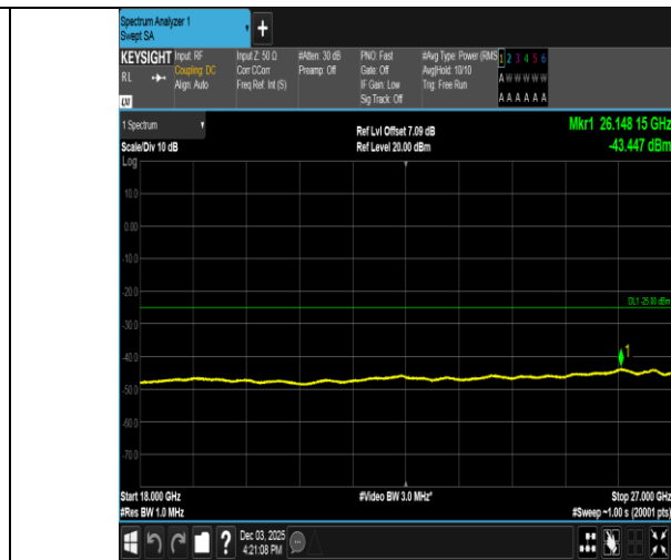
Band38-5MHz-16QAM-38225-1RB#0-18000~27000-PASS
