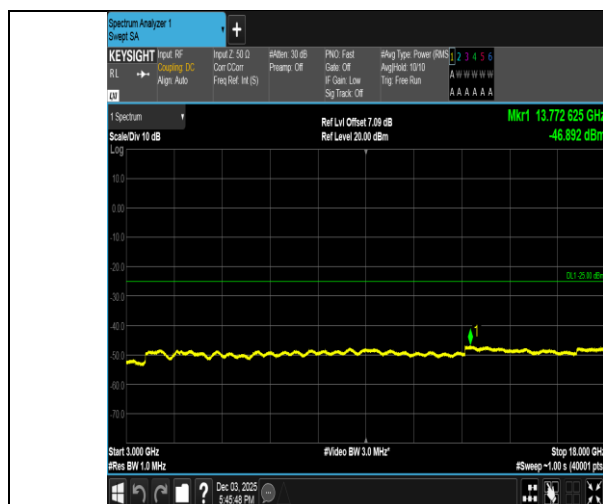
Band38-10MHz-QPSK-37800-1RB#0-3000~18000-PASS
