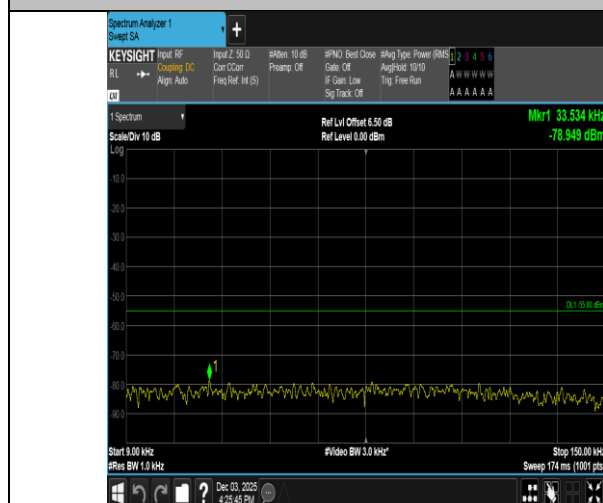
Band38-5MHz-QPSK-38225-25RB#0-0.009~0.15-PASS
