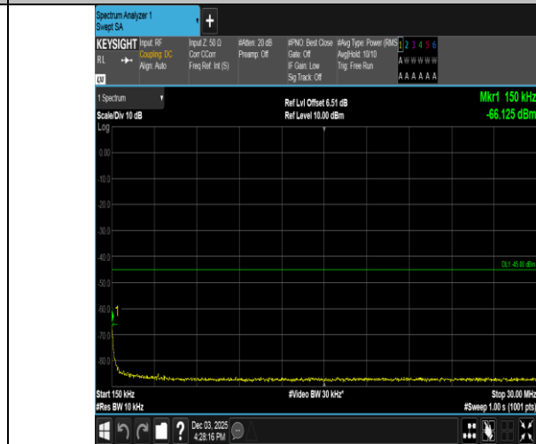
Band38-5MHz-16QAM-38225-25RB#0-0.15~30-PASS
