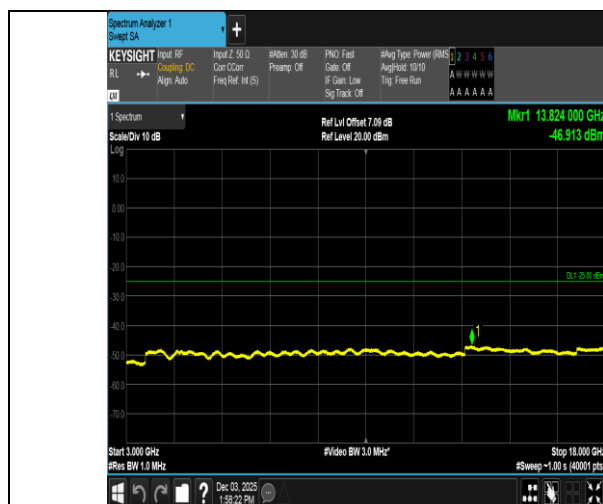
Band38-5MHz-QPSK-38000-1RB#24-3000~18000-PASS
