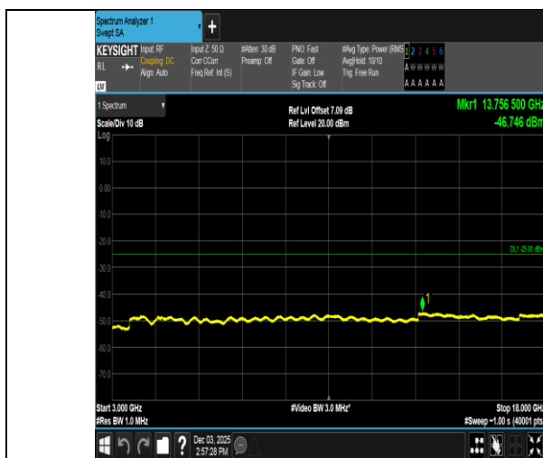
Band38-5MHz-16QAM-38000-1RB#24-3000~18000-PASS
