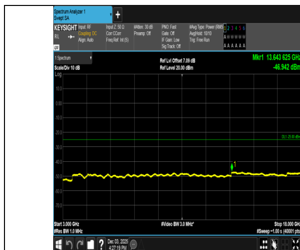
Band38-5MHz-QPSK-38225-25RB#0-3000~18000-PASS
