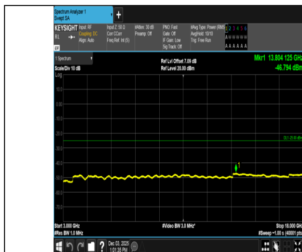
Band38-5MHz-16QAM-38000-1RB#0-3000~18000-PASS
