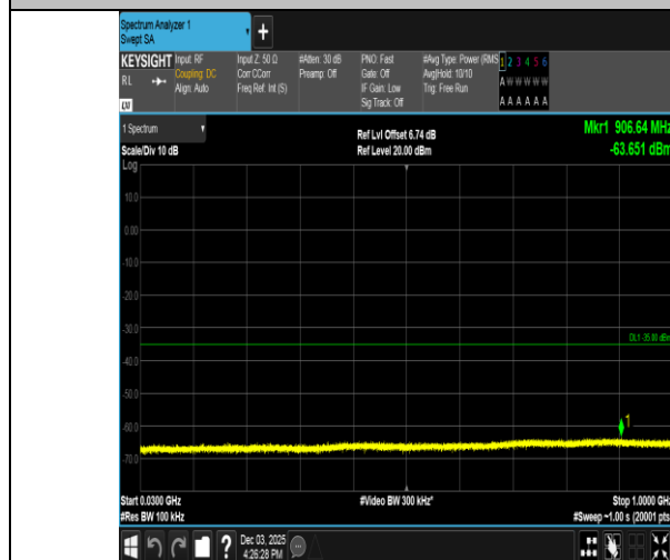
Band38-5MHz-QPSK-38225-25RB#0-30~1000-PASS
