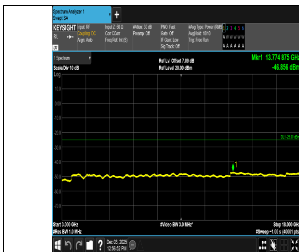
Band38-5MHz-16QAM-37775-25RB#0-3000~18000-PASS
