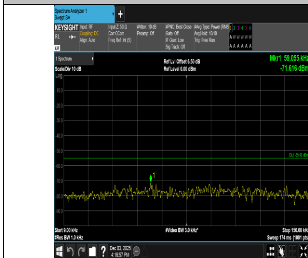
Band38-5MHz-QPSK-38225-1RB#0-0.009~0.15-PASS
