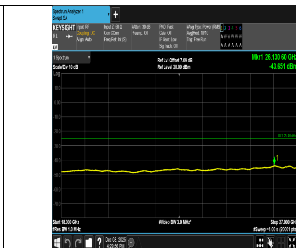
Band38-5MHz-16QAM-38225-25RB#0-18000~27000-PASS
