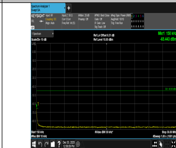
Band38-5MHz-QPSK-38000-1RB#0-0.15~30-PASS
