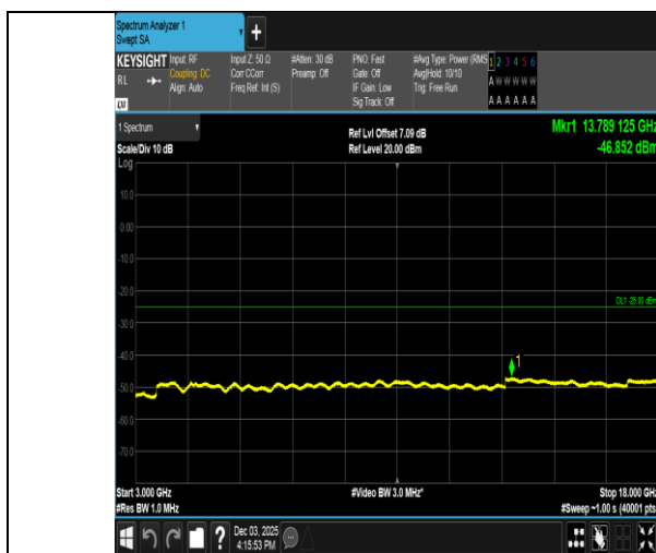
Band38-5MHz-16QAM-38000-25RB#0-3000~18000-PASS
