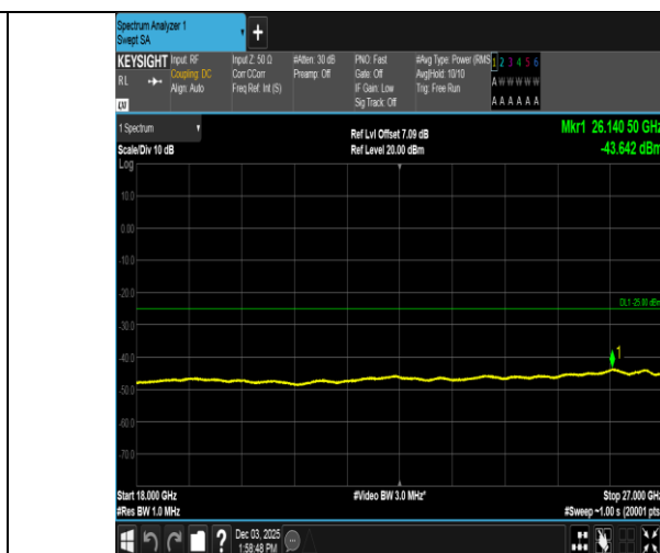
Band38-5MHz-QPSK-38000-1RB#24-18000~27000-PASS
