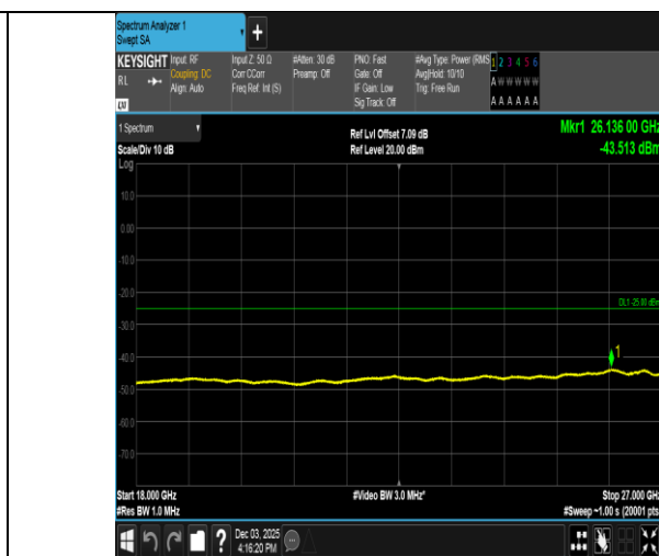
Band38-5MHz-16QAM-38000-25RB#0-18000~27000-PASS
