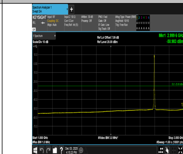
Band38-5MHz-16QAM-38000-25RB#0-1000~3000-PASS
