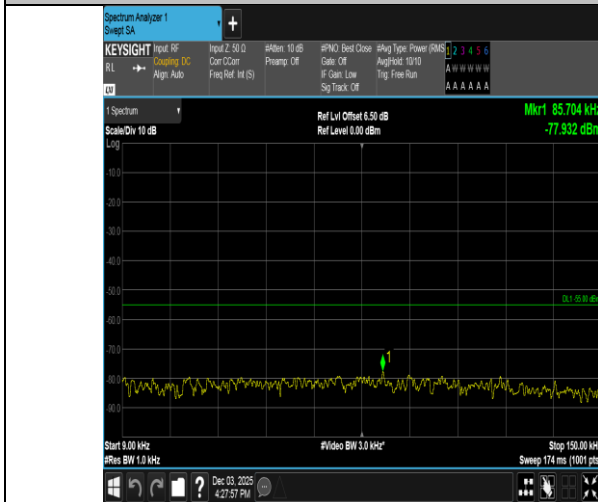
Band38-5MHz-16QAM-38225-25RB#0-0.009~0.15-PASS
