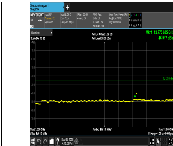
Band38-5MHz-QPSK-38225-1RB#0-3000~18000-PASS
