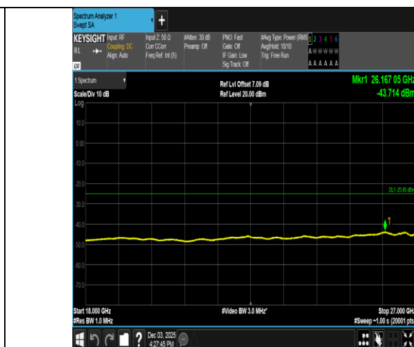
Band38-5MHz-QPSK-38225-25RB#0-18000~27000-PASS
