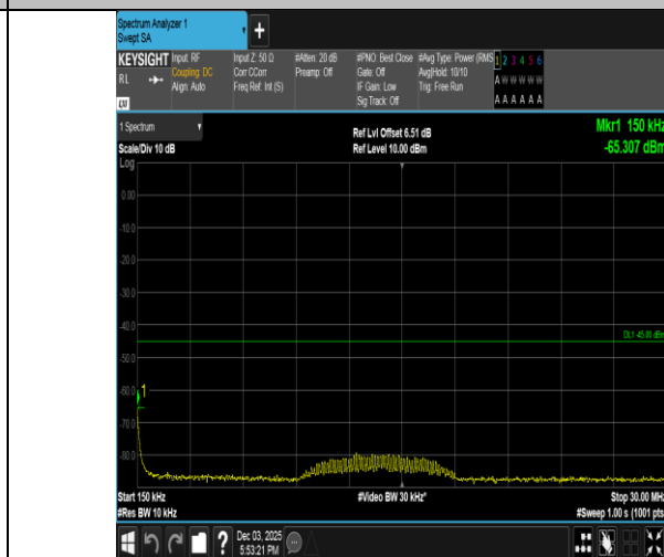
Band38-10MHz-QPSK-37800-50RB#0-0.15~30-PASS
