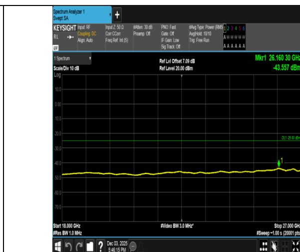
Band38-10MHz-QPSK-37800-1RB#0-18000~27000-PASS
