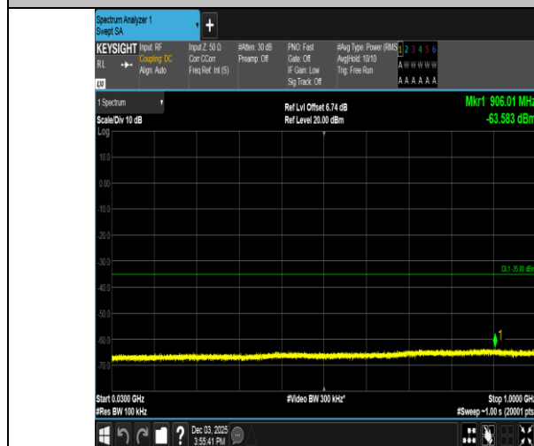
Band38-5MHz-QPSK-38000-25RB#0-30~1000-PASS
