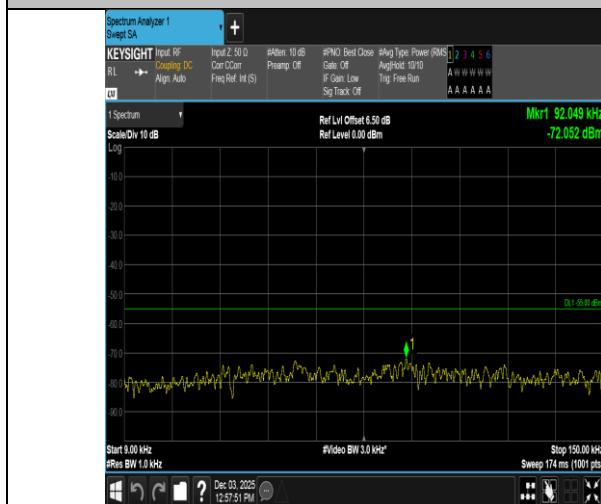
Band38-5MHz-QPSK-38000-1RB#0-0.009~0.15-PASS
