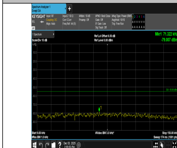
Band38-5MHz-16QAM-38000-1RB#24-0.009~0.15-PASS
