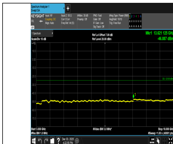
Band38-5MHz-QPSK-38225-1RB#24-3000~18000-PASS
