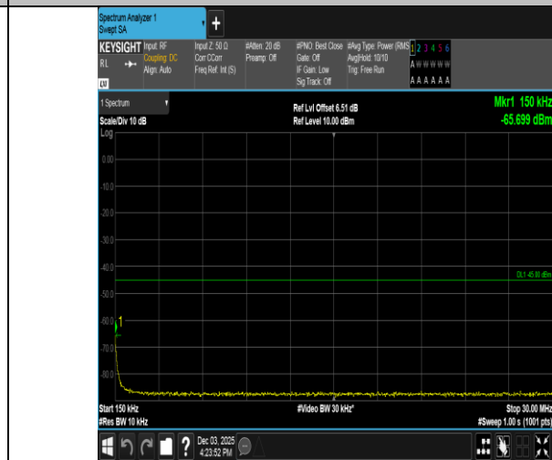
Band38-5MHz-16QAM-38225-1RB#24-0.15~30-PASS
