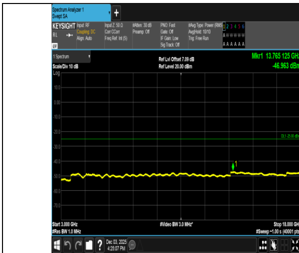
Band38-5MHz-16QAM-38225-1RB#24-3000~18000-PASS
