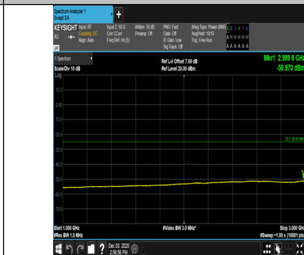
Band38-5MHz-16QAM-38000-1RB#24-1000~3000-PASS
