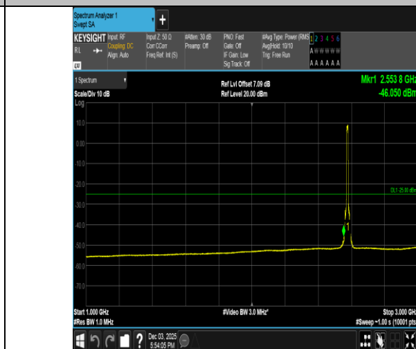
Band38-10MHz-QPSK-37800-50RB#0-1000~3000-PASS
