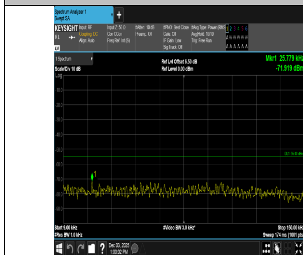
Band38-5MHz-16QAM-38000-1RB#0-0.009~0.15-PASS
