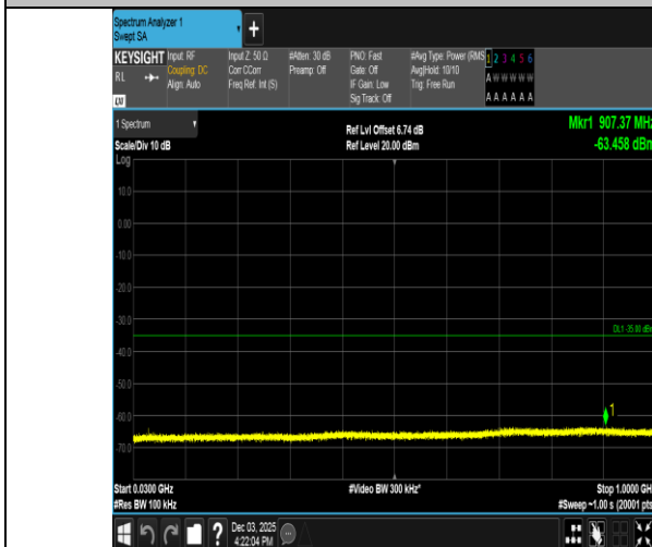
Band38-5MHz-QPSK-38225-1RB#24-30~1000-PASS
