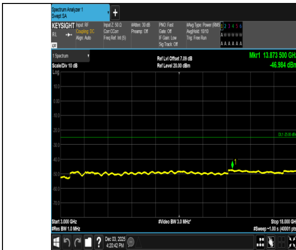
Band38-5MHz-16QAM-38225-1RB#0-3000~18000-PASS
