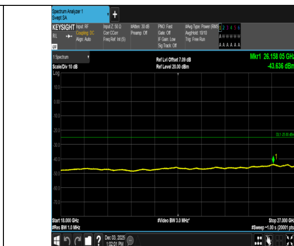
Band38-5MHz-16QAM-38000-1RB#0-18000~27000-PASS
