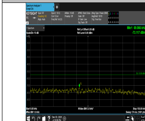
Band38-5MHz-16QAM-38225-1RB#0-0.009~0.15-PASS
