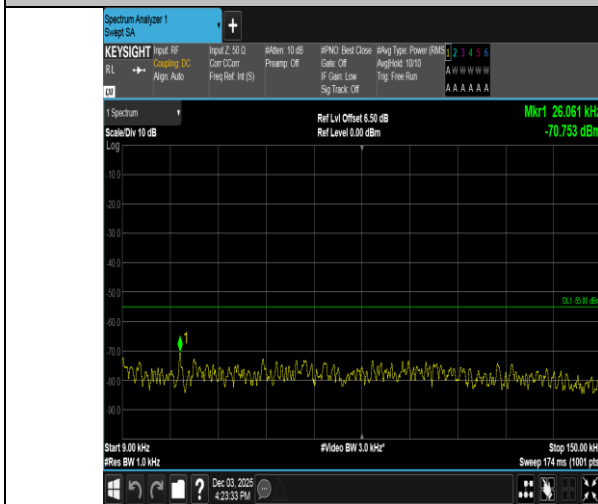
Band38-5MHz-16QAM-38225-1RB#24-0.009~0.15-PASS
