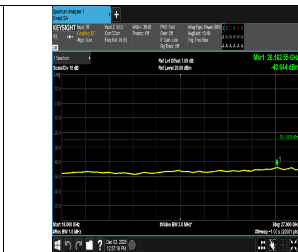
Band38-5MHz-16QAM-37775-25RB#0-18000~27000-PASS
