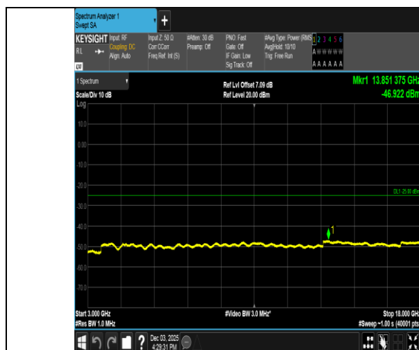
Band38-5MHz-16QAM-38225-25RB#0-3000~18000-PASS
