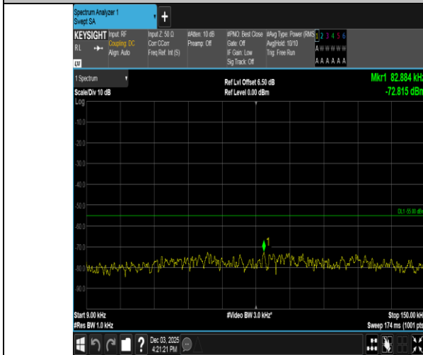
Band38-5MHz-QPSK-38225-1RB#24-0.009~0.15-PASS
