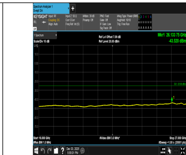
Band38-10MHz-QPSK-37800-50RB#0-18000~27000-PASS
