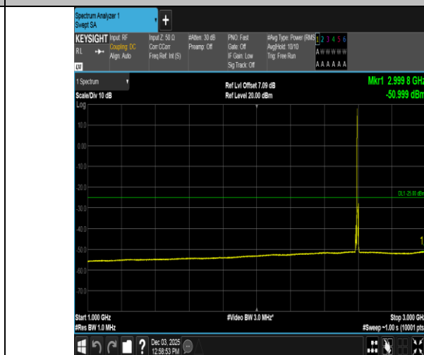
Band38-5MHz-QPSK-38000-1RB#0-1000~3000-PASS
