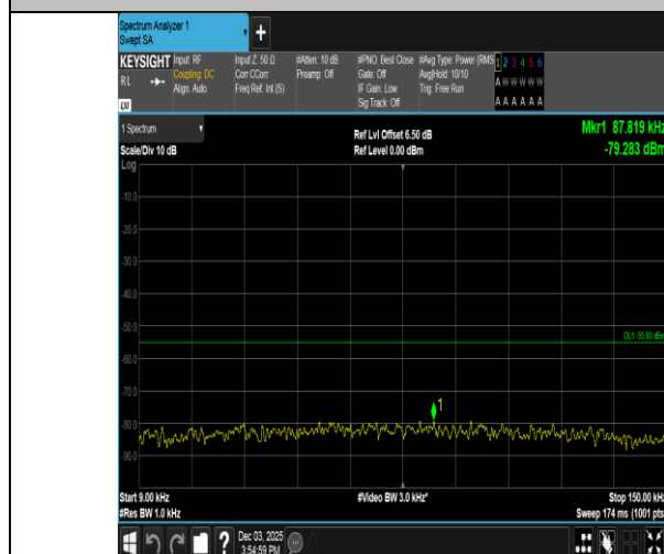
Band38-5MHz-QPSK-38000-25RB#0-0.009~0.15-PASS
