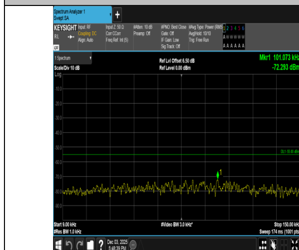
Band38-10MHz-QPSK-37800-1RB#49-0.009~0.15-PASS
