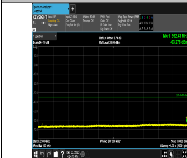
Band38-5MHz-16QAM-38225-1RB#24-30~1000-PASS
