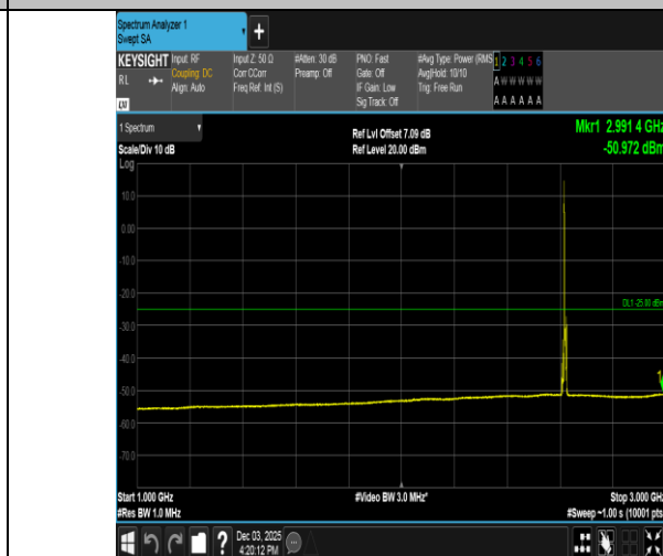
Band38-5MHz-16QAM-38225-1RB#0-1000~3000-PASS
