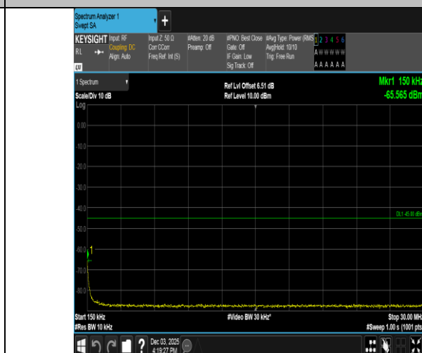
Band38-5MHz-16QAM-38225-1RB#0-0.15~30-PASS
