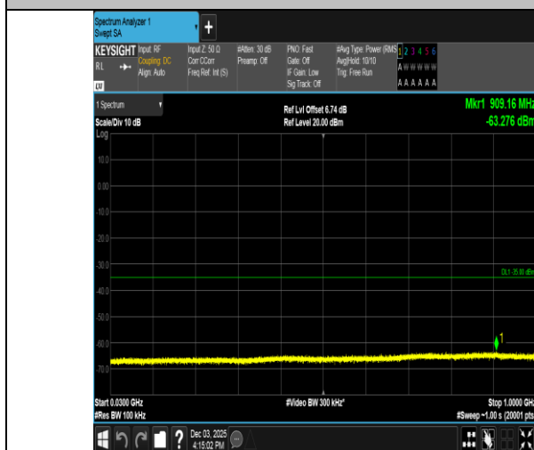
Band38-5MHz-16QAM-38000-25RB#0-30~1000-PASS
