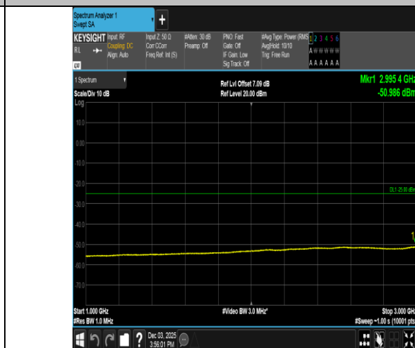
Band38-5MHz-QPSK-38000-25RB#0-1000~3000-PASS
