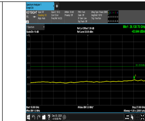
Band38-5MHz-QPSK-38225-1RB#0-18000~27000-PASS
