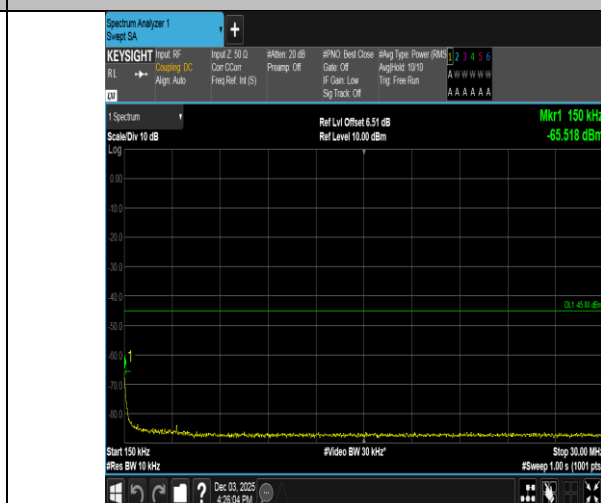
Band38-5MHz-QPSK-38225-25RB#0-0.15~30-PASS
