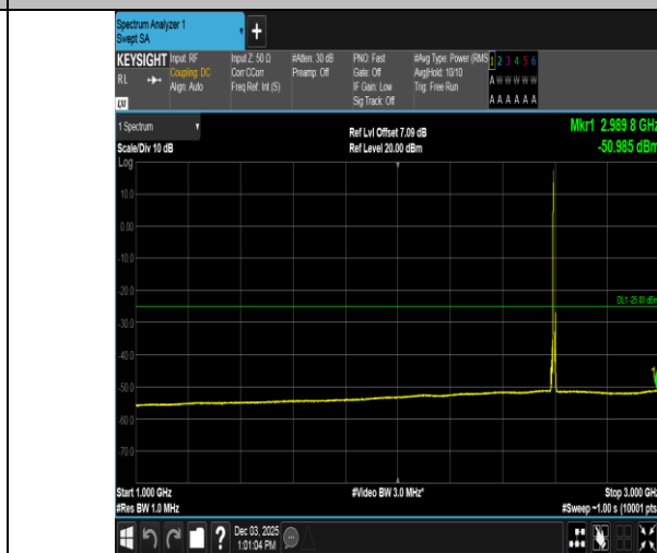
Band38-5MHz-16QAM-38000-1RB#0-1000~3000-PASS
