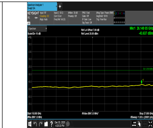
Band38-5MHz-16QAM-38225-1RB#24-18000~27000-PASS
