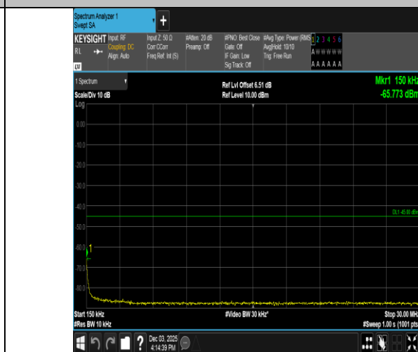
Band38-5MHz-16QAM-38000-25RB#0-0.15~30-PASS
