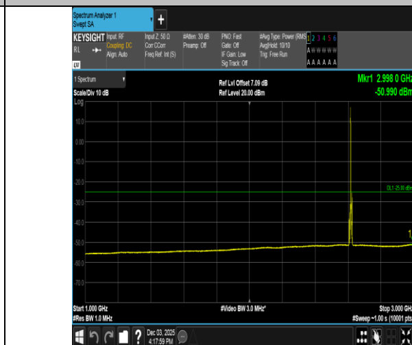
Band38-5MHz-QPSK-38225-1RB#0-1000~3000-PASS
