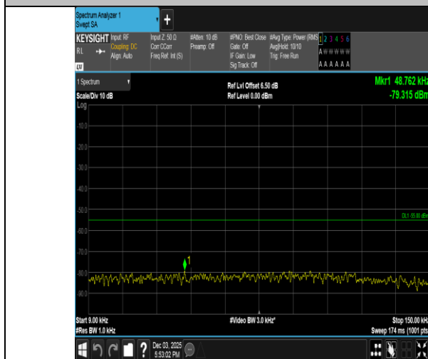
Band38-10MHz-QPSK-37800-50RB#0-0.009~0.15-PASS
