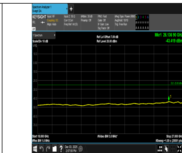
Band38-5MHz-16QAM-38000-1RB#24-18000~27000-PASS
