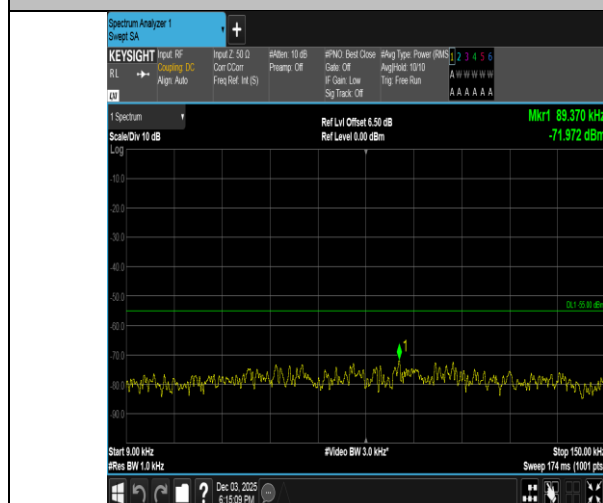
Band38-10MHz-QPSK-38200-1RB#49-0.009~0.15-PASS
