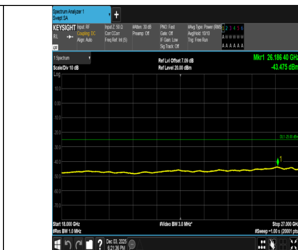
Band38-10MHz-QPSK-38200-50RB#0-18000~27000-PASS
