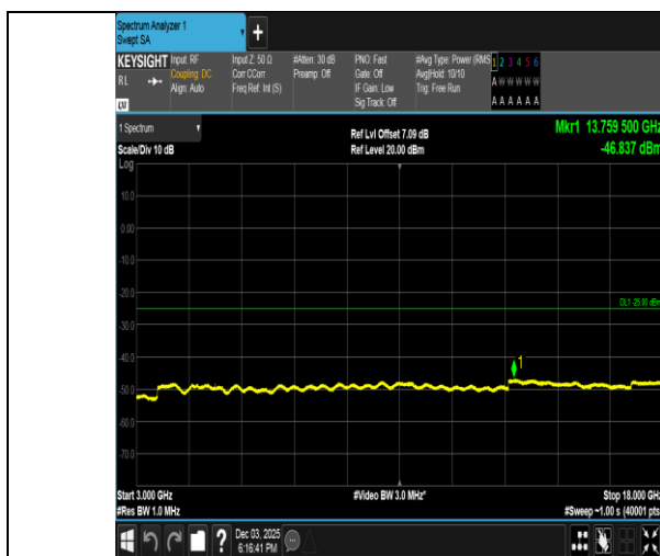
Band38-10MHz-QPSK-38200-1RB#49-3000~18000-PASS
