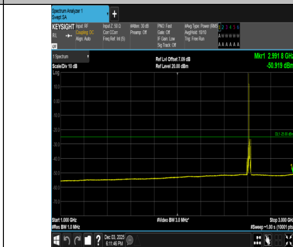
Band38-10MHz-QPSK-38200-1RB#0-1000~3000-PASS
