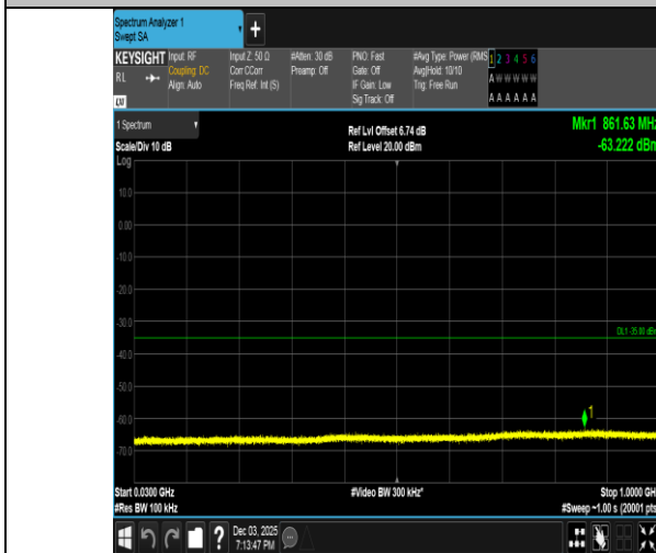
Band38-15MHz-QPSK-37825-1RB#0-30~1000-PASS
