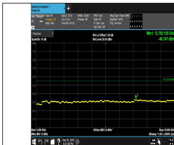
Band38-10MHz-QPSK-38200-50RB#0-3000~18000-PASS
