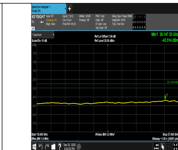
Band38-10MHz-QPSK-38000-1RB#49-18000~27000-PASS
