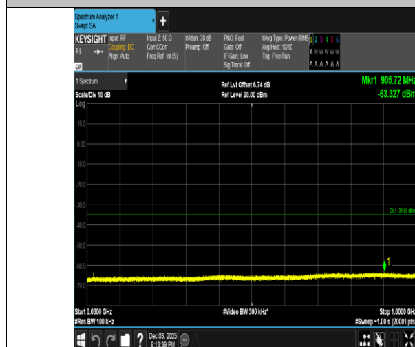
Band38-10MHz-16QAM-38200-1RB#0-30~1000-PASS
