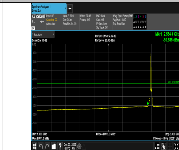
Band38-10MHz-QPSK-38000-50RB#0-1000~3000-PASS
