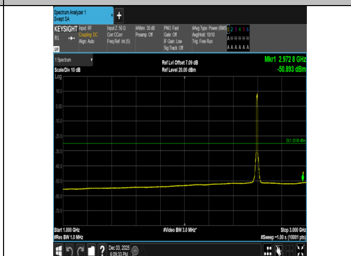
Band38-10MHz-16QAM-38000-50RB#0-1000~3000-PASS
