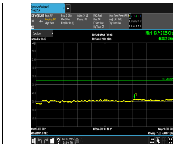
Band38-10MHz-QPSK-38200-1RB#0-3000~18000-PASS
