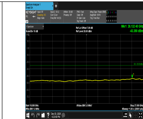
Band38-10MHz-16QAM-38200-50RB#0-18000~27000-PASS
