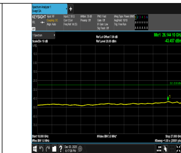
Band38-10MHz-QPSK-38200-1RB#49-18000~27000-PASS
