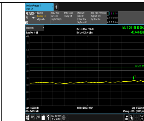
Band38-10MHz-16QAM-38200-1RB#0-18000~27000-PASS
