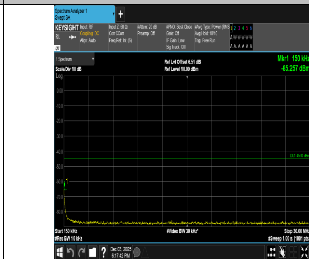
Band38-10MHz-16QAM-38200-1RB#49-0.15~30-PASS
