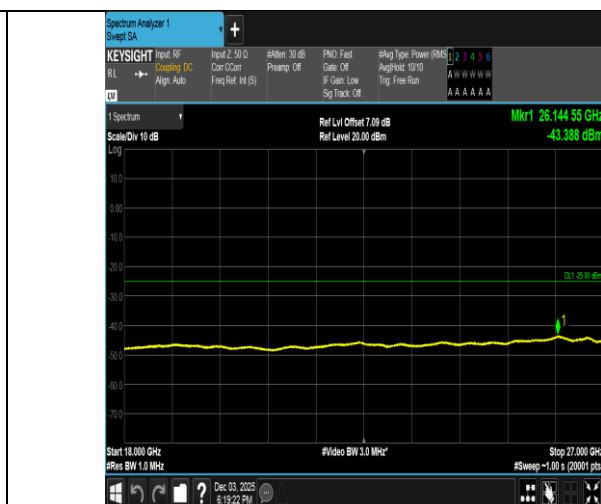
Band38-10MHz-16QAM-38200-1RB#49-18000~27000-PASS
