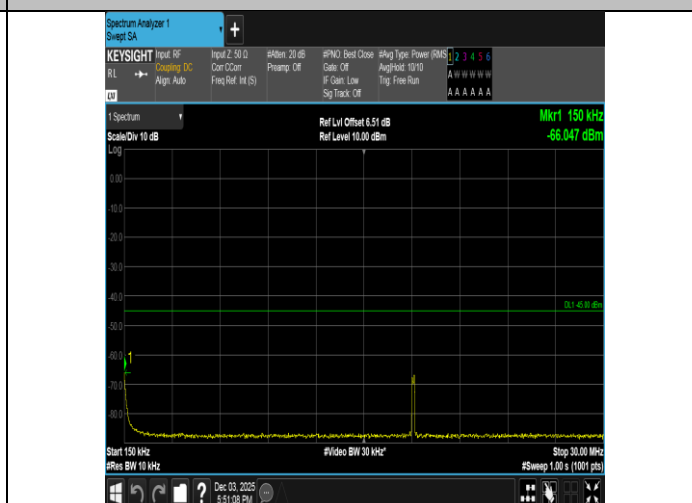
Band38-10MHz-16QAM-37800-1RB#49-0.15~30-PASS
