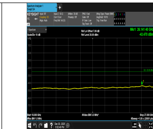
Band38-10MHz-16QAM-37800-1RB#49-18000~27000-PASS
