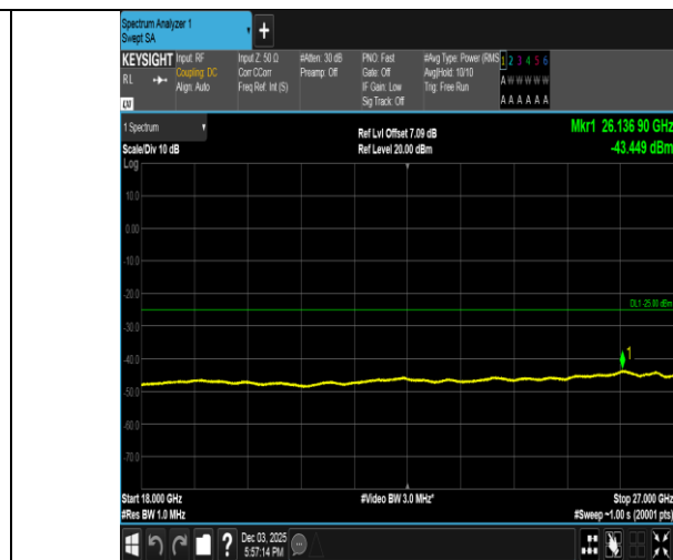
Band38-10MHz-16QAM-37800-50RB#0-18000~27000-PASS
