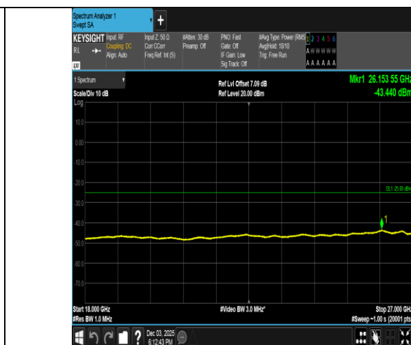
Band38-10MHz-QPSK-38200-1RB#0-18000~27000-PASS
