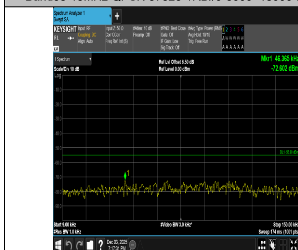
Band38-15MHz-QPSK-37825-1RB#74-0.009~0.15-PASS
