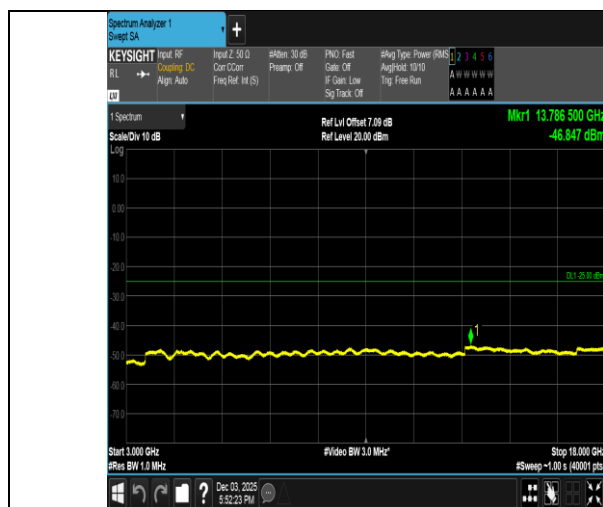
Band38-10MHz-16QAM-37800-1RB#49-3000~18000-PASS
