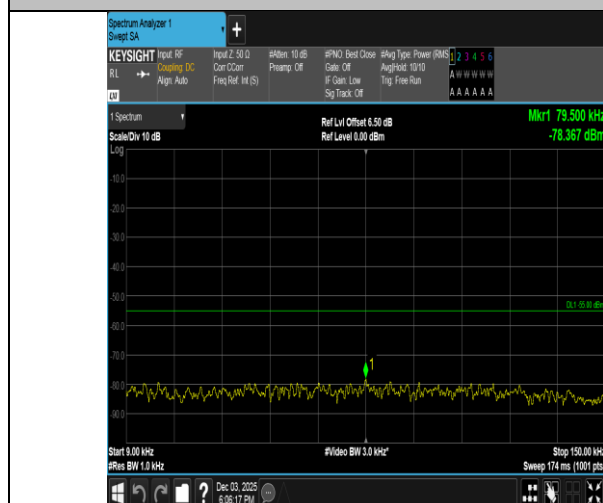
Band38-10MHz-QPSK-38000-50RB#0-0.009~0.15-PASS
