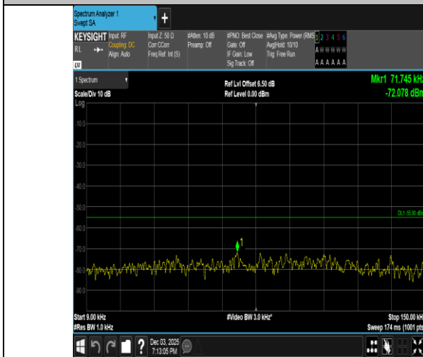
Band38-15MHz-QPSK-37825-1RB#0-0.009~0.15-PASS
