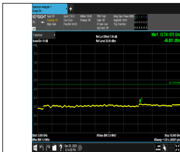
Band38-10MHz-16QAM-38200-1RB#0-3000~18000-PASS
