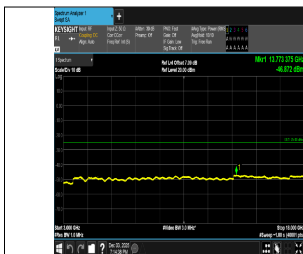
Band38-15MHz-QPSK-37825-1RB#0-3000~18000-PASS
