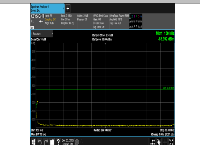
Band38-10MHz-16QAM-38000-50RB#0-0.15~30-PASS
