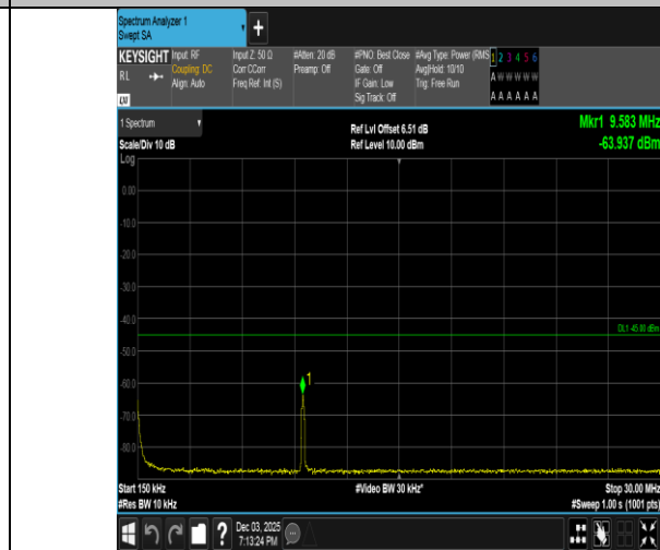
Band38-15MHz-QPSK-37825-1RB#0-0.15~30-PASS
