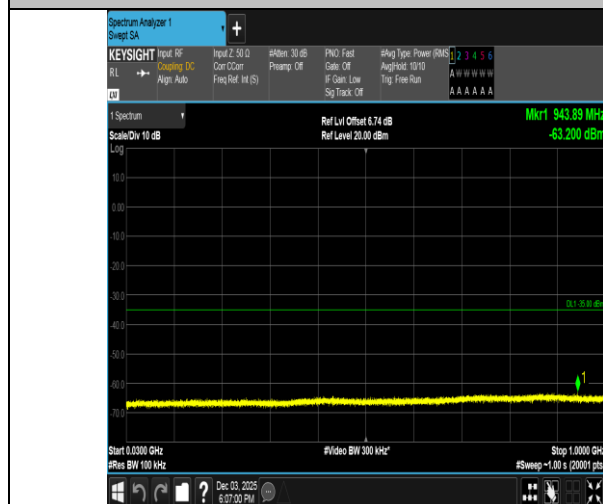
Band38-10MHz-QPSK-38000-50RB#0-30~1000-PASS
