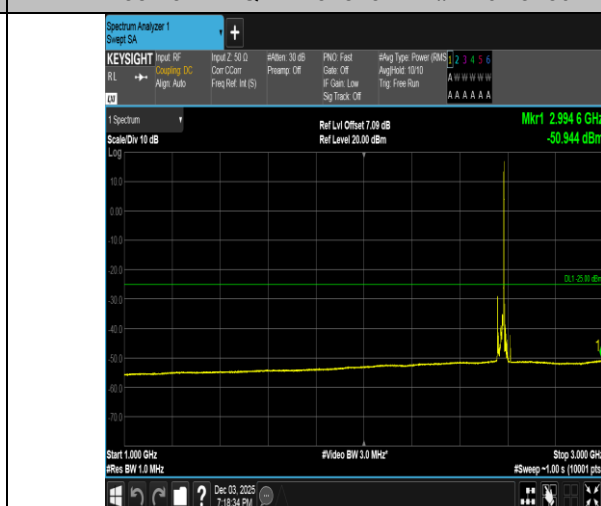
Band38-15MHz-QPSK-37825-1RB#74-1000~3000-PASS
