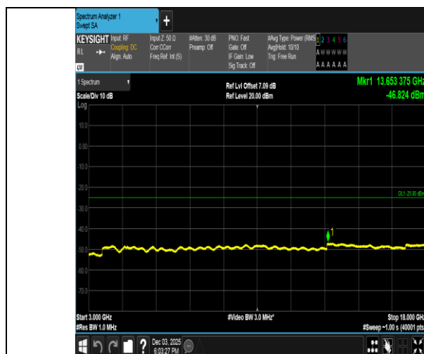
Band38-10MHz-QPSK-38000-1RB#49-3000~18000-PASS
