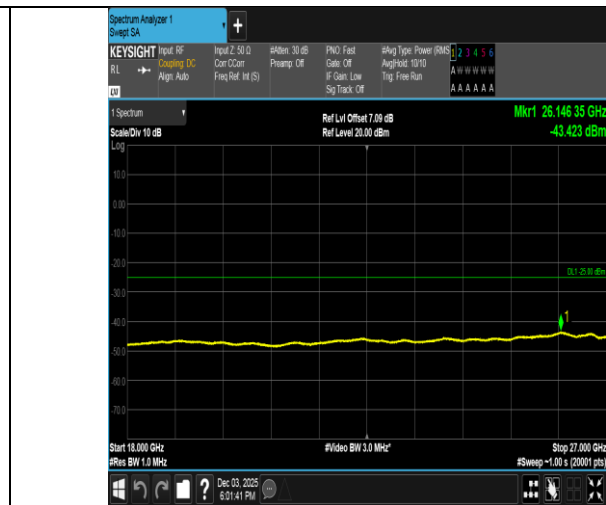
Band38-10MHz-16QAM-38000-1RB#0-18000~27000-PASS
