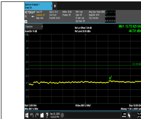
Band38-10MHz-16QAM-38200-50RB#0-3000~18000-PASS
