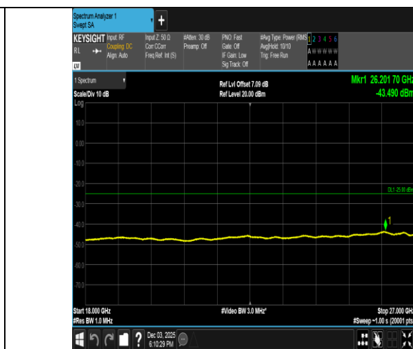
Band38-10MHz-16QAM-38000-50RB#0-18000~27000-PASS
