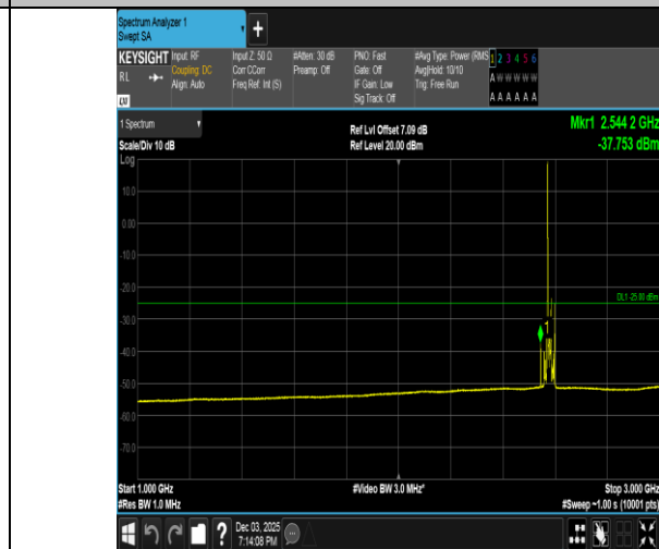
Band38-15MHz-QPSK-37825-1RB#0-1000~3000-PASS
