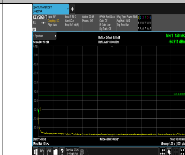
Band38-10MHz-16QAM-38200-50RB#0-0.15~30-PASS
