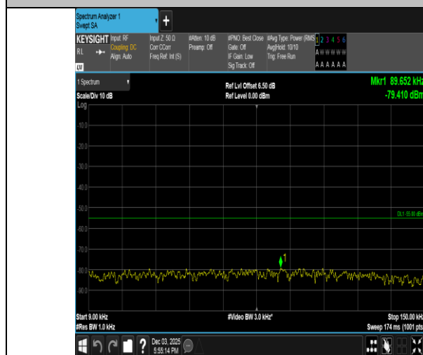
Band38-10MHz-16QAM-37800-50RB#0-0.009~0.15-PASS
