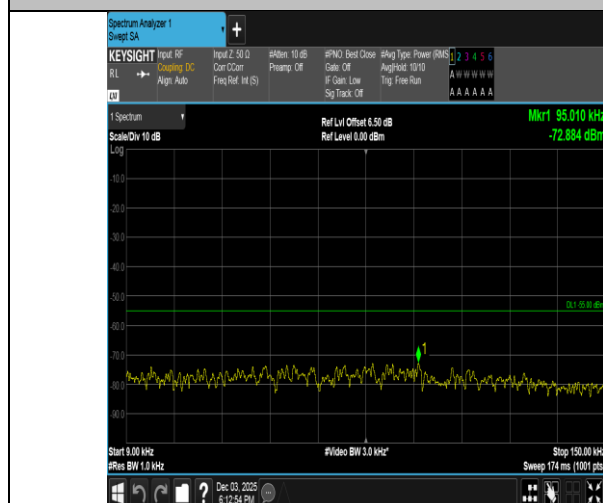
Band38-10MHz-16QAM-38200-1RB#0-0.009~0.15-PASS
