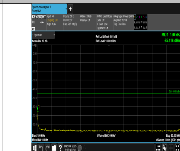
Band38-10MHz-QPSK-38000-50RB#0-0.15~30-PASS
