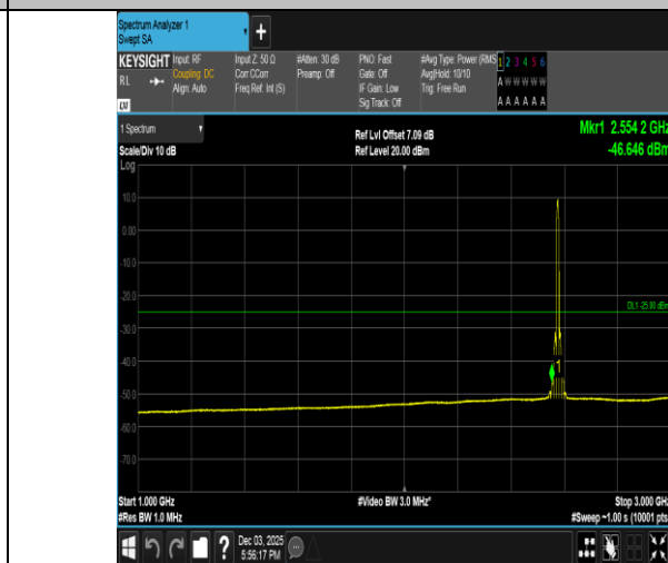
Band38-10MHz-16QAM-37800-50RB#0-1000~3000-PASS
