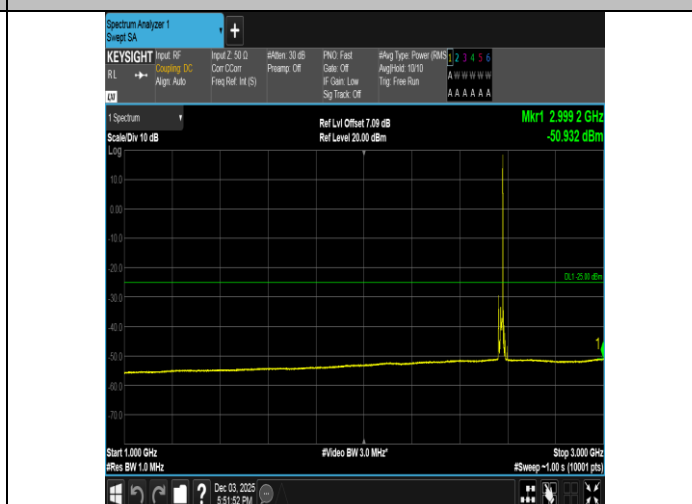
Band38-10MHz-16QAM-37800-1RB#49-1000~3000-PASS
