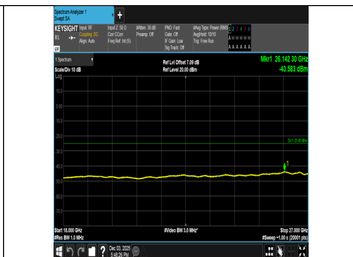
Band38-10MHz-16QAM-37800-1RB#0-18000~27000-PASS
