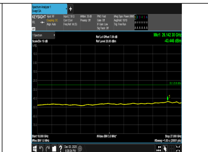
Band38-10MHz-16QAM-38000-1RB#49-18000~27000-PASS
