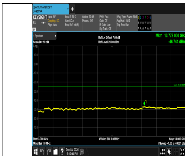
Band38-10MHz-16QAM-38000-50RB#0-3000~18000-PASS
