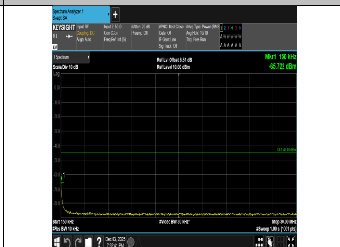
Band38-15MHz-16QAM-38000-1RB#74-0.15~30-PASS
