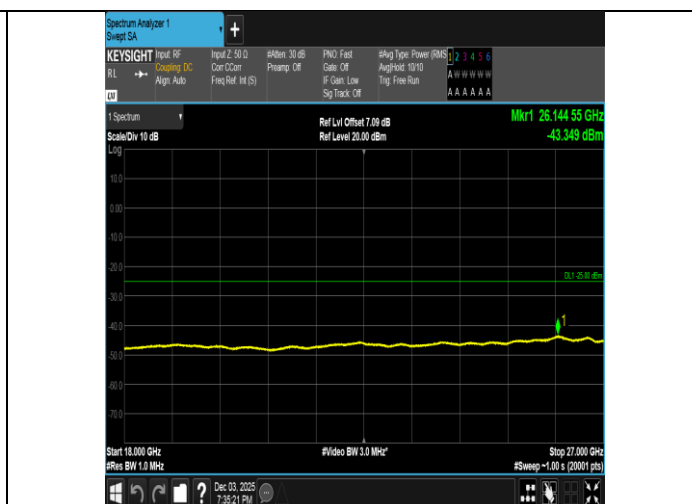
Band38-15MHz-16QAM-38000-1RB#74-18000~27000-PASS
