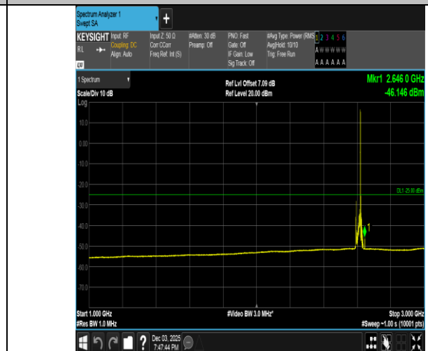
Band38-15MHz-16QAM-38175-1RB#74-1000~3000-PASS
