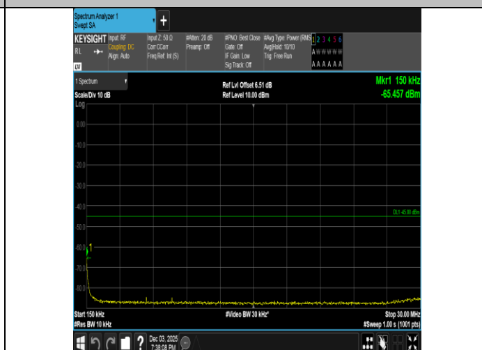
Band38-15MHz-16QAM-38000-75RB#0-0.15~30-PASS
