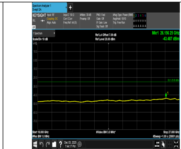
Band38-15MHz-16QAM-38175-1RB#0-18000~27000-PASS
