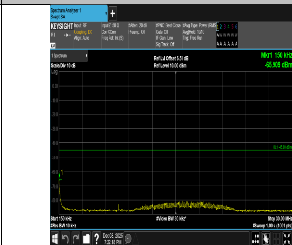
Band38-15MHz-QPSK-37825-75RB#0-0.15~30-PASS
