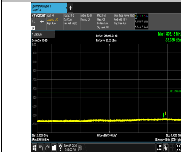
Band38-15MHz-16QAM-37825-1RB#0-30~1000-PASS
