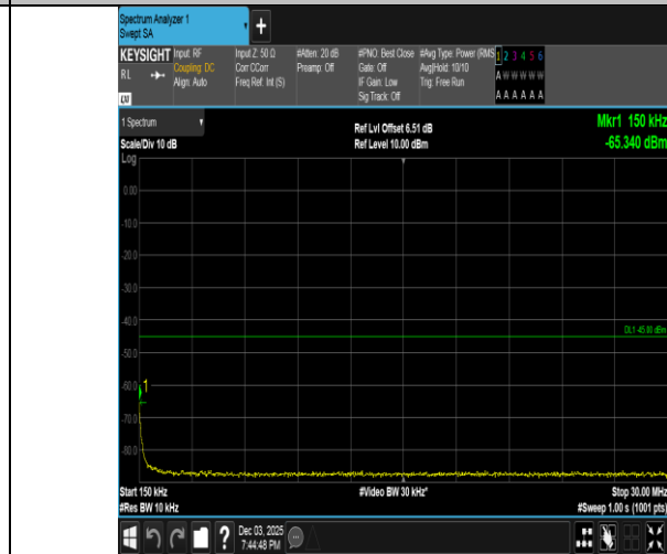
Band38-15MHz-QPSK-38175-1RB#74-0.15~30-PASS
