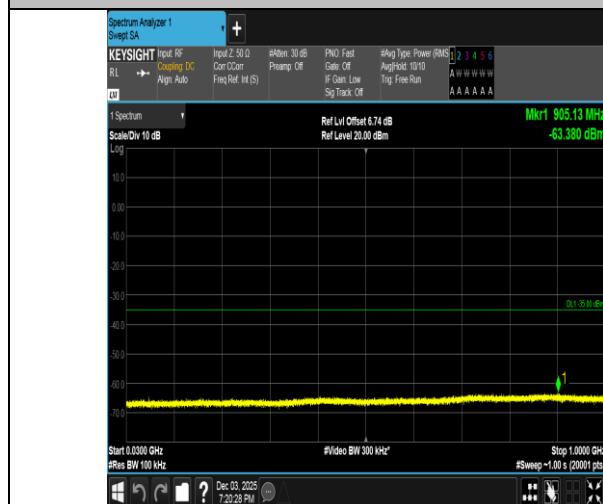
Band38-15MHz-16QAM-37825-1RB#74-30~1000-PASS
