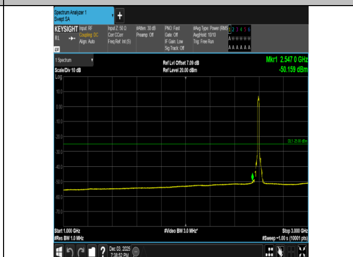
Band38-15MHz-16QAM-38000-75RB#0-1000~3000-PASS
