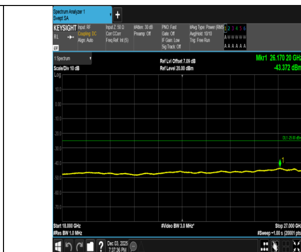
Band38-15MHz-QPSK-38000-75RB#0-18000~27000-PASS
