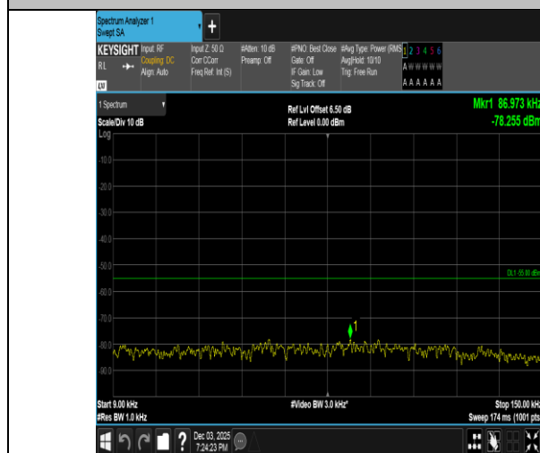
Band38-15MHz-16QAM-37825-75RB#0-0.009~0.15-PASS
