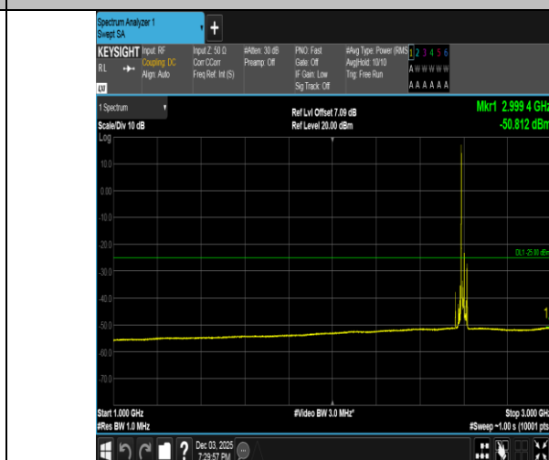
Band38-15MHz-16QAM-38000-1RB#0-1000~3000-PASS
