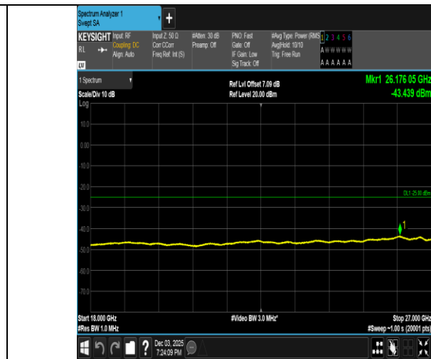
Band38-15MHz-QPSK-37825-75RB#0-18000~27000-PASS
