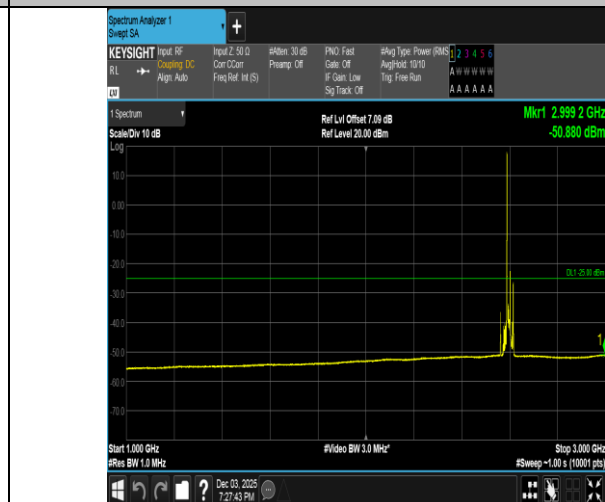
Band38-15MHz-QPSK-38000-1RB#0-1000~3000-PASS
