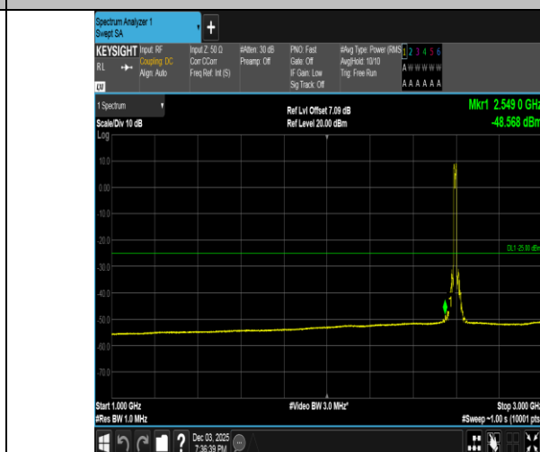
Band38-15MHz-QPSK-38000-75RB#0-1000~3000-PASS
