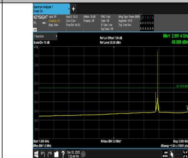
Band38-15MHz-16QAM-37825-1RB#74-1000~3000-PASS
