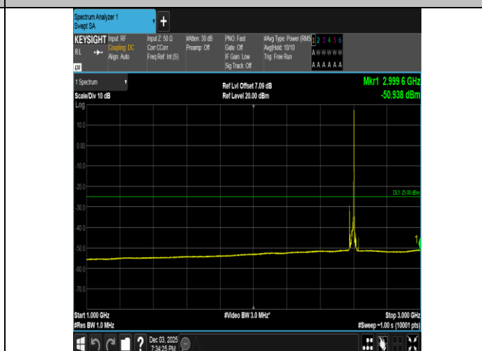
Band38-15MHz-16QAM-38000-1RB#74-1000~3000-PASS
