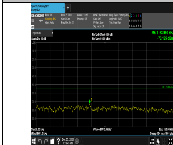
Band38-15MHz-16QAM-37825-1RB#74-0.009~0.15-PASS
