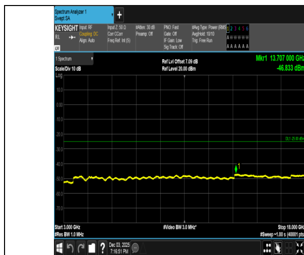
Band38-15MHz-16QAM-37825-1RB#0-3000~18000-PASS
