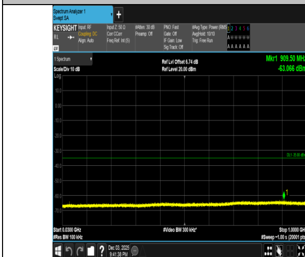
Band38-20MHz-QPSK-38150-1RB#99-30~1000-PASS
