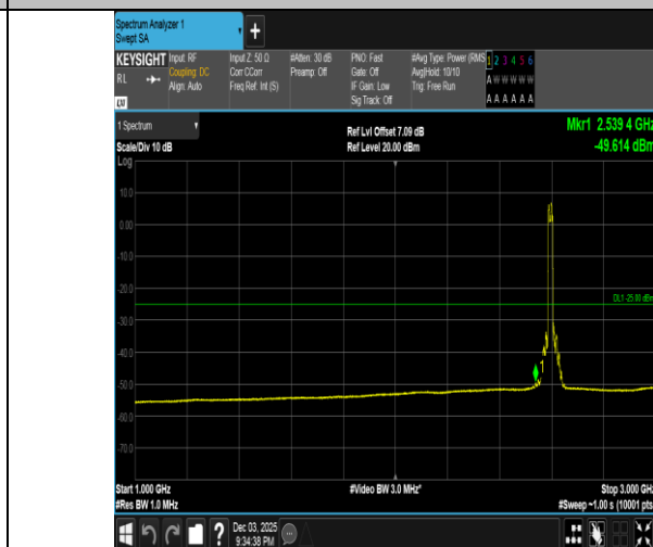
Band38-20MHz-16QAM-38000-100RB#0-1000~3000-PASS
