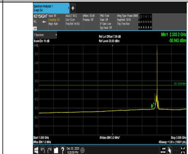
Band38-20MHz-16QAM-38000-1RB#99-1000~3000-PASS
