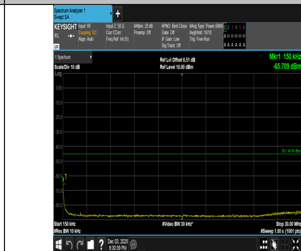
Band38-20MHz-QPSK-38000-100RB#0-0.15~30-PASS
