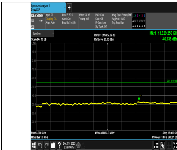
Band38-20MHz-QPSK-37850-100RB#0-3000~18000-PASS
