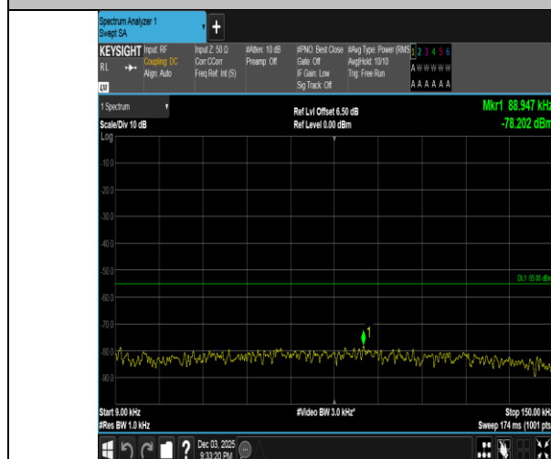
Band38-20MHz-16QAM-38000-100RB#0-0.009~0.15-PASS
