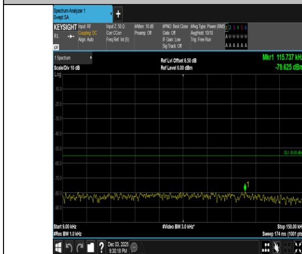
Band38-20MHz-QPSK-38000-100RB#0-0.009~0.15-PASS
