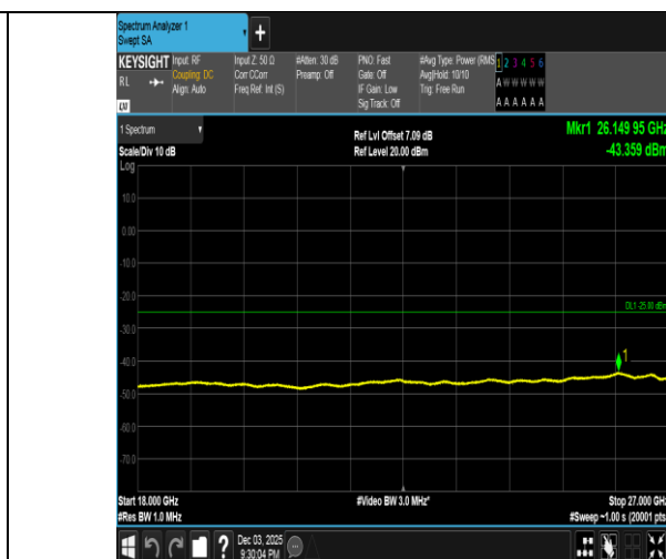
Band38-20MHz-16QAM-38000-1RB#99-18000~27000-PASS
