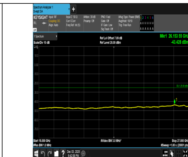
Band38-20MHz-QPSK-38150-1RB#99-18000~27000-PASS
