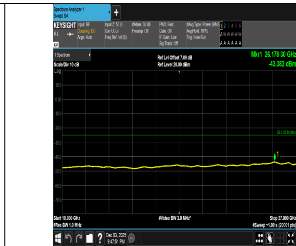
Band38-20MHz-QPSK-38150-100RB#0-18000~27000-PASS
