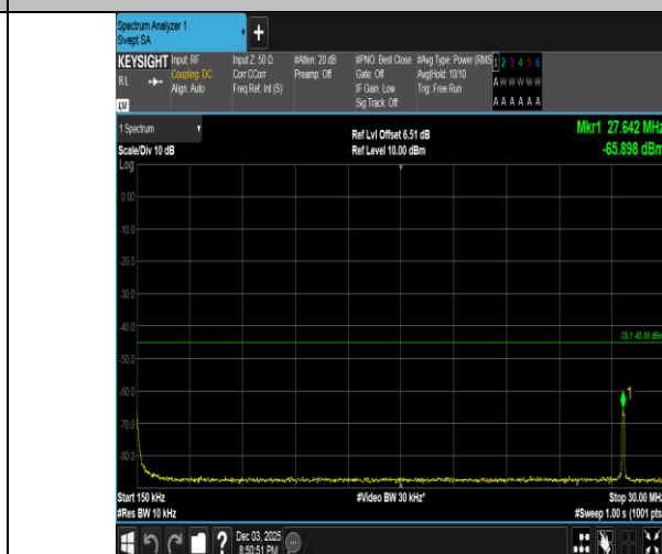
Band38-20MHz-QPSK-37850-1RB#99-0.15~30-PASS
