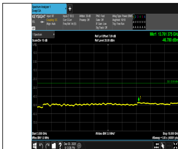
Band38-20MHz-QPSK-38000-1RB#0-3000~18000-PASS
