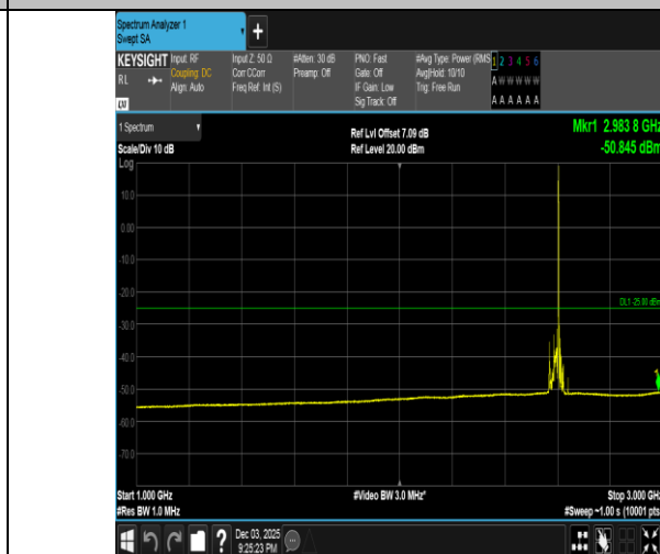
Band38-20MHz-QPSK-38000-1RB#99-1000~3000-PASS
