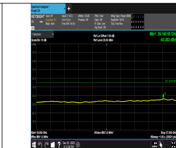
Band38-20MHz-QPSK-38000-1RB#0-18000~27000-PASS
