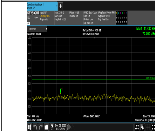
Band38-20MHz-16QAM-37850-1RB#0-0.009~0.15-PASS
