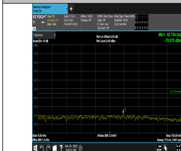
Band38-20MHz-QPSK-38150-100RB#0-0.009~0.15-PASS
