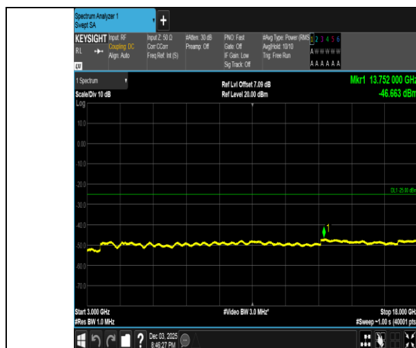
Band38-20MHz-QPSK-37850-1RB#0-3000~18000-PASS
