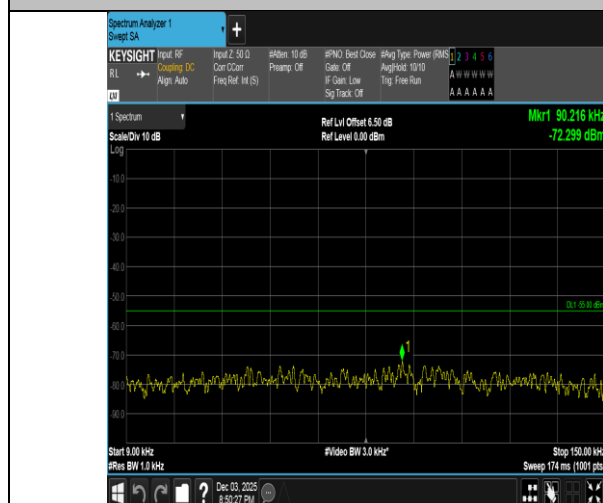
Band38-20MHz-QPSK-37850-1RB#99-0.009~0.15-PASS
