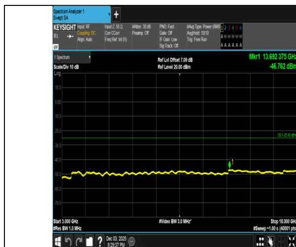
Band38-20MHz-16QAM-38000-1RB#99-3000~18000-PASS
