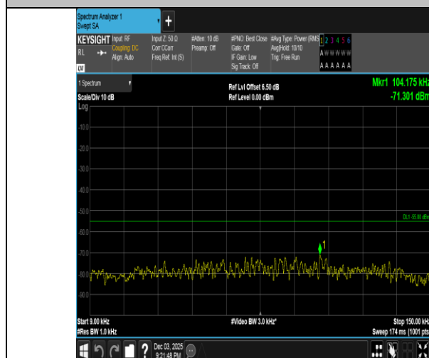
Band38-20MHz-QPSK-38000-1RB#99-0.009~0.15-PASS
