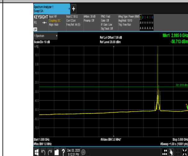
Band38-20MHz-QPSK-38000-1RB#0-1000~3000-PASS
