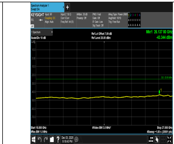
Band38-20MHz-16QAM-38000-1RB#0-18000~27000-PASS
