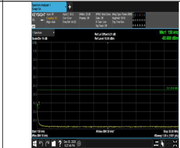
Band38-20MHz-16QAM-38000-1RB#99-0.15~30-PASS
