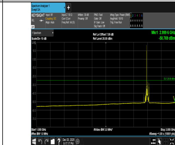
Band38-20MHz-16QAM-38000-1RB#0-1000~3000-PASS
