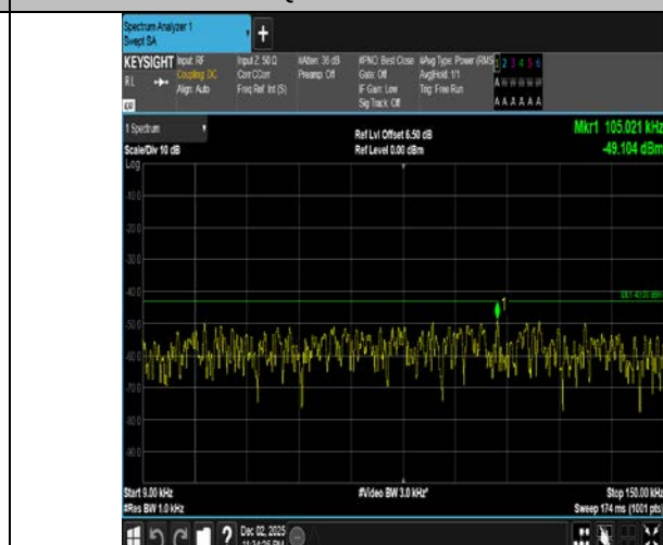
Band4-1.4MHz-16QAM-20175-6RB#0-0.009~0.15-PASS
