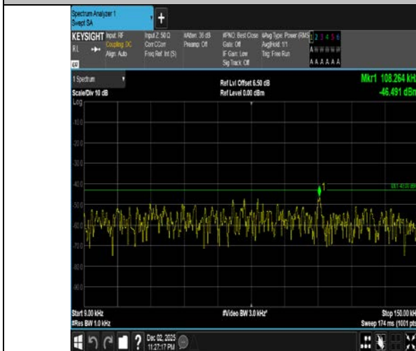
Band4-1.4MHz-QPSK-19957-6RB#0-0.009~0.15-PASS
