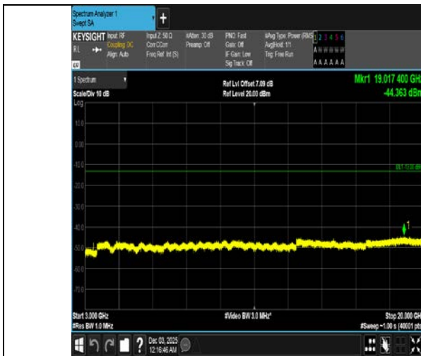
Band4-3MHz-QPSK-19965-15RB#0-3000~20000-PASS
