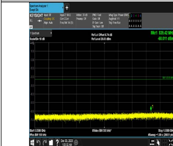
Band4-5MHz-QPSK-19975-25RB#0-30~1000-PASS
