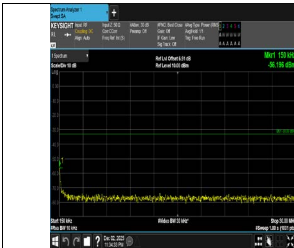
Band4-1.4MHz-16QAM-20175-6RB#0-0.15~30-PASS
