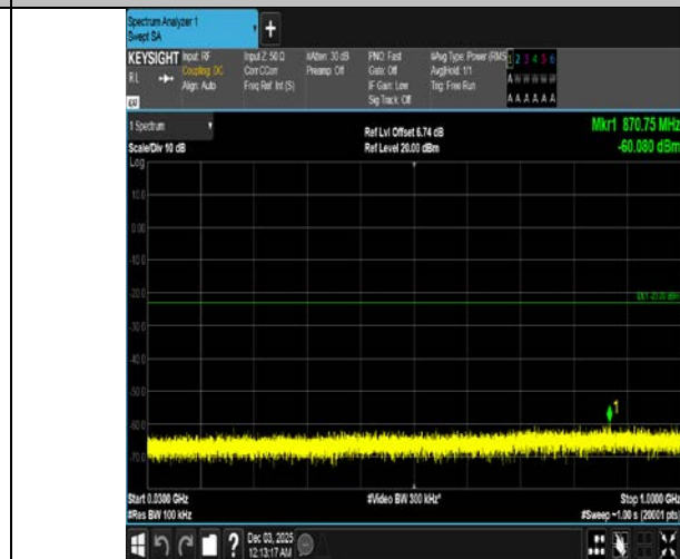
Band4-3MHz-16QAM-19965-1RB#0-30~1000-PASS
