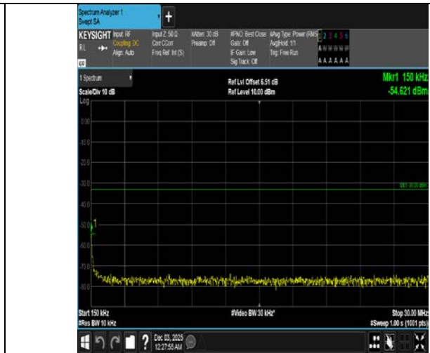
Band4-3MHz-16QAM-20385-1RB#14-0.15-30-PASS
