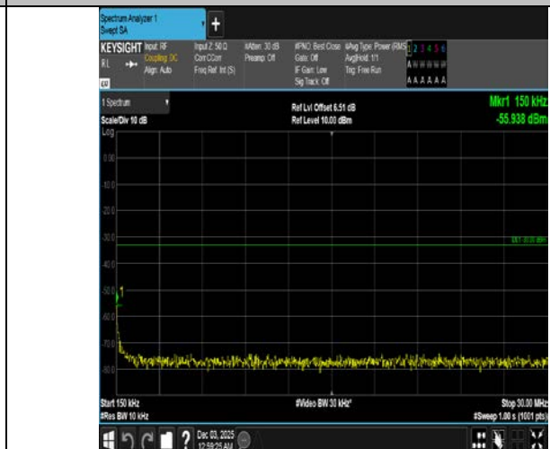
Band4-5MHz-QPSK-19975-1RB#0-0.15~30-PASS
