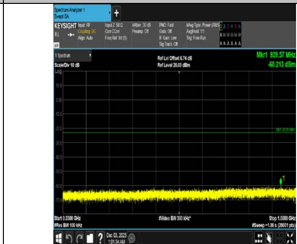
Band4-5MHz-QPSK-19975-1RB#24-30~1000-PASS
