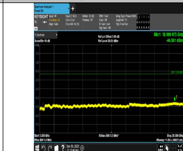
Band4-3MHz-16QAM-19965-1RB#0-3000~20000-PASS
