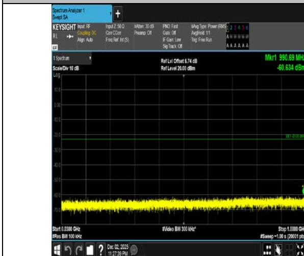
Band4-1.4MHz-QPSK-19957-6RB#0-30~1000-PASS
