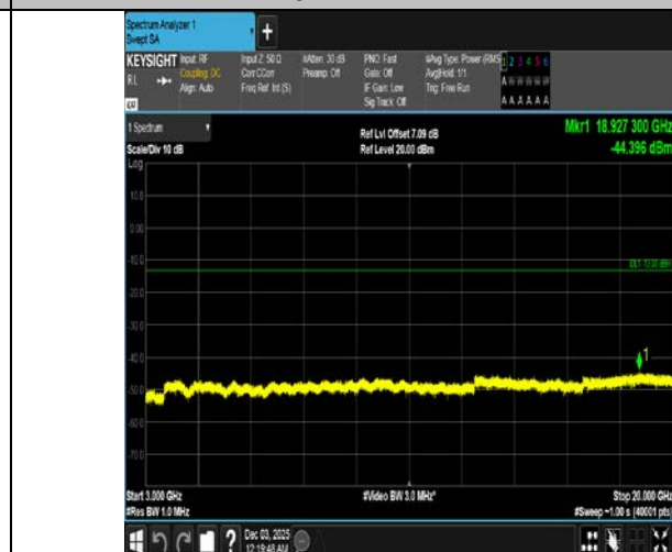
Band4-3MHz-16QAM-20175-1RB#0-3000~20000-PASS
