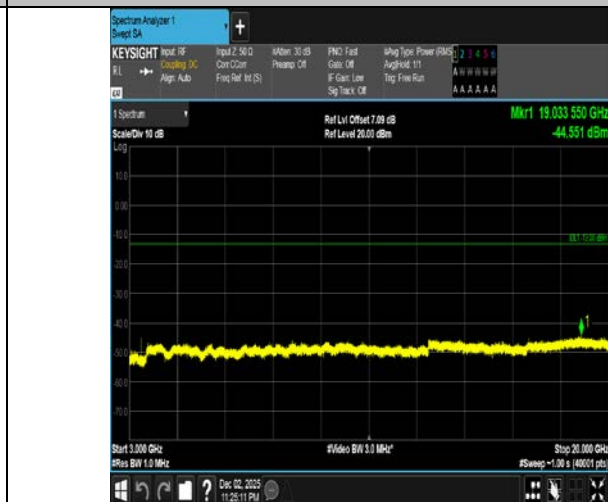
Band4-1.4MHz-16QAM-19957-1RB#0-3000~20000-PASS
