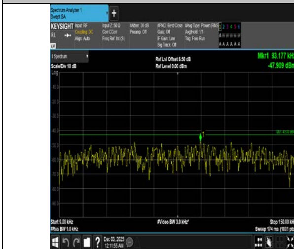
Band4-3MHz-QPSK-19965-1RB#0-0.009~0.15-PASS
