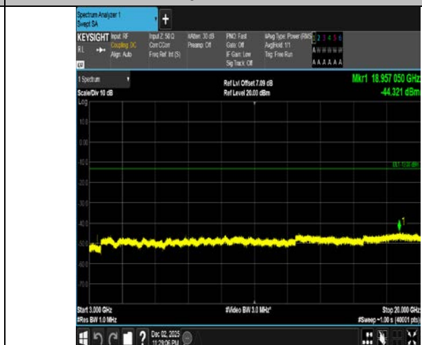
Band4-1.4MHz-16QAM-19957-6RB#0-3000~20000-PASS
