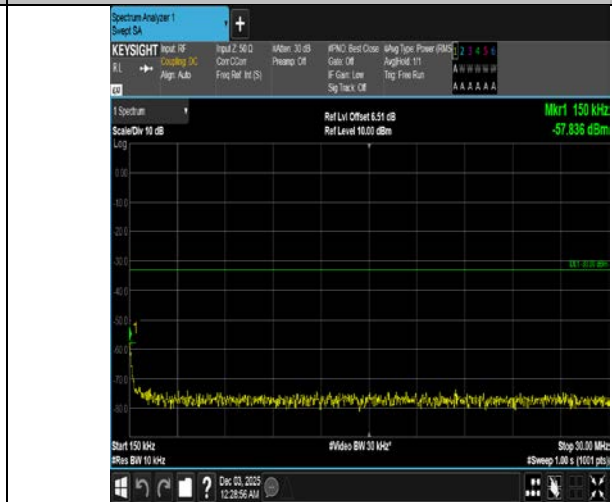
Band4-3MHz-QPSK-20385-15RB#0-0.15~30-PASS
