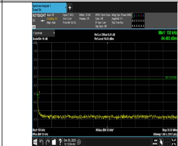
Band4-3MHz-QPSK-19965-1RB#0-0.15~30-PASS
