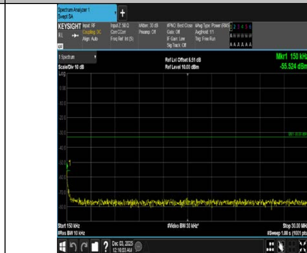
Band4-3MHz-QPSK-19965-15RB#0-0.15~30-PASS
