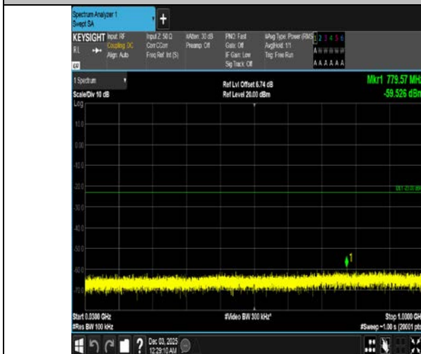
Band4-3MHz-QPSK-20385-15RB#0-30~1000-PASS
