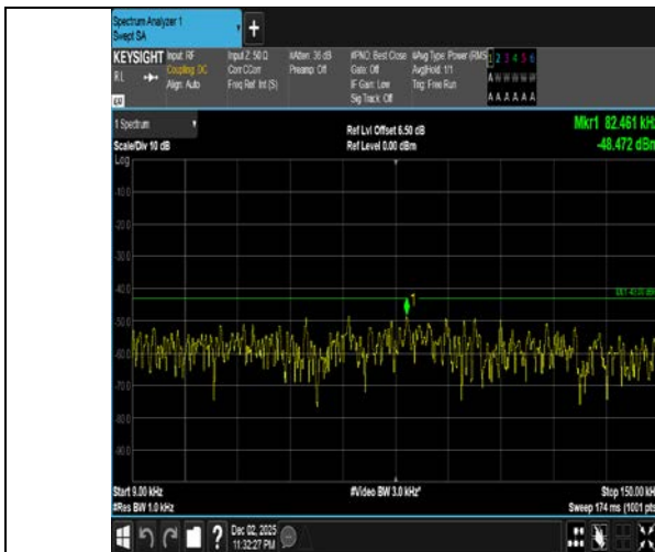
Band4-1.4MHz-16QAM-20175-1RB#5-0.009~0.15-PASS
