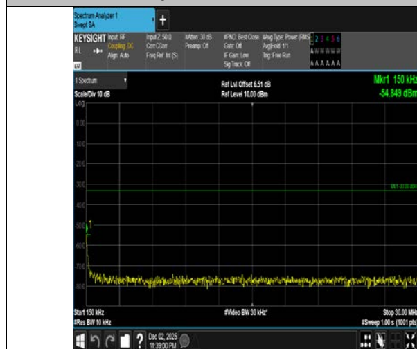
Band4-1.4MHz-QPSK-20393-1RB#5-0.15~30-PASS
