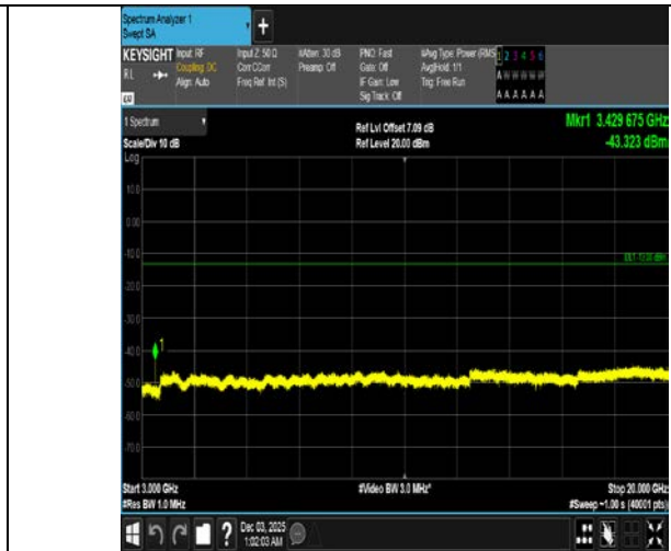
Band4-5MHz-QPSK-19975-1RB#24-3000~20000-PASS
