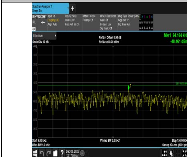
Band4-3MHz-QPSK-20175-1RB#0-0.009~0.15-PASS
