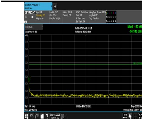
Band4-5MHz-QPSK-19975-1RB#24-0.15~30-PASS
