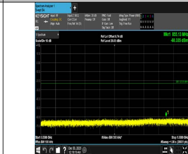
Band4-3MHz-16QAM-20175-1RB#0-30~1000-PASS
