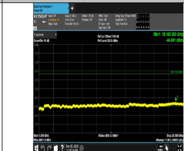
Band4-1.4MHz-16QAM-20175-6RB#0-3000~20000-PASS
