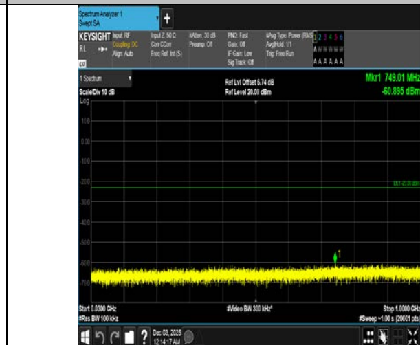
Band4-3MHz-QPSK-19965-1RB#14-30~1000-PASS
