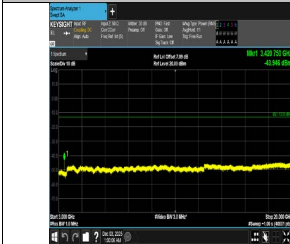
Band4-5MHz-QPSK-19975-1RB#0-3000~20000-PASS
