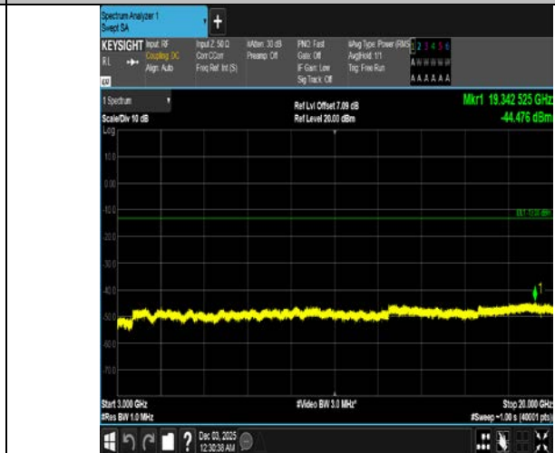
Band4-3MHz-16QAM-20385-15RB#0-3000~20000-PASS
