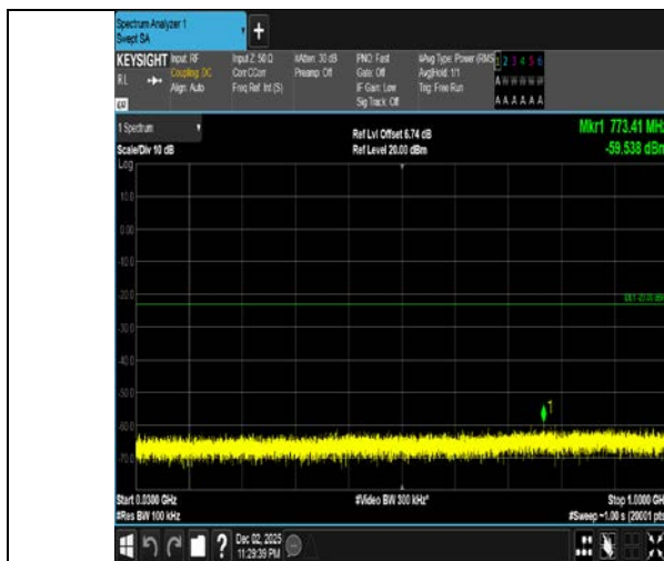
Band4-1.4MHz-QPSK-20175-1RB#0-30~1000-PASS
