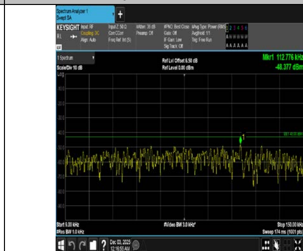
Band4-3MHz-16QAM-19965-15RB#0-0.009-0.15-PASS
