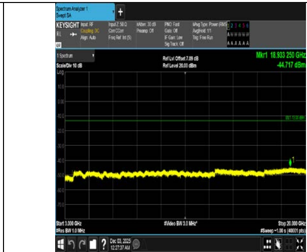
Band4-3MHz-QPSK-20385-1RB#14-3000~20000-PASS
