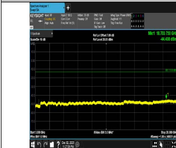
Band4-1.4MHz-16QAM-19957-1RB#5-3000~20000-PASS
