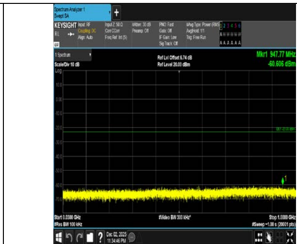
Band4-1.4MHz-16QAM-20175-6RB#0-30~1000-PASS
