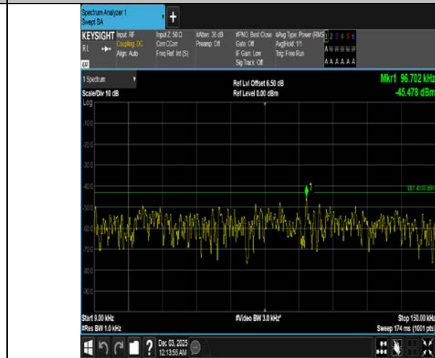
Band4-3MHz-QPSK-19965-1RB#14-0.009~0.15-PASS
