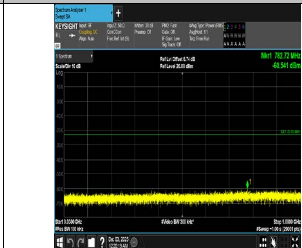
Band4-3MHz-QPSK-20175-1RB#14-30~1000-PASS
