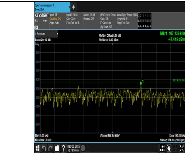
Band4-3MHz-16QAM-20175-1RB#0-0.009~0.15-PASS
