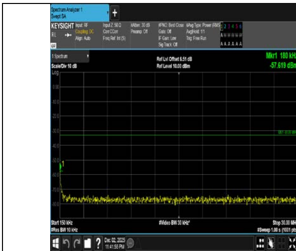
Band4-1.4MHz-16QAM-20393-6RB#0-0.15~30-PASS
