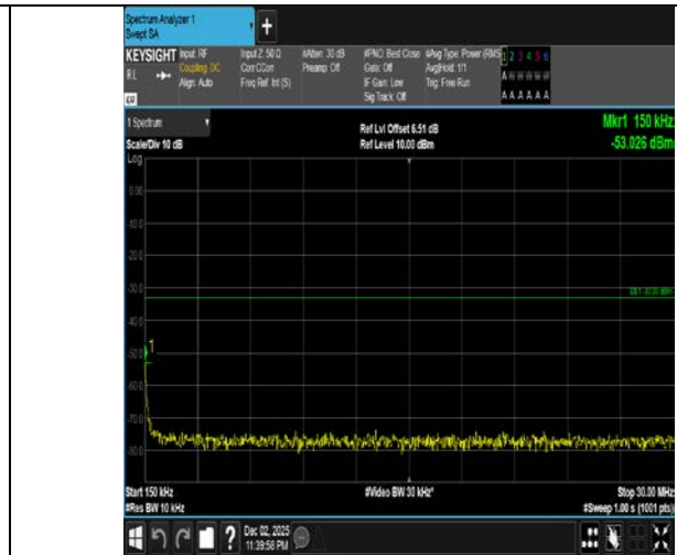
Band4-1.4MHz-16QAM-20393-1RB#5-0.15~30-PASS
