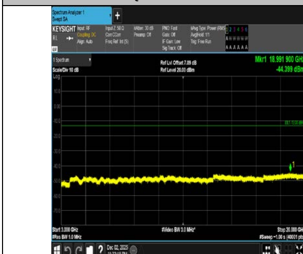
Band4-1.4MHz-16QAM-20175-1RB#5-3000~20000-PASS
