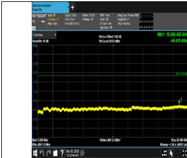
Band4-3MHz-QPSK-20175-15RB#0-3000~20000-PASS
