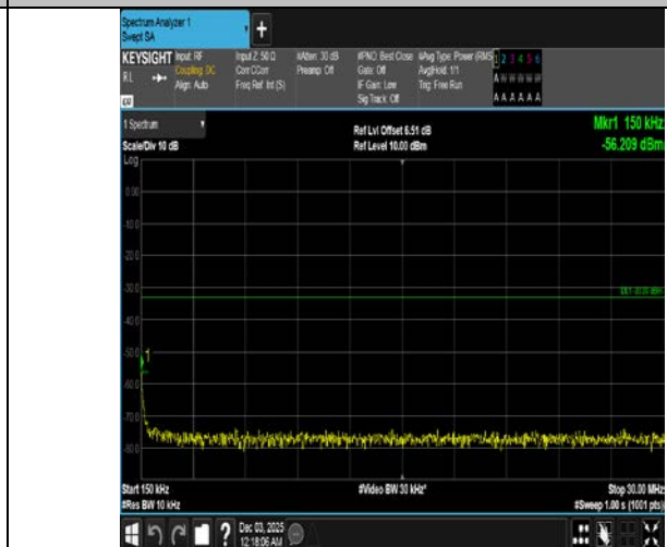
Band4-3MHz-QPSK-20175-1RB#0-0.15~30-PASS
