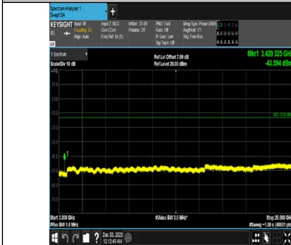
Band4-3MHz-QPSK-19965-1RB#0-3000~20000-PASS
