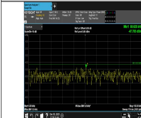
Band4-5MHz-QPSK-19975-1RB#0-0.009~0.15-PASS
