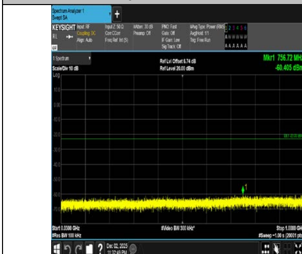
Band4-1.4MHz-16QAM-20175-1RB#5-30~1000-PASS
