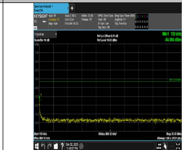
Band4-1.4MHz-QPSK-20393-6RB#0-0.15~30-PASS
