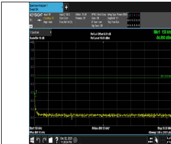
Band4-1.4MHz-16QAM-19957-6RB#0-0.15~30-PASS
