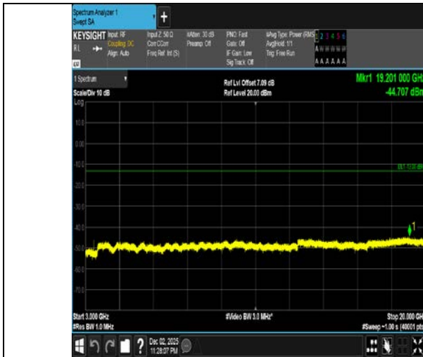
Band4-1.4MHz-QPSK-19957-6RB#0-3000~20000-PASS
