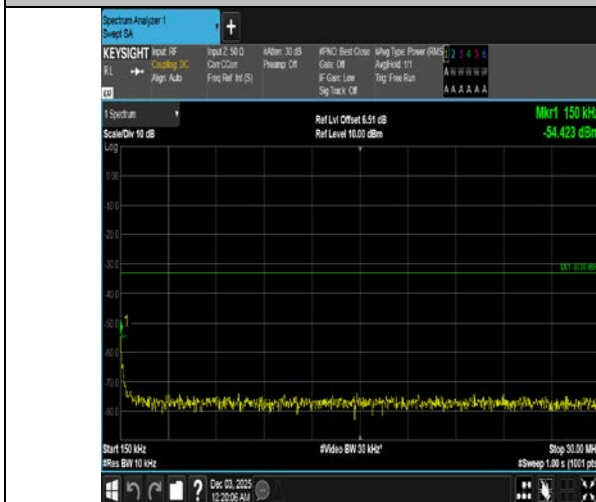
Band4-3MHz-QPSK-20175-1RB#14-0.15~30-PASS
