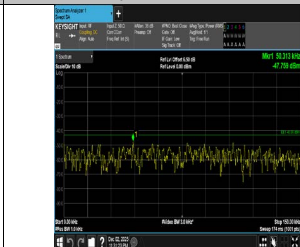
Band4-1.4MHz-QPSK-20175-1RB#5-0.009~0.15-PASS
