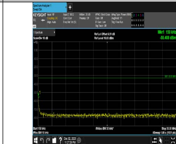
Band4-1.4MHz-QPSK-19957-6RB#0-0.15~30-PASS
