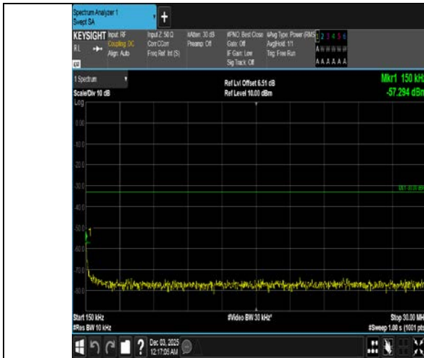
Band4-3MHz-16QAM-19965-15RB#0-0.15~30-PASS
