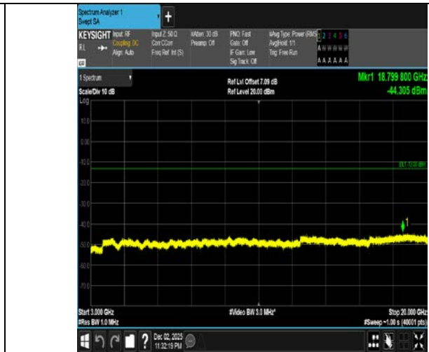
Band4-1.4MHz-QPSK-20175-1RB#5-3000~20000-PASS
