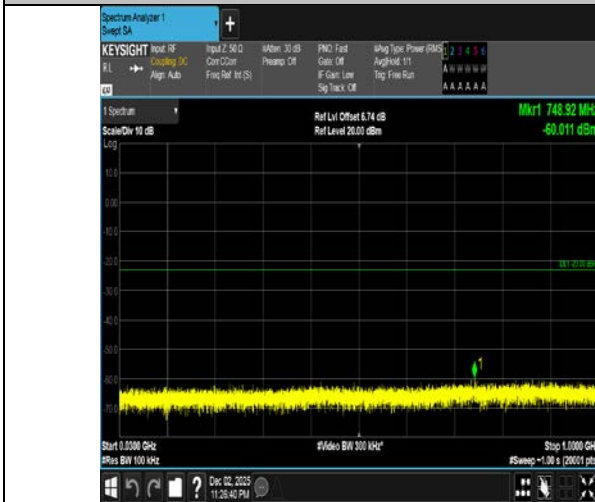
Band4-1.4MHz-16QAM-19957-1RB#5-30~1000-PASS
