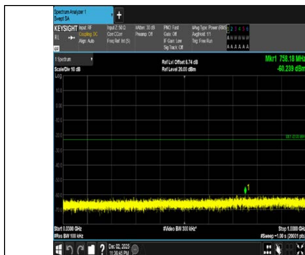
Band4-1.4MHz-OPSK-20393-1RB#0-30~1000-PASS
