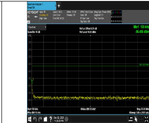
Band4-1.4MHz-16QAM-19957-1RB#5-0.15~30-PASS
