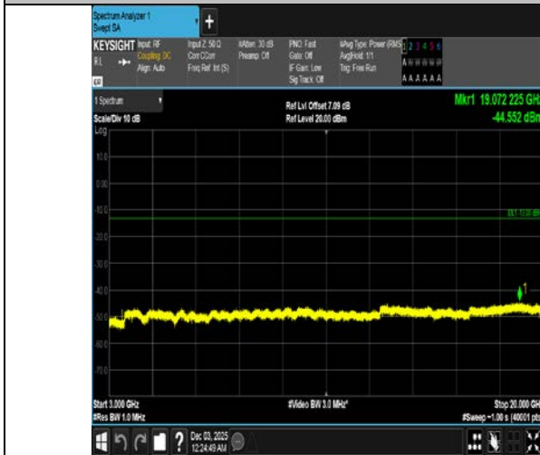
Band4-3MHz-QPSK-20385-1RB#0-3000~20000-PASS
