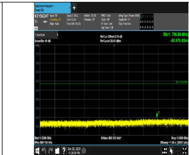
Band4-1.4MHz-16QAM-19957-6RB#0-30~1000-PASS
