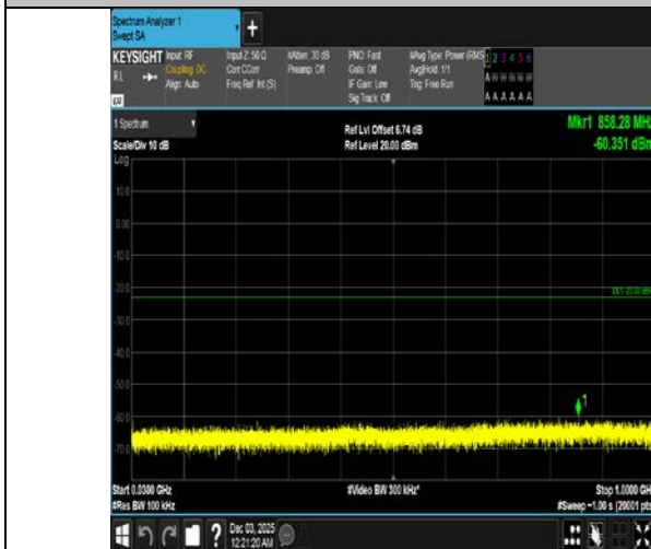
Band4-3MHz-16QAM-20175-1RB#14-30-1000-PASS
