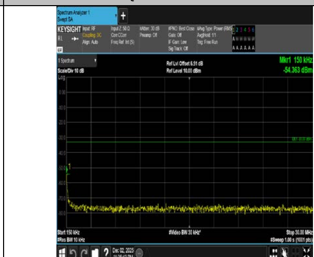
Band4-1.4MHz-QPSK-20393-1RB#0-0.15~30-PASS
