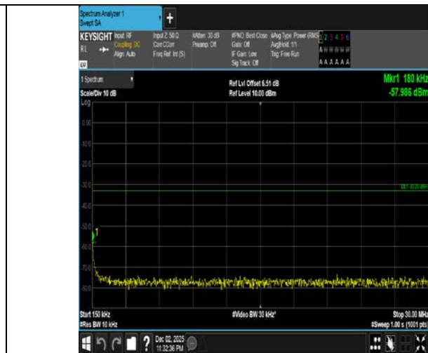
Band4-1.4MHz-16QAM-20175-1RB#5-0.15~30-PASS
