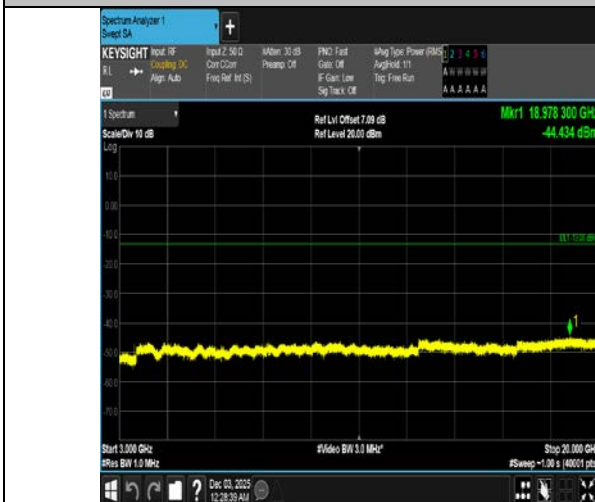
Band4-3MHz-16QAM-20385-1RB#14-3000-20000-PASS
