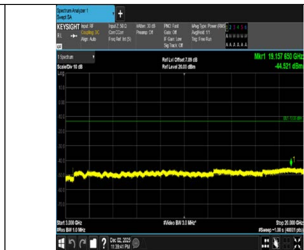
Band4-1.4MHz-QPSK-20393-1RB#5-3000~20000-PASS
