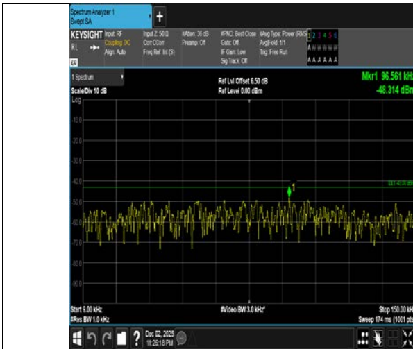
Band4-1.4MHz-16QAM-19957-1RB#5-0.009~0.15-PASS
