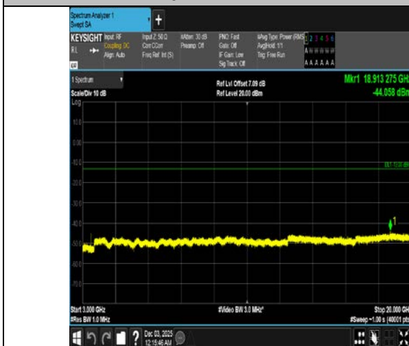
Band4-3MHz-16QAM-19965-1RB#14-3000-20000-PASS
