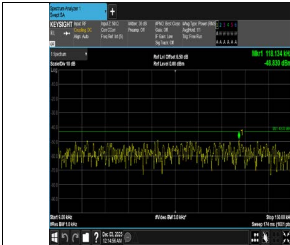
Band4-3MHz-16QAM-19965-1RB#14-0.009-0.15-PASS
