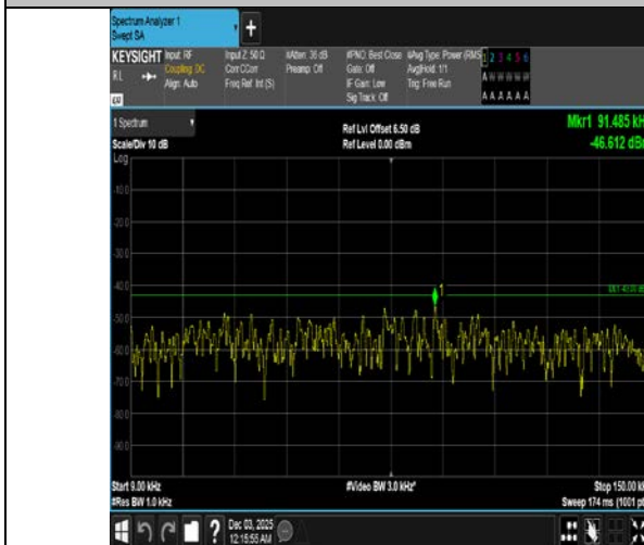
Band4-3MHz-QPSK-19965-15RB#0-0.009~0.15-PASS
