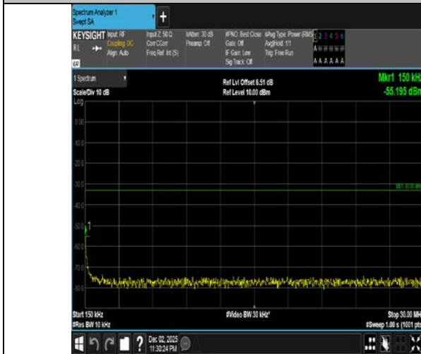
Band4-1.4MHz-16QAM-20175-1RB#0-0.15~30-PASS
