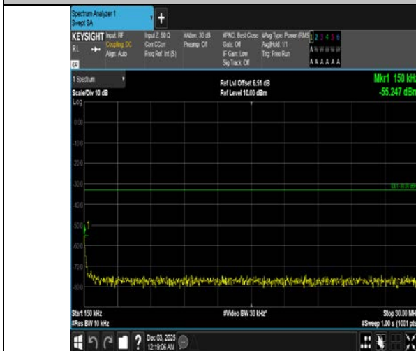
Band4-3MHz-16QAM-20175-1RB#0-0.15~30-PASS
