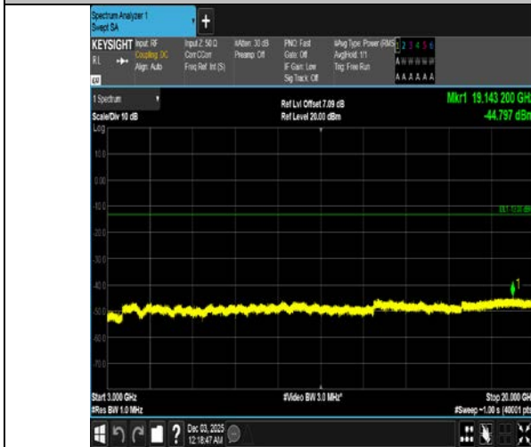
Band4-3MHz-QPSK-20175-1RB#0-3000~20000-PASS
