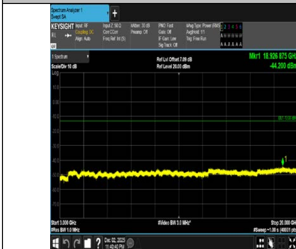
Band4-1.4MHz-16QAM-20393-1RB#5-3000~20000-PASS
