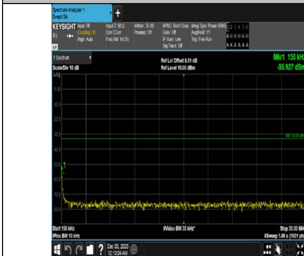
Band4-3MHz-16QAM-19965-1RB#0-0.15~30-PASS
