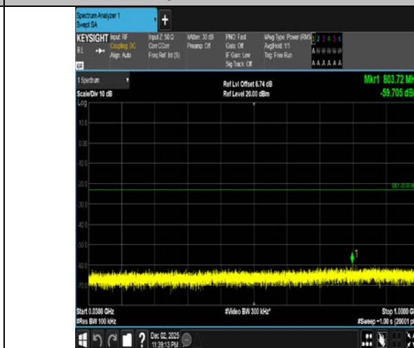
Band4-1.4MHz-QPSK-20393-1RB#5-30~1000-PASS
