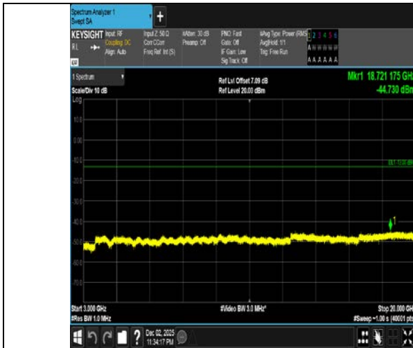
Band4-1.4MHz-QPSK-20175-6RB#0-3000~20000-PASS
