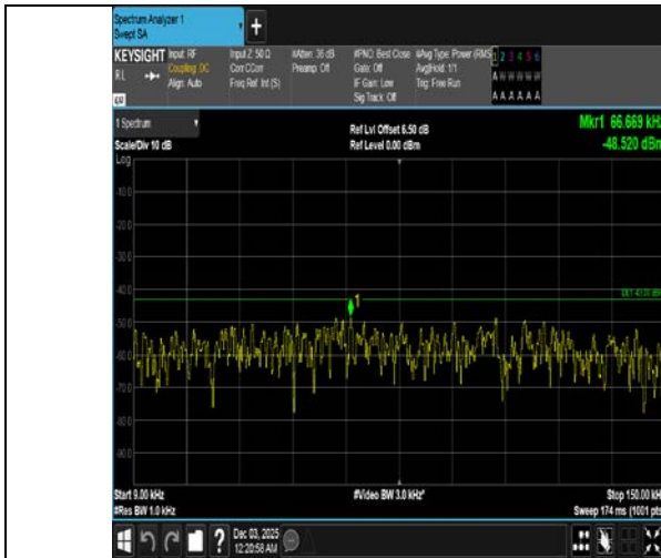
Band4-3MHz-16QAM-20175-1RB#14-0.009-0.15-PASS
