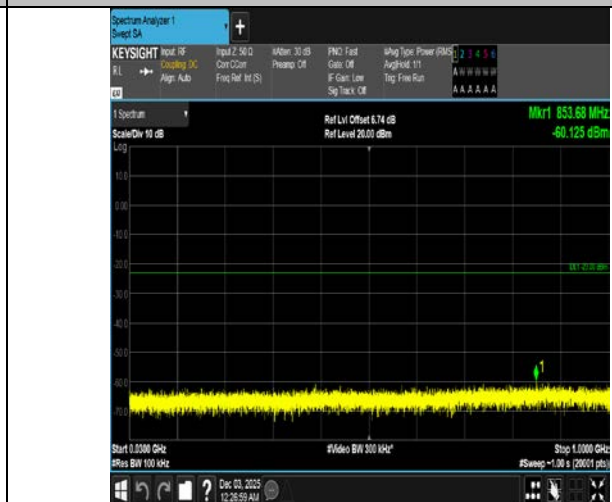
Band4-3MHz-QPSK-20385-1RB#14-30~1000-PASS
