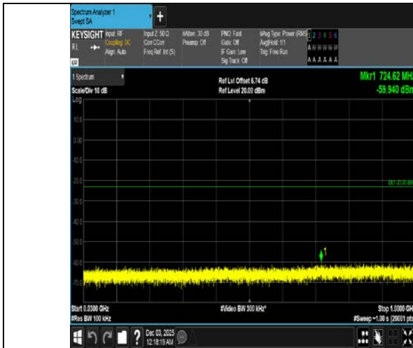
Band4-3MHz-QPSK-20175-1RB#0-30~1000-PASS
