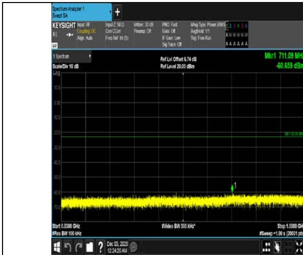
Band4-3MHz-QPSK-20385-1RB#0-30~1000-PASS
