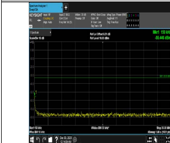
Band4-3MHz-QPSK-19965-1RB#14-0.15~30-PASS
