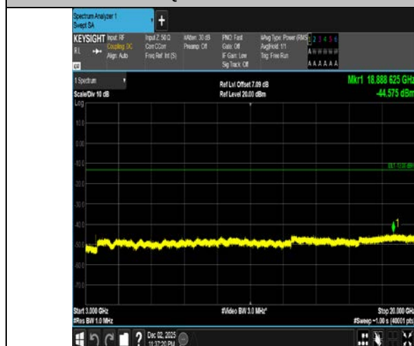
Band4-1.4MHz-OPSK-20393-1RB#0-3000~20000-PASS
