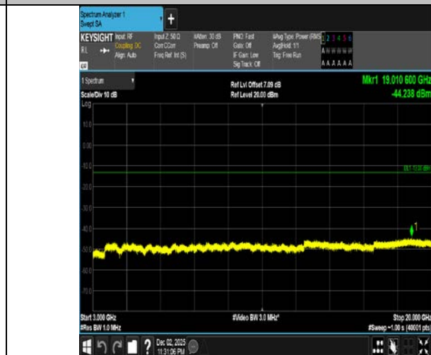
Band4-1.4MHz-16QAM-20175-1RB#0-3000~20000-PASS
