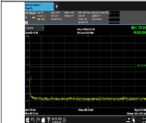
Band4-3MHz-QPSK-20385-1RB#14-0.15~30-PASS
