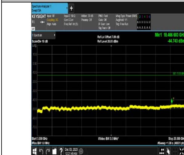
Band4-3MHz-16QAM-20175-1RB#14-3000-20000-PASS
