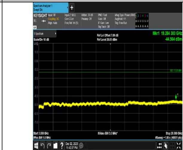
Band4-1.4MHz-16QAM-20393-6RB#0-3000~20000-PASS
