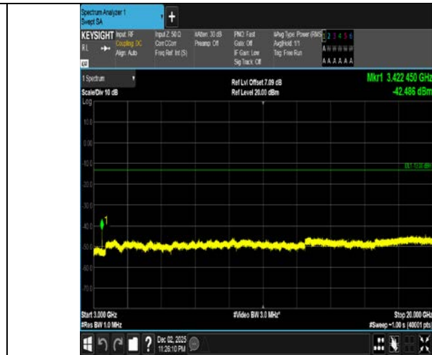
Band4-1.4MHz-QPSK-19957-1RB#5-3000~20000-PASS
