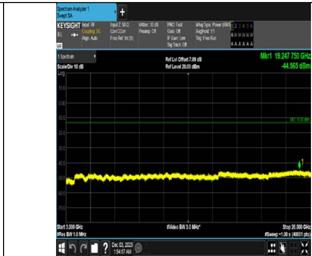
Band4-10MHz-QPSK-20175-1RB#49-3000~20000-PASS
