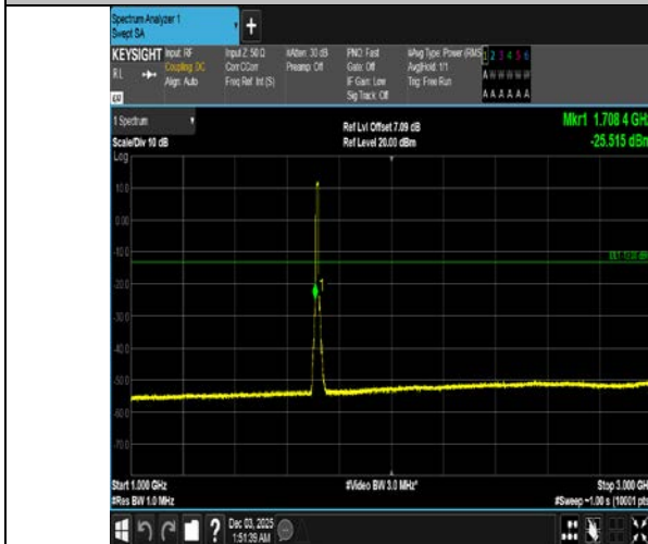
Band4-10MHz-16QAM-20000-50RB#0-1000~3000-PASS
