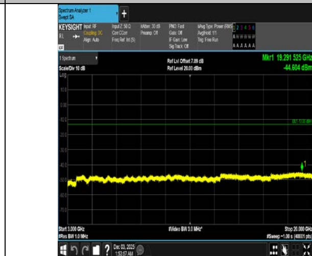
Band4-10MHz-16QAM-20175-1RB#0-3000~20000-PASS
