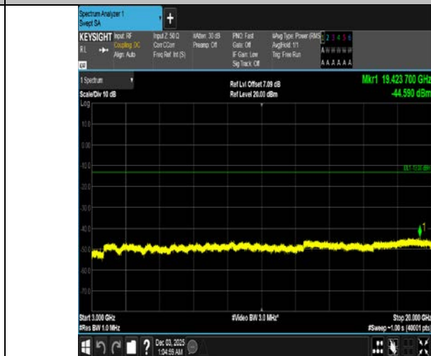
Band4-5MHz-16QAM-19975-25RB#0-3000~20000-PASS
