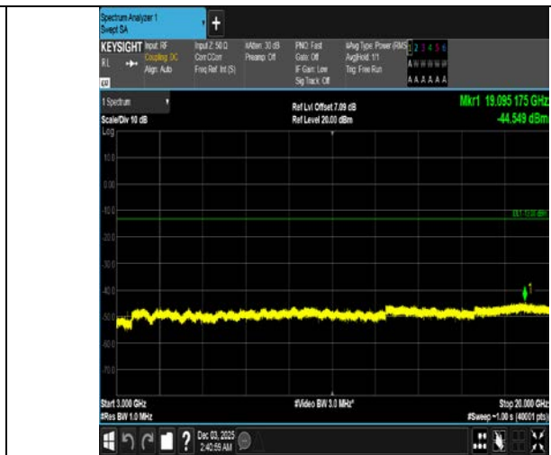
Band4-15MHz-QPSK-20025-1RB#74-3000~20000-PASS
