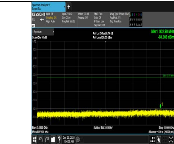
Band4-5MHz-16QAM-19975-25RB#0-30~1000-PASS
