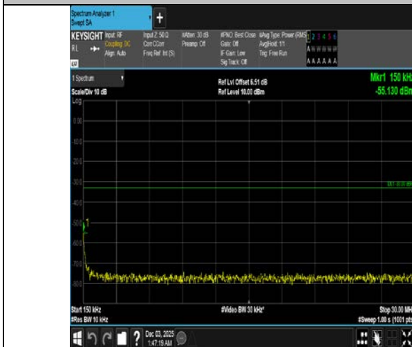
Band4-10MHz-16QAM-20000-1RB#0-0.15~30-PASS
