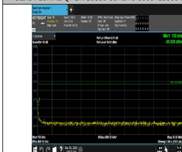
Band4-10MHz-16OAM-20350-1RB#0-0.15~30-PASS
