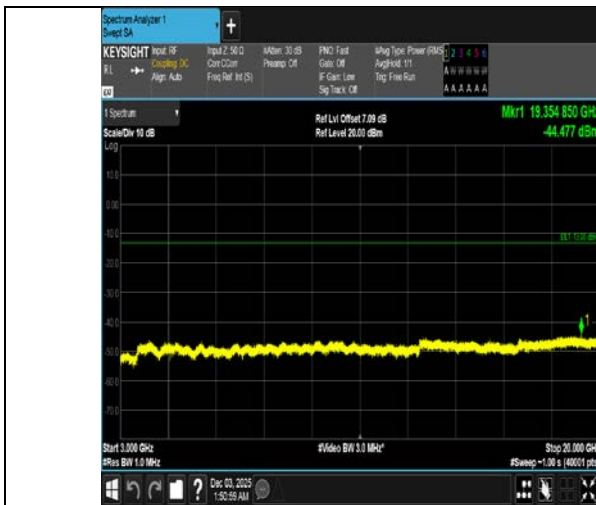
Band4-10MHz-QPSK-20000-50RB#0-3000~20000-PASS
