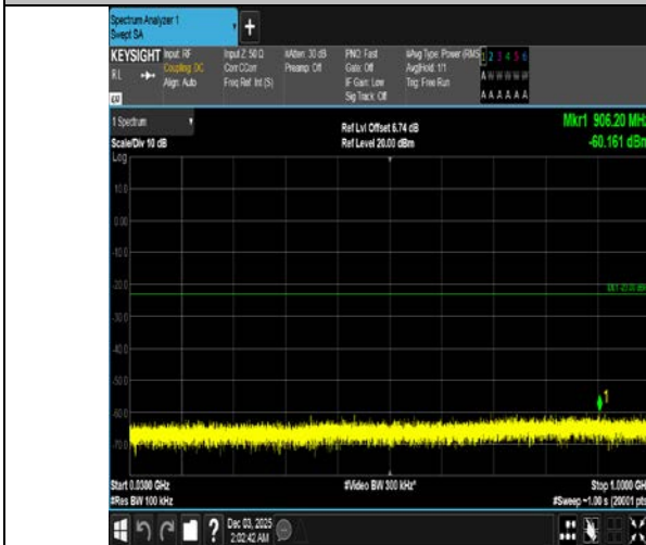
Band4-10MHz-QPSK-20350-50RB#0-30~1000-PASS
