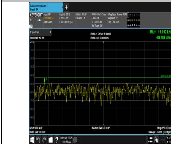
Band4-5MHz-QPSK-20375-25RB#0-0.009~0.15-PASS
