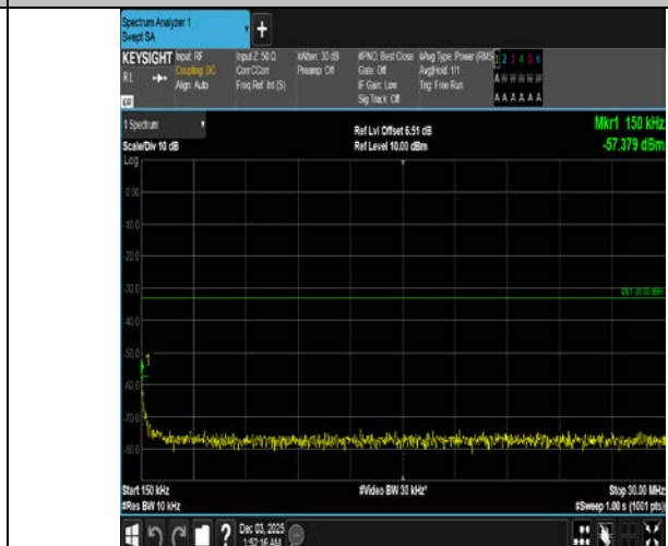
Band4-10MHz-QPSK-20175-1RB#0-0.15~30-PASS
