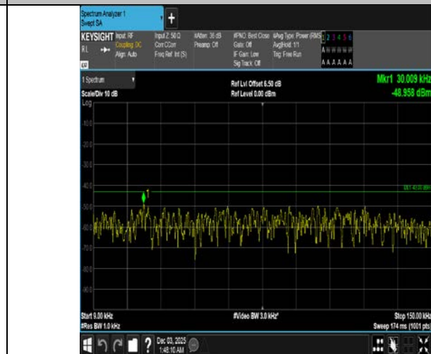
Band4-10MHz-QPSK-20000-1RB#49-0.009~0.15-PASS
