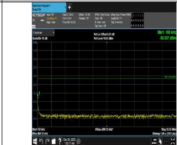
Band4-10MHz-QPSK-20000-50RB#0-0.15~30-PASS
