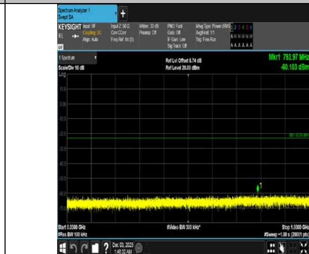
Band4-10MHz-QPSK-20000-1RB#49-30~1000-PASS
