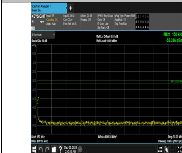
Band4-15MHz-QPSK-20025-1RB#74-0.15~30-PASS
