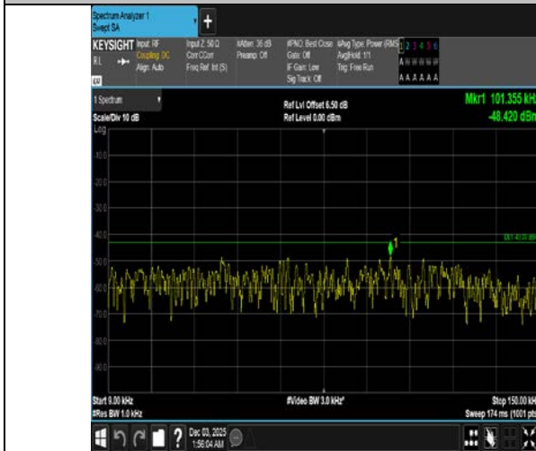
Band4-10MHz-QPSK-20175-50RB#0-0.009~0.15-PASS
