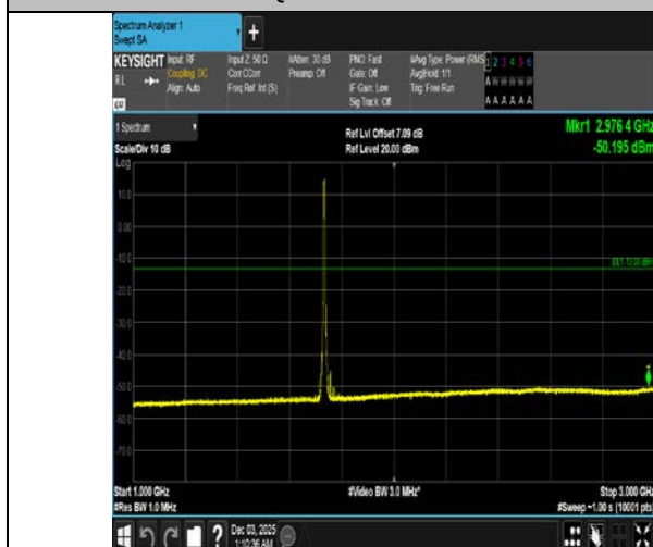
Band4-5MHz-16QAM-20175-25RB#0-1000~3000-PASS
