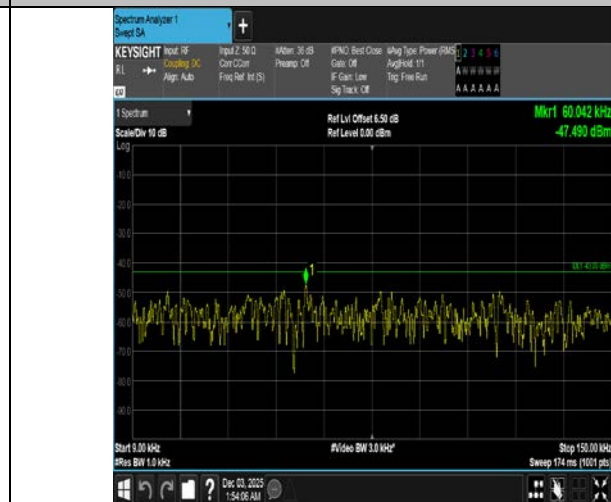
Band4-10MHz-QPSK-20175-1RB#49-0.009~0.15-PASS
