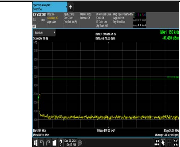
Band4-5MHz-QPSK-20175-25RB#0-0.15~30-PASS
