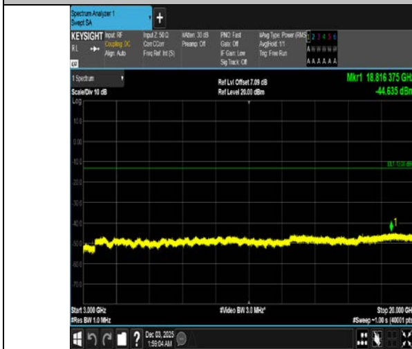
Band4-10MHz-QPSK-20350-1RB#0-3000~20000-PASS
