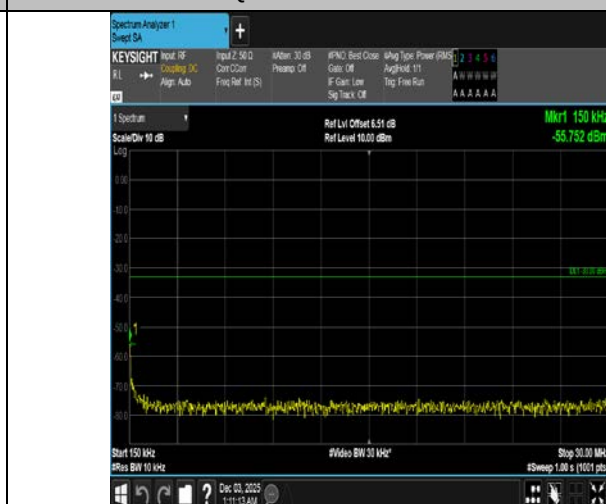
Band4-5MHz-QPSK-20375-1RB#0-0.15~30-PASS
