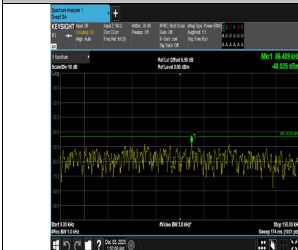
Band4-10MHz-QPSK-20175-1RB#0-0.009~0.15-PASS
