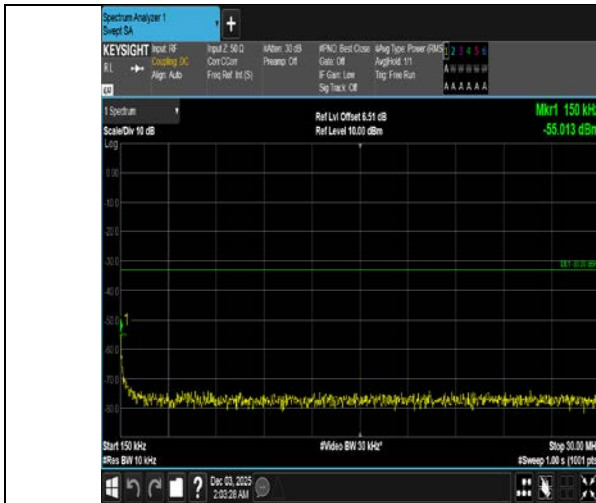
Band4-10MHz-16QAM-20350-50RB#0-0.15~30-PASS
