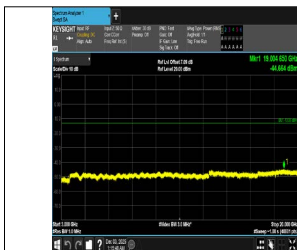
Band4-5MHz-OPSK-20375-25RB#0-3000~20000-PASS
