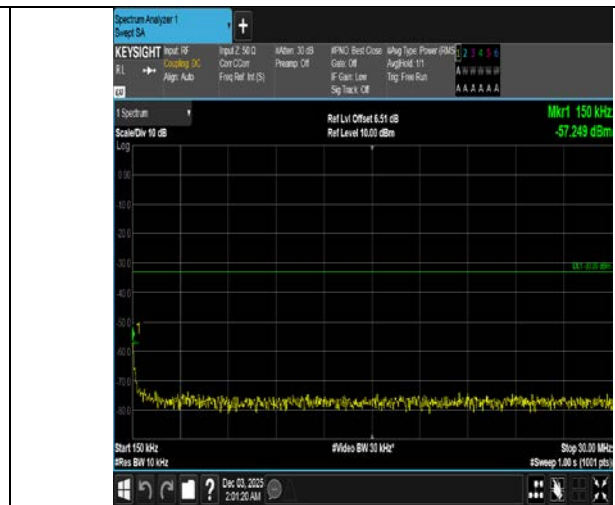
Band4-10MHz-16QAM-20350-1RB#49-0.15~30-PASS
