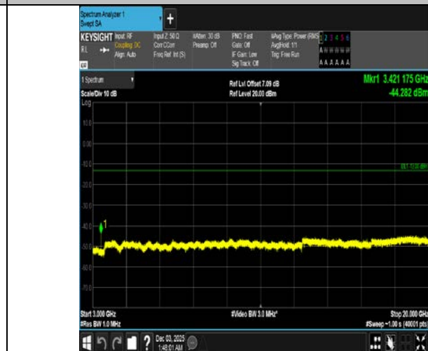
Band4-10MHz-16QAM-20000-1RB#0-3000~20000-PASS
