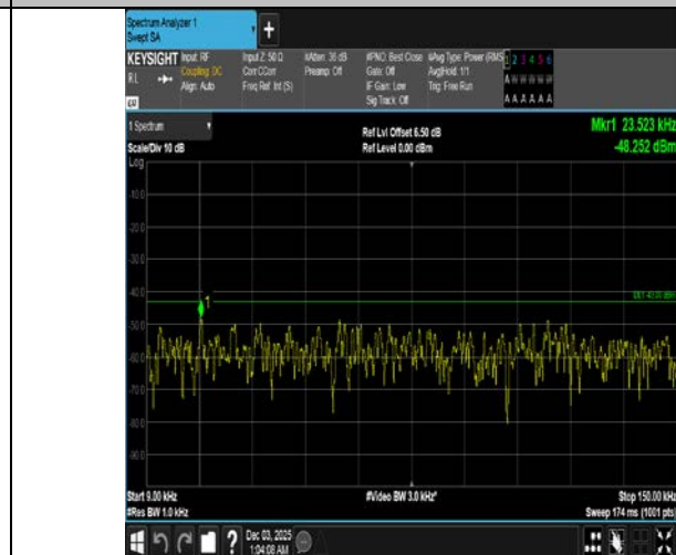
Band4-5MHz-16QAM-19975-25RB#0-0.009-0.15-PASS
