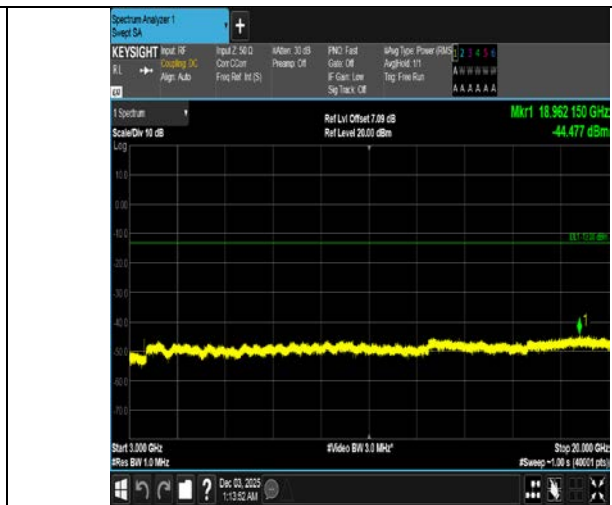
Band4-5MHz-QPSK-20375-1RB#24-3000~20000-PASS
