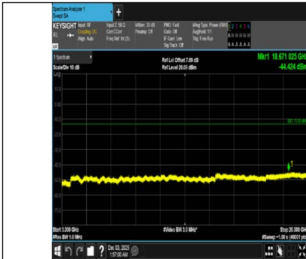
Band4-10MHz-QPSK-20175-50RB#0-3000~20000-PASS
