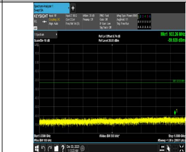
Band4-5MHz-QPSK-20375-1RB#24-30~1000-PASS
