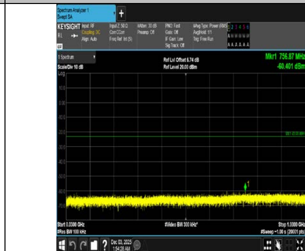
Band4-10MHz-QPSK-20175-1RB#49-30~1000-PASS
