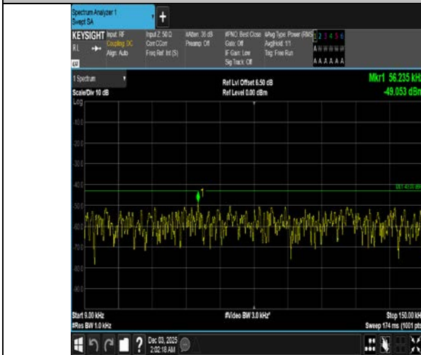
Band4-10MHz-QPSK-20350-50RB#0-0.009~0.15-PASS
