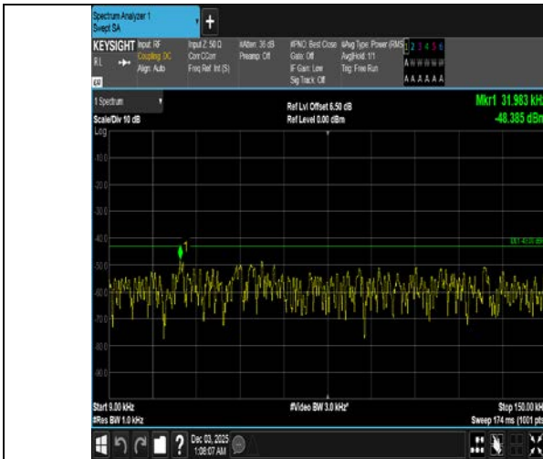
Band4-5MHz-16QAM-20175-1RB#24-0.009~0.15-PASS
