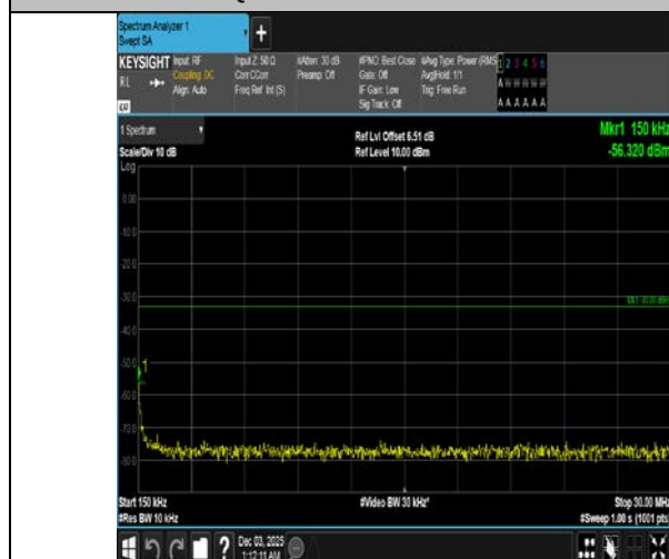
Band4-5MHz-16OAM-20375-1RB#0-0.15~30-PASS
