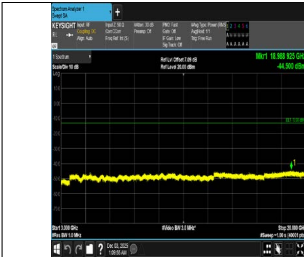
Band4-5MHz-QPSK-20175-25RB#0-3000~20000-PASS
