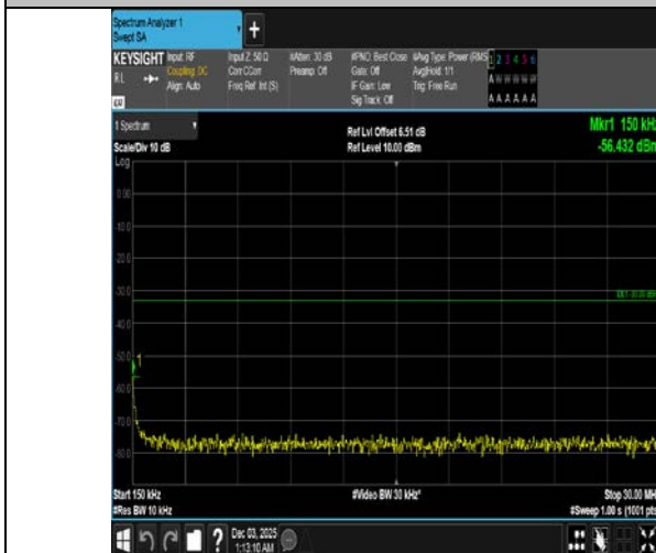
Band4-5MHz-QPSK-20375-1RB#24-0.15~30-PASS
