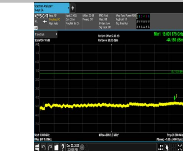
Band4-15MHz-16QAM-20025-1RB#0-3000~20000-PASS
