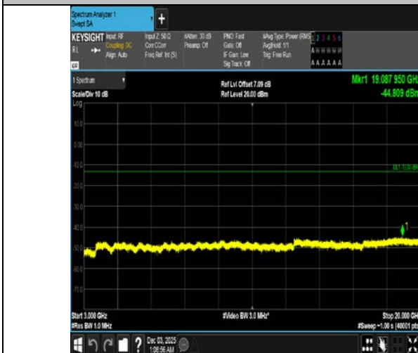
Band4-5MHz-16QAM-20175-1RB#24-3000~20000-PASS
