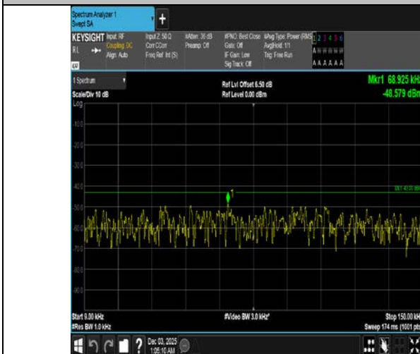
Band4-5MHz-QPSK-20175-1RB#0-0.009~0.15-PASS
