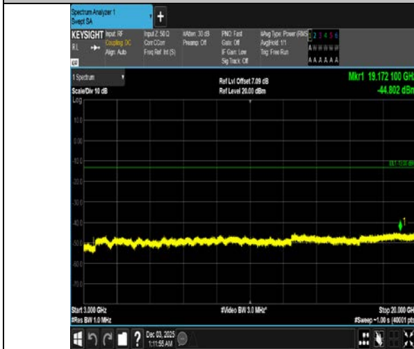
Band4-5MHz-QPSK-20375-1RB#0-3000~20000-PASS
