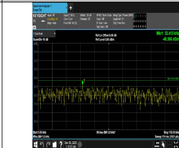
Band4-5MHz-16QAM-20375-25RB#0-0.009~0.15-PASS
