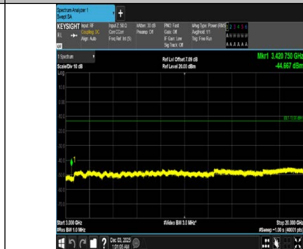
Band4-5MHz-16QAM-19975-1RB#0-3000~20000-PASS
