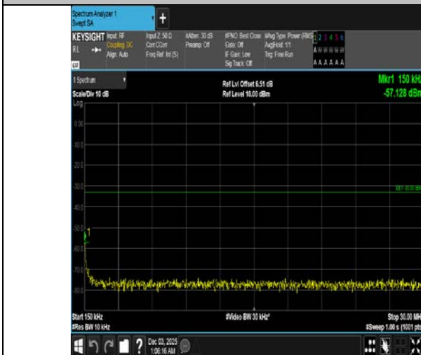
Band4-5MHz-16QAM-20175-1RB#0-0.15~30-PASS
