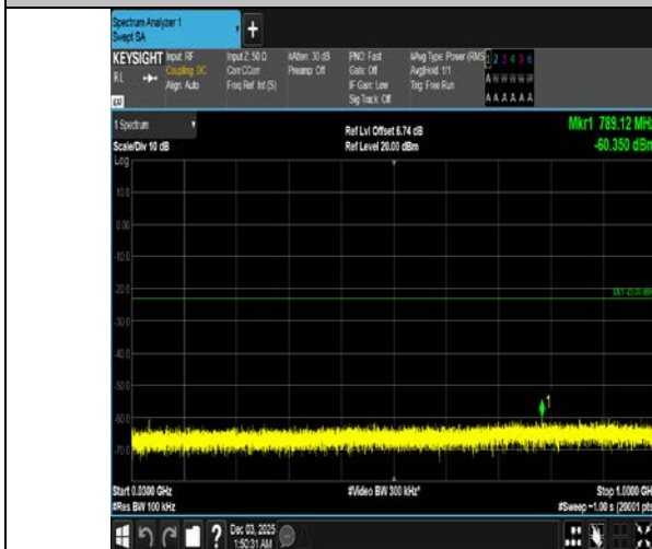
Band4-10MHz-QPSK-20000-50RB#0-30~1000-PASS
