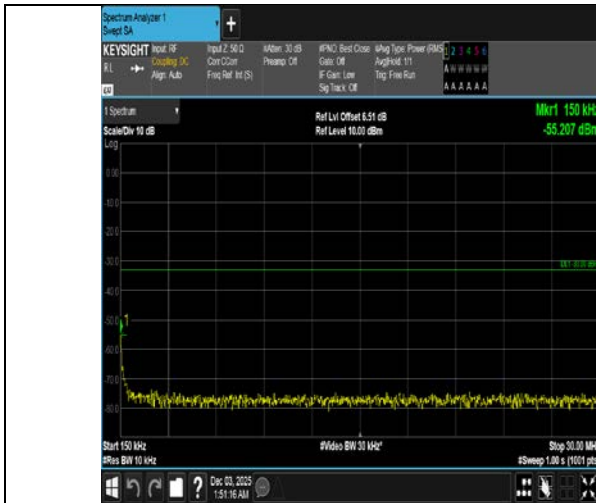
Band4-10MHz-16QAM-20000-50RB#0-0.15~30-PASS
