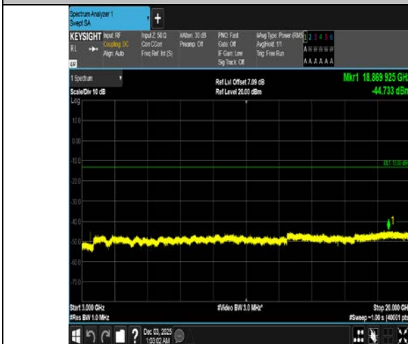
Band4-5MHz-16QAM-19975-1RB#24-3000-20000-PASS
