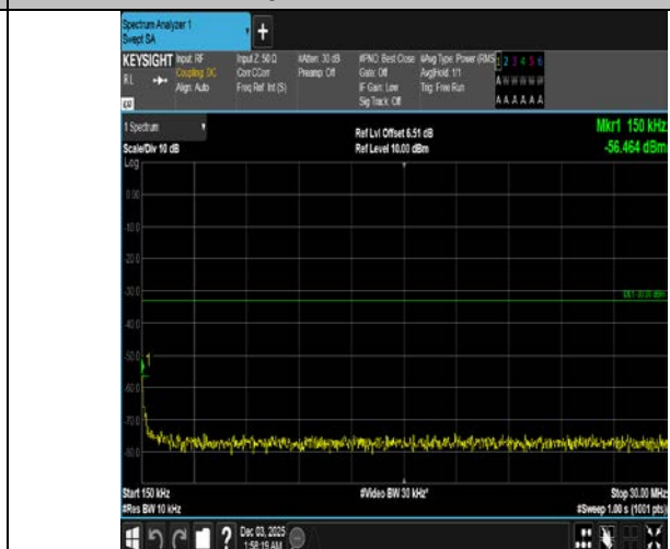
Band4-10MHz-QPSK-20350-1RB#0-0.15~30-PASS
