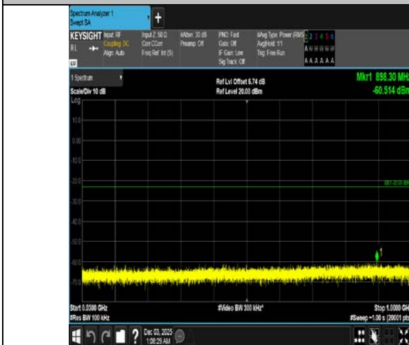
Band4-5MHz-16QAM-20175-1RB#24-30~1000-PASS
