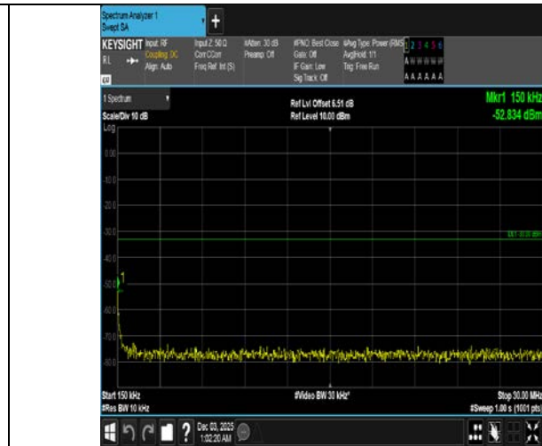
Band4-5MHz-16QAM-19975-1RB#24-0.15-30-PASS
