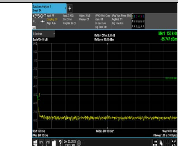
Band4-15MHz-QPSK-20025-1RB#0-0.15~30-PASS
