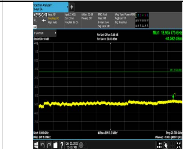
Band4-10MHz-16QAM-20000-50RB#0-3000~20000-PASS
