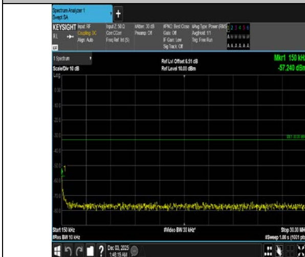
Band4-10MHz-QPSK-20000-1RB#49-0.15~30-PASS
