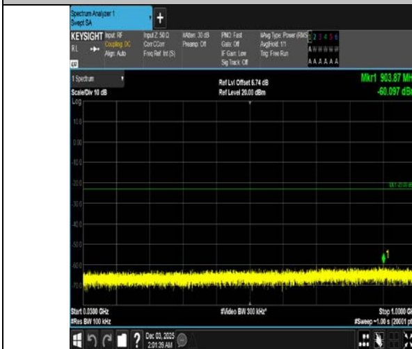
Band4-10MHz-16QAM-20350-1RB#49-30~1000-PASS
