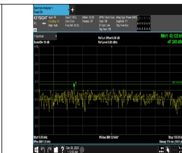
Band4-5MHz-16OAM-20375-1RB#0-0.009~0.15-PASS
