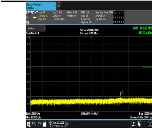
Band4-5MHz-16QAM-19975-1RB#24-30-1000-PASS
