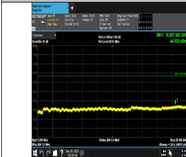
Band4-10MHz-QPSK-20175-1RB#0-3000~20000-PASS
