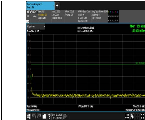
Band4-5MHz-16QAM-20375-1RB#24-0.15~30-PASS
