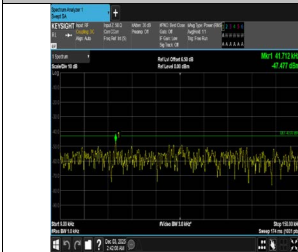
Band4-15MHz-QPSK-20025-75RB#0-0.009~0.15-PASS
