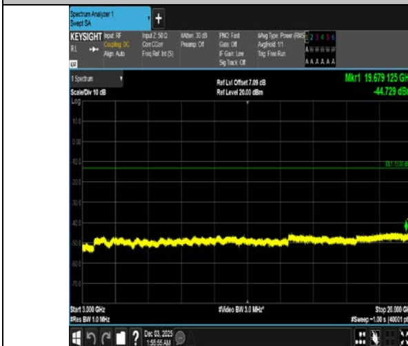
Band4-10MHz-16QAM-20175-1RB#49-3000~20000-PASS
