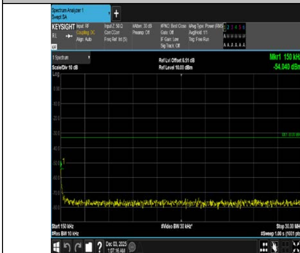
Band4-5MHz-QPSK-20175-1RB#24-0.15~30-PASS
