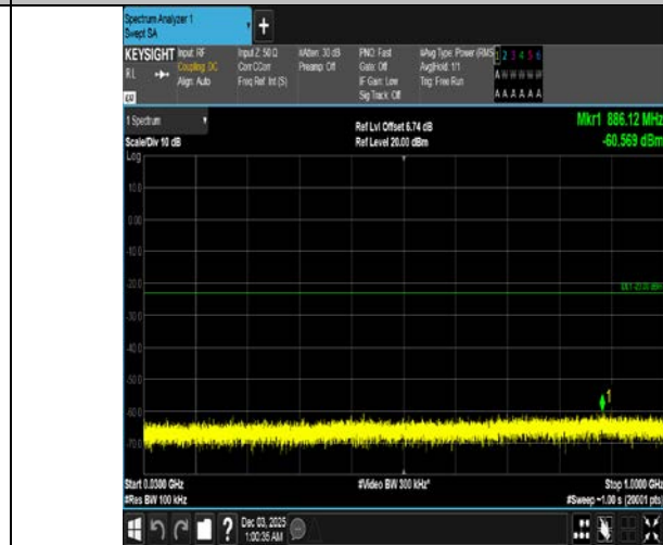
Band4-5MHz-16QAM-19975-1RB#0-30~1000-PASS
