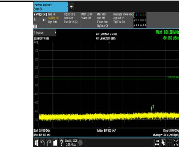
Band4-15MHz-16QAM-20025-1RB#0-30~1000-PASS
