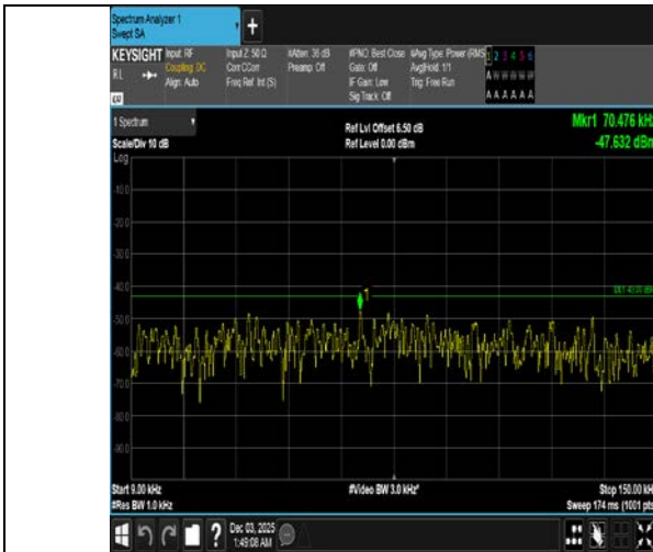
Band4-10MHz-16QAM-20000-1RB#49-0.009~0.15-PASS
