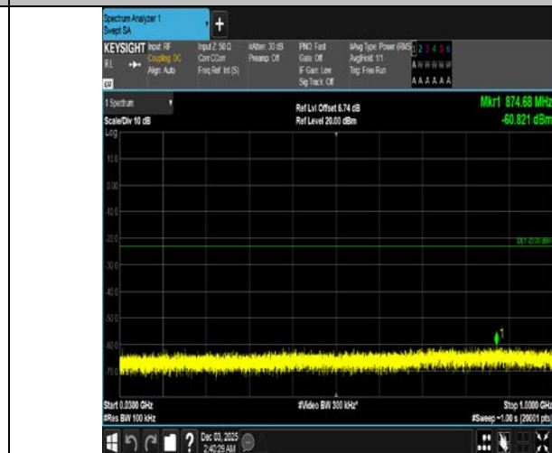
Band4-15MHz-QPSK-20025-1RB#74-30~1000-PASS
