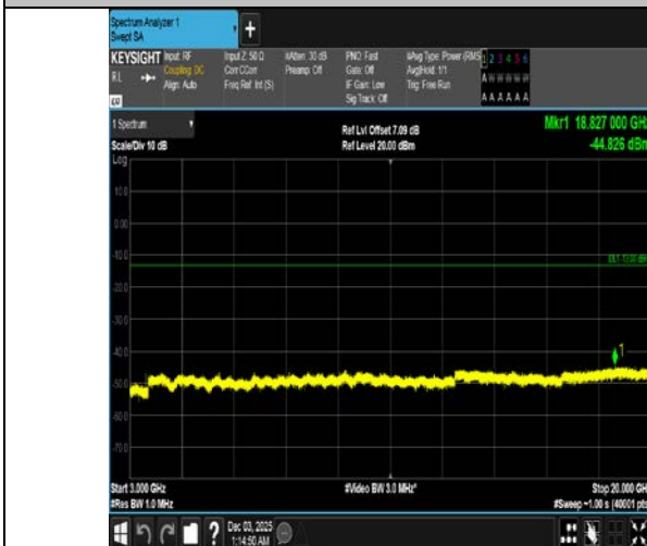
Band4-5MHz-16QAM-20375-1RB#24-3000~20000-PASS
