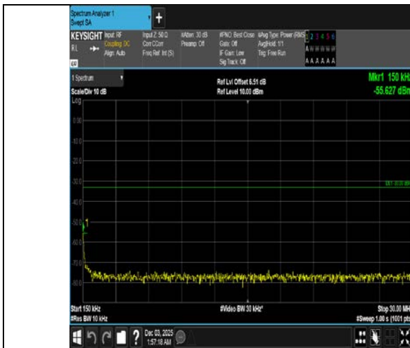
Band4-10MHz-16QAM-20175-50RB#0-0.15~30-PASS
