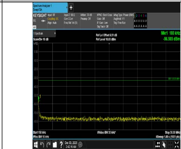
Band4-15MHz-QPSK-20025-75RB#0-0.15~30-PASS
