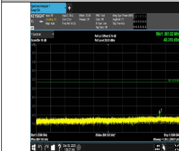
Band4-5MHz-QPSK-20175-25RB#0-30~1000-PASS
