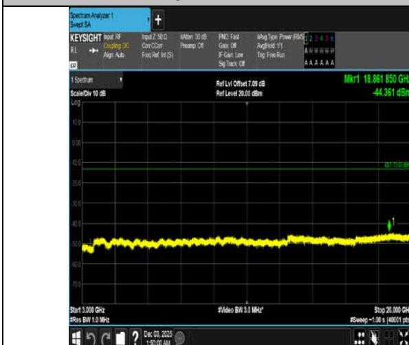
Band4-10MHz-16QAM-20000-1RB#49-3000~20000-PASS
