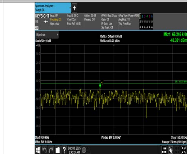
Band4-15MHz-QPSK-20025-1RB#74-0.009~0.15-PASS
