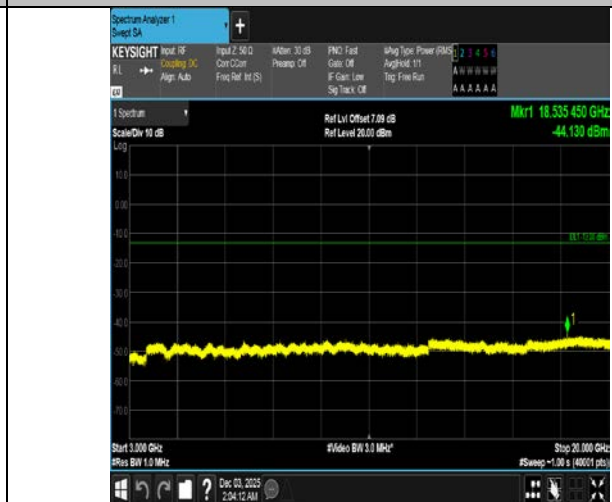
Band4-10MHz-16QAM-20350-50RB#0-3000~20000-PASS
