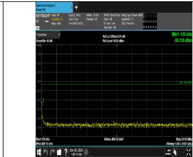
Band4-10MHz-16QAM-20175-1RB#49-0.15~30-PASS
