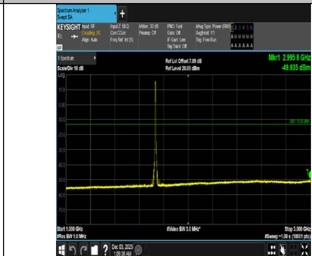
Band4-5MHz-QPSK-20175-25RB#0-1000~3000-PASS
