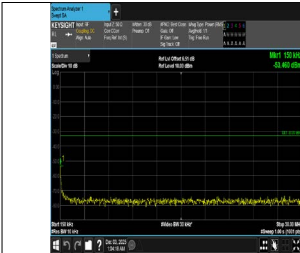
Band4-5MHz-16QAM-19975-25RB#0-0.15~30-PASS
