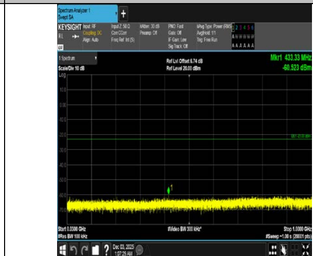
Band4-5MHz-QPSK-20175-1RB#24-30~1000-PASS
