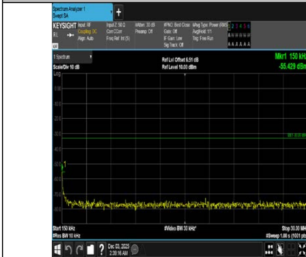
Band4-15MHz-16QAM-20025-1RB#0-0.15~30-PASS
