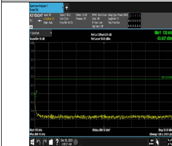
Band4-10MHz-QPSK-20350-1RB#49-0.15~30-PASS
