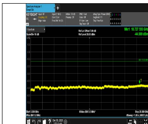
Band4-10MHz-OPSK-20350-50RB#0-3000~20000-PASS
