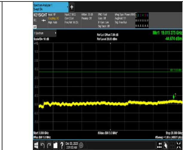
Band4-10MHz-QPSK-20350-1RB#49-3000~20000-PASS
