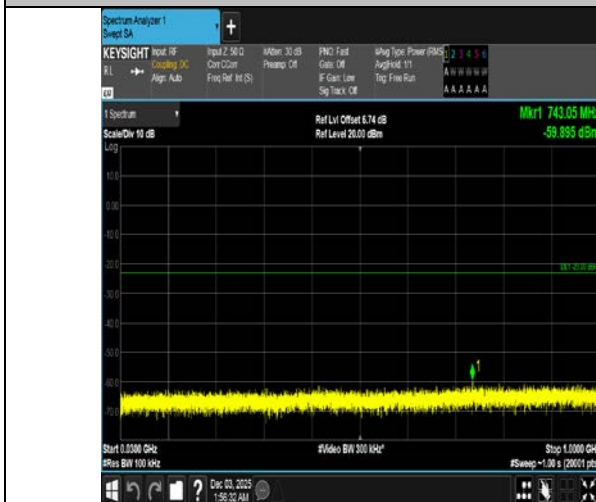
Band4-10MHz-QPSK-20175-50RB#0-30~1000-PASS
