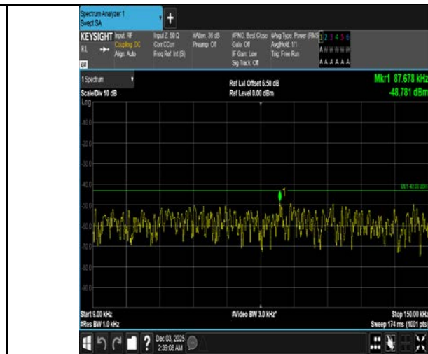
Band4-15MHz-16QAM-20025-1RB#0-0.009~0.15-PASS
