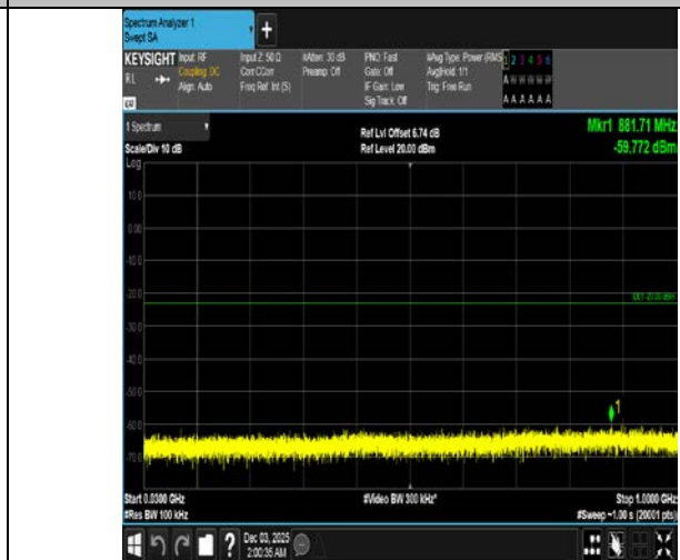
Band4-10MHz-QPSK-20350-1RB#49-30~1000-PASS
