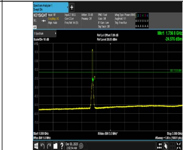
Band4-10MHz-QPSK-20350-50RB#0-1000~3000-PASS
