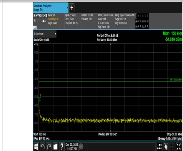
Band4-5MHz-QPSK-20375-25RB#0-0.15~30-PASS
