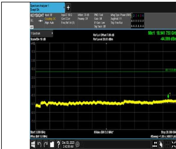
Band4-15MHz-QPSK-20025-75RB#0-3000~20000-PASS
