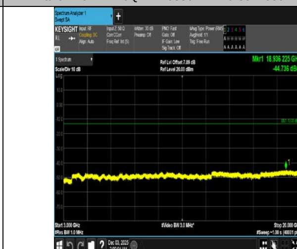
Band4-10MHz-16OAM-20350-1RB#0-3000~20000-PASS
