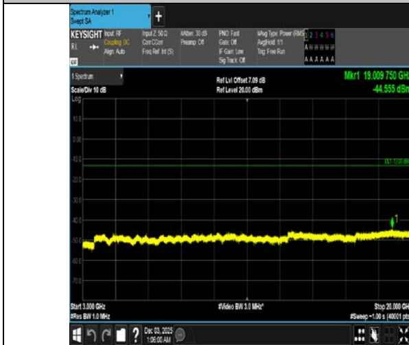
Band4-5MHz-QPSK-20175-1RB#0-3000~20000-PASS
