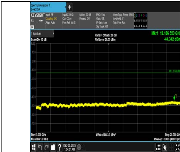
Band4-5MHz-QPSK-19975-25RB#0-3000~20000-PASS
