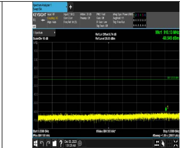
Band4-10MHz-16QAM-20000-50RB#0-30~1000-PASS
