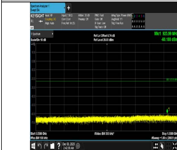
Band4-15MHz-QPSK-20025-75RB#0-30~1000-PASS
