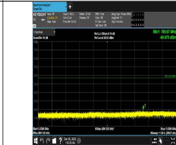
Band4-10MHz-16QAM-20175-1RB#0-30~1000-PASS
