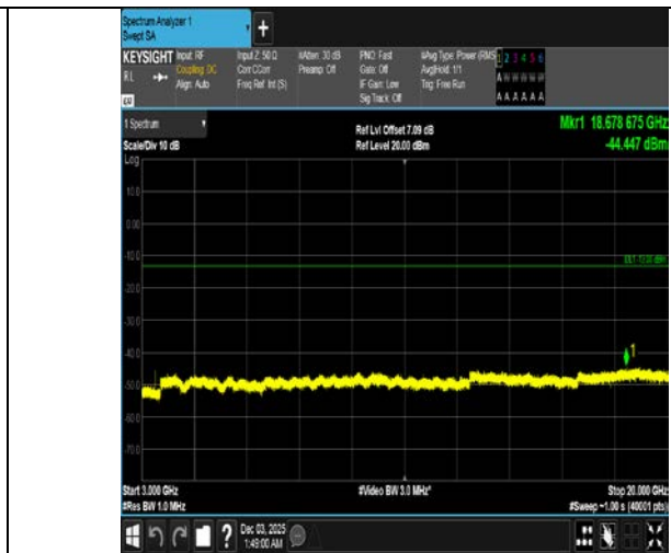
Band4-10MHz-QPSK-20000-1RB#49-3000~20000-PASS
