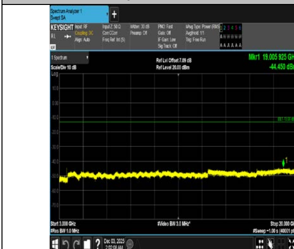
Band4-10MHz-16QAM-20350-1RB#49-3000~20000-PASS
