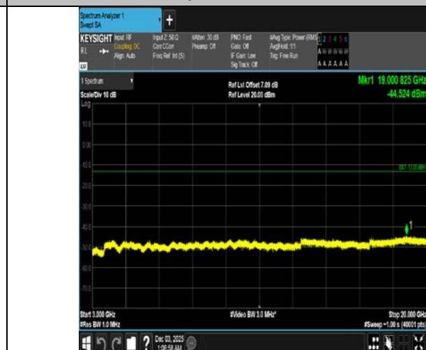
Band4-5MHz-16QAM-20175-1RB#0-3000~20000-PASS
