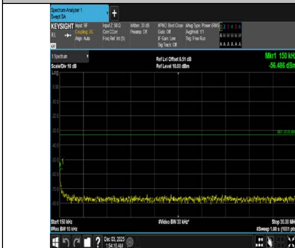
Band4-10MHz-QPSK-20175-1RB#49-0.15~30-PASS
