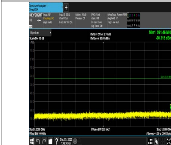
Band4-10MHz-16QAM-20000-1RB#49-30~1000-PASS
