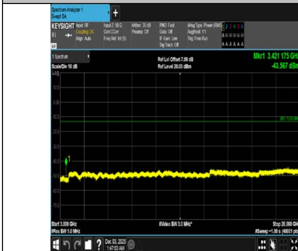
Band4-10MHz-QPSK-20000-1RB#0-3000~20000-PASS
