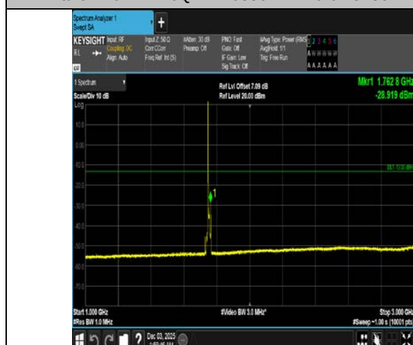
Band4-10MHz-16OAM-20350-1RB#0-1000~3000-PASS
