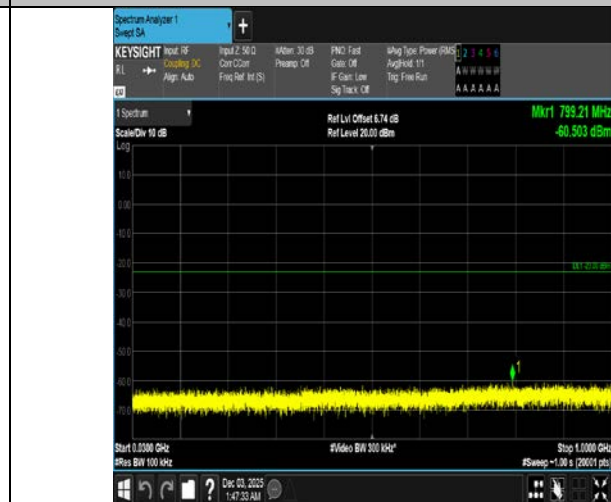
Band4-10MHz-16QAM-20000-1RB#0-30~1000-PASS
