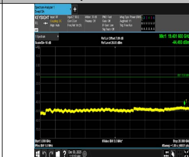
Band4-5MHz-16QAM-20175-25RB#0-3000~20000-PASS
