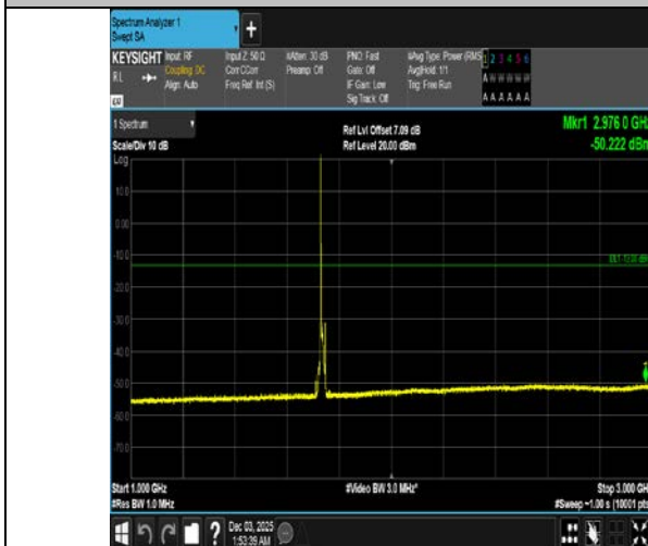
Band4-10MHz-16QAM-20175-1RB#0-1000~3000-PASS
