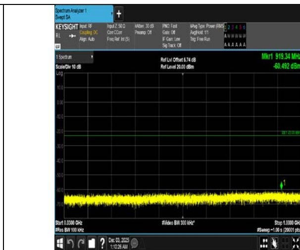
Band4-5MHz-16QAM-20175-25RB#0-30~1000-PASS
