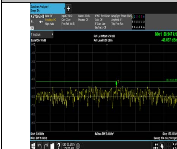
Band4-10MHz-QPSK-20350-1RB#0-0.009~0.15-PASS
