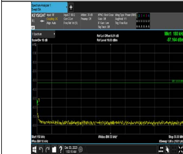
Band4-10MHz-16QAM-20175-1RB#0-0.15~30-PASS
