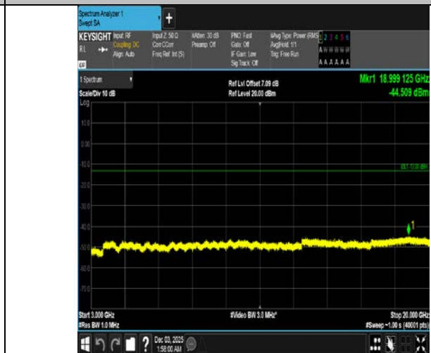
Band4-10MHz-16QAM-20175-50RB#0-3000~20000-PASS
