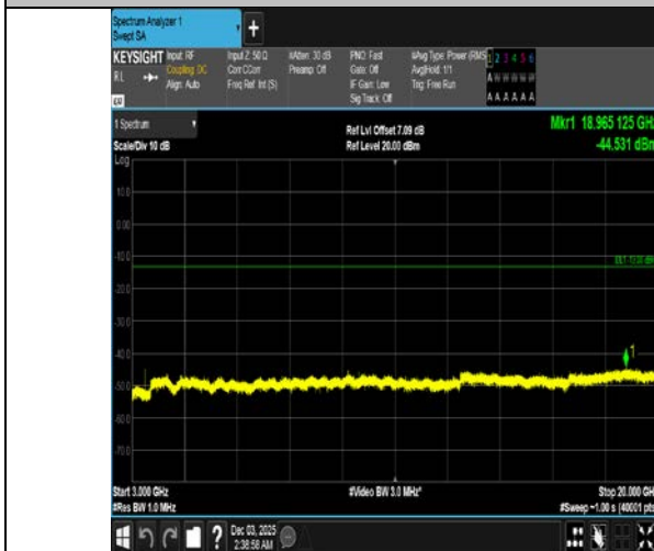
Band4-15MHz-QPSK-20025-1RB#0-3000~20000-PASS
