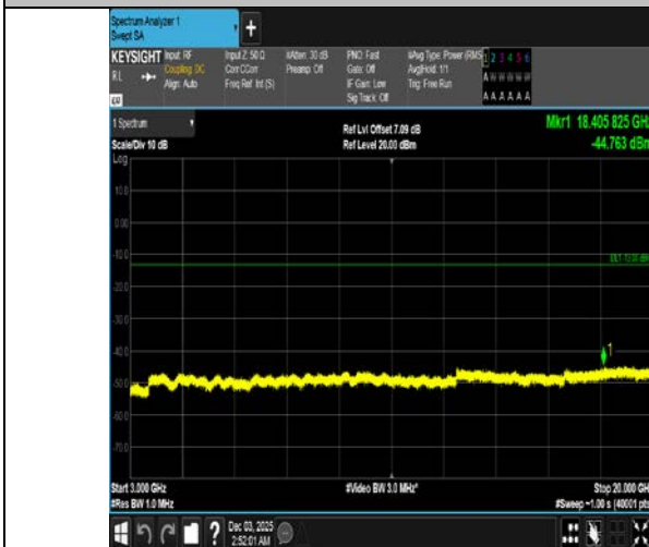
Band4-15MHz-QPSK-20325-1RB#0-3000~20000-PASS
