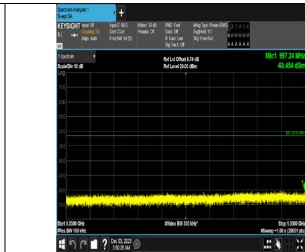
Band4-20MHz-16QAM-20175-100RB#0-30~1000-PASS
