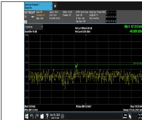
Band4-15MHz-16QAM-20325-1RB#74-0.009~0.15-PASS
