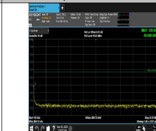
Band4-20MHz-QPSK-20050-1RB#0-0.15~30-PASS
