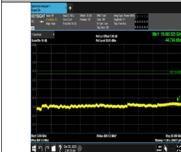
Band4-15MHz-16QAM-20175-1RB#74-3000~20000-PASS
