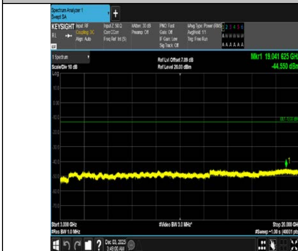
Band4-20MHz-16QAM-20175-1RB#99-3000~20000-PASS
