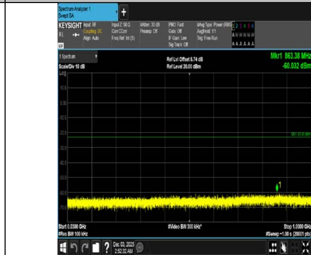
Band4-15MHz-16QAM-20325-1RB#0-30~1000-PASS
