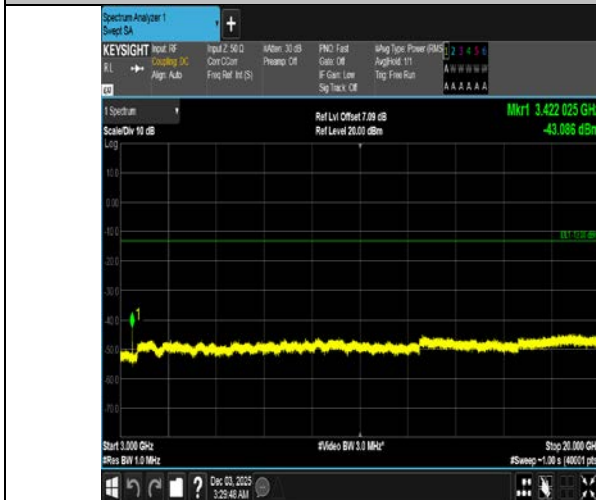
Band4-20MHz-QPSK-20050-1RB#0-3000~20000-PASS
