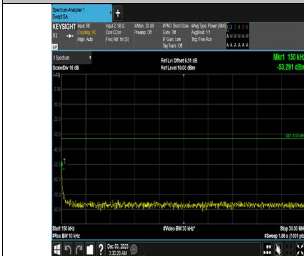
Band4-20MHz-16QAM-20050-1RB#0-0.15~30-PASS
