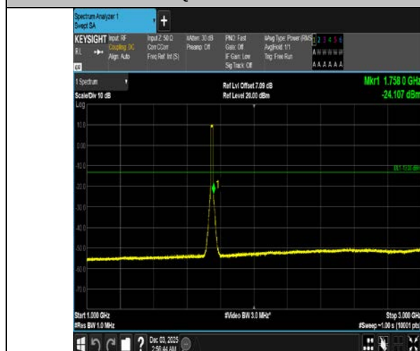
Band4-15MHz-16QAM-20325-75RB#0-1000~3000-PASS
