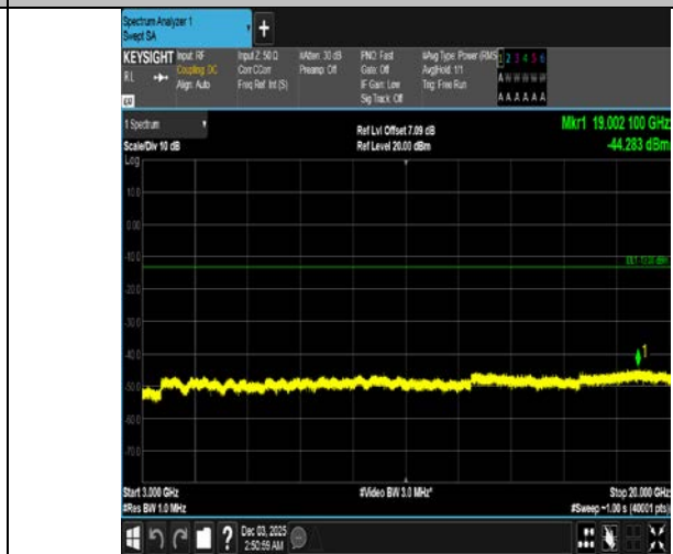
Band4-15MHz-16QAM-20175-75RB#0-3000~20000-PASS
