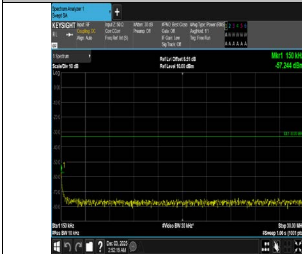
Band4-15MHz-16QAM-20325-1RB#0-0.15~30-PASS
