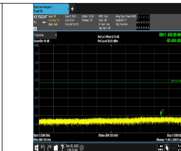
Band4-15MHz-16QAM-20325-75RB#0-30~1000-PASS
