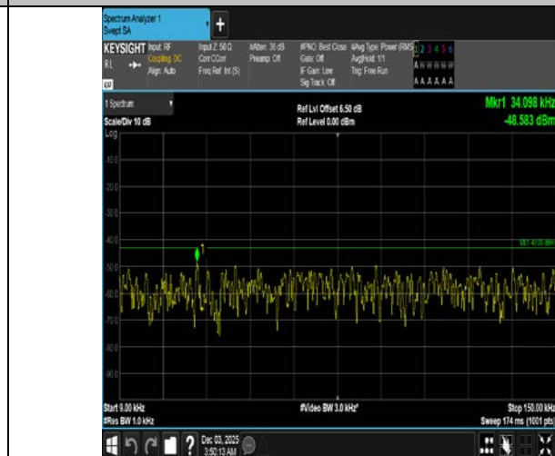
Band4-20MHz-16QAM-20175-100RB#0-0.009~0.15-PASS
