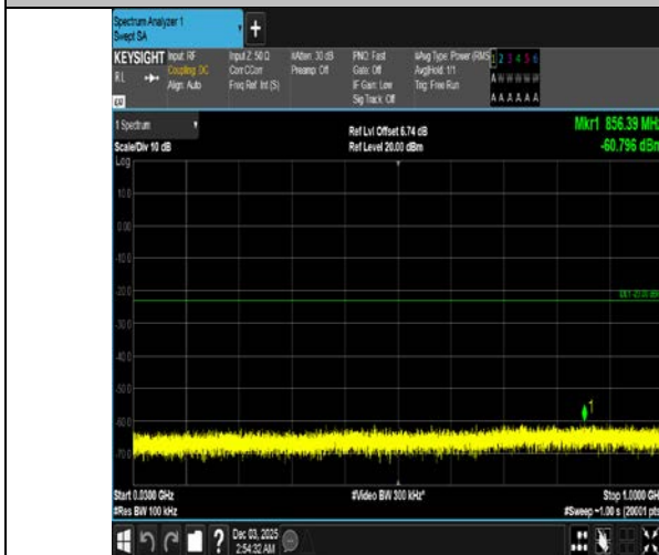
Band4-15MHz-16QAM-20325-1RB#74-30~1000-PASS
