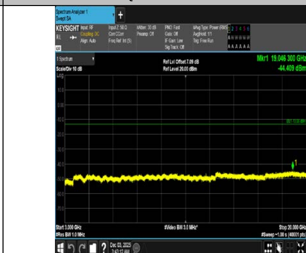
Band4-20MHz-16OAM-20050-100RB#0-3000~20000-PASS
