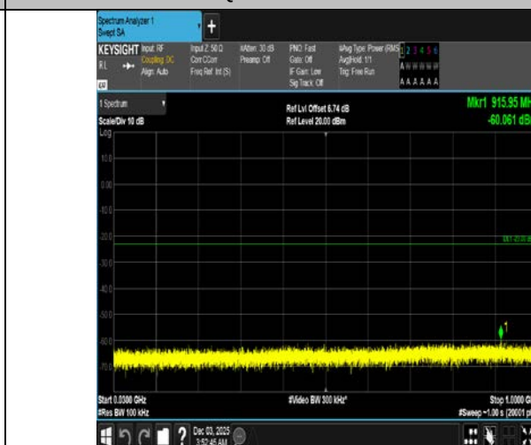
Band4-20MHz-16OAM-20300-1RB#0-30~1000-PASS
