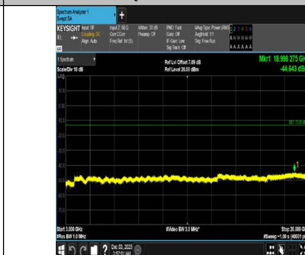
Band4-15MHz-16QAM-20325-75RB#0-3000~20000-PASS
