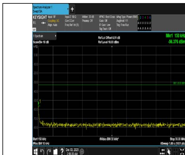
Band4-15MHz-16QAM-20325-75RB#0-0.15~30-PASS
