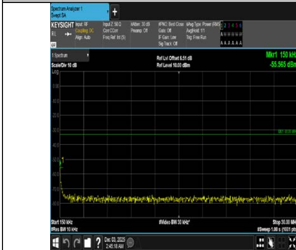
Band4-15MHz-16QAM-20175-1RB#0-0.15~30-PASS
