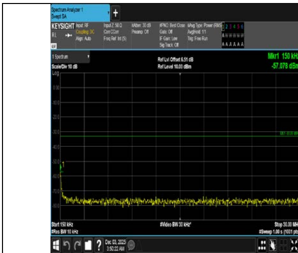
Band4-20MHz-16QAM-20175-100RB#0-0.15~30-PASS
