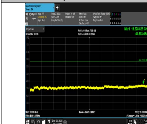
Band4-20MHz-16QAM-20300-1RB#99-3000~20000-PASS
