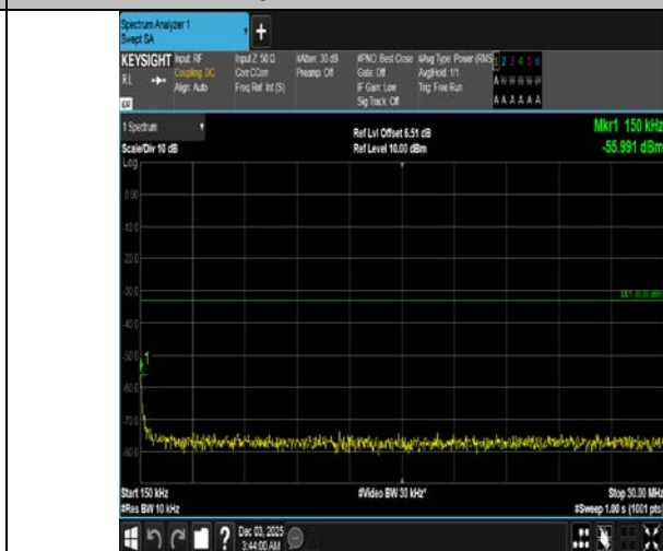
Band4-20MHz-QPSK-20175-1RB#0-0.15~30-PASS
