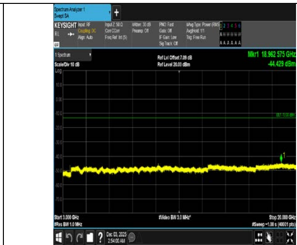
Band4-15MHz-QPSK-20325-1RB#74-3000~20000-PASS
