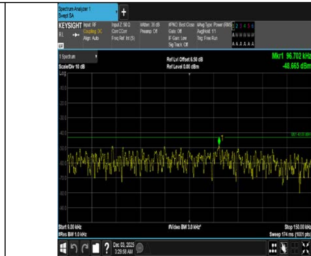
Band4-20MHz-16QAM-20050-1RB#0-0.009~0.15-PASS
