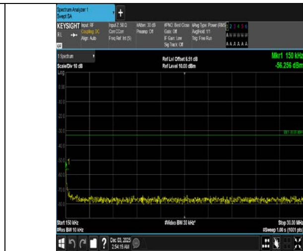
Band4-15MHz-16QAM-20325-1RB#74-0.15~30-PASS
