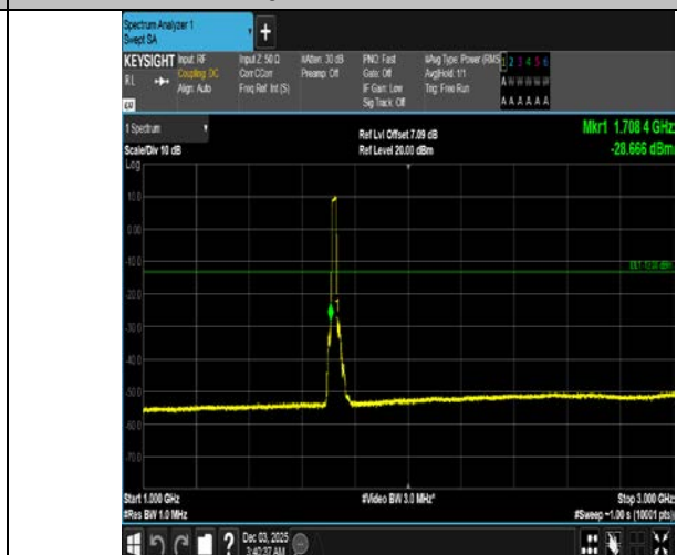
Band4-20MHz-QPSK-20050-100RB#0-1000~3000-PASS
