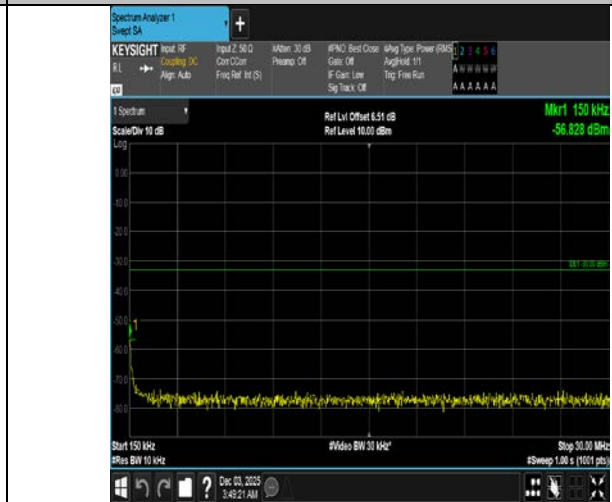
Band4-20MHz-QPSK-20175-100RB#0-0.15~30-PASS
