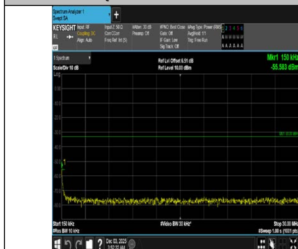
Band4-20MHz-16OAM-20300-1RB#0-0.15~30-PASS
