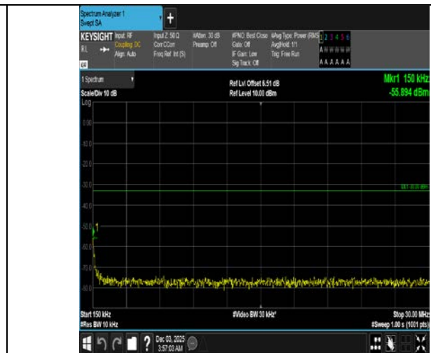
Band4-20MHz-16QAM-20300-1RB#99-0.15~30-PASS
