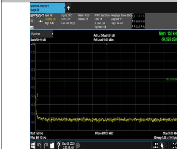
Band4-15MHz-QPSK-20325-1RB#74-0.15~30-PASS
