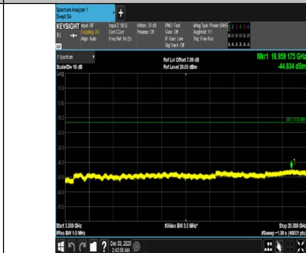
Band4-15MHz-16QAM-20025-75RB#0-3000~20000-PASS
