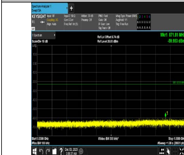
Band4-20MHz-QPSK-20300-100RB#0-30~1000-PASS
