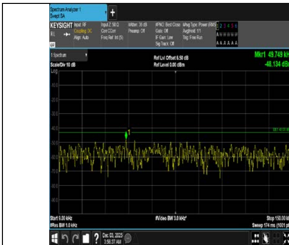
Band4-20MHz-16QAM-20300-1RB#99-0.009~0.15-PASS
