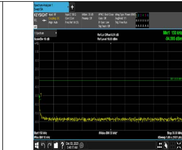
Band4-20MHz-16QAM-20175-1RB#99-0.15~30-PASS
