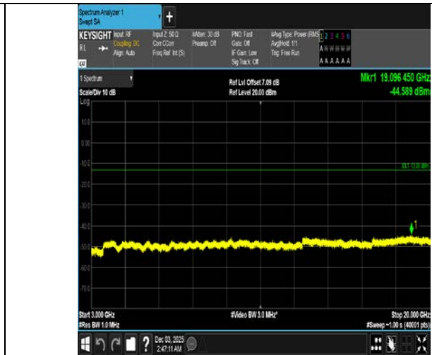
Band4-15MHz-QPSK-20175-1RB#74-3000~20000-PASS
