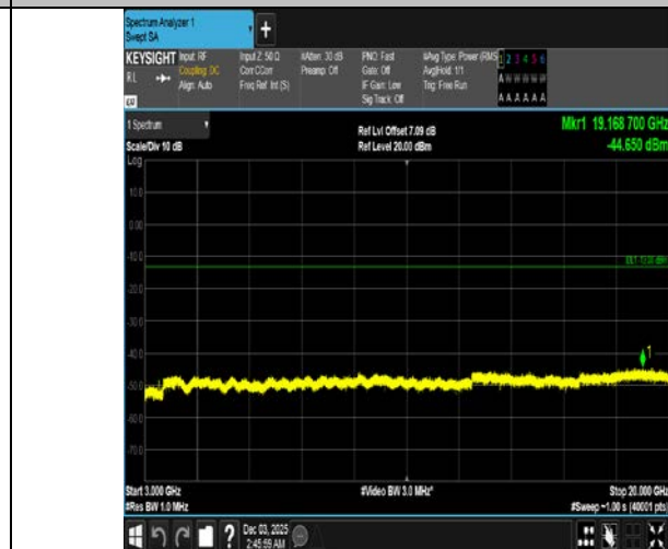
Band4-15MHz-16QAM-20175-1RB#0-3000~20000-PASS
