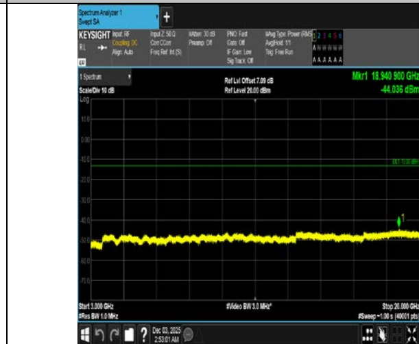
Band4-15MHz-16QAM-20325-1RB#0-3000~20000-PASS
