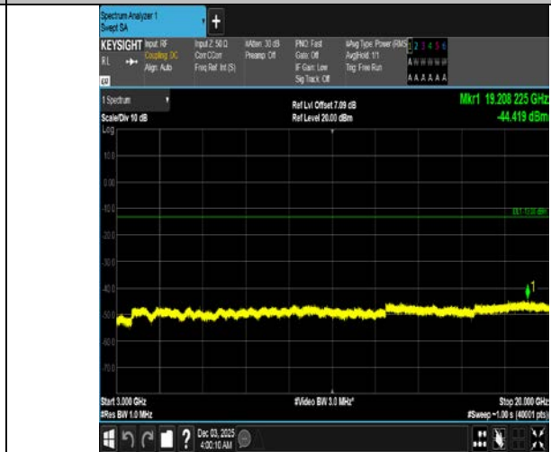
Band4-20MHz-16QAM-20300-100RB#0-3000~20000-PASS
