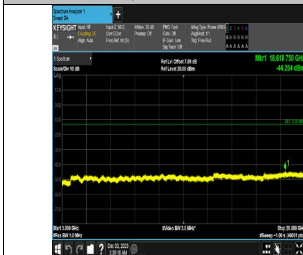
Band4-20MHz-16QAM-20050-1RB#99-3000~20000-PASS
