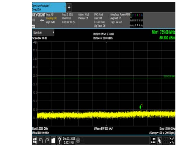
Band4-15MHz-16QAM-20175-75RB#0-30~1000-PASS
