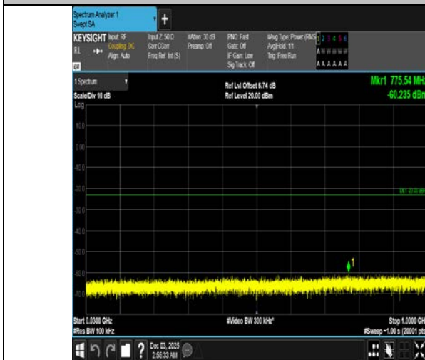
Band4-15MHz-QPSK-20325-75RB#0-30~1000-PASS
