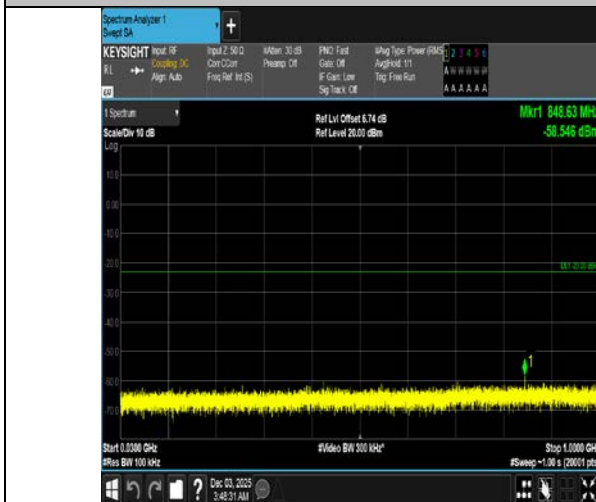
Band4-20MHz-16QAM-20175-1RB#99-30~1000-PASS
