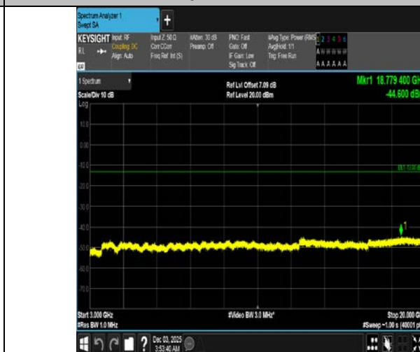
Band4-20MHz-16QAM-20300-1RB#0-3000~20000-PASS
