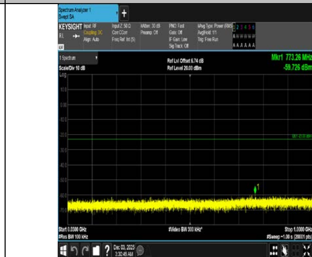
Band4-20MHz-16QAM-20050-1RB#0-30~1000-PASS
