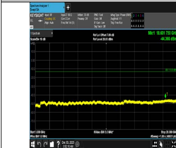
Band4-20MHz-QPSK-20300-1RB#0-3000~20000-PASS
