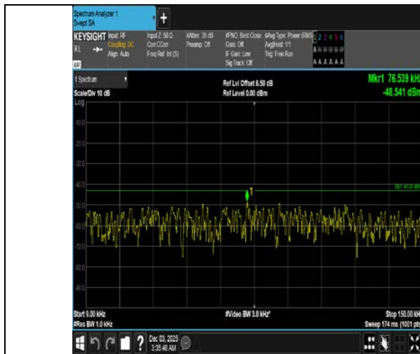
Band4-20MHz-16QAM-20050-1RB#99-0.009~0.15-PASS
