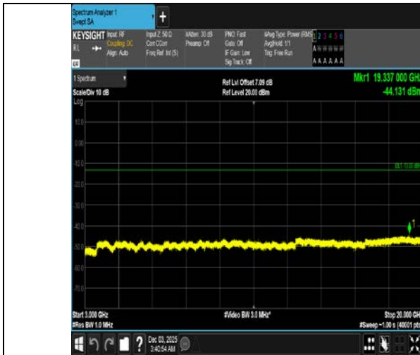
Band4-20MHz-QPSK-20050-100RB#0-3000~20000-PASS
