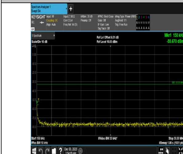
Band4-20MHz-QPSK-20300-1RB#99-0.15~30-PASS
