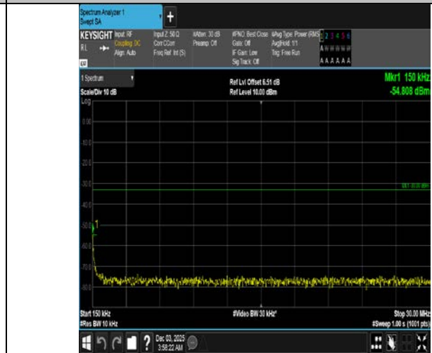
Band4-20MHz-QPSK-20300-100RB#0-0.15~30-PASS
