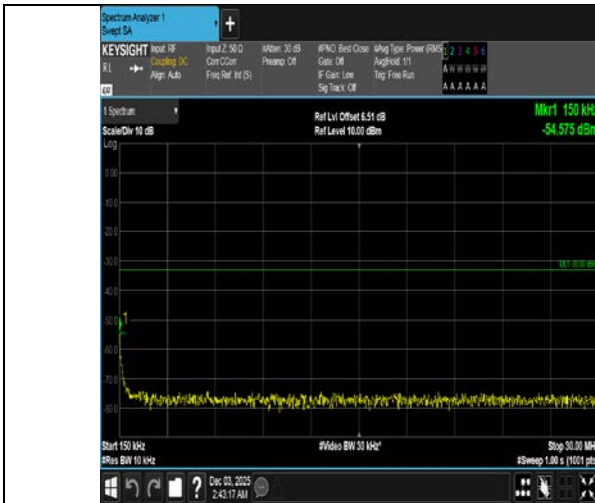
Band4-15MHz-16QAM-20025-75RB#0-0.15~30-PASS
