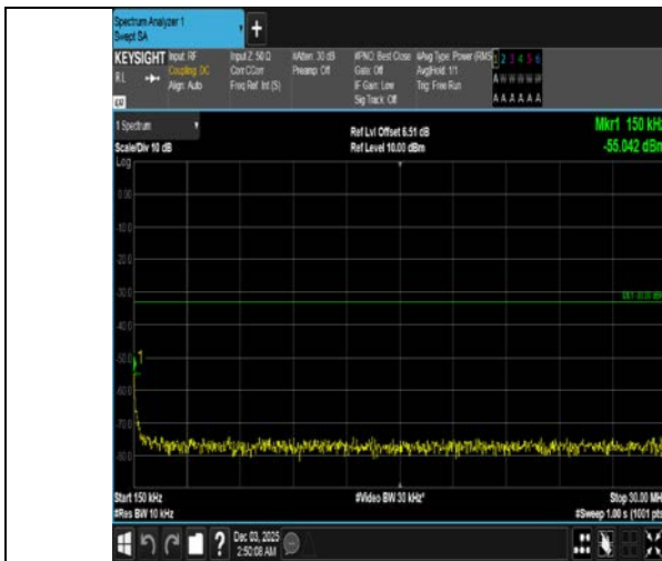
Band4-15MHz-16QAM-20175-75RB#0-0.15~30-PASS
