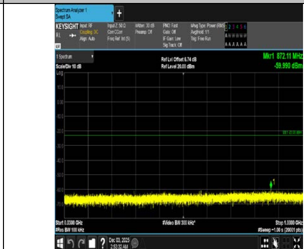
Band4-15MHz-QPSK-20325-1RB#74-30~1000-PASS
