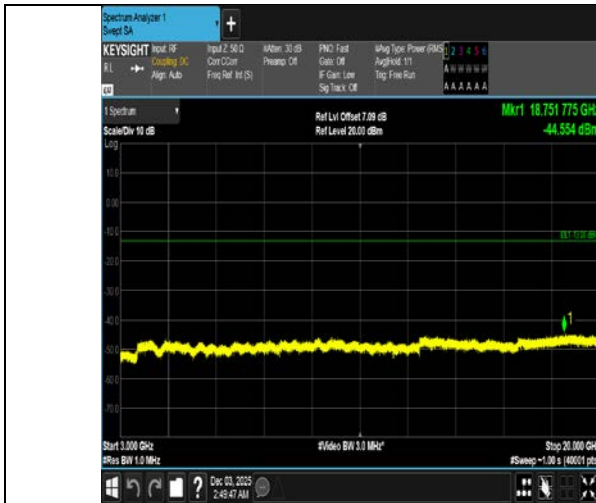
Band4-15MHz-QPSK-20175-75RB#0-3000~20000-PASS
