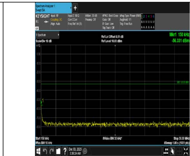
Band4-20MHz-16QAM-20050-1RB#99-0.15~30-PASS
