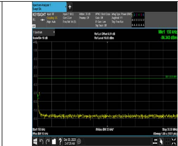
Band4-15MHz-16QAM-20175-1RB#74-0.15~30-PASS
