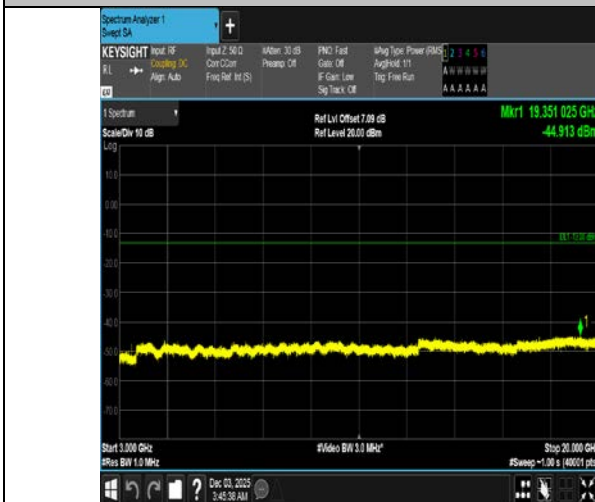
Band4-20MHz-QPSK-20175-1RB#0-3000~20000-PASS
