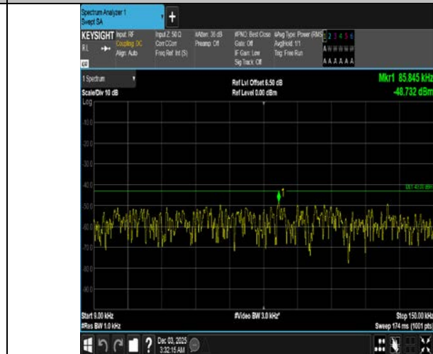
Band4-20MHz-QPSK-20050-1RB#99-0.009~0.15-PASS
