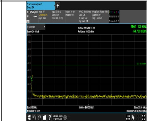
Band4-15MHz-QPSK-20175-75RB#0-0.15~30-PASS
