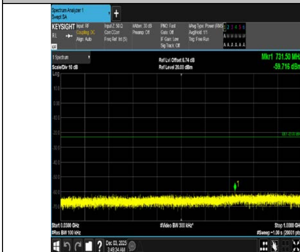
Band4-20MHz-QPSK-20175-100RB#0-30~1000-PASS
