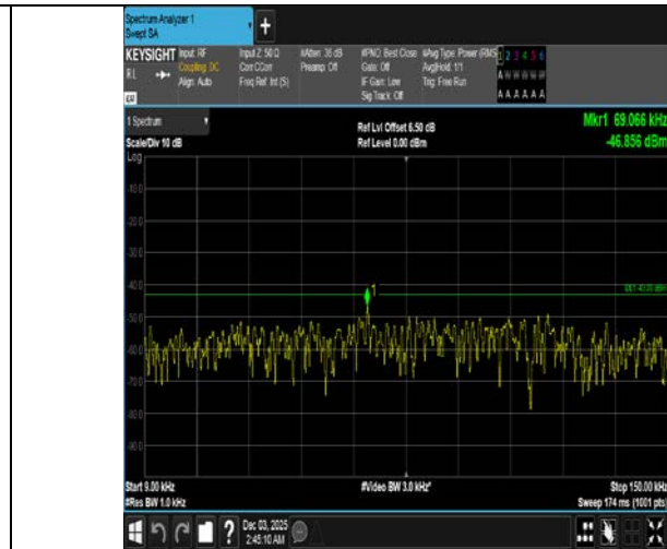
Band4-15MHz-16QAM-20175-1RB#0-0.009~0.15-PASS
