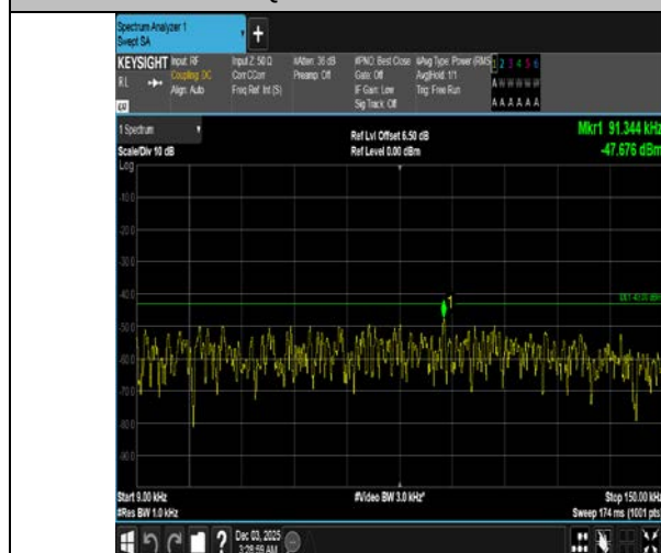
Band4-20MHz-QPSK-20050-1RB#0-0.009~0.15-PASS
