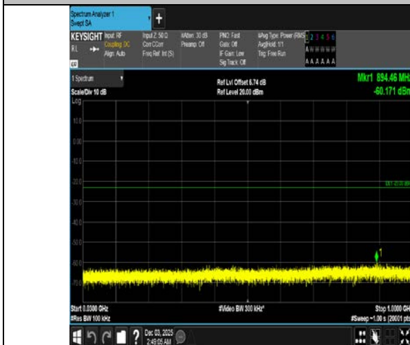
Band4-15MHz-QPSK-20175-75RB#0-30~1000-PASS
