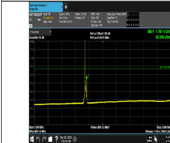
Band4-15MHz-16QAM-20325-1RB#0-1000~3000-PASS
