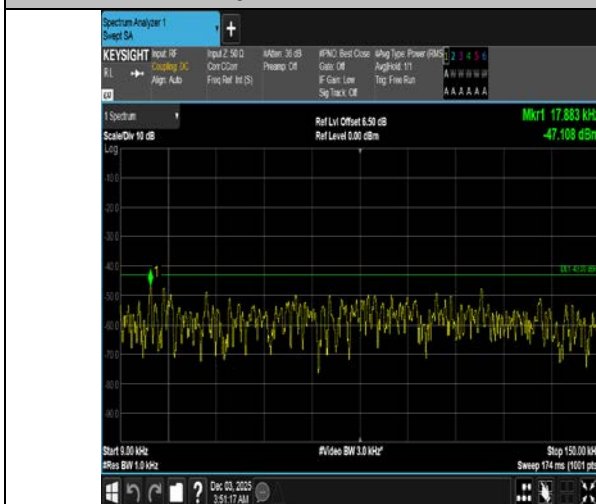
Band4-20MHz-QPSK-20300-1RB#0-0.009~0.15-PASS
