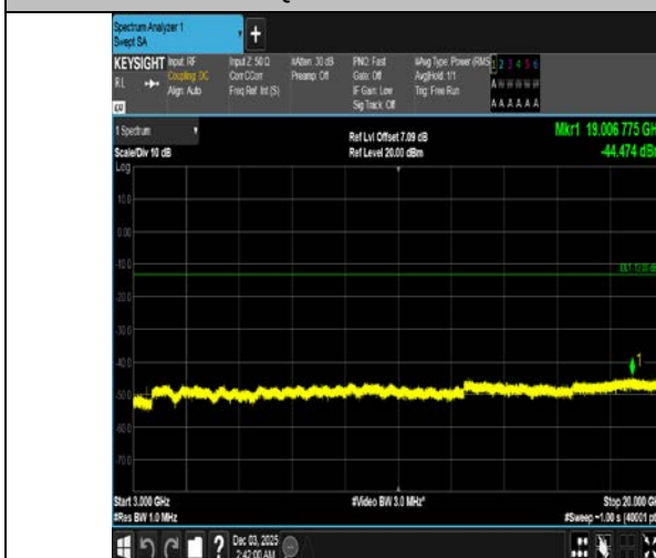
Band4-15MHz-16QAM-20025-1RB#74-3000~20000-PASS
