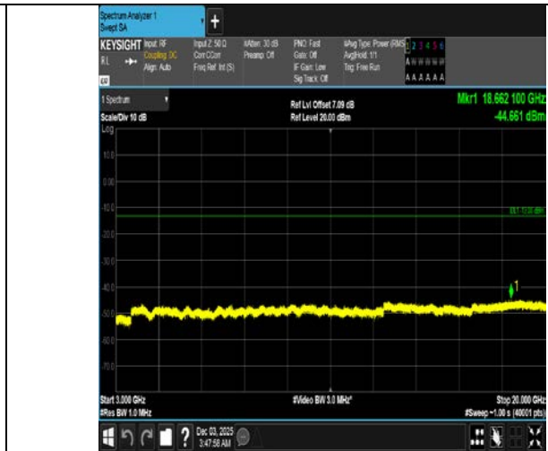
Band4-20MHz-QPSK-20175-1RB#99-3000~20000-PASS
