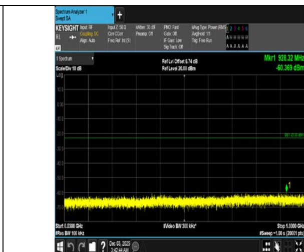
Band4-20MHz-16OAM-20050-100RB#0-30~1000-PASS
