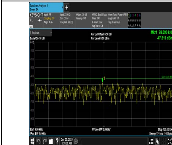
Band4-20MHz-QPSK-20050-100RB#0-0.009~0.15-PASS
