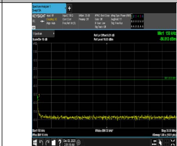
Band4-15MHz-QPSK-20325-1RB#0-0.15~30-PASS
