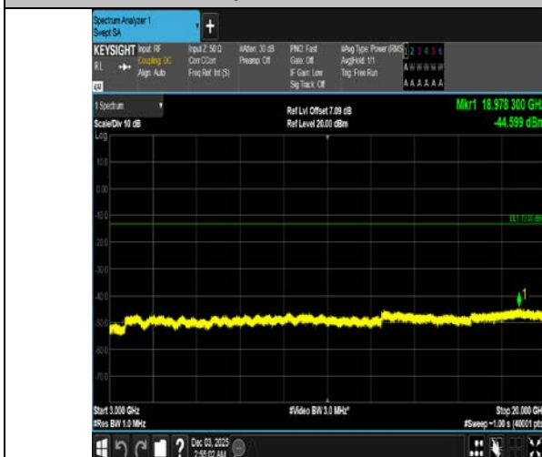
Band4-15MHz-16QAM-20325-1RB#74-3000~20000-PASS
