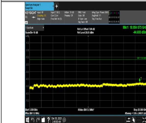
Band4-15MHz-QPSK-20175-1RB#0-3000~20000-PASS
