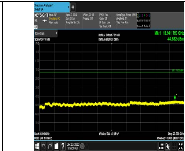
Band4-20MHz-QPSK-20300-1RB#99-3000~20000-PASS
