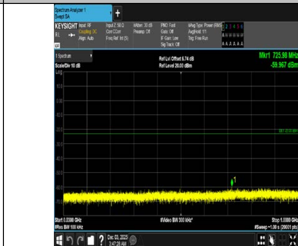
Band4-20MHz-QPSK-20175-1RB#99-30~1000-PASS
