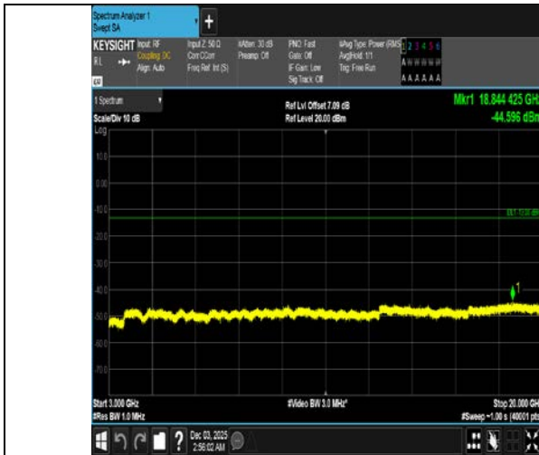
Band4-15MHz-QPSK-20325-75RB#0-3000~20000-PASS
