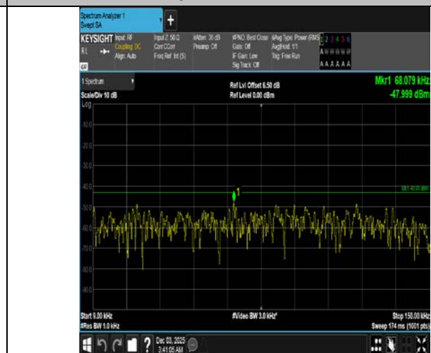
Band4-20MHz-16QAM-20050-100RB#0-0.009~0.15-PASS
