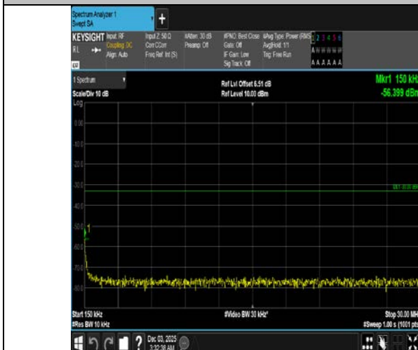
Band4-20MHz-QPSK-20050-1RB#99-0.15~30-PASS
