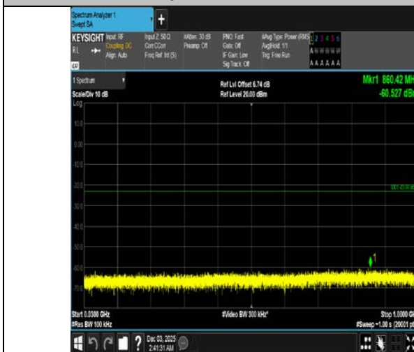
Band4-15MHz-16QAM-20025-1RB#74-30~1000-PASS
