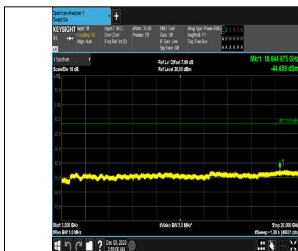
Band4-20MHz-OPSK-20300-100RB#0-3000~20000-PASS
