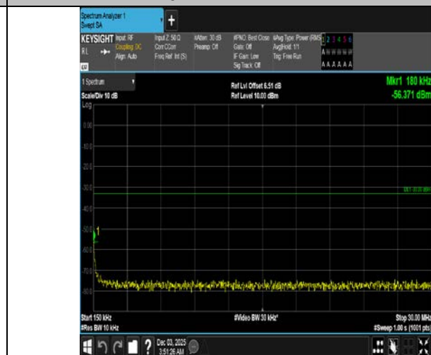
Band4-20MHz-QPSK-20300-1RB#0-0.15~30-PASS
