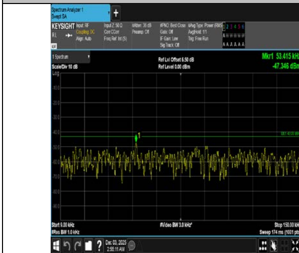
Band4-15MHz-QPSK-20325-75RB#0-0.009~0.15-PASS
