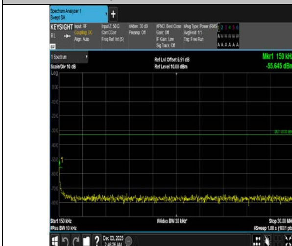
Band4-15MHz-QPSK-20175-1RB#74-0.15~30-PASS
