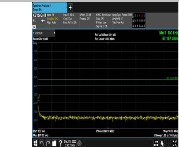
Band4-20MHz-QPSK-20050-100RB#0-0.15~30-PASS
