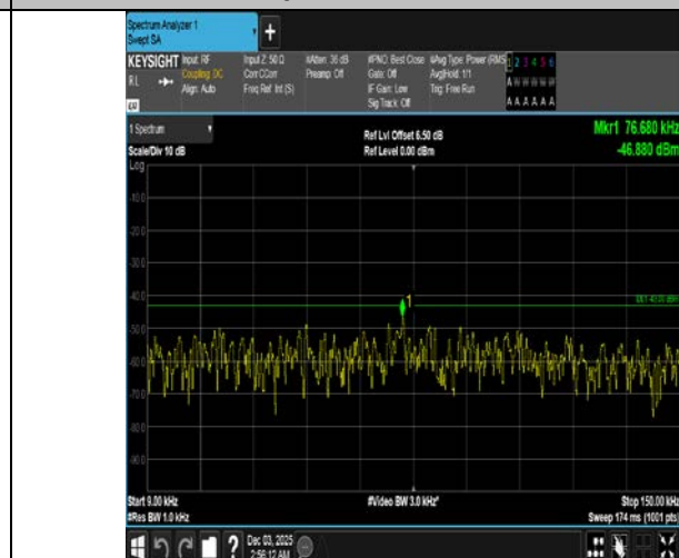
Band4-15MHz-16QAM-20325-75RB#0-0.009~0.15-PASS
