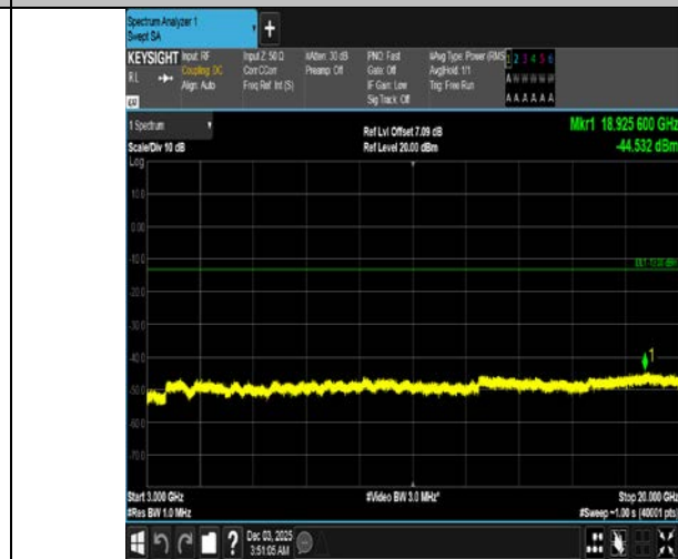
Band4-20MHz-16QAM-20175-100RB#0-3000~20000-PASS
