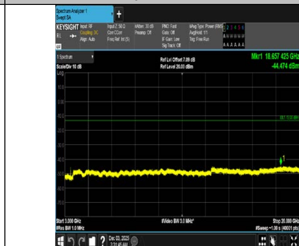
Band4-20MHz-16QAM-20050-1RB#0-3000~20000-PASS
