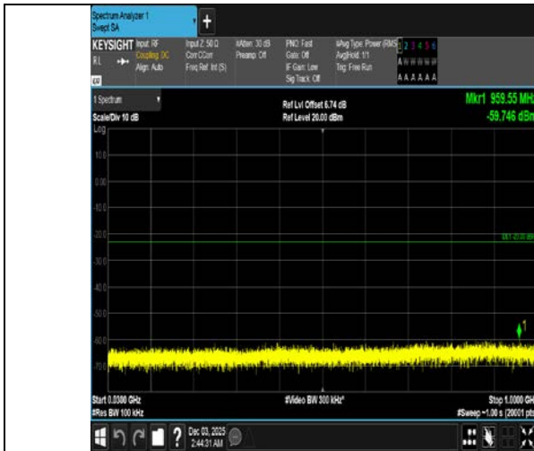
Band4-15MHz-QPSK-20175-1RB#0-30~1000-PASS
