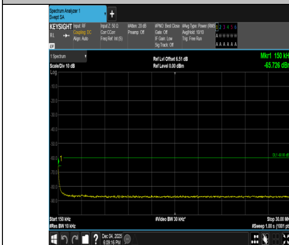
Band40(2305-2315)-10MHz-16QAM-38750-1RB#0-0.15~30-PASS
