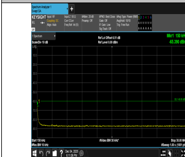
Band40(2305-2315)-10MHz-QPSK-38750-1RB#49-0.15~30-PASS
