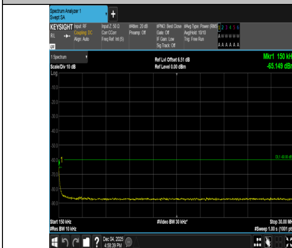
Band40(2305-2315)-5MHz-16QAM-38750-1RB#0-0.15~30-PASS
