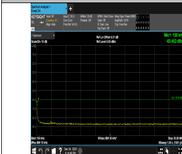
Band40(2305-2315)-10MHz-QPSK-38750-50RB#0-0.15~30-PASS
