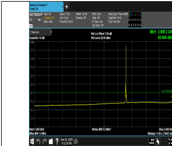
Band40(2305-2315)-5MHz-QPSK-38775-1RB#24-1000~3000-PASS
