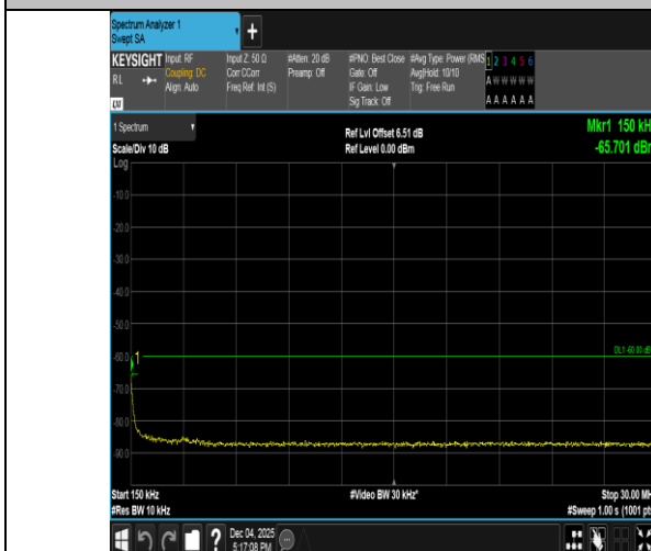
Band40(2305-2315)-5MHz-16QAM-38775-25RB#0-0.15~30-PASS
