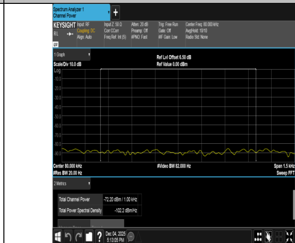
Band40(2305-2315)-5MHz-16QAM-38775-1RB#24-0.009~0.15-PASS
