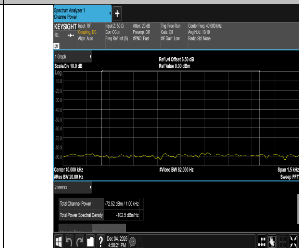
Band40(2305-2315)-5MHz-16QAM-38750-1RB#0-0.009~0.15-PASS
