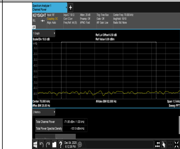
Band40(2305-2315)-10MHz-16QAM-38750-1RB#49-0.009~0.15-PASS
