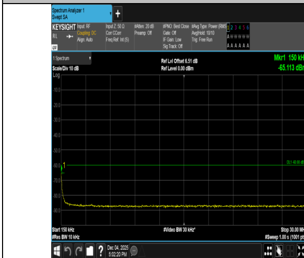
Band40(2305-2315)-5MHz-16QAM-38750-1RB#24-0.15~30-PASS
