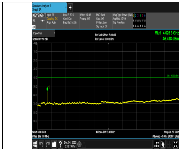
Band40(2305-2315)-5MHz-16QAM-38775-25RB#0-3000~26500-PASS
