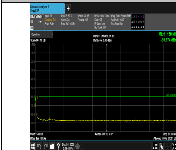
Band40(2305-2315)-5MHz-16QAM-38775-1RB#0-0.15~30-PASS
