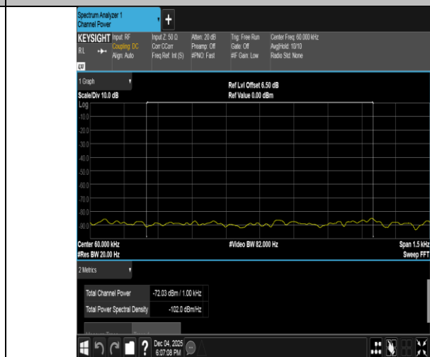
Band40(2305-2315)-10MHz-QPSK-38750-1RB#0-0.009~0.15-PASS
