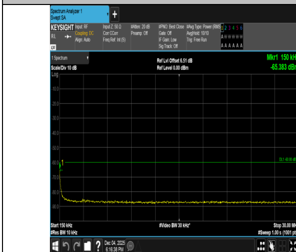
Band40(2305-2315)-10MHz-16QAM-38750-50RB#0-0.15~30-PASS
