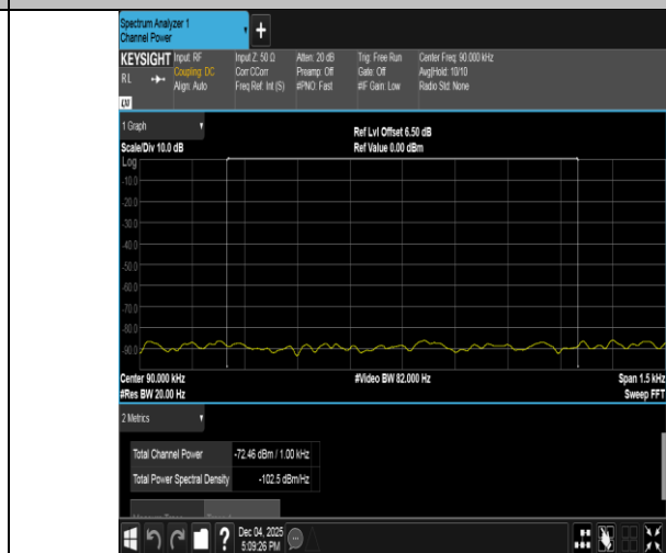
Band40(2305-2315)-5MHz-16QAM-38775-1RB#0-0.009~0.15-PASS
