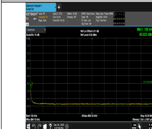
Band40(2305-2315)-5MHz-QPSK-38775-1RB#0-0.15~30-PASS
