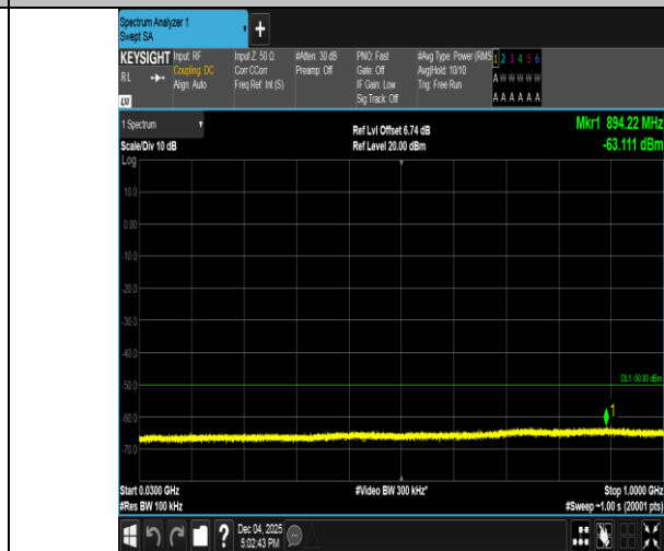
Band40(2305-2315)-5MHz-16QAM-38750-1RB#24-30~1000-PASS
