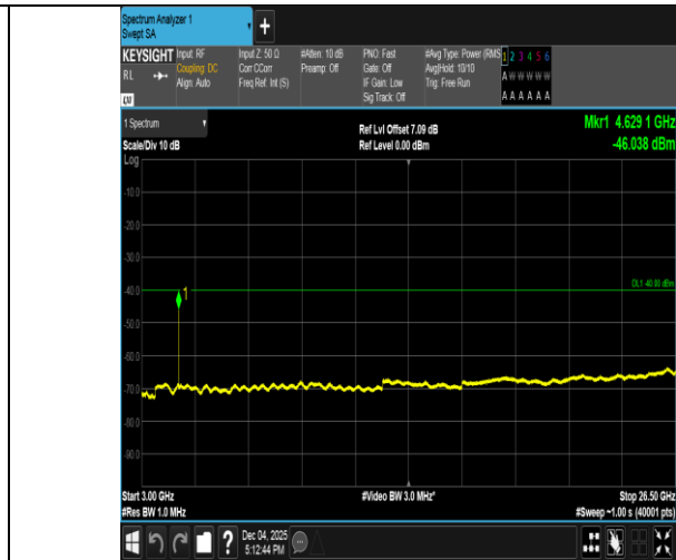
Band40(2305-2315)-5MHz-QPSK-38775-1RB#24-3000~26500-PASS
