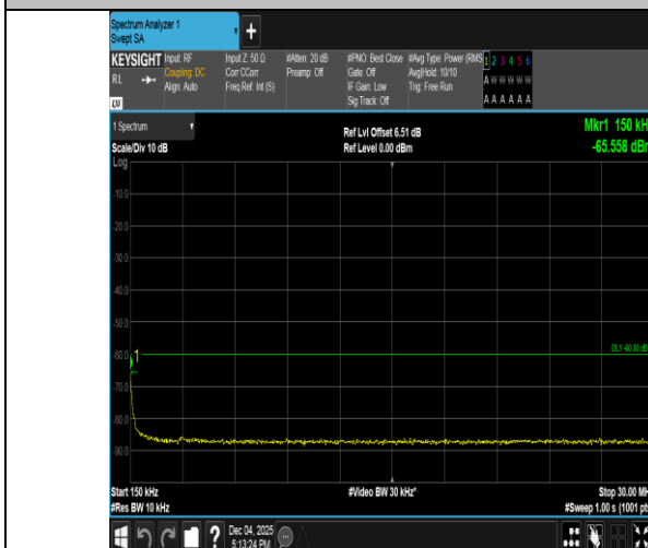
Band40(2305-2315)-5MHz-16QAM-38775-1RB#24-0.15~30-PASS
