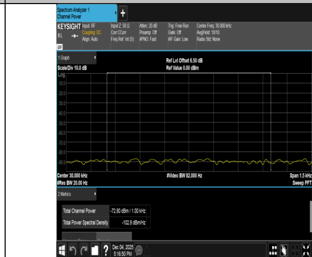
Band40(2305-2315)-5MHz-16QAM-38775-25RB#0-0.009~0.15-PASS
