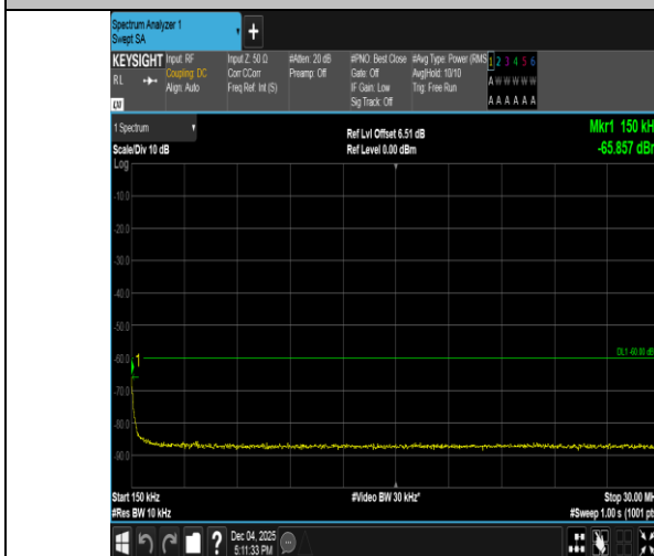
Band40(2305-2315)-5MHz-QPSK-38775-1RB#24-0.15~30-PASS
