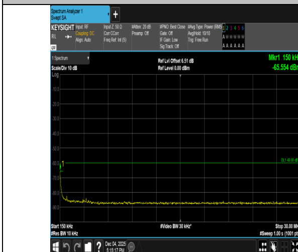
Band40(2305-2315)-5MHz-QPSK-38775-25RB#0-0.15~30-PASS
