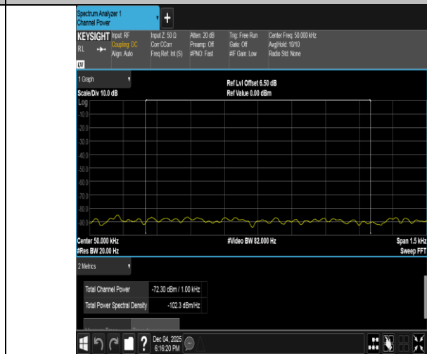
Band40(2305-2315)-10MHz-16QAM-38750-50RB#0-0.009~0.15-PASS
