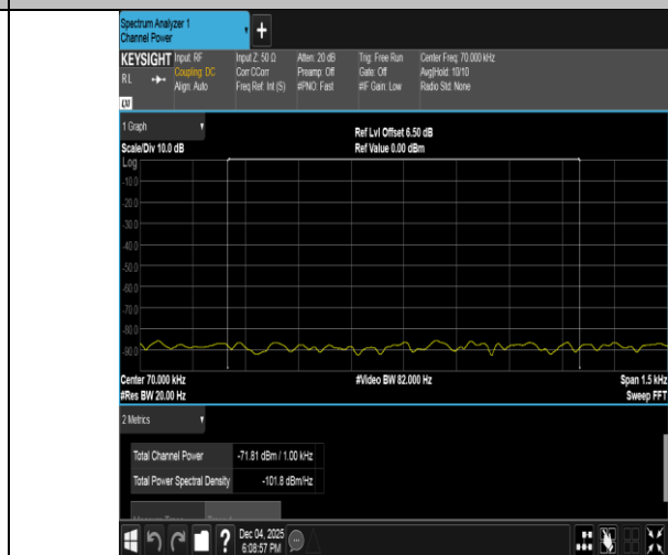
Band40(2305-2315)-10MHz-16QAM-38750-1RB#0-0.009~0.15-PASS
