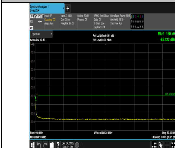
Band40(2305-2315)-5MHz-16QAM-38750-25RB#0-0.15~30-PASS
