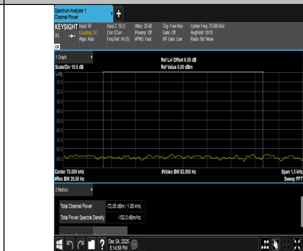
Band40(2305-2315)-5MHz-QPSK-38775-25RB#0-0.009~0.15-PASS
