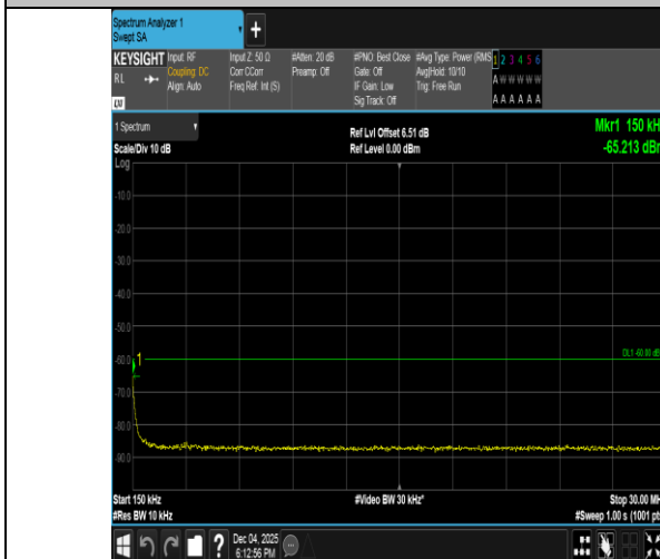
Band40(2305-2315)-10MHz-16QAM-38750-1RB#49-0.15~30-PASS
