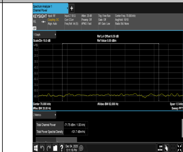
Band40(2305-2315)-5MHz-QPSK-38775-1RB#24-0.009~0.15-PASS
