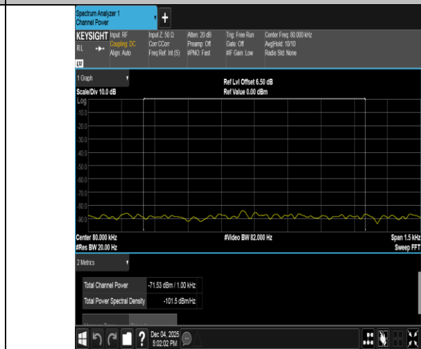
Band40(2305-2315)-5MHz-16QAM-38750-1RB#24-0.009~0.15-PASS
