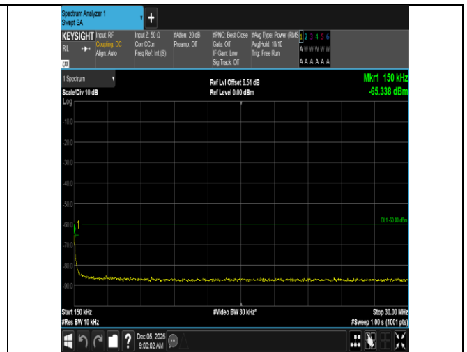
Band40(2350-2360)-10MHz-16QAM-39200-50RB#0-0.15~30-PASS
