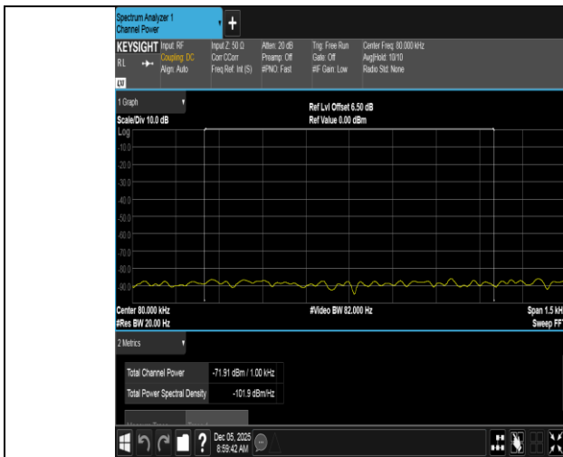
Band40(2350-2360)-10MHz-16QAM-39200-50RB#0-0.009~0.15-PASS
