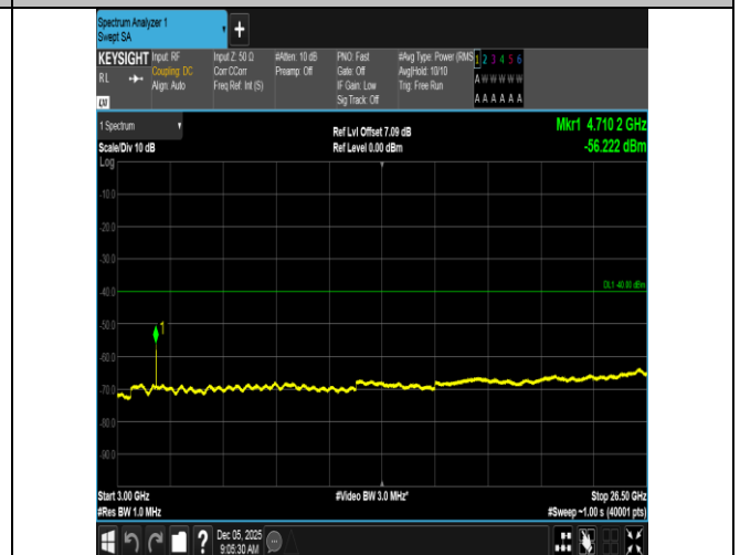
Band40(2350-2360)-10MHz-16QAM-39200-50RB#0-3000~26500-PASS
