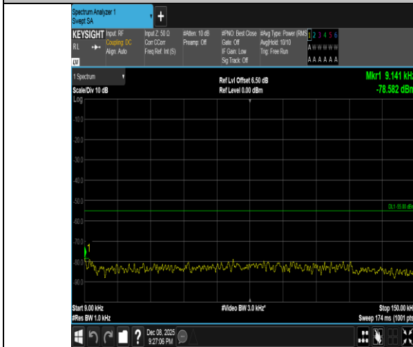
Band41-5MHz-QPSK-39675-25RB#0-0.009~0.15-PASS
