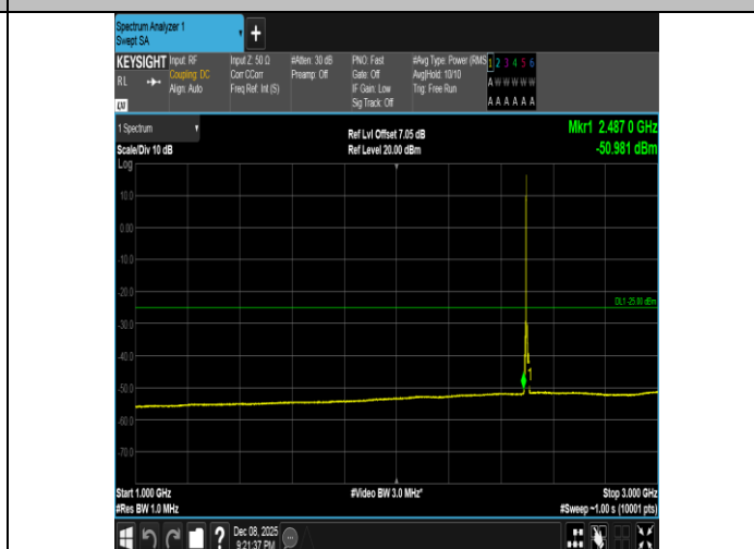
Band41-5MHz-16QAM-39675-1RB#0-1000~3000-PASS
