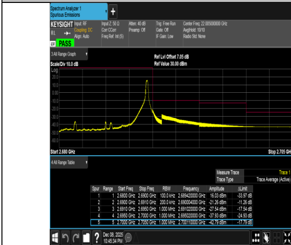
Band41-10MHz-16QAM-41540-1RB#49-PASS
