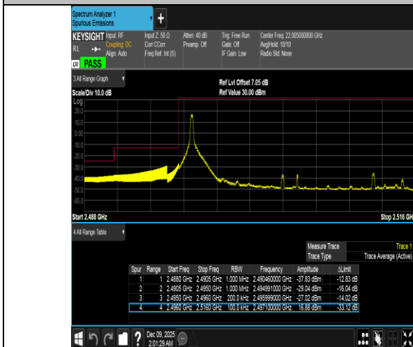
Band41-20MHz-QPSK-39750-1RB#0-PASS
