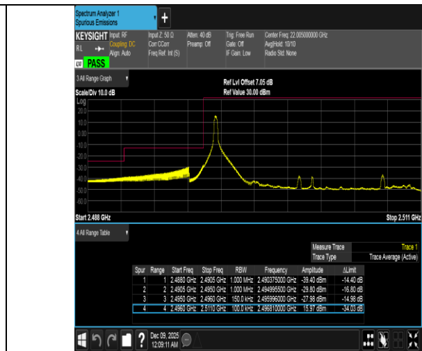
Band41-15MHz-16QAM-39725-1RB#0-PASS
