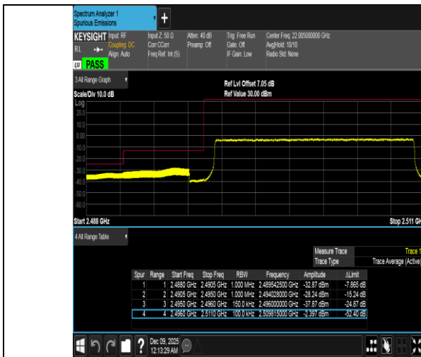
Band41-15MHz-QPSK-39725-75RB#0-PASS
