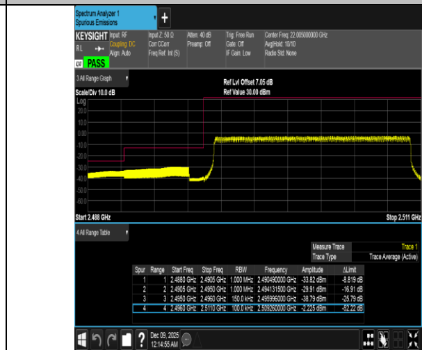
Band41-15MHz-16QAM-39725-75RB#0-PASS
