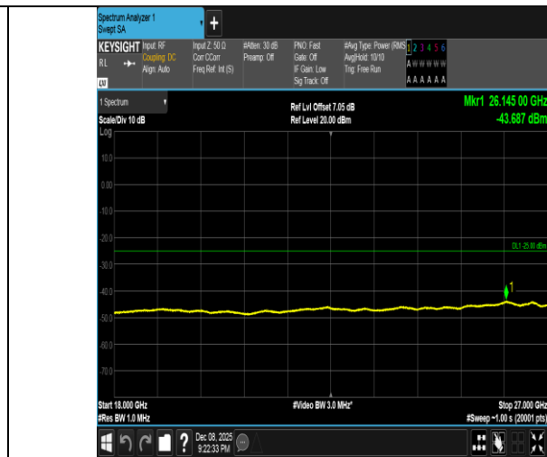
Band41-5MHz-16QAM-39675-1RB#0-18000~27000-PASS
