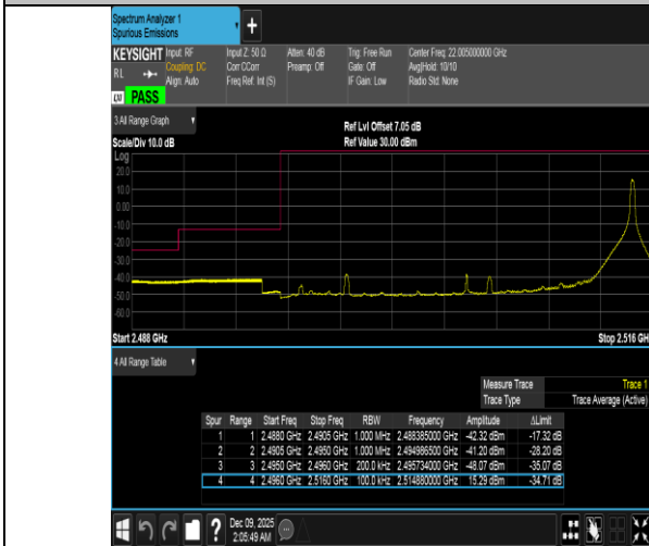
Band41-20MHz-16QAM-39750-1RB#99-PASS
