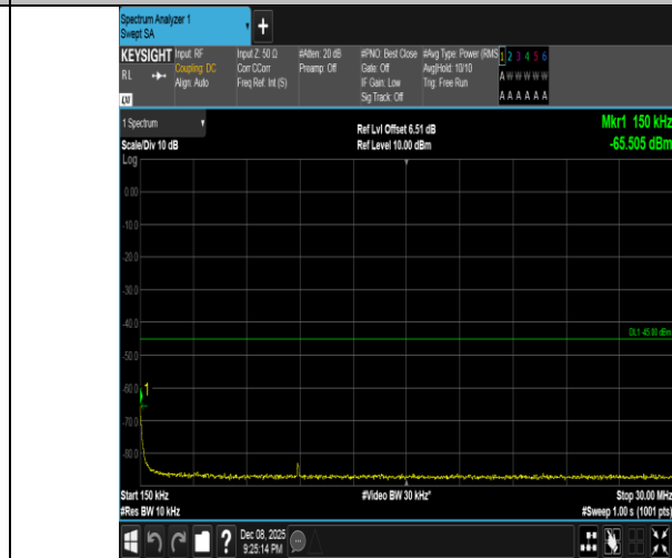
Band41-5MHz-16QAM-39675-1RB#24-0.15~30-PASS
