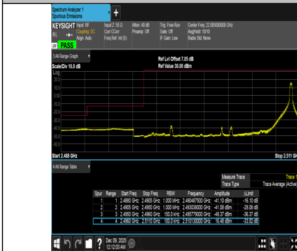
Band41-15MHz-16QAM-39725-1RB#74-PASS
