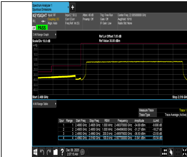
Band41-20MHz-QPSK-39750-100RB#0-PASS
