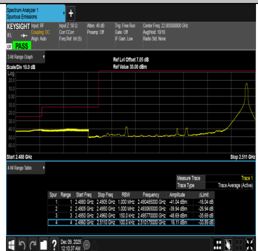
Band41-15MHz-QPSK-39725-1RB#74-PASS
