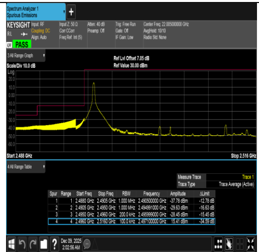
Band41-20MHz-16QAM-39750-1RB#0-PASS
