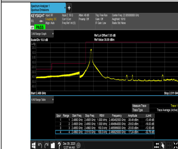
Band41-15MHz-QPSK-39725-1RB#0-PASS
