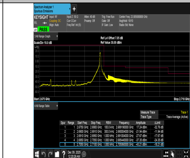
Band41-15MHz-QPSK-41515-1RB#74-PASS
