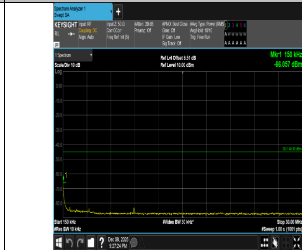
Band41-5MHz-QPSK-39675-25RB#0-0.15~30-PASS
