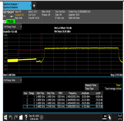
Band41-20MHz-16QAM-39750-100RB#0-PASS
