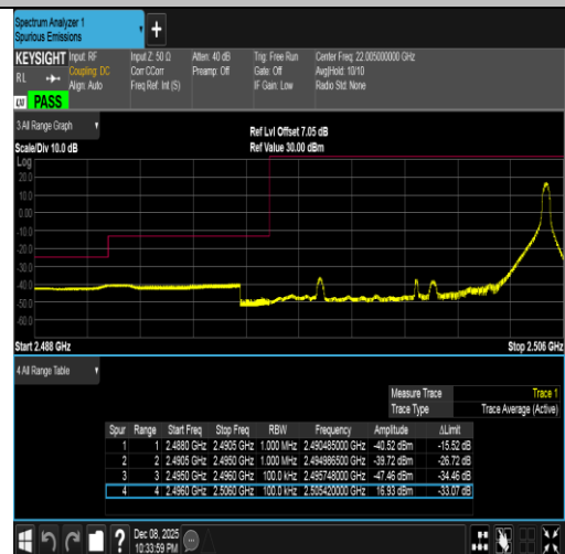
Band41-10MHz-QPSK-39700-1RB#49-PASS
