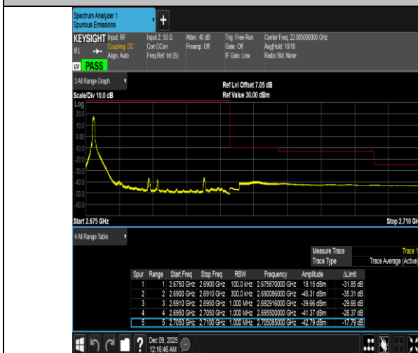
Band41-15MHz-QPSK-41515-1RB#0-PASS
