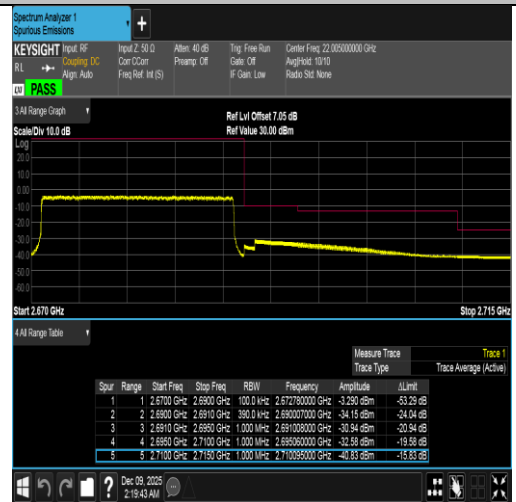
Band41-20MHz-16QAM-41490-100RB#0-PASS
