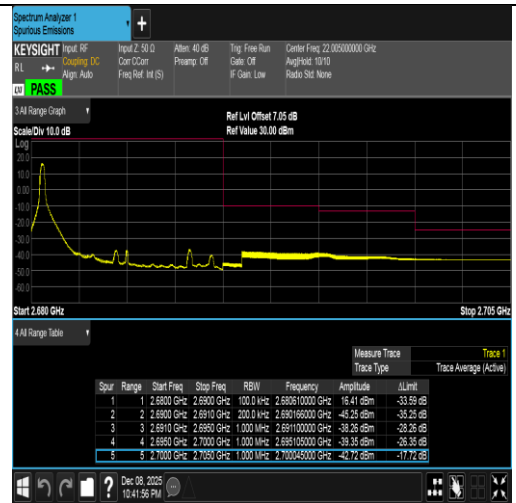
Band41-10MHz-16QAM-41540-1RB#0-PASS
