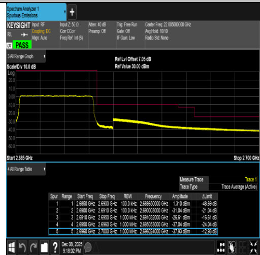
Band41-5MHz-16QAM-41565-25RB#0-PASS
