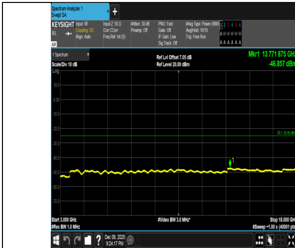
Band41-5MHz-QPSK-39675-1RB#24-3000~18000-PASS
