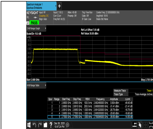
Band41-10MHz-QPSK-41540-50RB#0-PASS
