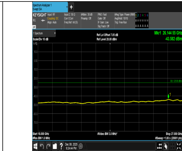
Band41-5MHz-QPSK-39675-1RB#24-18000~27000-PASS
