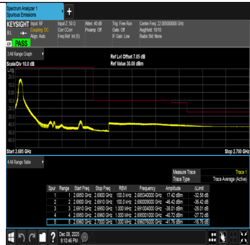
Band41-5MHz-16QAM-41565-1RB#0-PASS
