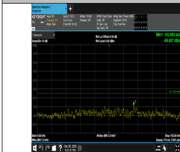
Band41-5MHz-QPSK-40620-1RB#0-0.009~0.15-PASS
