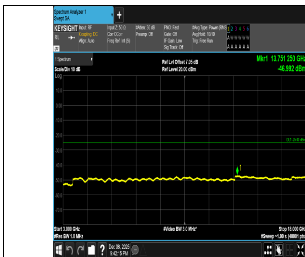
Band41-5MHz-QPSK-40620-25RB#0-3000~18000-PASS
