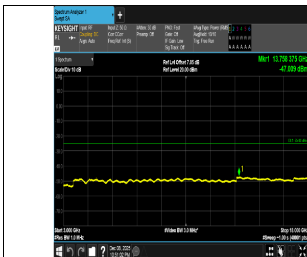
Band41-10MHz-QPSK-39700-1RB#0-3000~18000-PASS
