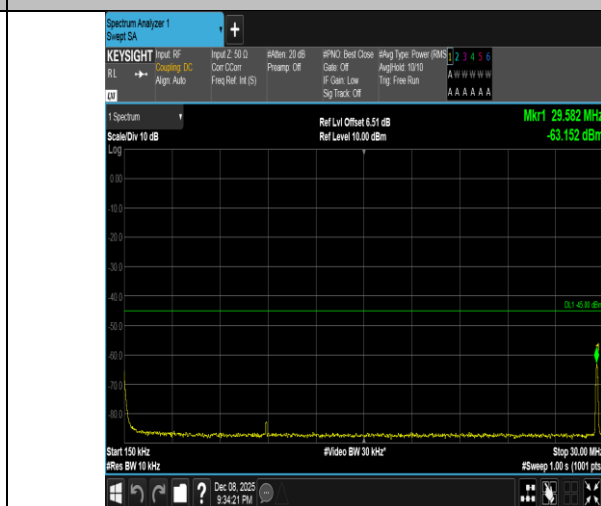
Band41-5MHz-16QAM-40620-1RB#0-0.15~30-PASS
