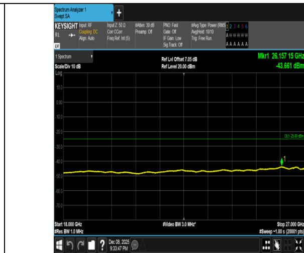
Band41-5MHz-QPSK-40620-1RB#0-18000~27000-PASS
