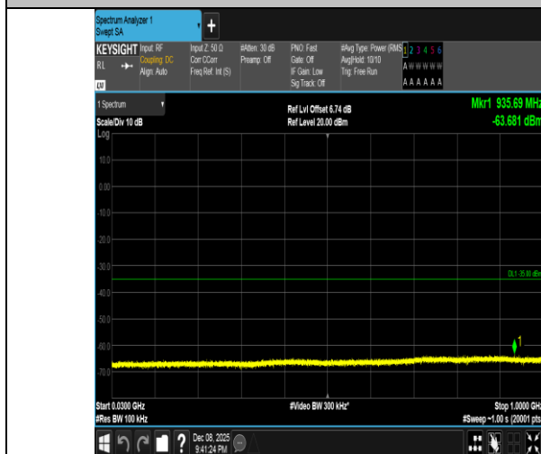
Band41-5MHz-QPSK-40620-25RB#0-30~1000-PASS
