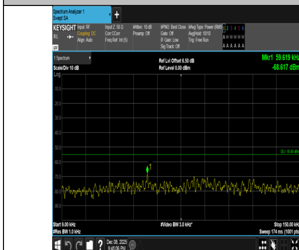
Band41-5MHz-QPSK-41565-1RB#0-0.009~0.15-PASS
