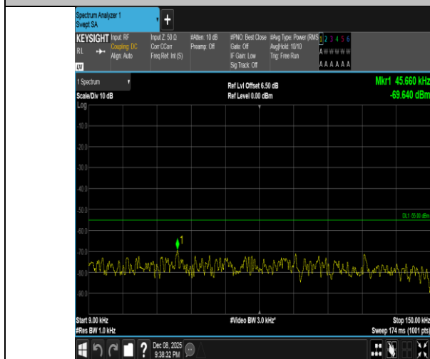
Band41-5MHz-16QAM-40620-1RB#24-0.009~0.15-PASS
