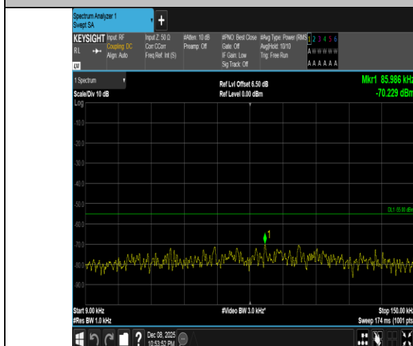
Band41-10MHz-QPSK-39700-1RB#49-0.009~0.15-PASS
