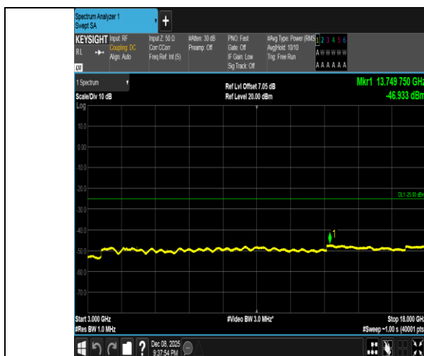
Band41-5MHz-QPSK-40620-1RB#24-3000~18000-PASS
