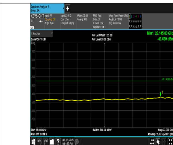
Band41-5MHz-QPSK-41565-1RB#24-18000~27000-PASS
