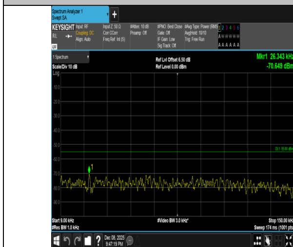
Band41-5MHz-16QAM-41565-1RB#0-0.009~0.15-PASS
