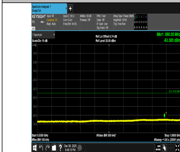
Band41-5MHz-16QAM-41565-1RB#0-30~1000-PASS
