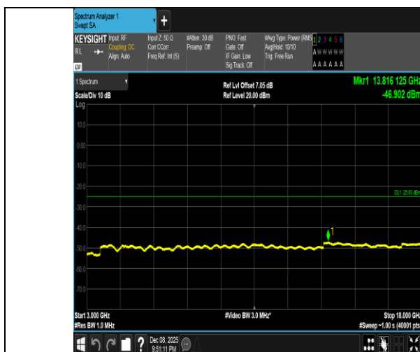
Band41-5MHz-QPSK-41565-1RB#24-3000~18000-PASS
