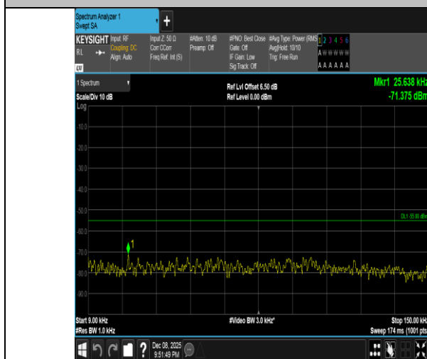
Band41-5MHz-16QAM-41565-1RB#24-0.009~0.15-PASS
