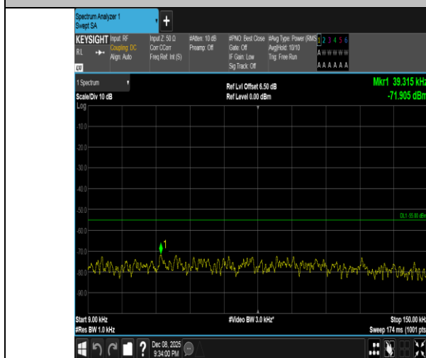
Band41-5MHz-16QAM-40620-1RB#0-0.009~0.15-PASS
