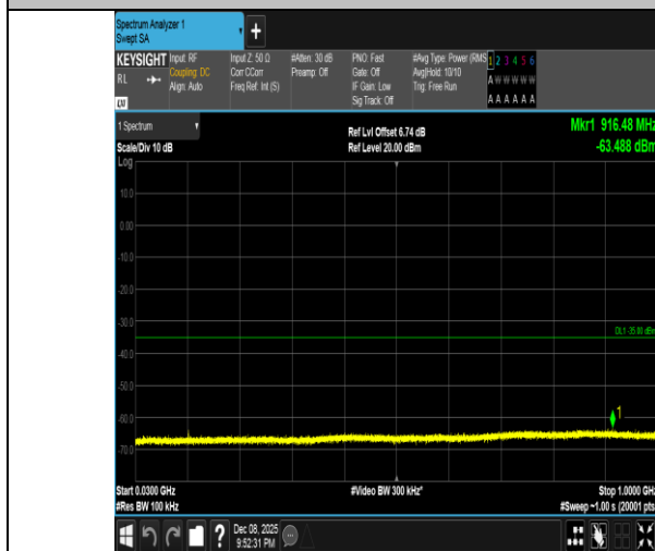
Band41-5MHz-16QAM-41565-1RB#24-30~1000-PASS
