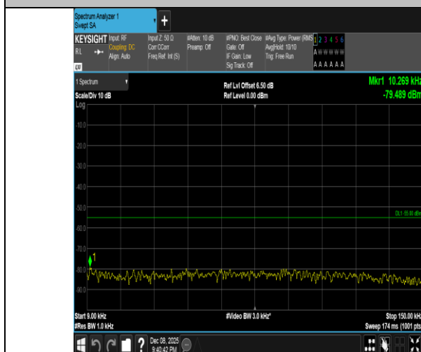
Band41-5MHz-QPSK-40620-25RB#0-0.009~0.15-PASS
