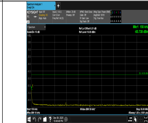
Band41-10MHz-QPSK-39700-1RB#0-0.15~30-PASS
