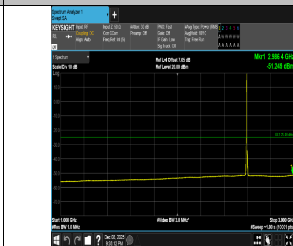
Band41-5MHz-16QAM-40620-1RB#0-1000~3000-PASS
