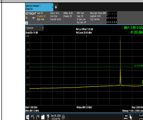
Band41-5MHz-QPSK-40620-1RB#0-1000~3000-PASS
