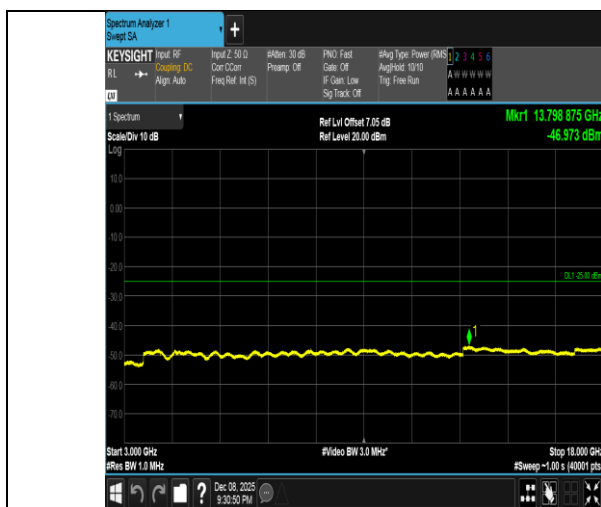
Band41-5MHz-16QAM-39675-25RB#0-3000~18000-PASS
