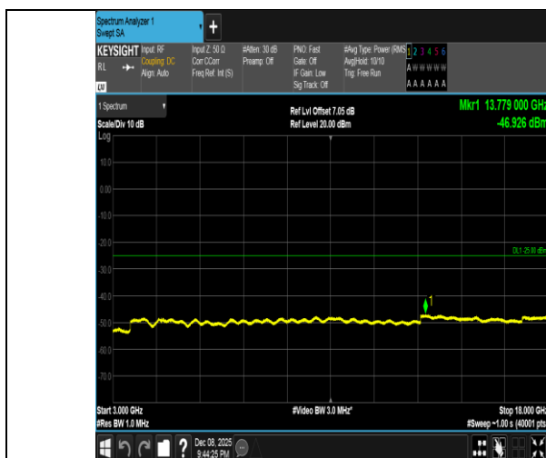
Band41-5MHz-16QAM-40620-25RB#0-3000~18000-PASS
