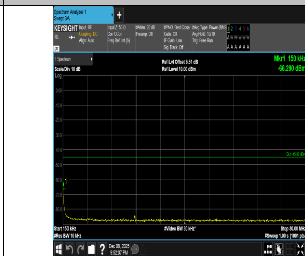
Band41-5MHz-16QAM-41565-1RB#24-0.15~30-PASS
