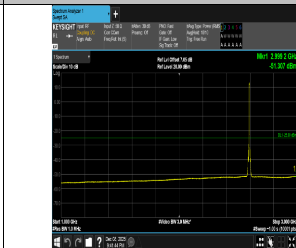
Band41-5MHz-QPSK-40620-25RB#0-1000~3000-PASS
