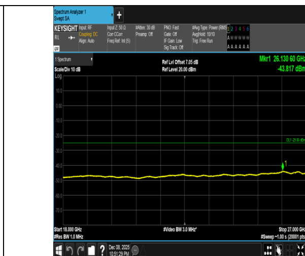
Band41-10MHz-QPSK-39700-1RB#0-18000~27000-PASS
