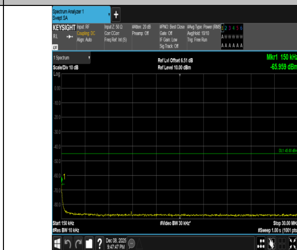
Band41-5MHz-16QAM-41565-1RB#0-0.15~30-PASS
