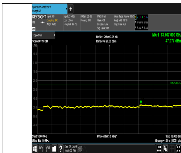
Band41-5MHz-16QAM-41565-1RB#0-3000~18000-PASS
