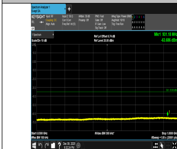
Band41-5MHz-QPSK-40620-1RB#0-30~1000-PASS
