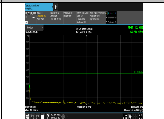
Band41-10MHz-QPSK-39700-50RB#0-0.15~30-PASS
