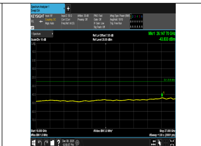
Band41-10MHz-QPSK-39700-1RB#49-18000~27000-PASS
