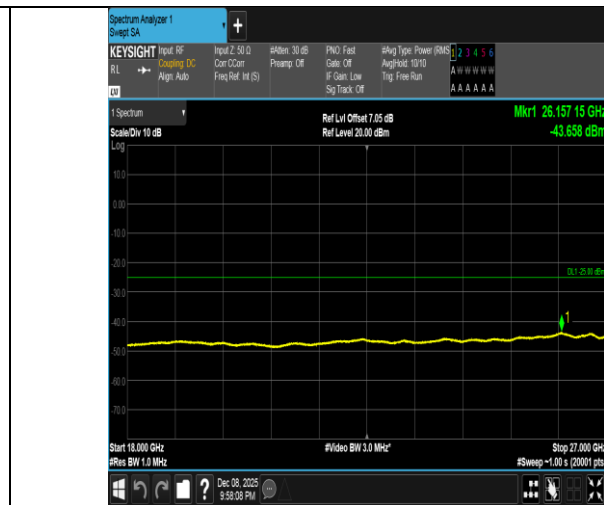
Band41-5MHz-16QAM-41565-25RB#0-18000~27000-PASS
