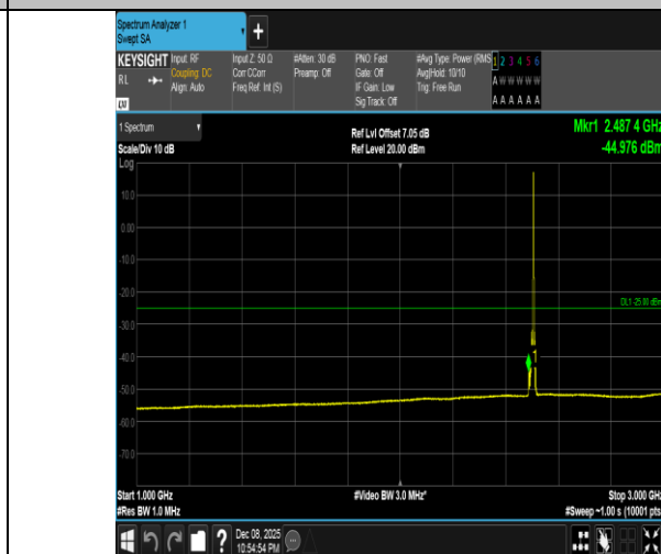
Band41-10MHz-QPSK-39700-1RB#49-1000~3000-PASS
