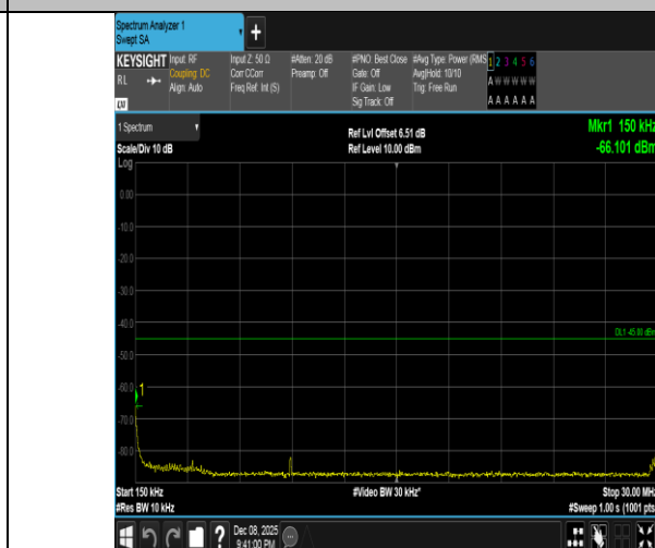
Band41-5MHz-QPSK-40620-25RB#0-0.15~30-PASS
