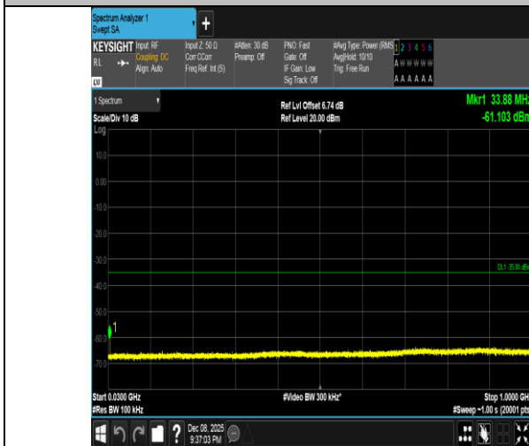
Band41-5MHz-QPSK-40620-1RB#24-30~1000-PASS
