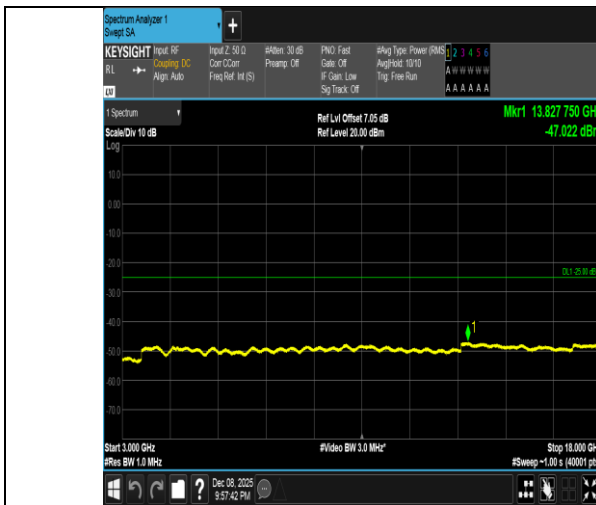
Band41-5MHz-16QAM-41565-25RB#0-3000~18000-PASS
