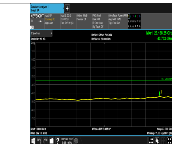
Band41-5MHz-QPSK-40620-1RB#24-18000~27000-PASS
