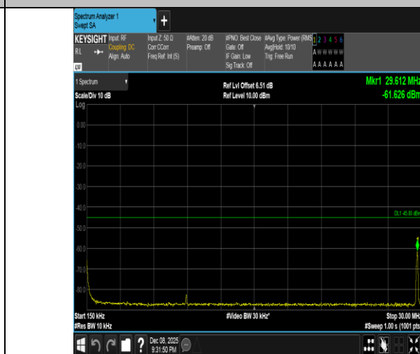
Band41-5MHz-QPSK-40620-1RB#0-0.15~30-PASS
