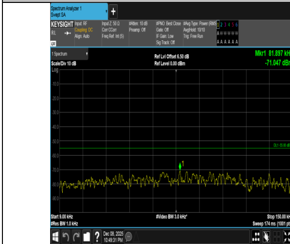
Band41-10MHz-QPSK-39700-1RB#0-0.009~0.15-PASS
