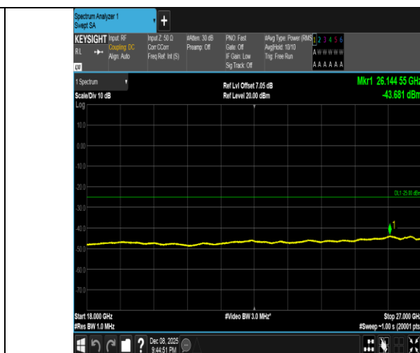
Band41-5MHz-16QAM-40620-25RB#0-18000~27000-PASS
