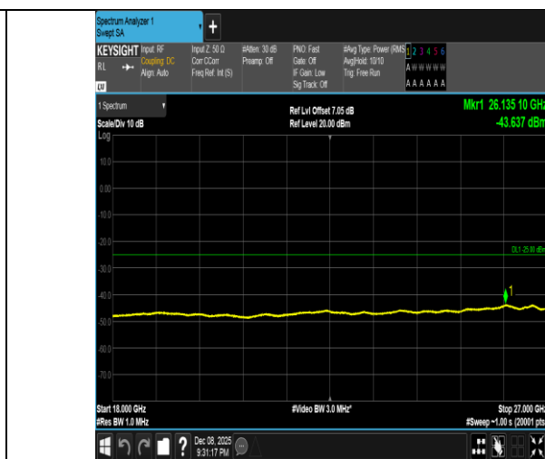
Band41-5MHz-16QAM-39675-25RB#0-18000~27000-PASS
