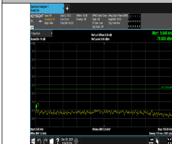
Band41-5MHz-QPSK-41565-25RB#0-0.009~0.15-PASS
