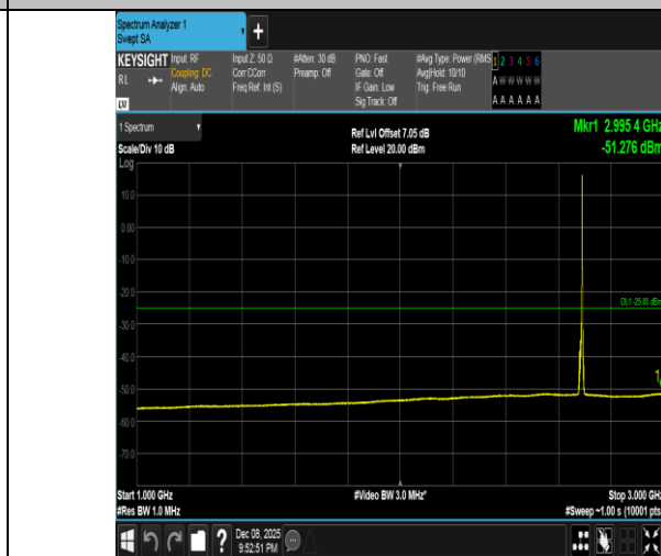
Band41-5MHz-16QAM-41565-1RB#24-1000~3000-PASS
