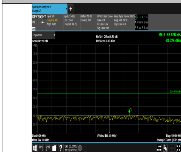
Band41-10MHz-16QAM-40620-50RB#0-0.009~0.15-PASS
