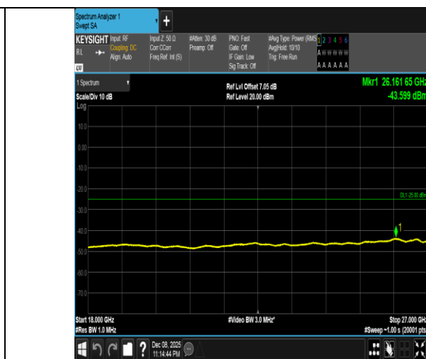
Band41-10MHz-16QAM-40620-1RB#49-18000~27000-PASS
