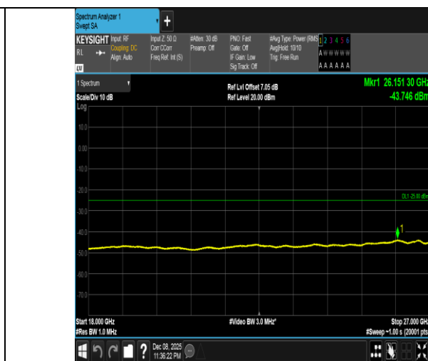
Band41-10MHz-16QAM-41540-50RB#0-18000~27000-PASS
