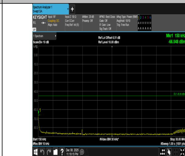
Band41-10MHz-16QAM-40620-50RB#0-0.15~30-PASS
