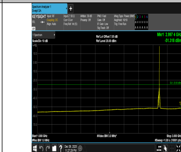
Band41-10MHz-QPSK-41540-1RB#49-1000~3000-PASS
