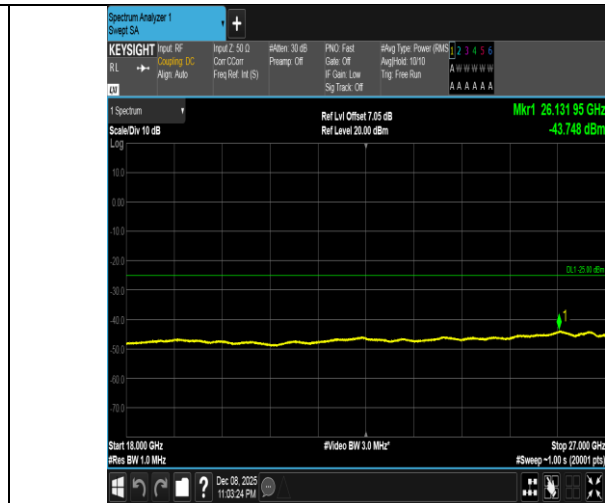
Band41-10MHz-16QAM-39700-50RB#0-18000~27000-PASS
