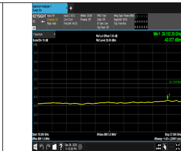
Band41-10MHz-QPSK-40620-1RB#49-18000~27000-PASS
