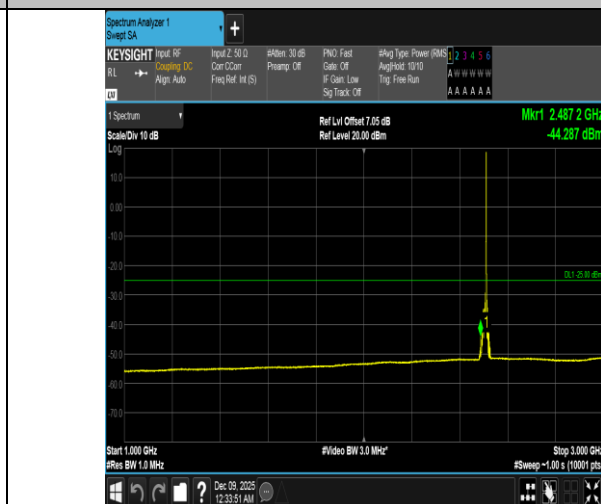
Band41-15MHz-QPSK-39725-1RB#74-1000~3000-PASS
