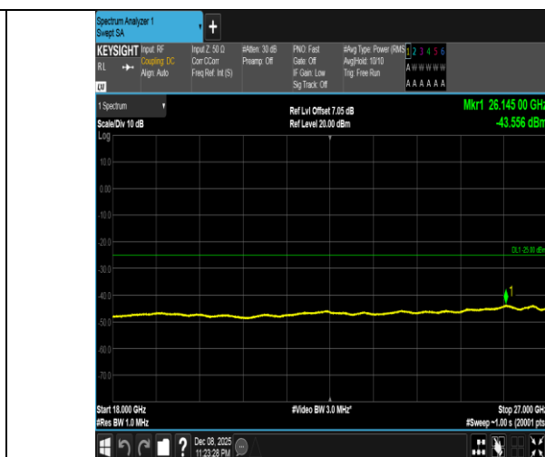
Band41-10MHz-QPSK-41540-1RB#0-18000~27000-PASS
