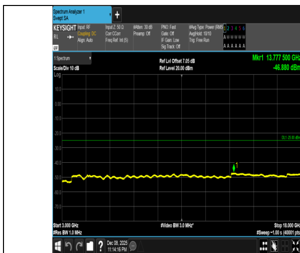
Band41-10MHz-16QAM-40620-1RB#49-3000~18000-PASS
