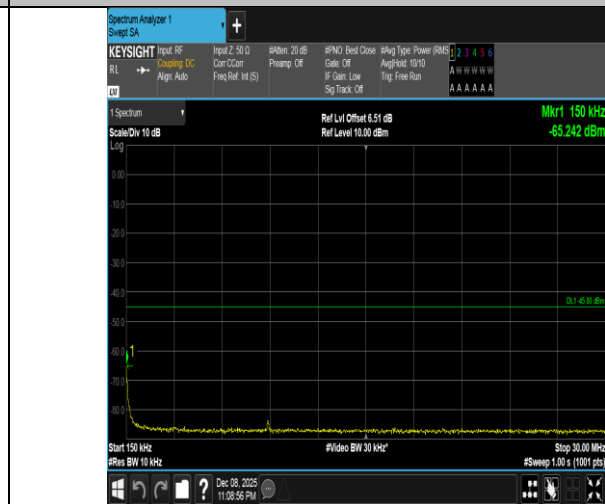
Band41-10MHz-QPSK-40620-1RB#49-0.15~30-PASS
