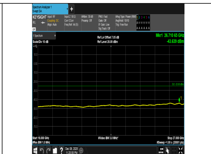
Band41-10MHz-16QAM-41540-1RB#0-18000~27000-PASS
