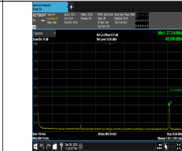
Band41-10MHz-QPSK-40620-1RB#0-0.15~30-PASS
