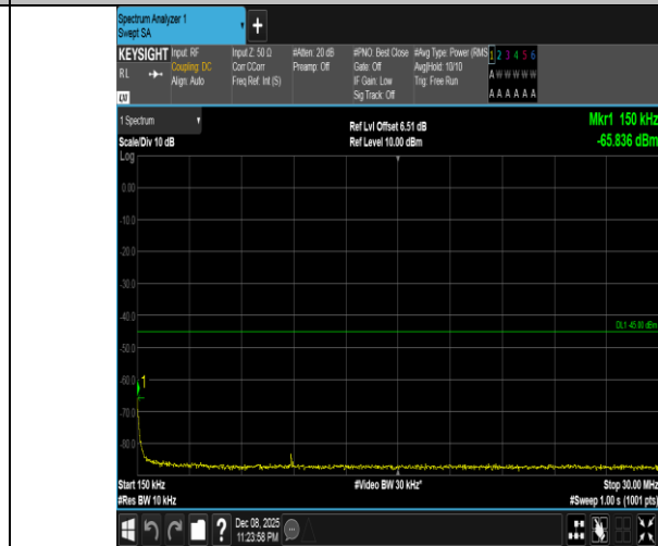
Band41-10MHz-16QAM-41540-1RB#0-0.15~30-PASS
