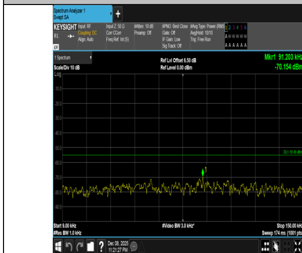
Band41-10MHz-QPSK-41540-1RB#0-0.009~0.15-PASS
