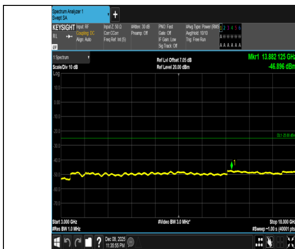
Band41-10MHz-16QAM-41540-50RB#0-3000~18000-PASS
