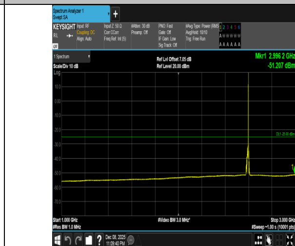
Band41-10MHz-QPSK-40620-1RB#49-1000~3000-PASS
