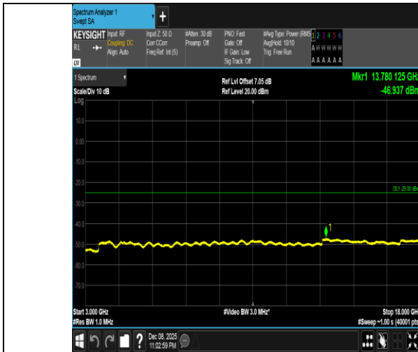
Band41-10MHz-16QAM-39700-50RB#0-3000~18000-PASS
