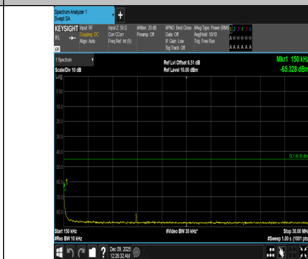
Band41-15MHz-QPSK-39725-1RB#0-0.15~30-PASS
