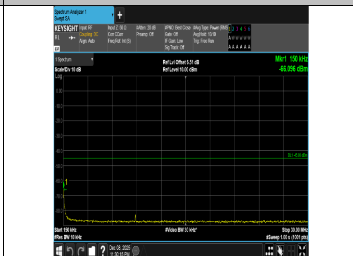
Band41-10MHz-16QAM-41540-1RB#49-0.15~30-PASS
