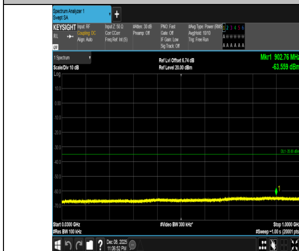
Band41-10MHz-16QAM-40620-1RB#0-30~1000-PASS
