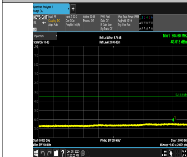
Band41-10MHz-16QAM-41540-50RB#0-30~1000-PASS
