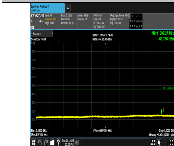
Band41-10MHz-QPSK-41540-50RB#0-30~1000-PASS
