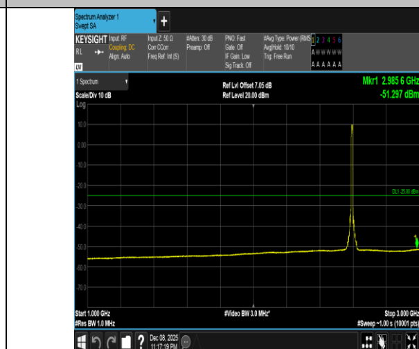
Band41-10MHz-QPSK-40620-50RB#0-1000~3000-PASS
