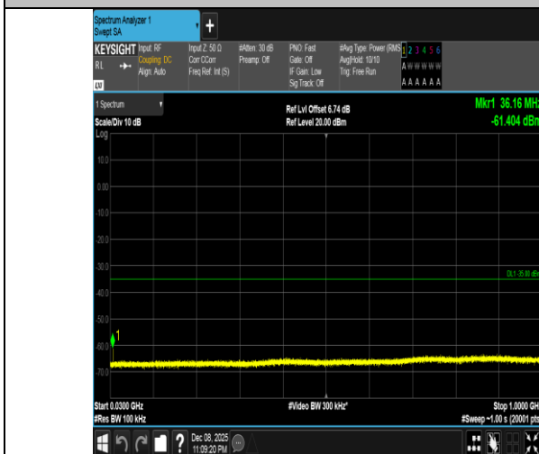
Band41-10MHz-QPSK-40620-1RB#49-30~1000-PASS
