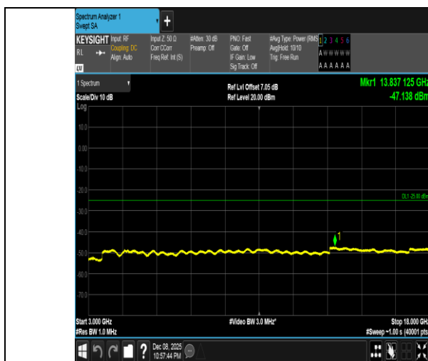
Band41-10MHz-16QAM-39700-1RB#49-3000~18000-PASS
