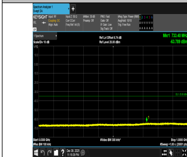
Band41-10MHz-16QAM-40620-50RB#0-30~1000-PASS
