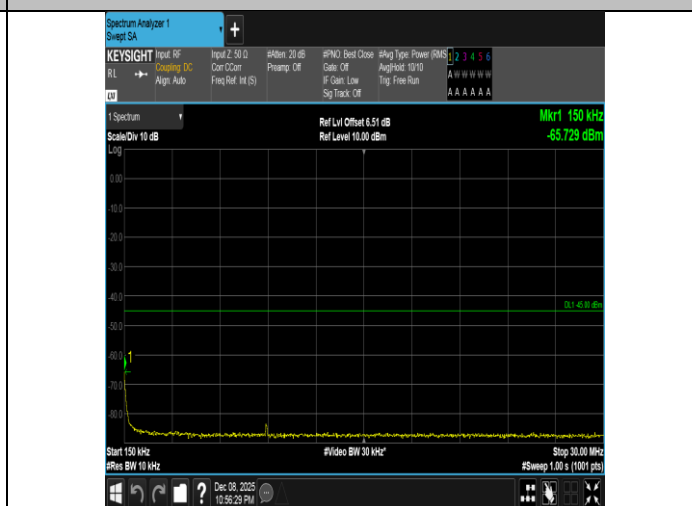
Band41-10MHz-16QAM-39700-1RB#49-0.15~30-PASS
