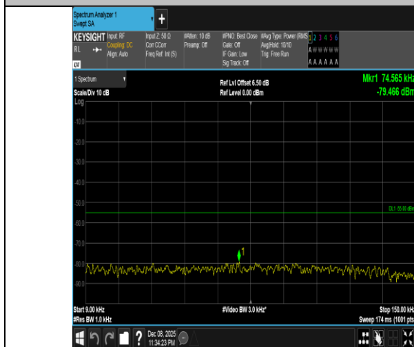
Band41-10MHz-16QAM-41540-50RB#0-0.009~0.15-PASS
