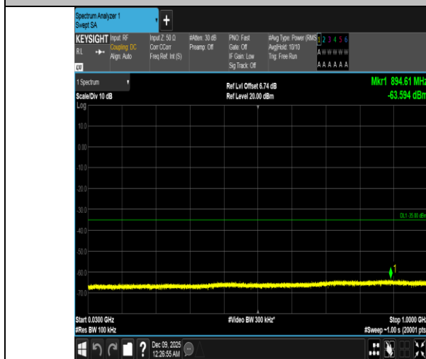
Band41-15MHz-QPSK-39725-1RB#0-30~1000-PASS
