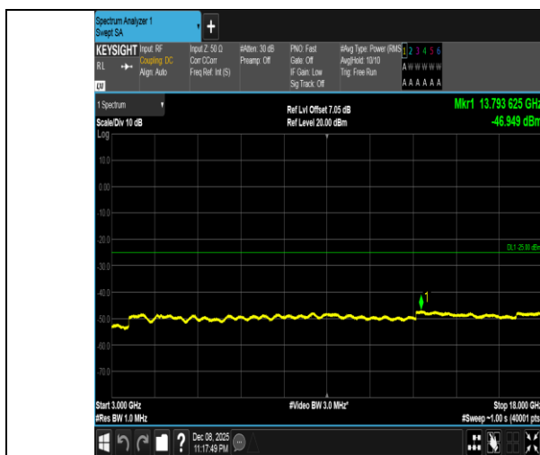
Band41-10MHz-QPSK-40620-50RB#0-3000~18000-PASS
