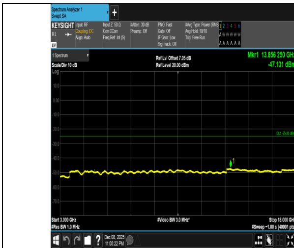
Band41-10MHz-QPSK-40620-1RB#0-3000~18000-PASS
