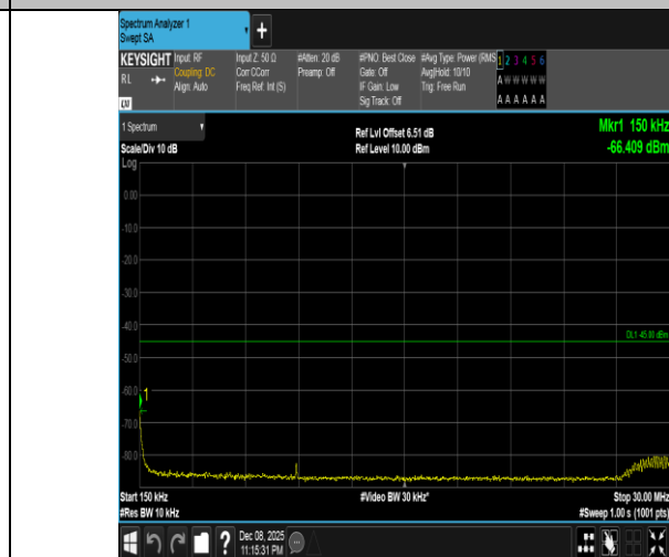
Band41-10MHz-QPSK-40620-50RB#0-0.15~30-PASS
