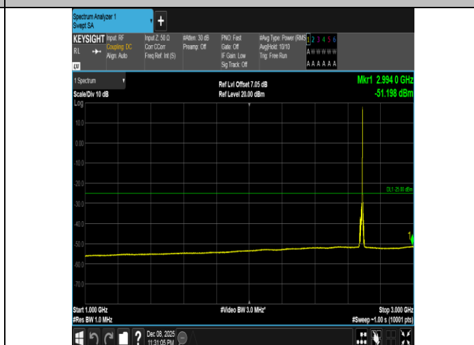
Band41-10MHz-16QAM-41540-1RB#49-1000~3000-PASS
