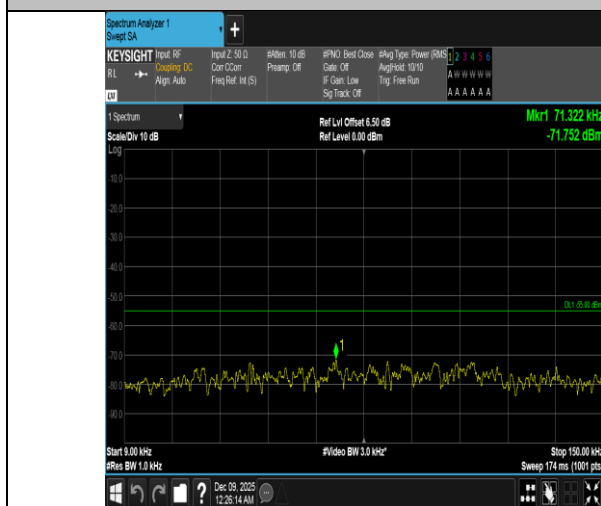
Band41-15MHz-QPSK-39725-1RB#0-0.009~0.15-PASS
