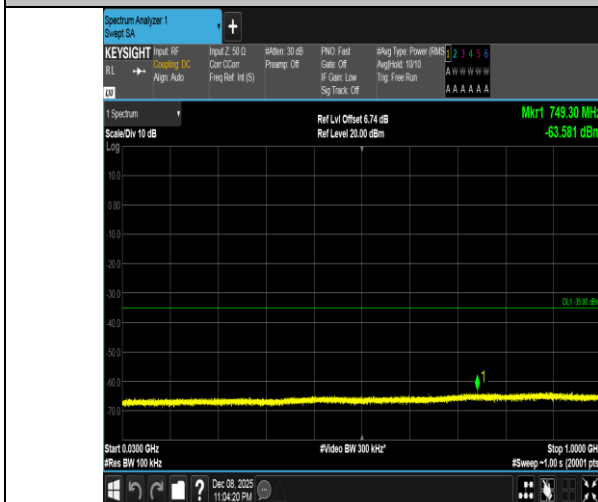
Band41-10MHz-QPSK-40620-1RB#0-30~1000-PASS
