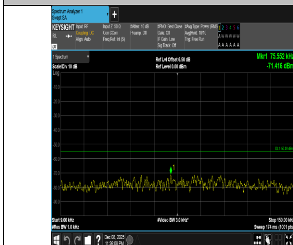
Band41-10MHz-QPSK-41540-1RB#49-0.009~0.15-PASS
