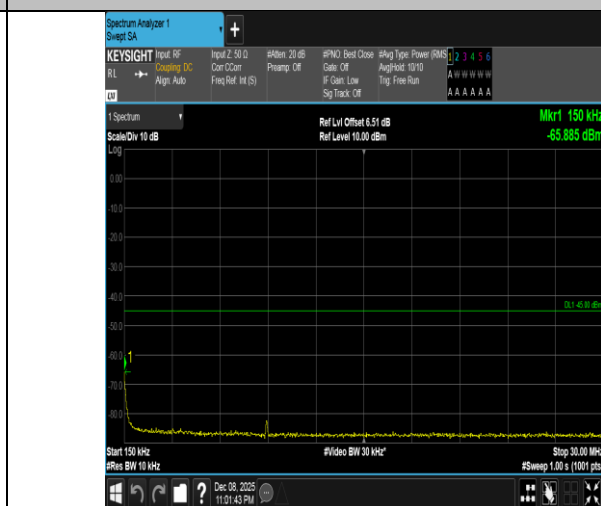
Band41-10MHz-16QAM-39700-50RB#0-0.15~30-PASS
