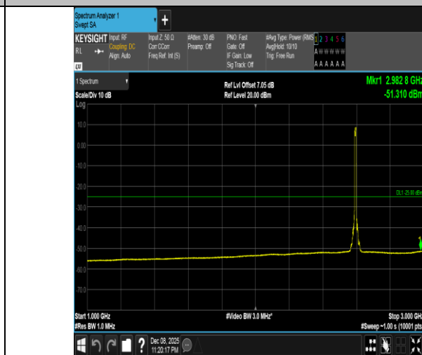
Band41-10MHz-16QAM-40620-50RB#0-1000~3000-PASS
