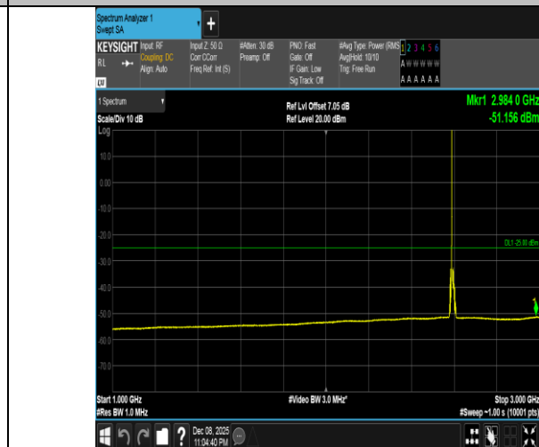
Band41-10MHz-QPSK-40620-1RB#0-1000~3000-PASS
