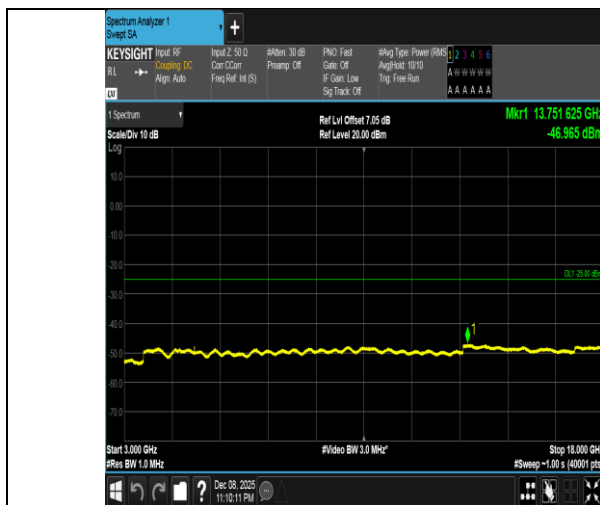
Band41-10MHz-QPSK-40620-1RB#49-3000~18000-PASS
