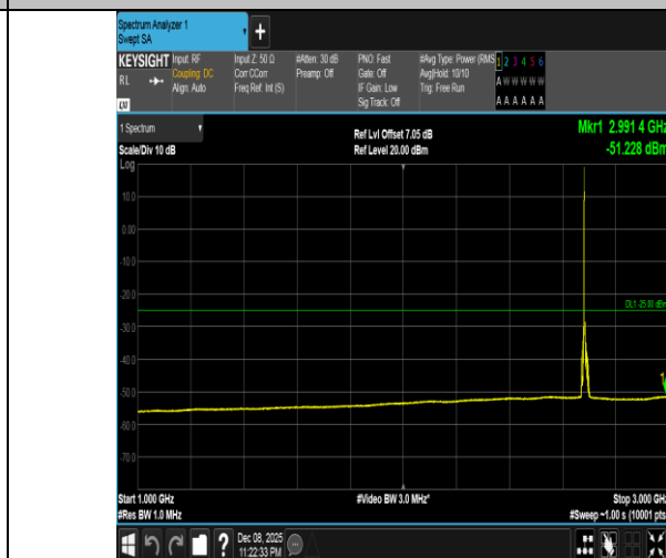
Band41-10MHz-QPSK-41540-1RB#0-1000~3000-PASS
