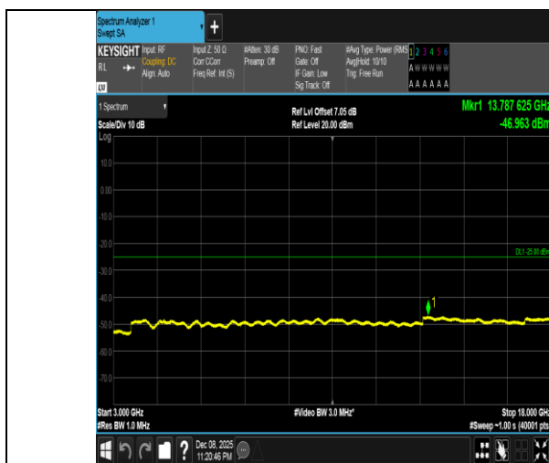
Band41-10MHz-16QAM-40620-50RB#0-3000~18000-PASS
