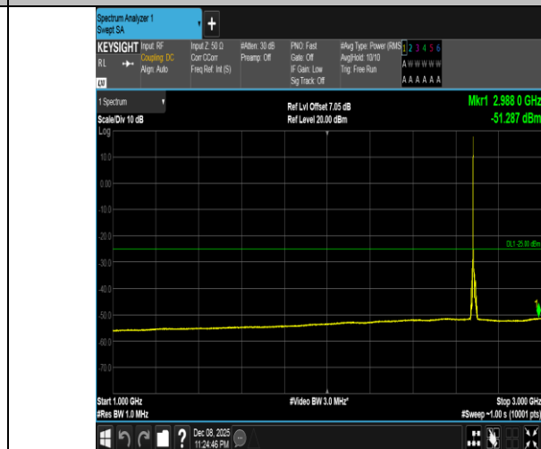
Band41-10MHz-16QAM-41540-1RB#0-1000~3000-PASS
