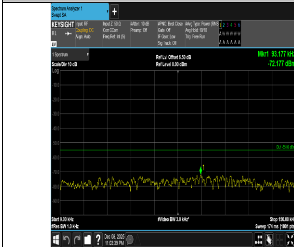
Band41-10MHz-QPSK-40620-1RB#0-0.009~0.15-PASS
