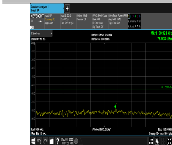
Band41-10MHz-16QAM-39700-50RB#0-0.009~0.15-PASS
