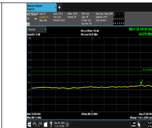
Band41-10MHz-16QAM-40620-50RB#0-18000~27000-PASS
