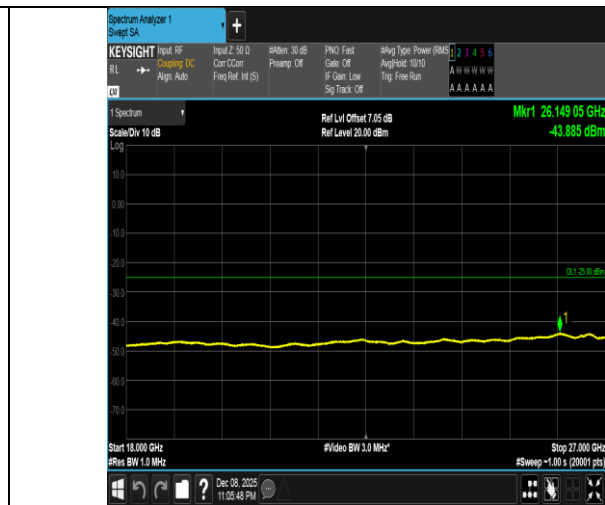
Band41-10MHz-QPSK-40620-1RB#0-18000~27000-PASS
