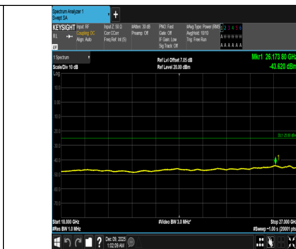
Band41-15MHz-QPSK-41515-1RB#0-18000~27000-PASS
