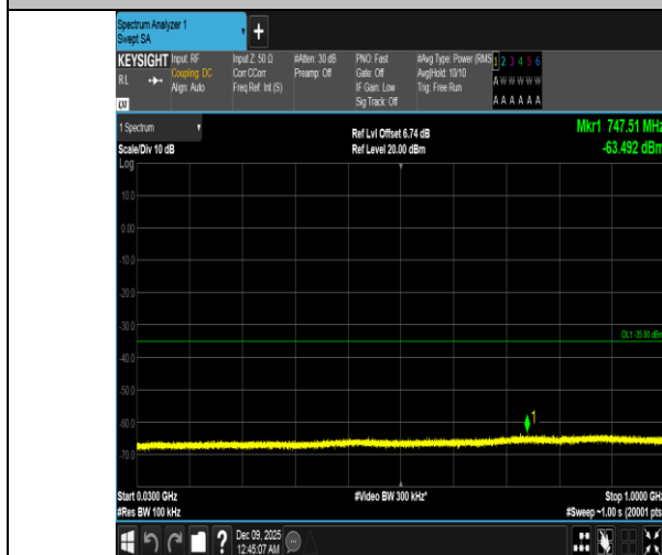
Band41-15MHz-16QAM-40620-1RB#0-30~1000-PASS
