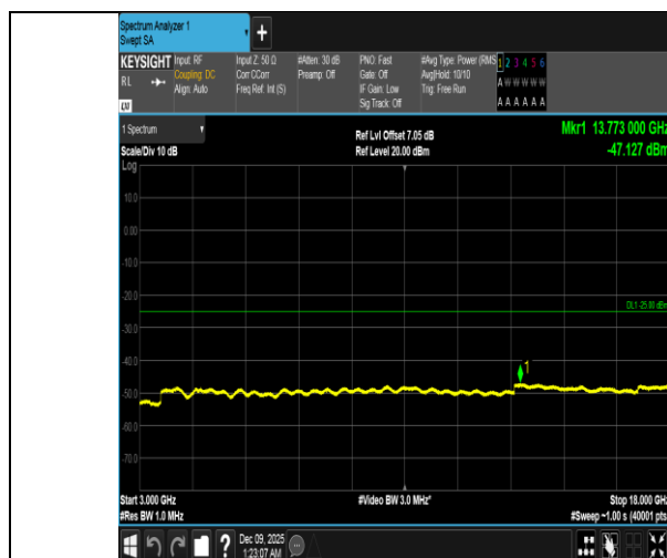
Band41-15MHz-QPSK-41515-75RB#0-3000~18000-PASS
