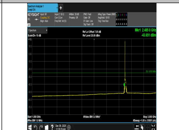
Band41-15MHz-16QAM-39725-1RB#0-1000~3000-PASS
