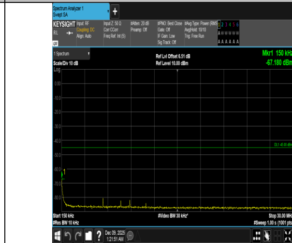
Band41-15MHz-QPSK-41515-75RB#0-0.15~30-PASS
