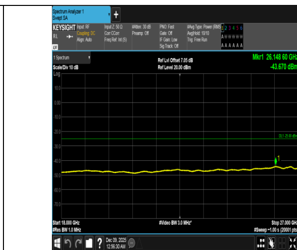
Band41-15MHz-QPSK-40620-75RB#0-18000~27000-PASS
