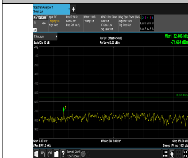
Band41-15MHz-QPSK-40620-1RB#74-0.009~0.15-PASS
