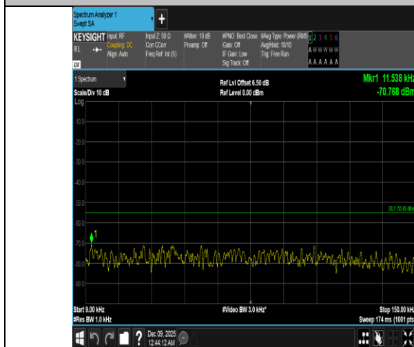
Band41-15MHz-16QAM-40620-1RB#0-0.009~0.15-PASS
