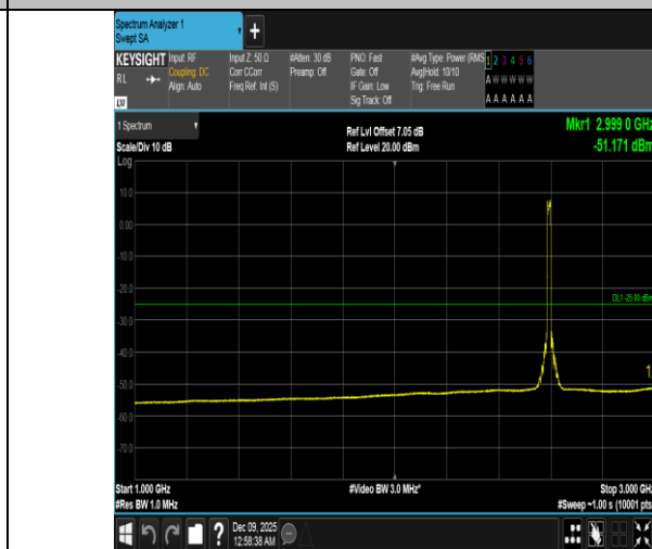
Band41-15MHz-16QAM-40620-75RB#0-1000~3000-PASS
