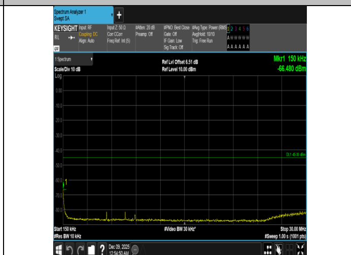
Band41-15MHz-QPSK-40620-75RB#0-0.15~30-PASS
