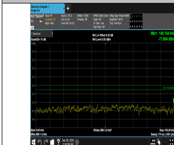
Band41-15MHz-QPSK-40620-1RB#0-0.009~0.15-PASS
