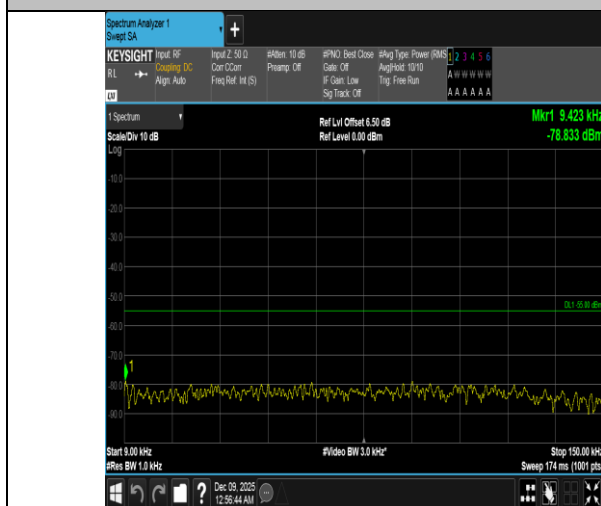
Band41-15MHz-16QAM-40620-75RB#0-0.009~0.15-PASS
