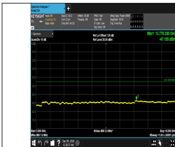
Band41-15MHz-16QAM-39725-1RB#0-3000~18000-PASS
