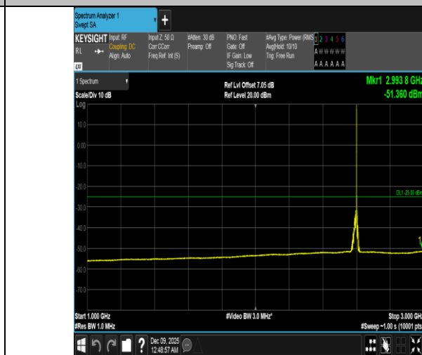
Band41-15MHz-QPSK-40620-1RB#74-1000~3000-PASS
