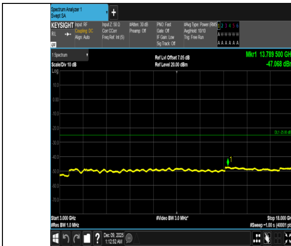
Band41-15MHz-QPSK-41515-1RB#74-3000~18000-PASS
