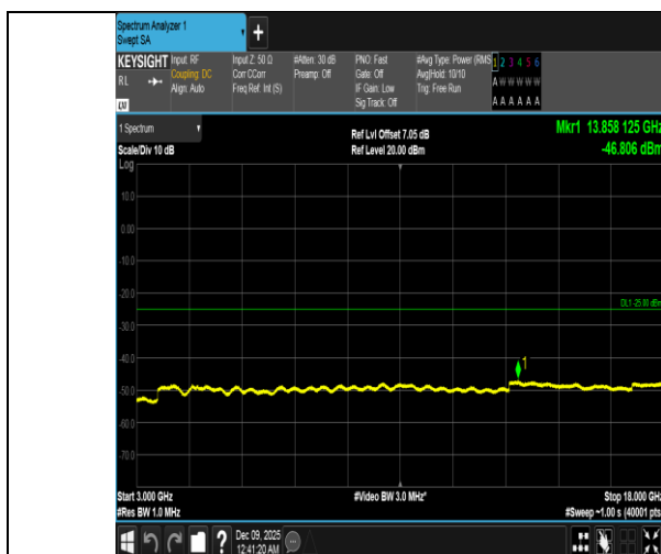
Band41-15MHz-16QAM-39725-75RB#0-3000~18000-PASS
