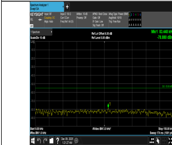
Band41-15MHz-QPSK-41515-75RB#0-0.009~0.15-PASS
