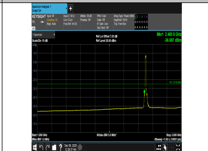
Band41-15MHz-QPSK-39725-75RB#0-1000~3000-PASS
