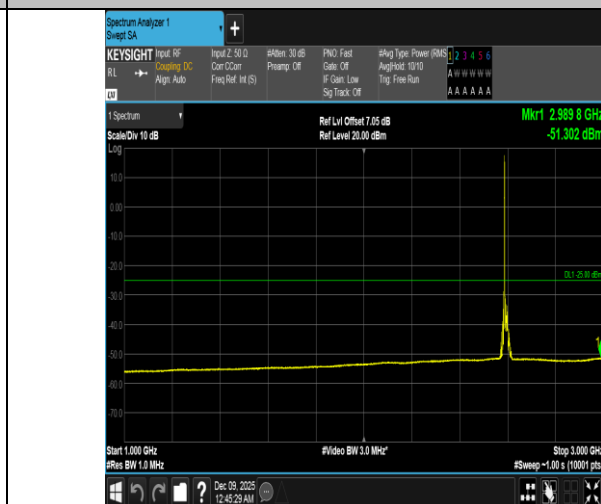
Band41-15MHz-16QAM-40620-1RB#0-1000~3000-PASS
