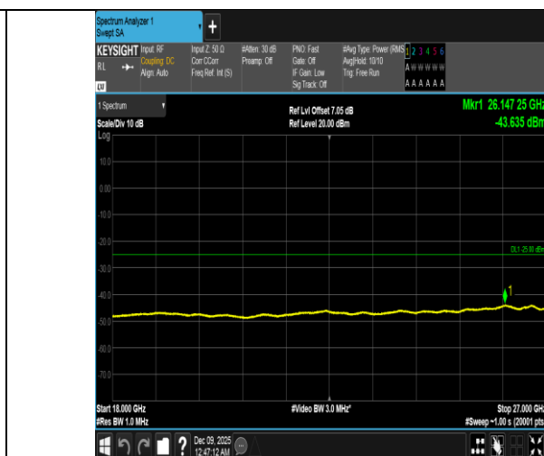
Band41-15MHz-16QAM-40620-1RB#0-18000~27000-PASS
