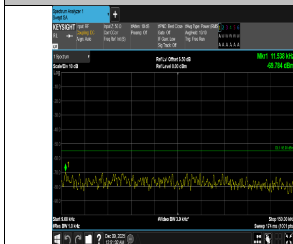
Band41-15MHz-16QAM-40620-1RB#74-0.009~0.15-PASS
