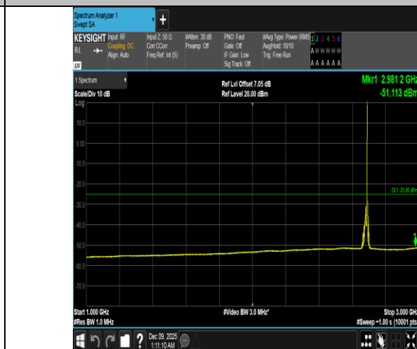
Band41-15MHz-QPSK-41515-1RB#74-1000~3000-PASS
