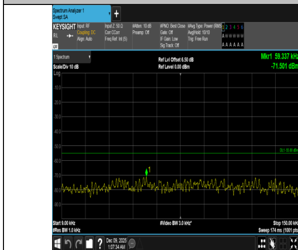
Band41-15MHz-QPSK-41515-1RB#74-0.009~0.15-PASS
