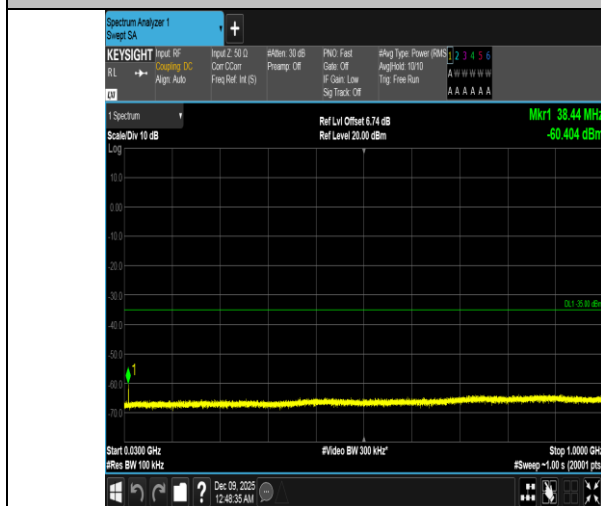
Band41-15MHz-QPSK-40620-1RB#74-30~1000-PASS
