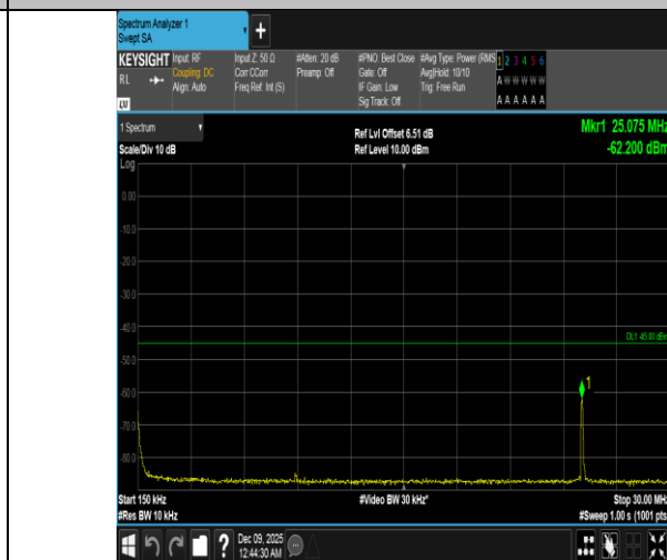
Band41-15MHz-16QAM-40620-1RB#0-0.15~30-PASS
