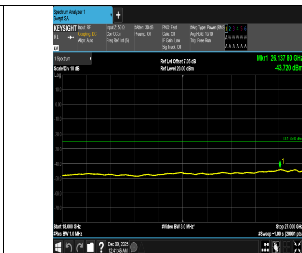
Band41-15MHz-16QAM-39725-75RB#0-18000~27000-PASS
