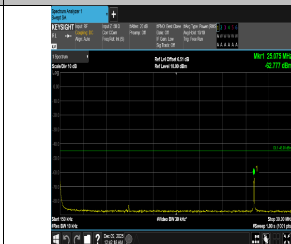
Band41-15MHz-QPSK-40620-1RB#0-0.15~30-PASS
