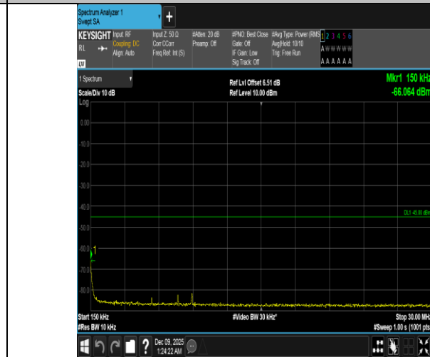
Band41-15MHz-16QAM-41515-75RB#0-0.15~30-PASS
