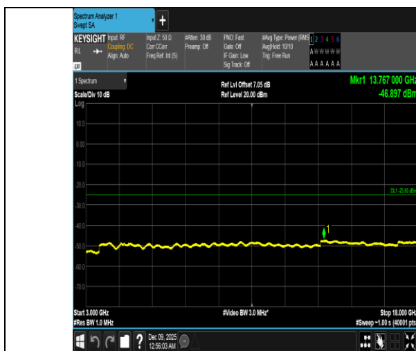
Band41-15MHz-QPSK-40620-75RB#0-3000~18000-PASS
