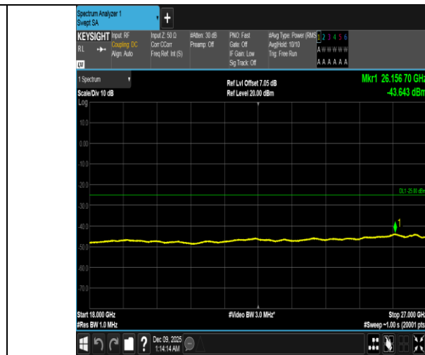
Band41-15MHz-QPSK-41515-1RB#74-18000~27000-PASS
