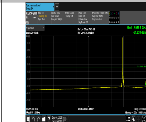
Band41-15MHz-QPSK-40620-1RB#0-1000~3000-PASS
