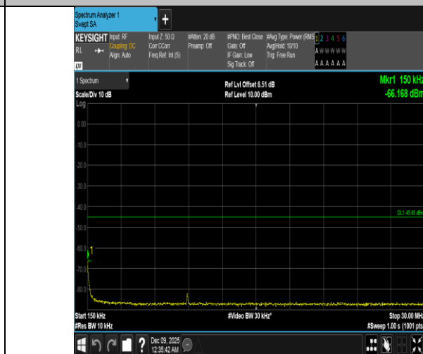
Band41-15MHz-16QAM-39725-1RB#74-0.15~30-PASS
