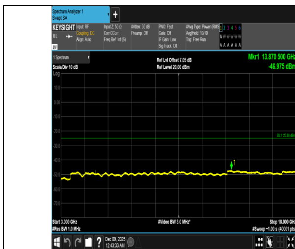
Band41-15MHz-QPSK-40620-1RB#0-3000~18000-PASS
