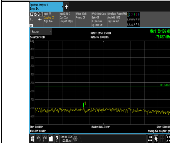
Band41-15MHz-16QAM-41515-75RB#0-0.009~0.15-PASS
