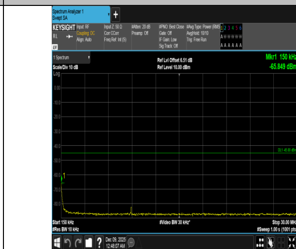
Band41-15MHz-QPSK-40620-1RB#74-0.15~30-PASS
