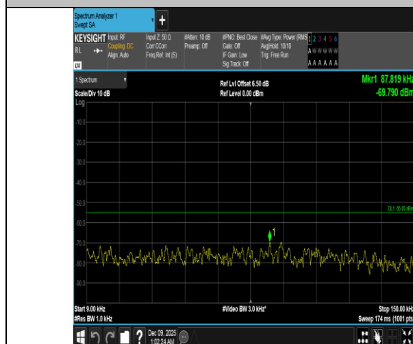
Band41-15MHz-16QAM-41515-1RB#0-0.009~0.15-PASS
