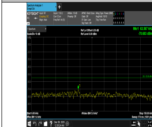
Band41-15MHz-16QAM-39725-1RB#74-0.009~0.15-PASS
