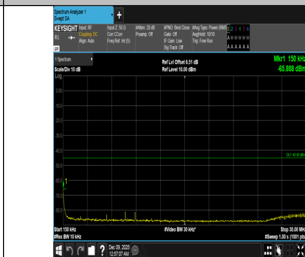
Band41-15MHz-16QAM-40620-75RB#0-0.15~30-PASS
