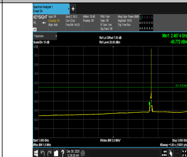
Band41-15MHz-16QAM-39725-1RB#74-1000~3000-PASS
