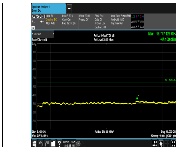
Band41-15MHz-16QAM-40620-1RB#0-3000~18000-PASS
