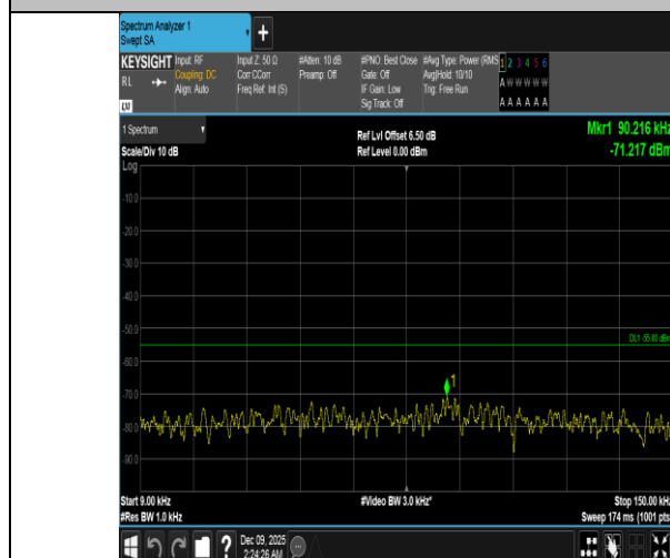
Band41-20MHz-QPSK-39750-1RB#99-0.009~0.15-PASS
