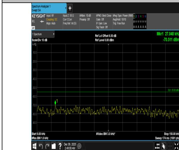
Band41-20MHz-16QAM-41490-1RB#0-0.009~0.15-PASS
