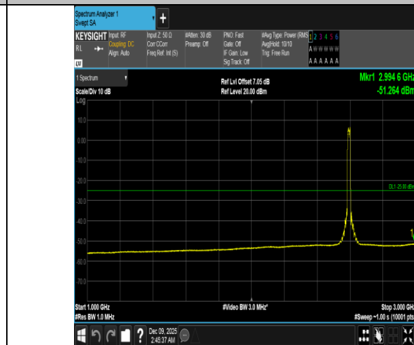
Band41-20MHz-16QAM-40620-100RB#0-1000~3000-PASS
