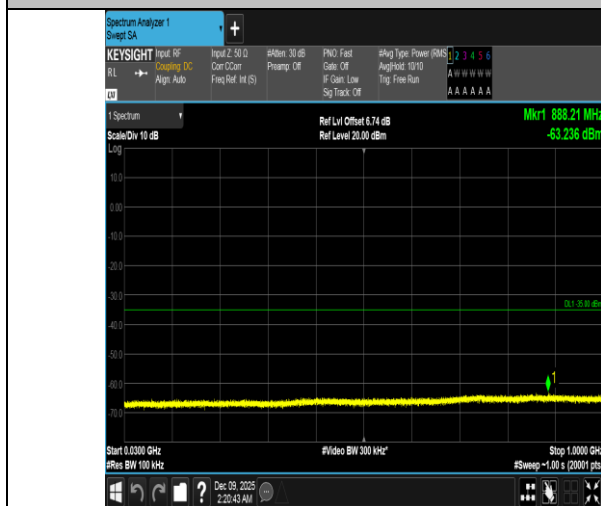
Band41-20MHz-QPSK-39750-1RB#0-30~1000-PASS
