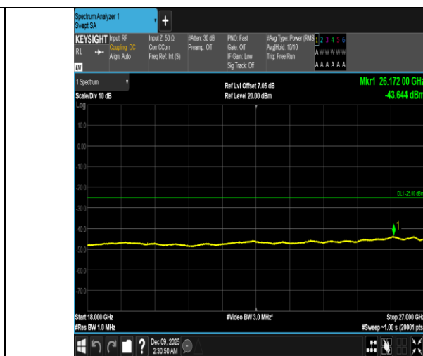
Band41-20MHz-QPSK-39750-100RB#0-18000~27000-PASS
