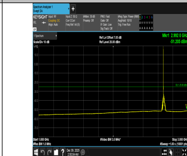
Band41-20MHz-16QAM-41490-1RB#0-1000~3000-PASS
