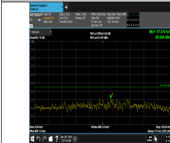
Band41-20MHz-QPSK-40620-1RB#99-0.009~0.15-PASS
