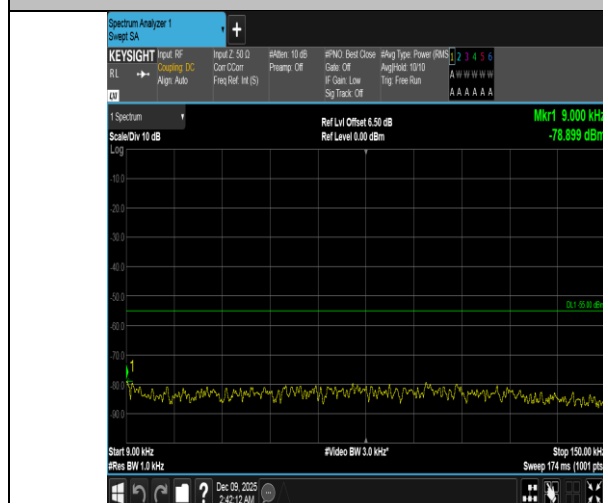
Band41-20MHz-QPSK-40620-100RB#0-0.009~0.15-PASS
