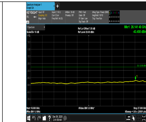
Band41-20MHz-16QAM-40620-1RB#99-18000~27000-PASS
