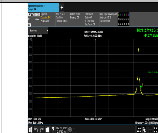
Band41-20MHz-QPSK-41490-100RB#0-1000~3000-PASS
