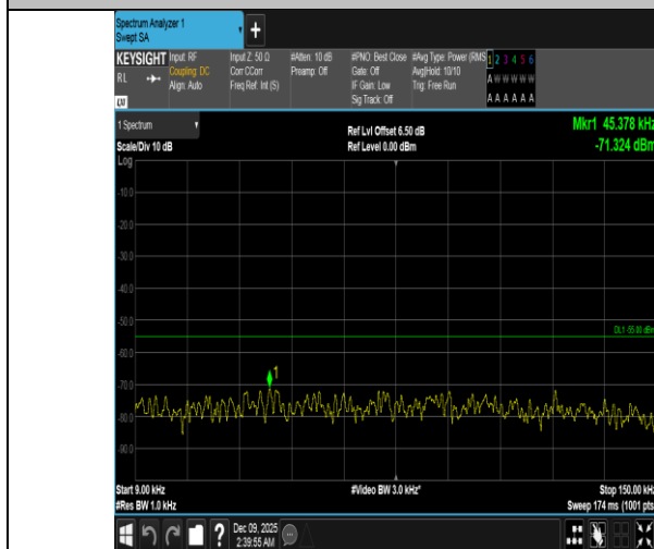
Band41-20MHz-16QAM-40620-1RB#99-0.009~0.15-PASS
