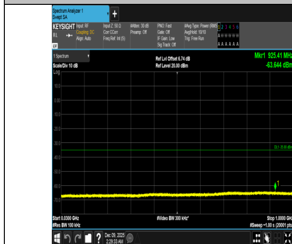
Band41-20MHz-QPSK-39750-100RB#0-30~1000-PASS
