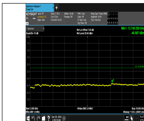
Band41-20MHz-QPSK-40620-1RB#99-3000~18000-PASS
