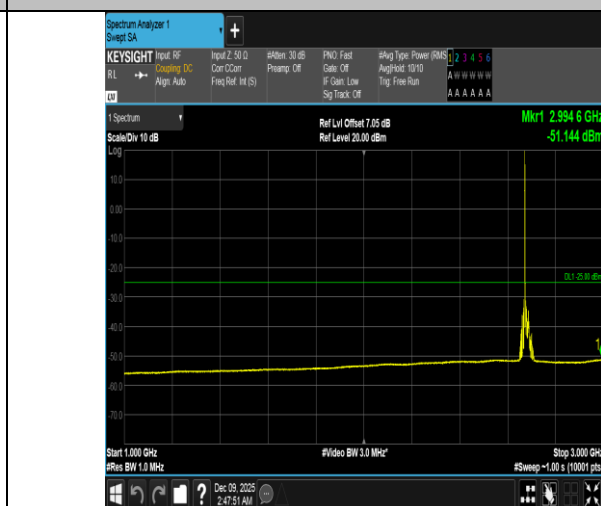
Band41-20MHz-QPSK-41490-1RB#0-1000~3000-PASS
