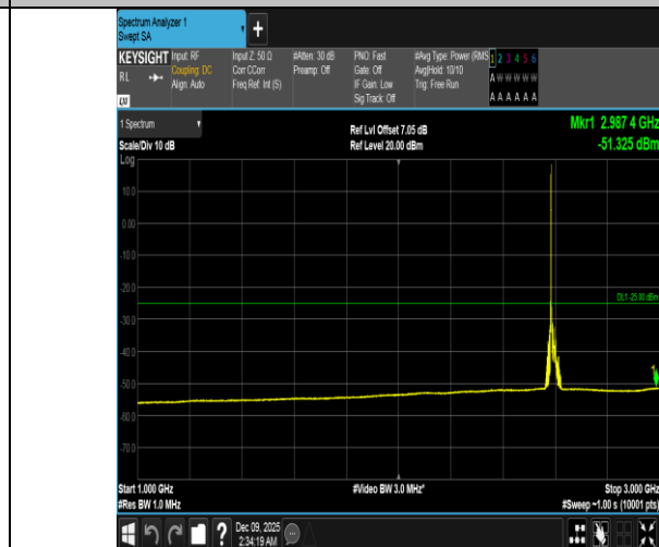
Band41-20MHz-QPSK-40620-1RB#0-1000~3000-PASS
