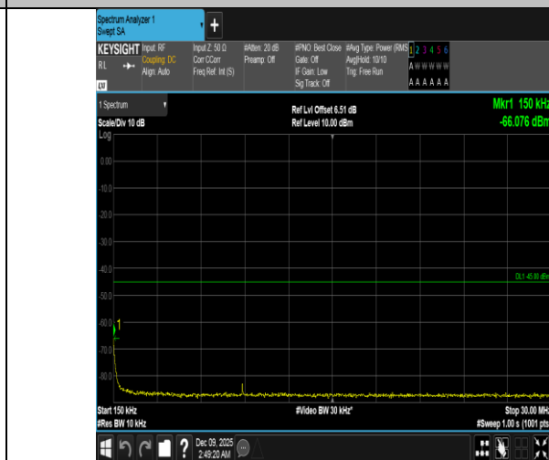
Band41-20MHz-16QAM-41490-1RB#0-0.15~30-PASS
