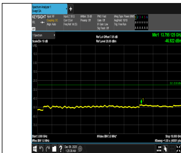
Band41-15MHz-16QAM-41515-75RB#0-3000~18000-PASS
