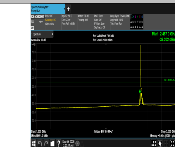
Band41-20MHz-16QAM-39750-1RB#0-1000~3000-PASS
