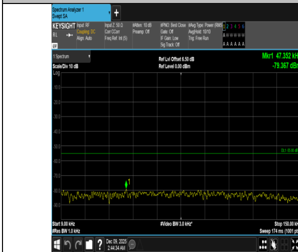
Band41-20MHz-16QAM-40620-100RB#0-0.009~0.15-PASS
