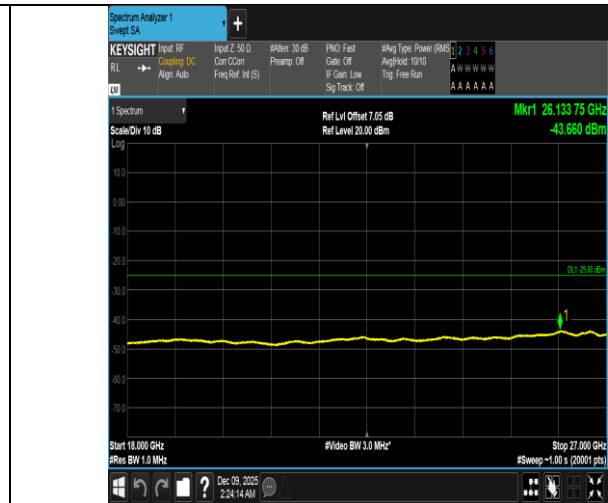
Band41-20MHz-16QAM-39750-1RB#0-18000~27000-PASS
