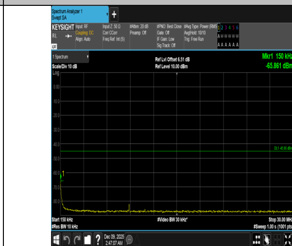
Band41-20MHz-QPSK-41490-1RB#0-0.15~30-PASS
