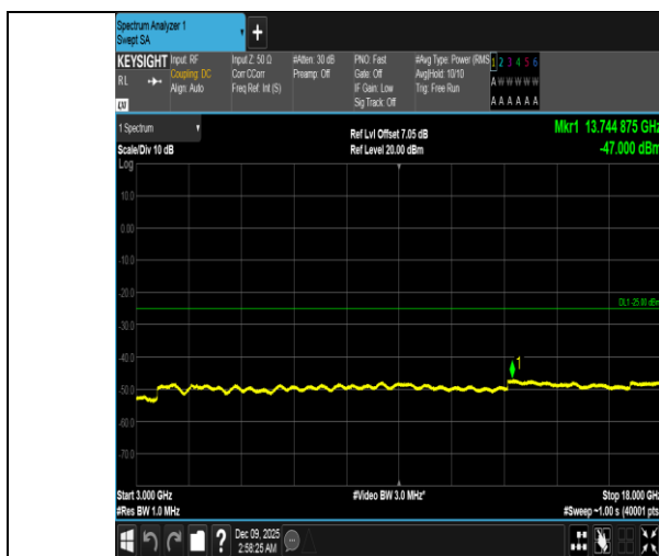
Band41-20MHz-QPSK-41490-100RB#0-3000~18000-PASS
