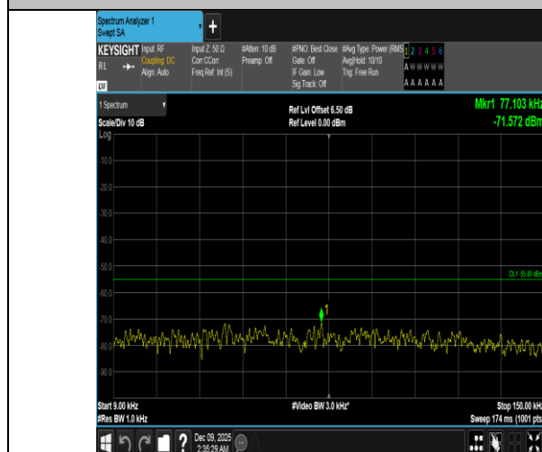
Band41-20MHz-16QAM-40620-1RB#0-0.009~0.15-PASS
