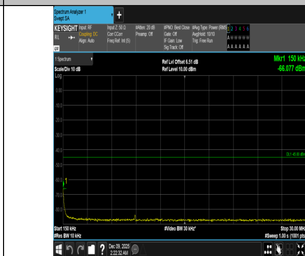
Band41-20MHz-16QAM-39750-1RB#0-0.15~30-PASS
