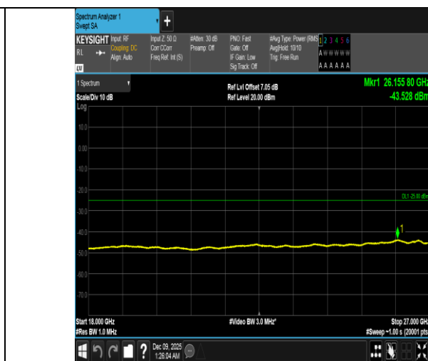
Band41-15MHz-16QAM-41515-75RB#0-18000~27000-PASS
