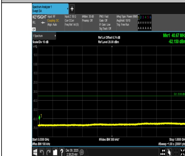
Band41-20MHz-QPSK-40620-1RB#99-30~1000-PASS
