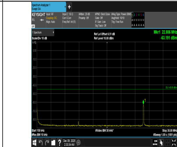
Band41-20MHz-QPSK-40620-1RB#0-0.15~30-PASS
