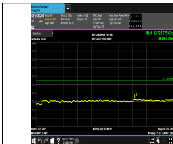
Band41-20MHz-QPSK-39750-1RB#99-3000~18000-PASS
