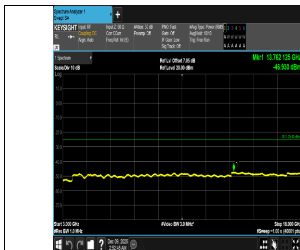
Band41-20MHz-QPSK-41490-1RB#99-3000~18000-PASS
