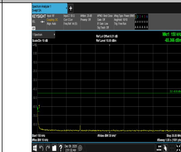
Band41-20MHz-QPSK-41490-1RB#99-0.15~30-PASS
