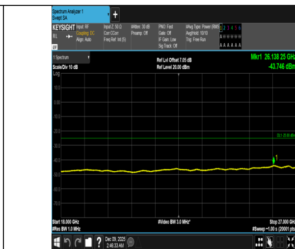
Band41-20MHz-16QAM-40620-100RB#0-18000~27000-PASS
