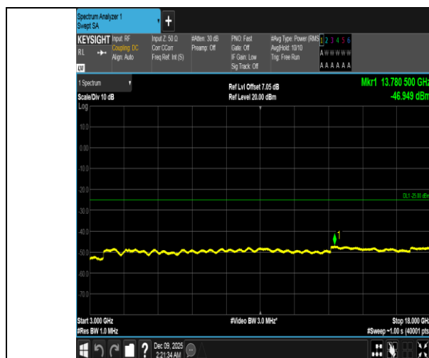
Band41-20MHz-QPSK-39750-1RB#0-3000~18000-PASS
