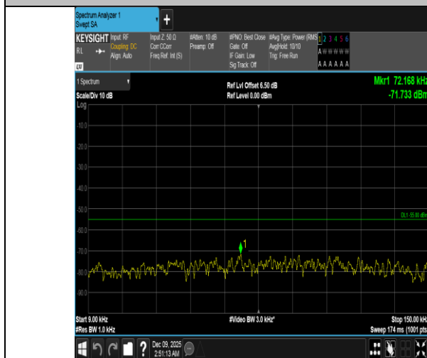
Band41-20MHz-QPSK-41490-1RB#99-0.009~0.15-PASS
