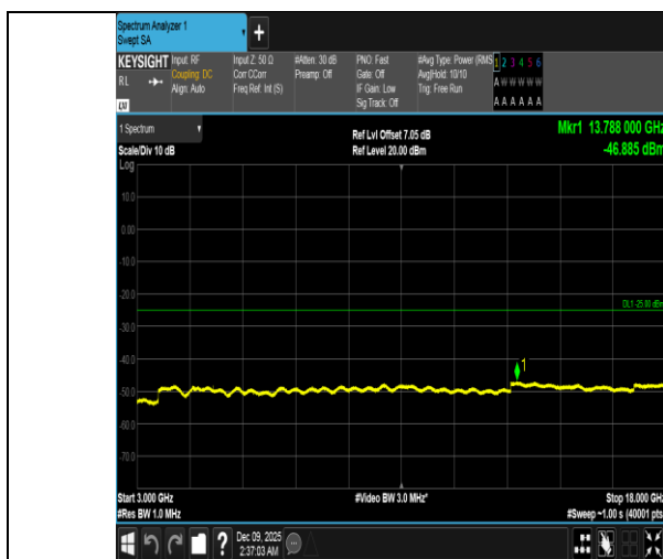
Band41-20MHz-16QAM-40620-1RB#0-3000~18000-PASS
