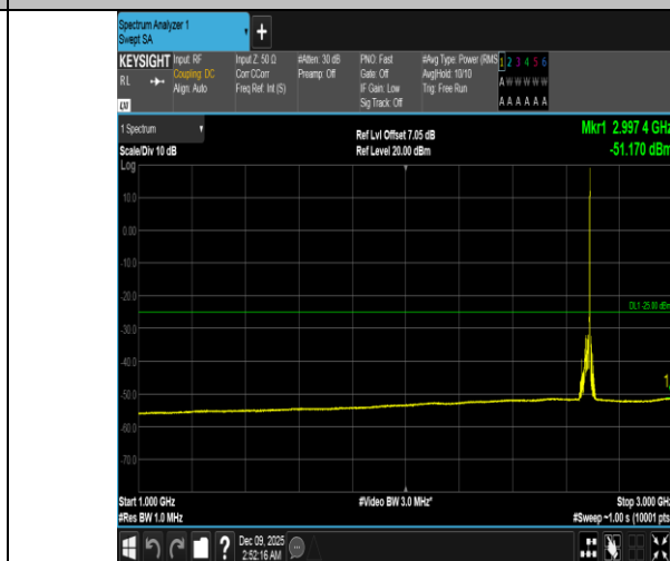
Band41-20MHz-QPSK-41490-1RB#99-1000~3000-PASS
