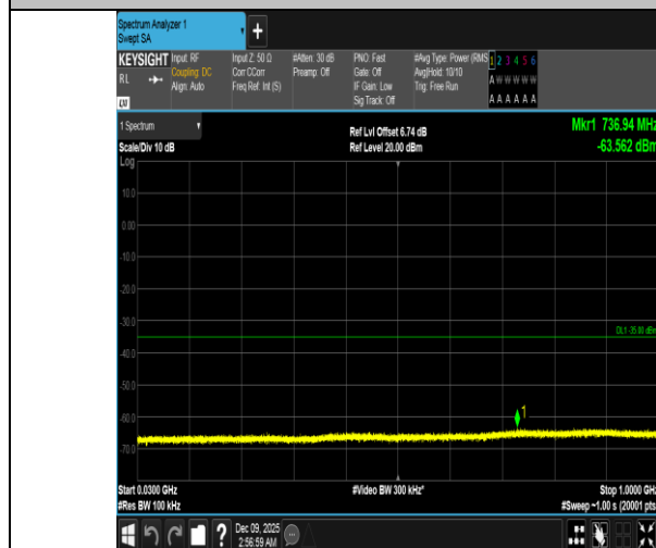
Band41-20MHz-QPSK-41490-100RB#0-30~1000-PASS
