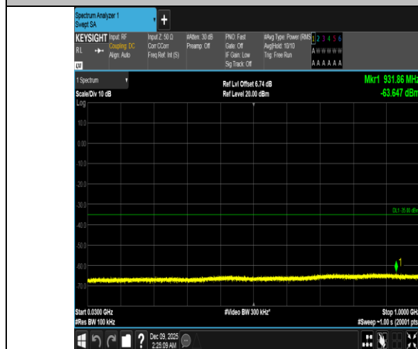
Band41-20MHz-QPSK-39750-1RB#99-30~1000-PASS
