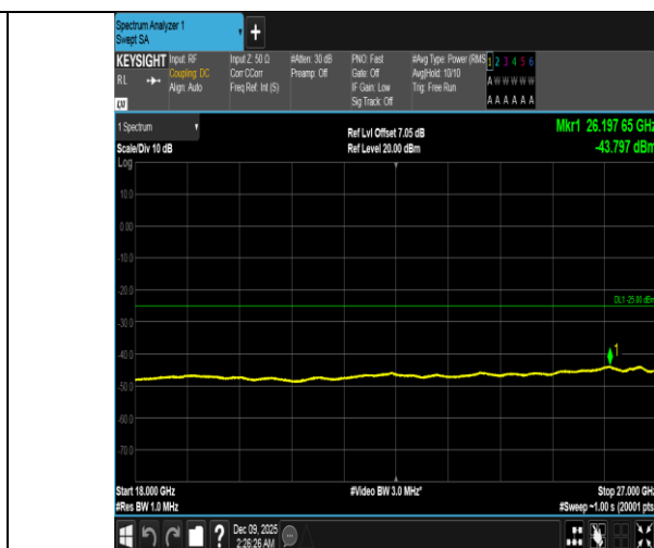
Band41-20MHz-QPSK-39750-1RB#99-18000~27000-PASS
