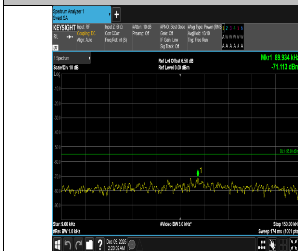
Band41-20MHz-QPSK-39750-1RB#0-0.009~0.15-PASS
