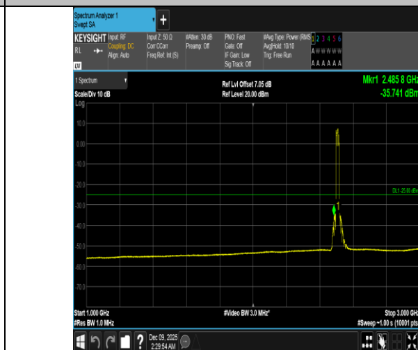
Band41-20MHz-QPSK-39750-100RB#0-1000~3000-PASS
