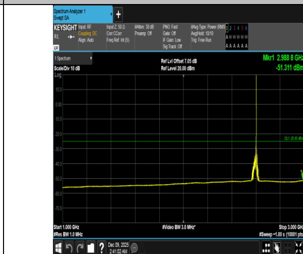
Band41-20MHz-16QAM-40620-1RB#99-1000~3000-PASS
