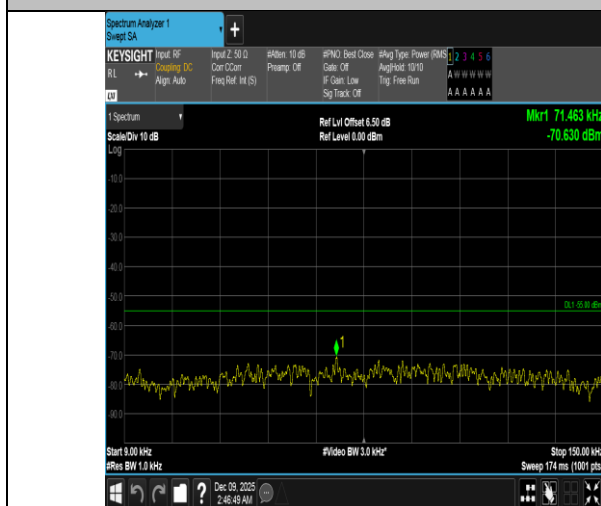
Band41-20MHz-QPSK-41490-1RB#0-0.009~0.15-PASS
