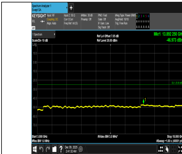
Band41-20MHz-16QAM-40620-1RB#99-3000~18000-PASS
