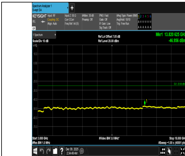
Band41-20MHz-QPSK-40620-1RB#0-3000~18000-PASS
