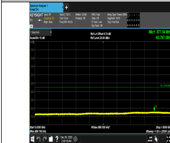
Band41-20MHz-16QAM-40620-100RB#0-30~1000-PASS
