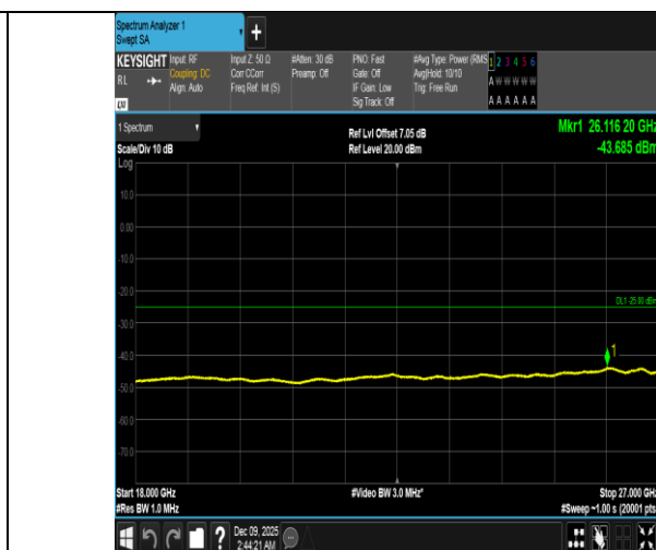
Band41-20MHz-QPSK-40620-100RB#0-18000~27000-PASS
