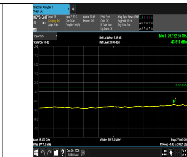
Band41-20MHz-QPSK-41490-100RB#0-18000~27000-PASS
