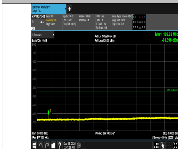
Band41-20MHz-QPSK-41490-1RB#0-30~1000-PASS
