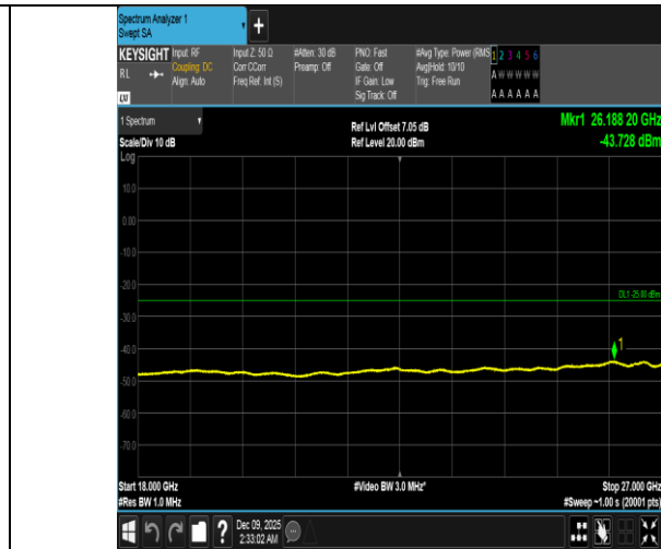
Band41-20MHz-16QAM-39750-100RB#0-18000~27000-PASS
