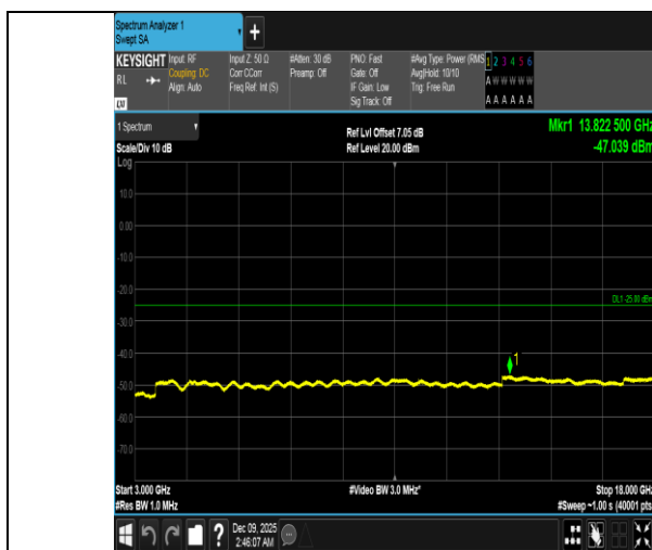
Band41-20MHz-16QAM-40620-100RB#0-3000~18000-PASS
