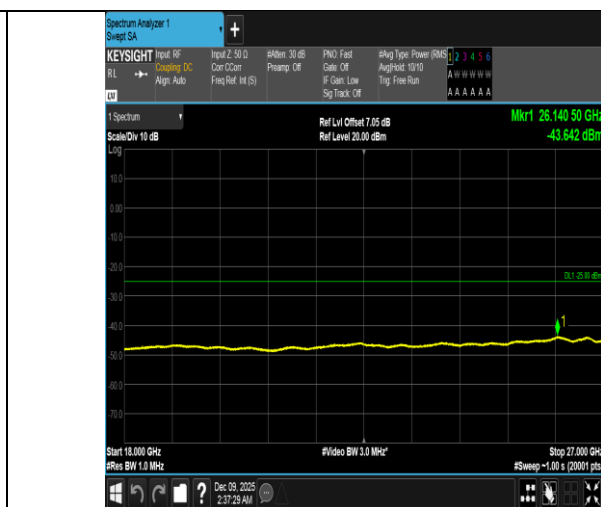
Band41-20MHz-16QAM-40620-1RB#0-18000~27000-PASS
