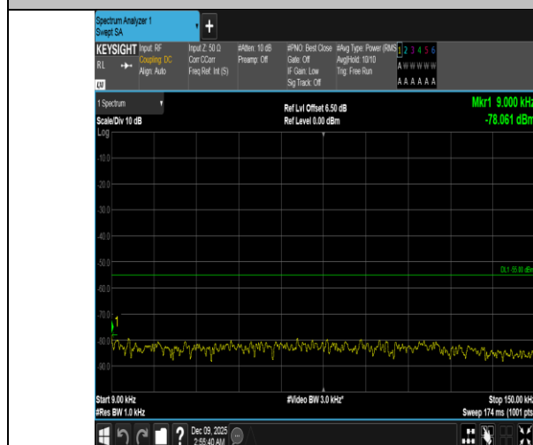
Band41-20MHz-QPSK-41490-100RB#0-0.009~0.15-PASS
