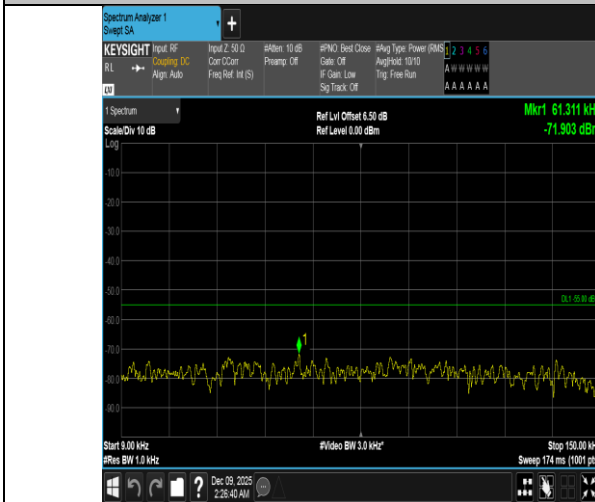
Band41-20MHz-16QAM-39750-1RB#99-0.009~0.15-PASS
