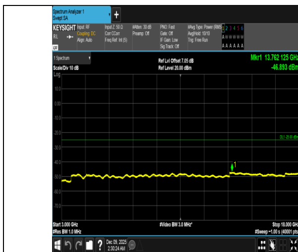
Band41-20MHz-QPSK-39750-100RB#0-3000~18000-PASS
