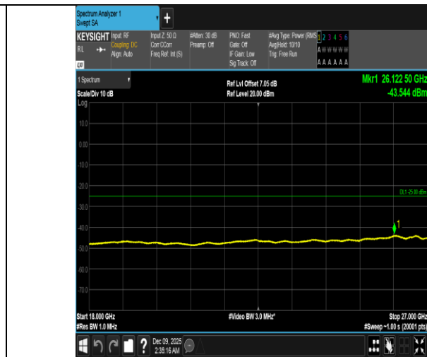
Band41-20MHz-QPSK-40620-1RB#0-18000~27000-PASS
