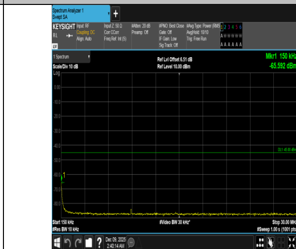
Band41-20MHz-16QAM-40620-1RB#99-0.15~30-PASS
