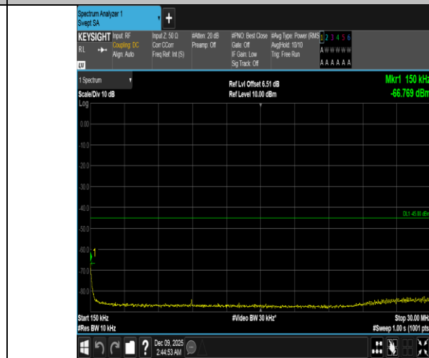
Band41-20MHz-16QAM-40620-100RB#0-0.15~30-PASS
