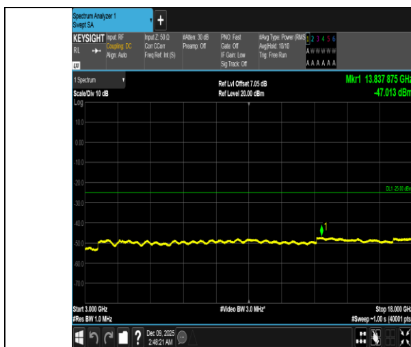
Band41-20MHz-QPSK-41490-1RB#0-3000~18000-PASS
