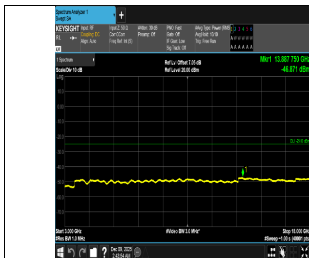
Band41-20MHz-QPSK-40620-100RB#0-3000~18000-PASS
