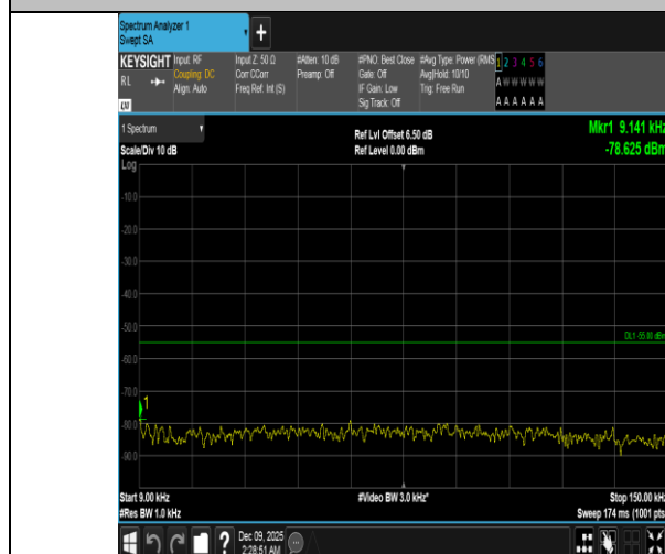
Band41-20MHz-QPSK-39750-100RB#0-0.009~0.15-PASS
