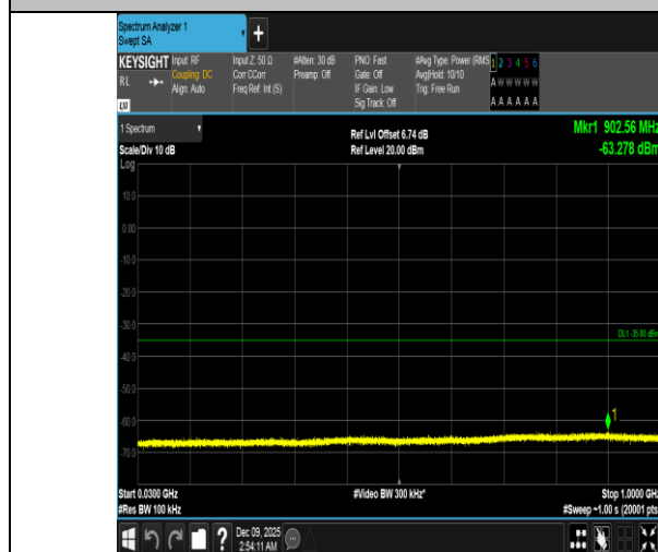
Band41-20MHz-16QAM-41490-1RB#99-30~1000-PASS
