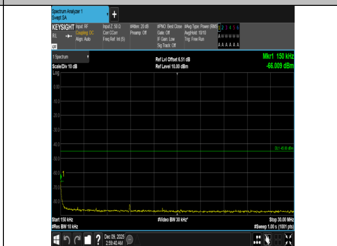
Band41-20MHz-16QAM-41490-100RB#0-0.15~30-PASS
