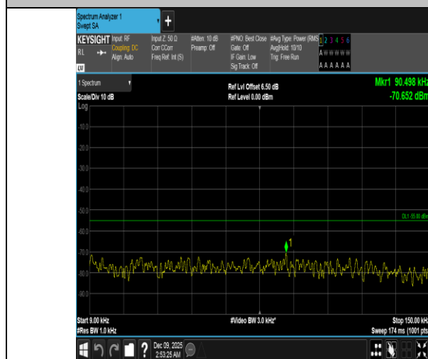
Band41-20MHz-16QAM-41490-1RB#99-0.009~0.15-PASS
