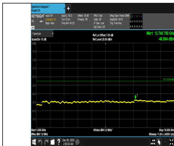
Band41-20MHz-16QAM-41490-1RB#0-3000~18000-PASS
