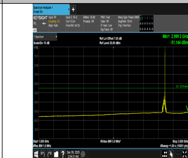
Band41-20MHz-16QAM-41490-1RB#99-1000~3000-PASS
