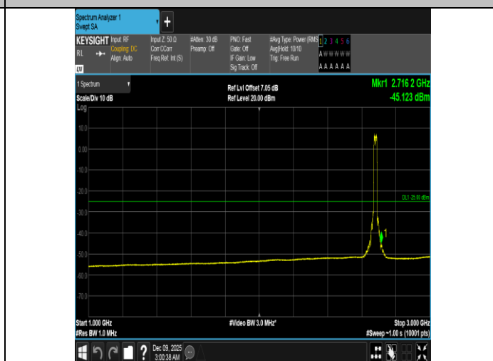
Band41-20MHz-16QAM-41490-100RB#0-1000~3000-PASS
