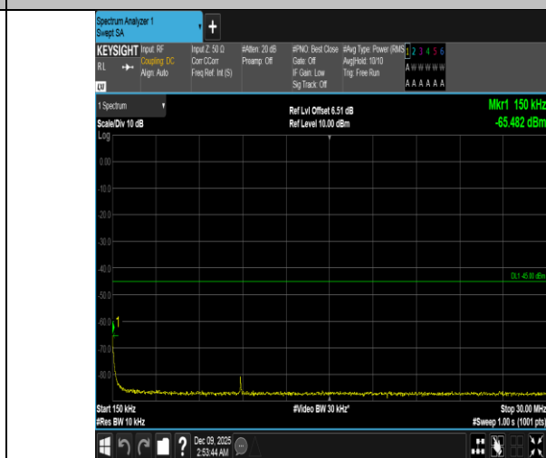
Band41-20MHz-16QAM-41490-1RB#99-0.15~30-PASS
