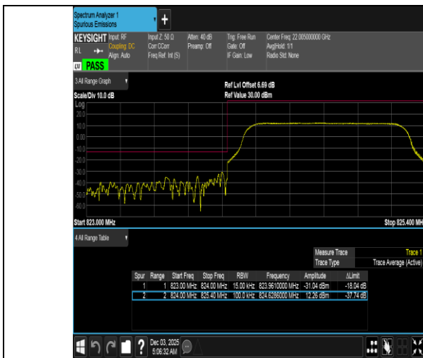
Band5-1.4MHz-QPSK-20407-6RB#0-PASS
