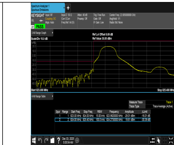
Band5-1.4MHz-16QAM-20407-1RB#0-PASS
