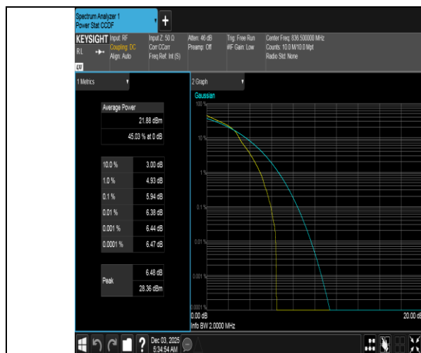
Band5-1.4MHz-16QAM-20525-1RB#0-PASS
