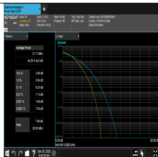
Band5-5MHz-16QAM-20525-25RB#0-PASS
