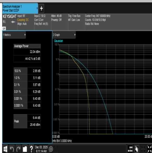
Band5-3MHz-16QAM-20635-1RB#0-PASS
