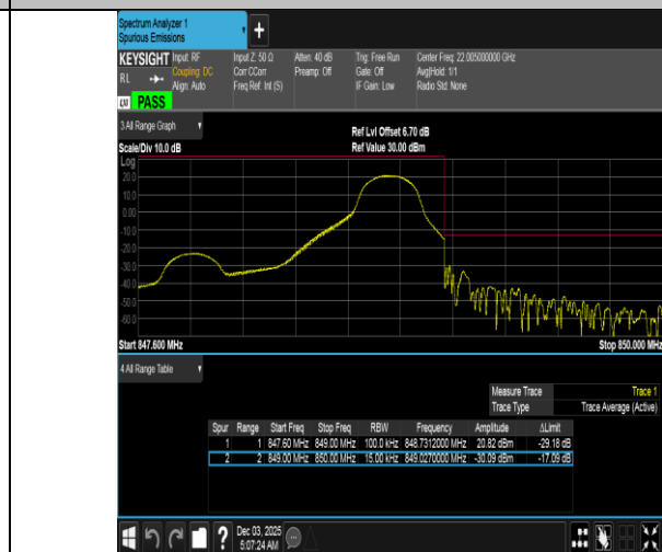
Band5-1.4MHz-QPSK-20643-1RB#5-PASS
