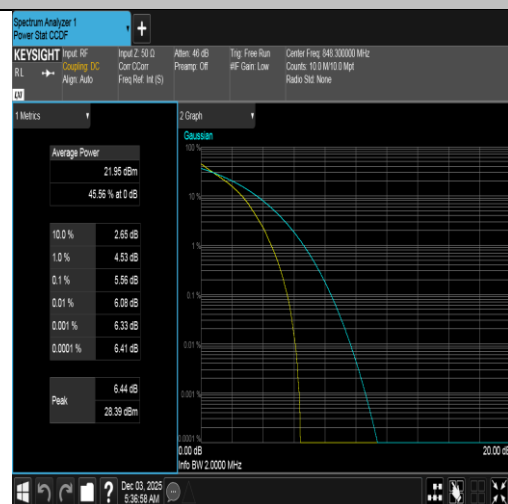
Band5-1.4MHz-QPSK-20643-6RB#0-PASS
