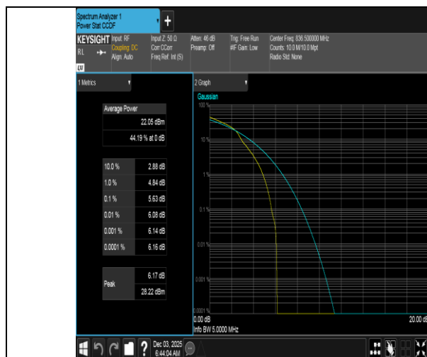
Band5-5MHz-16QAM-20525-1RB#0-PASS
