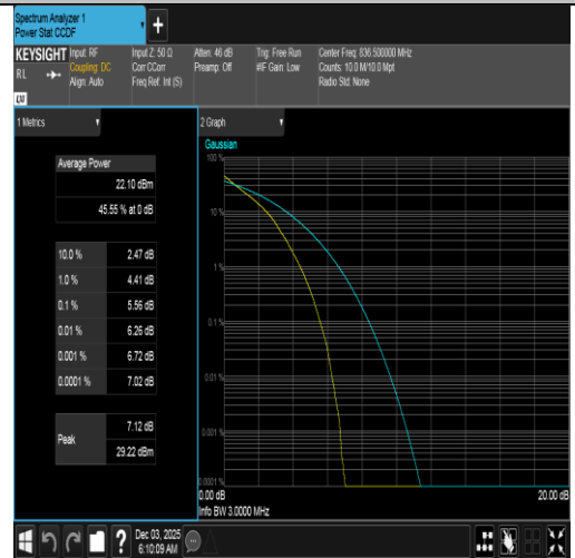
Band5-3MHz-QPSK-20525-15RB#0-PASS
