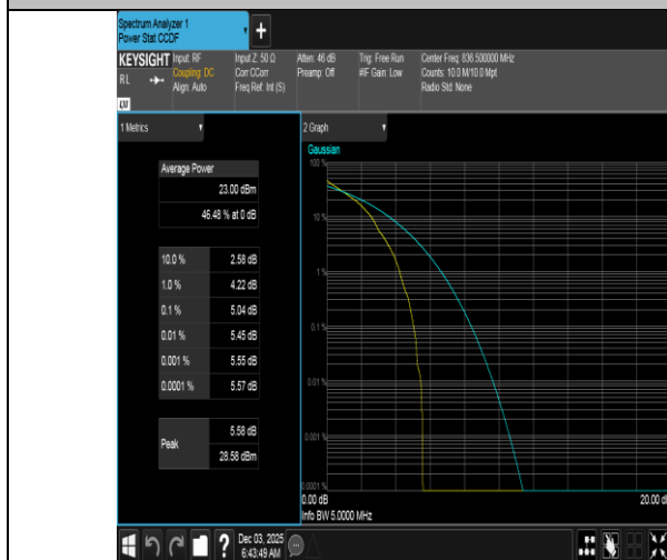
Band5-5MHz-QPSK-20525-1RB#0-PASS
