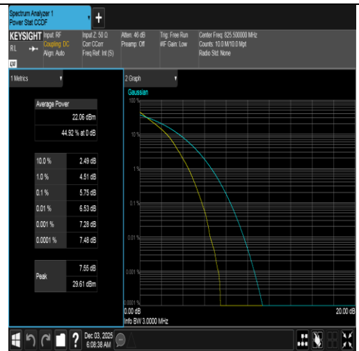
Band5-3MHz-QPSK-20415-15RB#0-PASS
