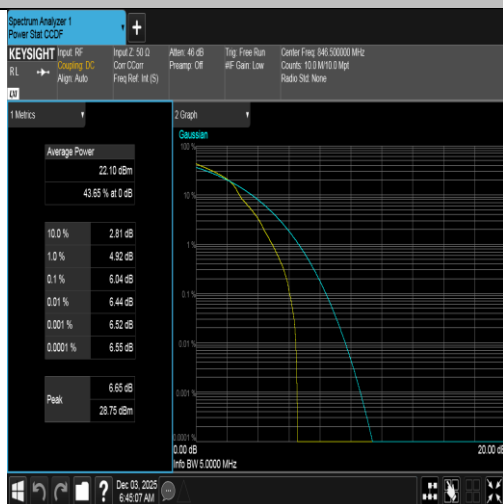
Band5-5MHz-16QAM-20625-1RB#0-PASS
