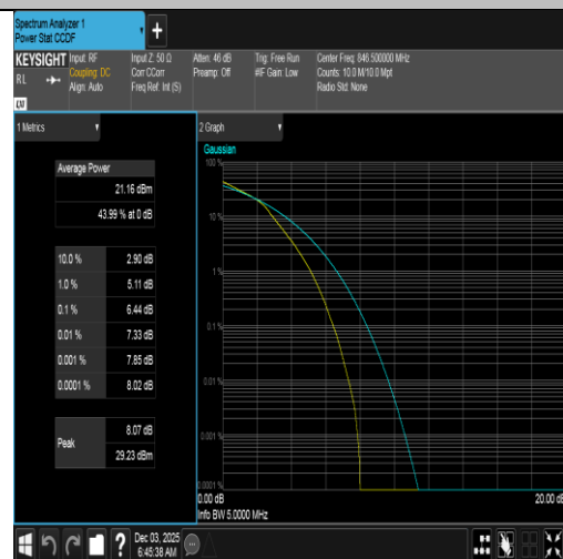
Band5-5MHz-16QAM-20625-25RB#0-PASS
