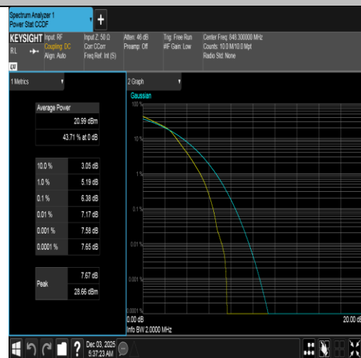
Band5-1.4MHz-16QAM-20643-6RB#0-PASS
