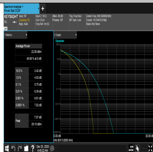
Band5-5MHz-QPSK-20625-25RB#0-PASS
