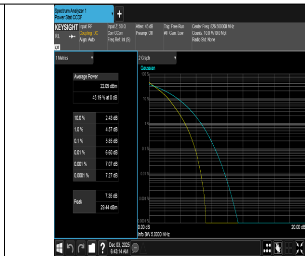
Band5-5MHz-QPSK-20425-25RB#0-PASS
