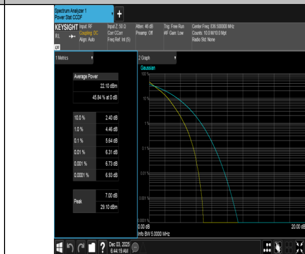
Band5-5MHz-QPSK-20525-25RB#0-PASS
