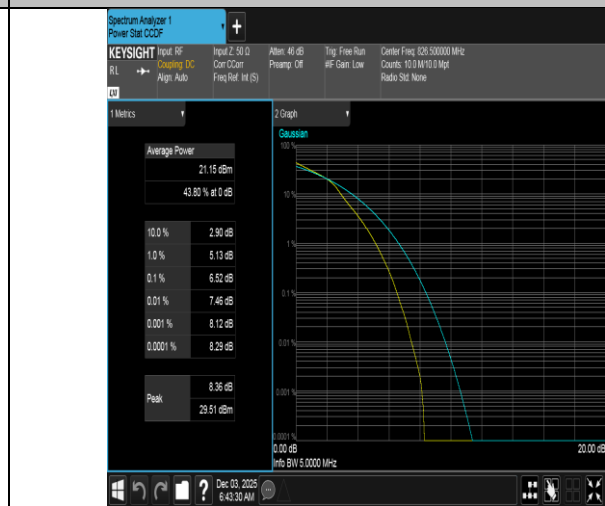
Band5-5MHz-16QAM-20425-25RB#0-PASS
