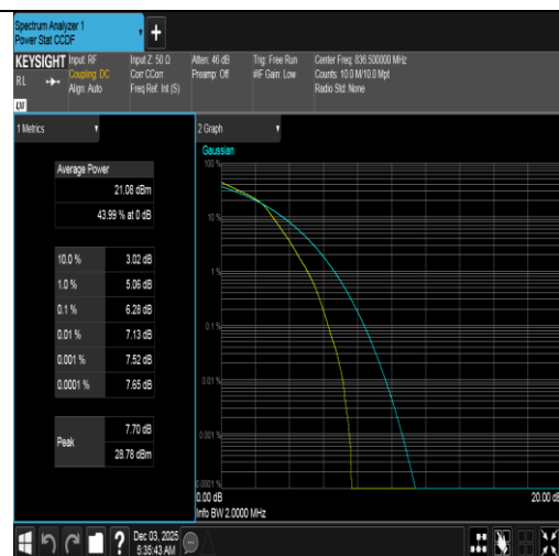
Band5-1.4MHz-16QAM-20525-6RB#0-PASS
