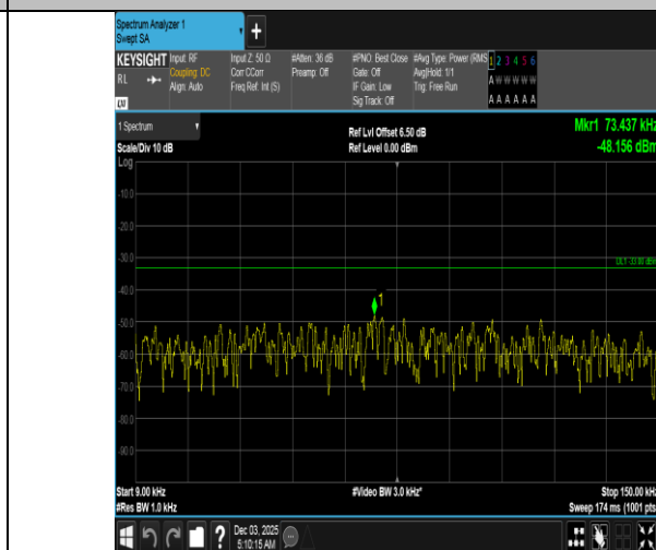
Band5-1.4MHz-QPSK-20407-1RB#5-0.009~0.15-PASS
