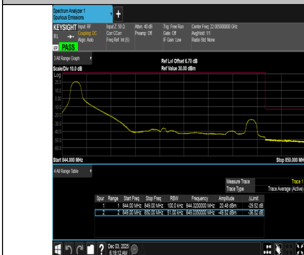
Band5-5MHz-QPSK-20625-1RB#0-PASS
