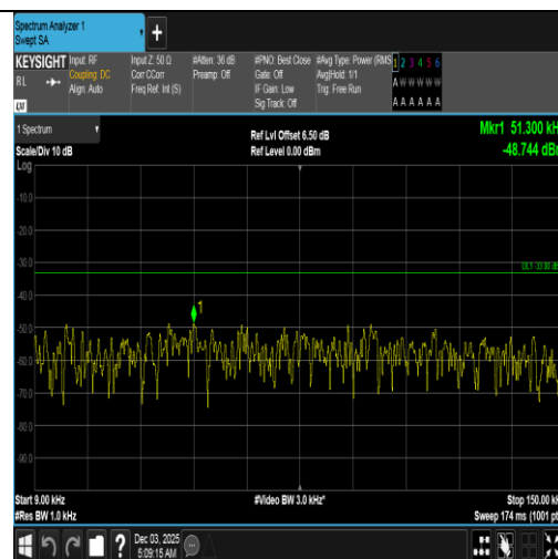
Band5-1.4MHz-16QAM-20407-1RB#0-0.009~0.15-PASS
