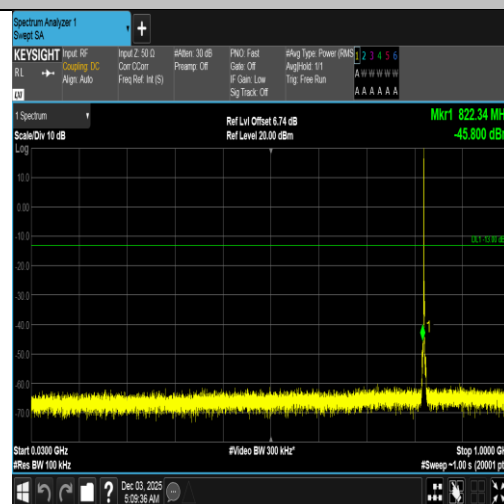
Band5-1.4MHz-16QAM-20407-1RB#0-30~1000-PASS
