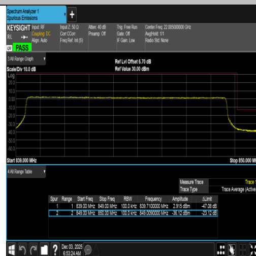
Band5-10MHz-16QAM-20600-50RB#0-PASS
