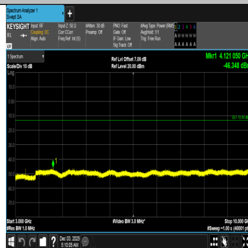
Band5-1.4MHz-16QAM-20407-1RB#0-3000~10000-PASS
