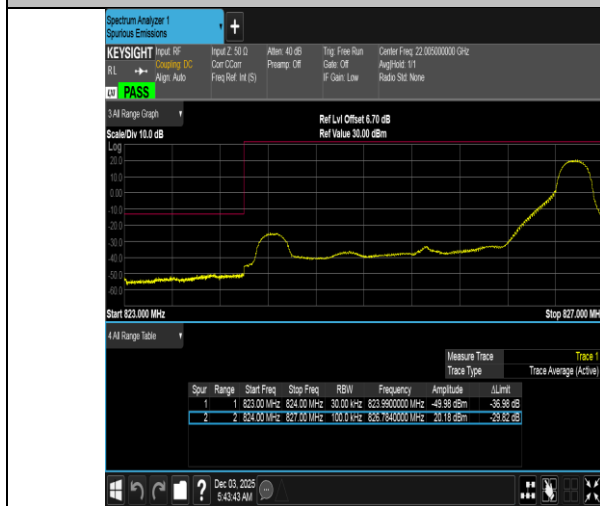
Band5-3MHz-16QAM-20415-1RB#14-PASS
