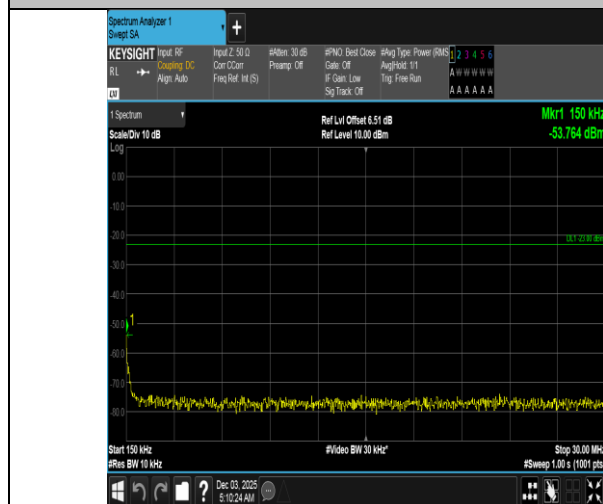
Band5-1.4MHz-QPSK-20407-1RB#5-0.15~30-PASS
