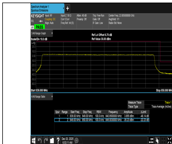
Band5-10MHz-QPSK-20600-50RB#0-PASS
