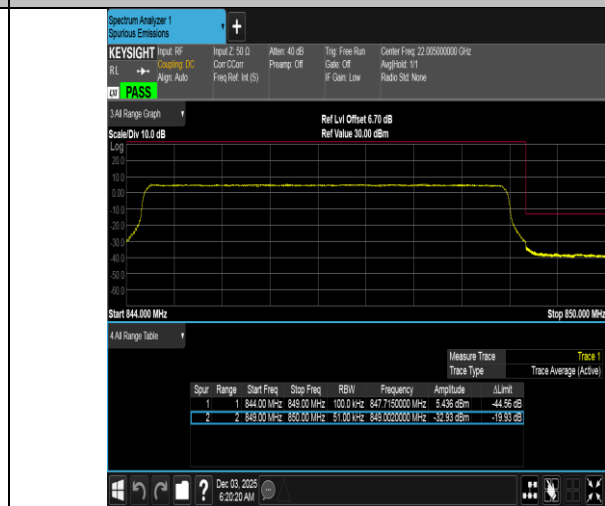
Band5-5MHz-16QAM-20625-25RB#0-PASS
