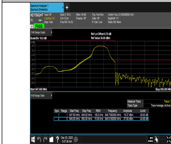
Band5-1.4MHz-16QAM-20643-1RB#5-PASS
