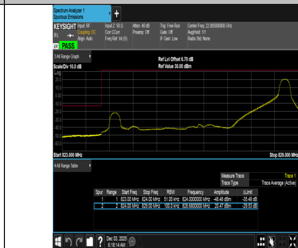
Band5-5MHz-QPSK-20425-1RB#24-PASS
