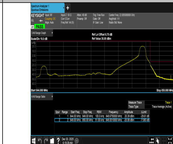
Band5-5MHz-QPSK-20625-1RB#24-PASS
