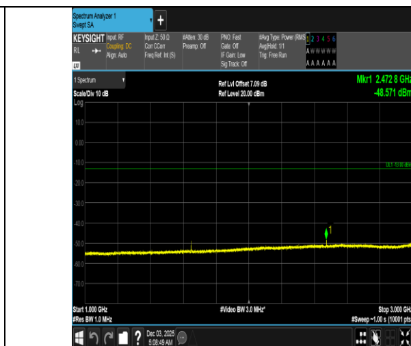
Band5-1.4MHz-QPSK-20407-1RB#0-1000~3000-PASS
