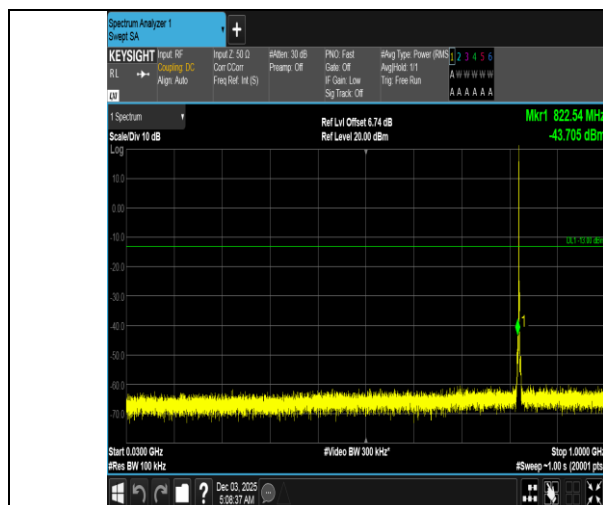
Band5-1.4MHz-QPSK-20407-1RB#0-30~1000-PASS
