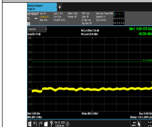
Band5-1.4MHz-QPSK-20407-1RB#0-3000~10000-PASS
