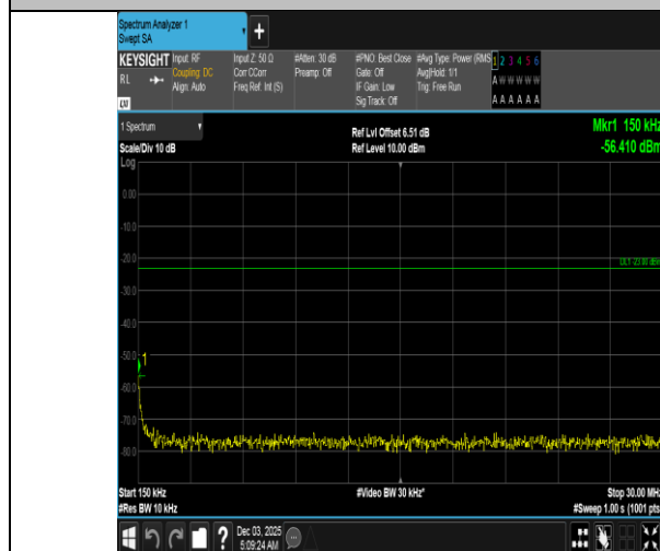
Band5-1.4MHz-16QAM-20407-1RB#0-0.15~30-PASS
