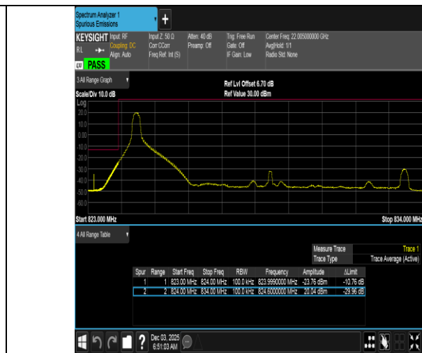
Band5-10MHz-16QAM-20450-1RB#0-PASS
