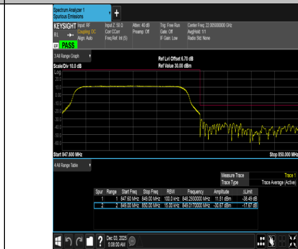
Band5-1.4MHz-16QAM-20643-6RB#0-PASS
