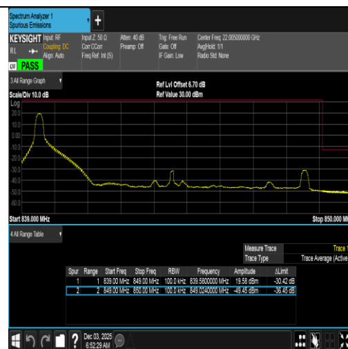
Band5-10MHz-16QAM-20600-1RB#0-PASS
