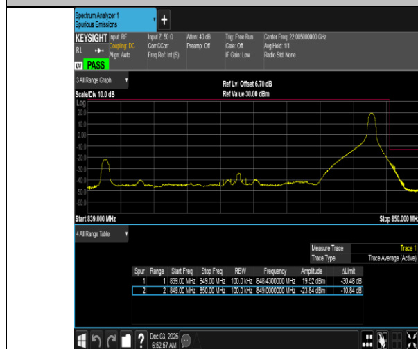
Band5-10MHz-16QAM-20600-1RB#49-PASS
