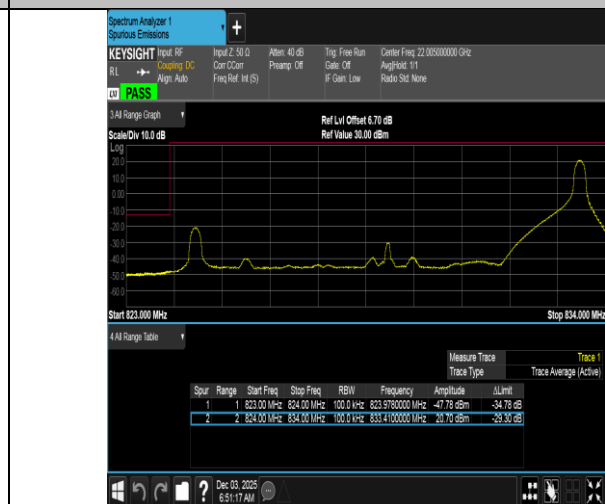
Band5-10MHz-QPSK-20450-1RB#49-PASS
