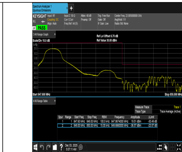
Band5-1.4MHz-16QAM-20643-1RB#0-PASS
