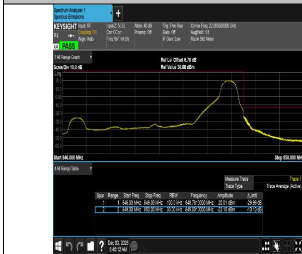
Band5-3MHz-16QAM-20635-1RB#14-PASS
