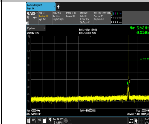
Band5-1.4MHz-QPSK-20407-1RB#5-30~1000-PASS
