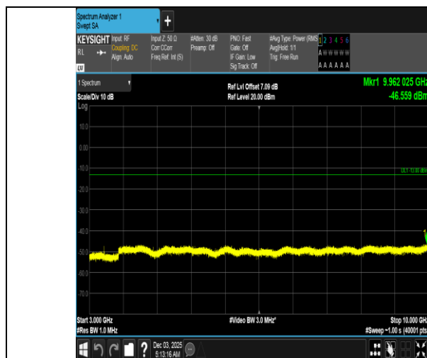
Band5-1.4MHz-QPSK-20407-6RB#0-3000~10000-PASS
