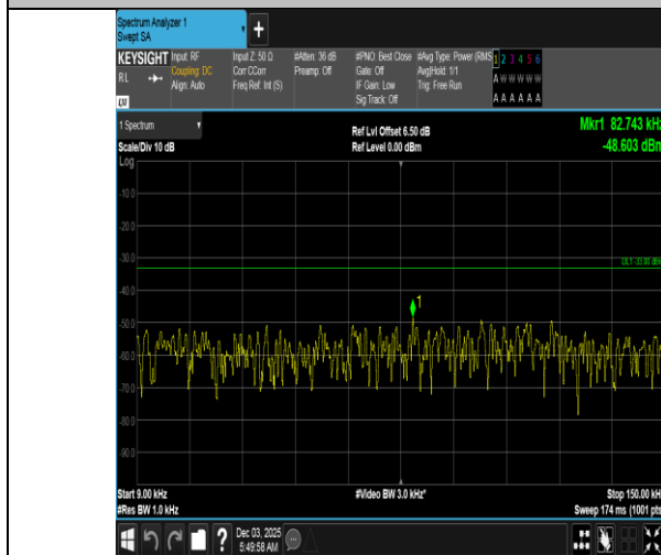
Band5-3MHz-QPSK-20415-15RB#0-0.009~0.15-PASS
