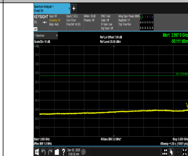
Band5-3MHz-QPSK-20415-15RB#0-1000~3000-PASS
