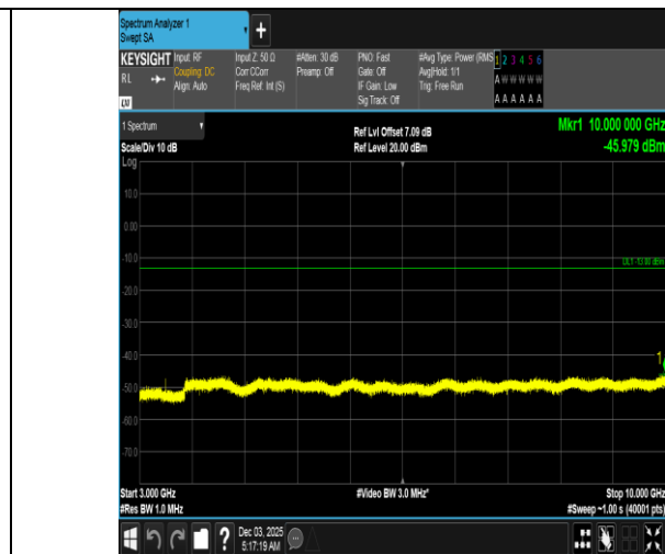
Band5-1.4MHz-QPSK-20525-1RB#5-3000~10000-PASS
