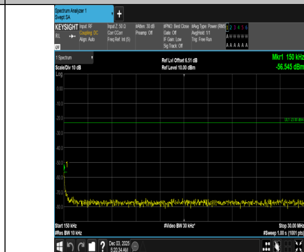
Band5-1.4MHz-QPSK-20643-1RB#0-0.15~30-PASS
