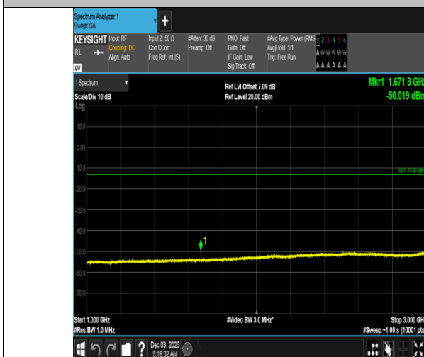
Band5-1.4MHz-16QAM-20525-1RB#0-1000~3000-PASS
