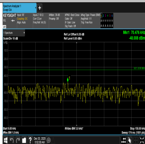
Band5-3MHz-QPSK-20525-1RB#0-0.009~0.15-PASS
