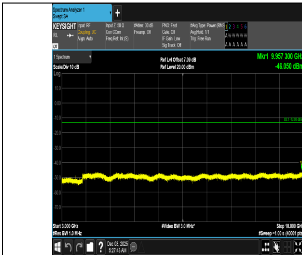
Band5-1.4MHz-QPSK-20643-6RB#0-3000~10000-PASS
