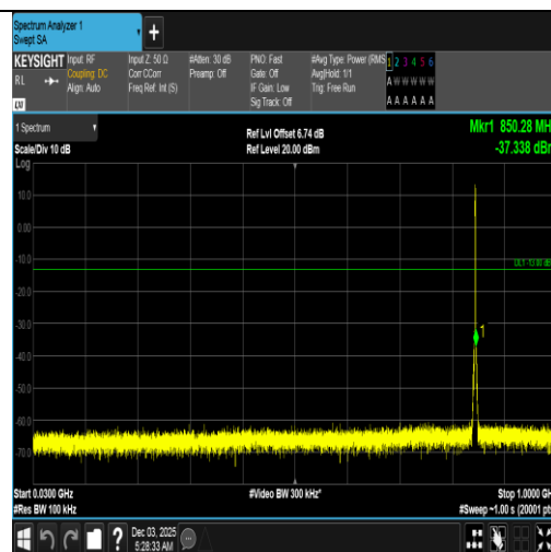
Band5-1.4MHz-16QAM-20643-6RB#0-30~1000-PASS
