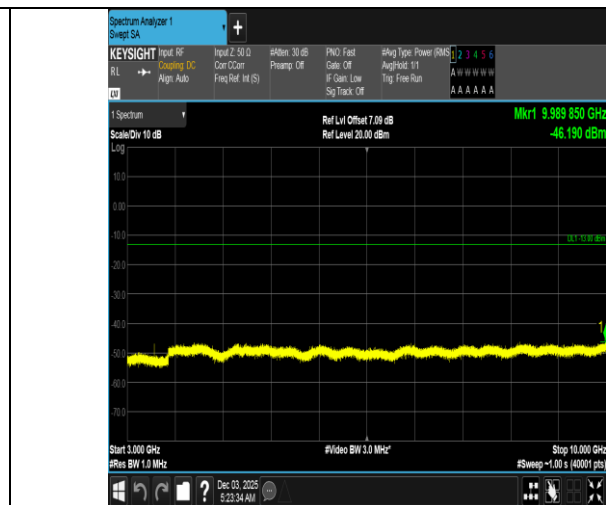
Band5-1.4MHz-QPSK-20643-1RB#5-3000~10000-PASS
