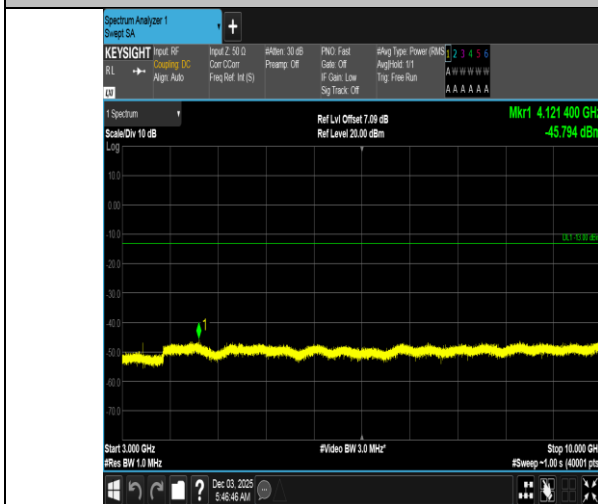
Band5-3MHz-QPSK-20415-1RB#0-3000~10000-PASS
