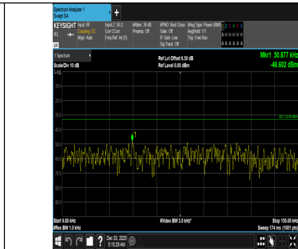
Band5-1.4MHz-16QAM-20525-1RB#0-0.009~0.15-PASS
