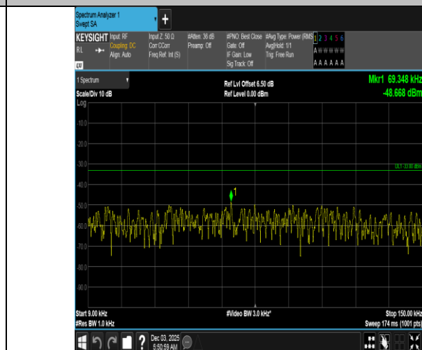
Band5-3MHz-16QAM-20415-15RB#0-0.009~0.15-PASS
