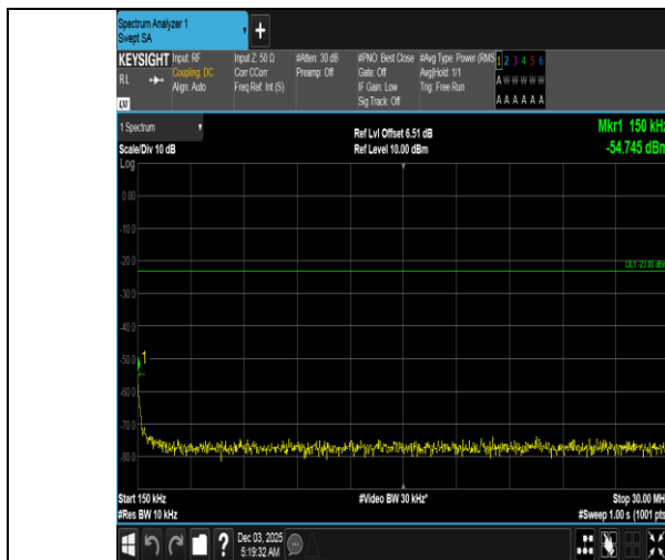
Band5-1.4MHz-16QAM-20525-6RB#0-0.15~30-PASS
