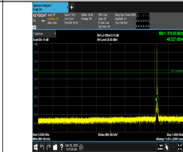
Band5-3MHz-16QAM-20415-1RB#0-30~1000-PASS
