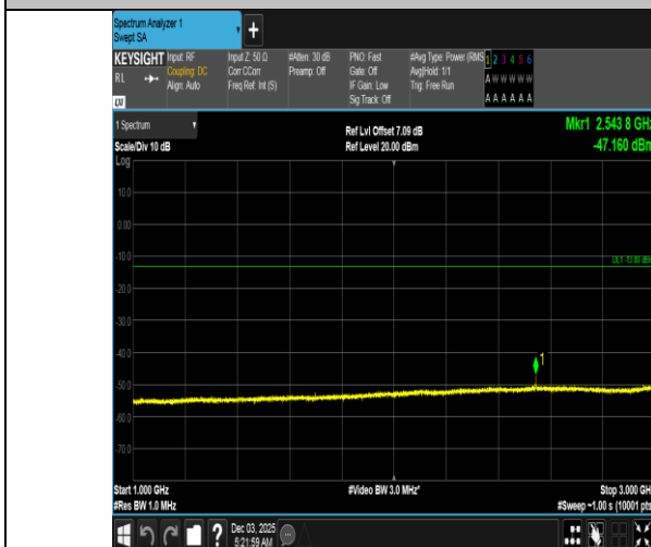
Band5-1.4MHz-16QAM-20643-1RB#0-1000~3000-PASS
