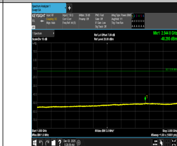
Band5-1.4MHz-QPSK-20643-6RB#0-1000~3000-PASS
