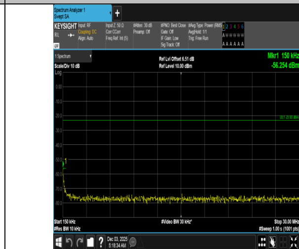
Band5-1.4MHz-QPSK-20525-6RB#0-0.15~30-PASS
