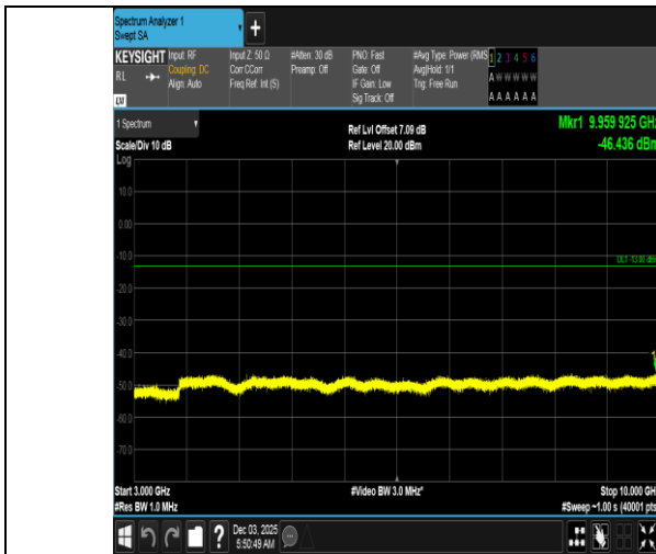
Band5-3MHz-QPSK-20415-15RB#0-3000~10000-PASS
