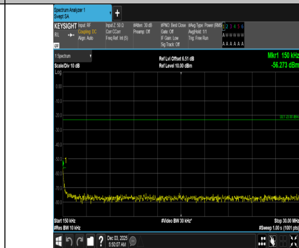
Band5-3MHz-QPSK-20415-15RB#0-0.15~30-PASS
