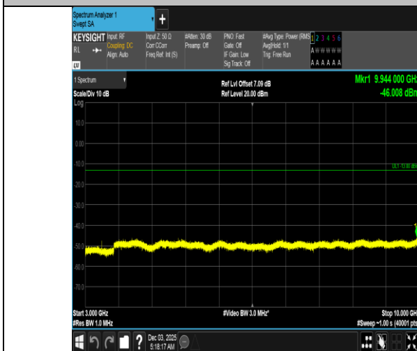
Band5-1.4MHz-16QAM-20525-1RB#5-3000~10000-PASS
