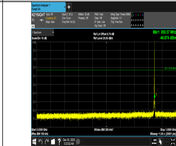
Band5-1.4MHz-QPSK-20643-1RB#5-30~1000-PASS
