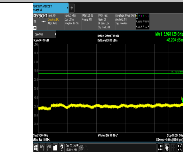
Band5-1.4MHz-16QAM-20525-6RB#0-3000~10000-PASS
