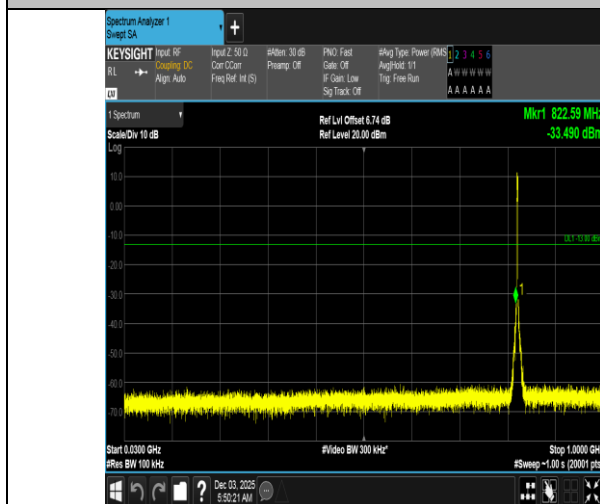
Band5-3MHz-QPSK-20415-15RB#0-30~1000-PASS
