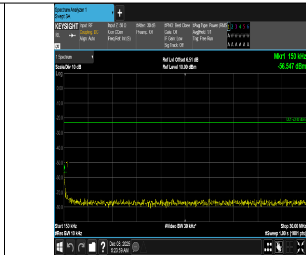
Band5-1.4MHz-16QAM-20643-1RB#5-0.15~30-PASS
