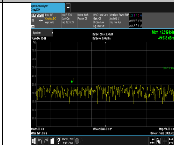
Band5-3MHz-QPSK-20415-1RB#14-0.009~0.15-PASS
