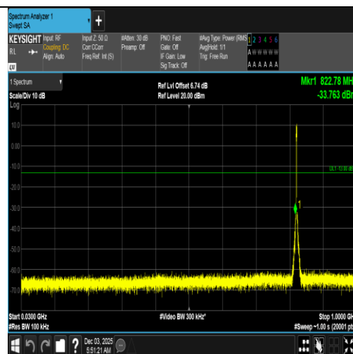
Band5-3MHz-16QAM-20415-15RB#0-30~1000-PASS
