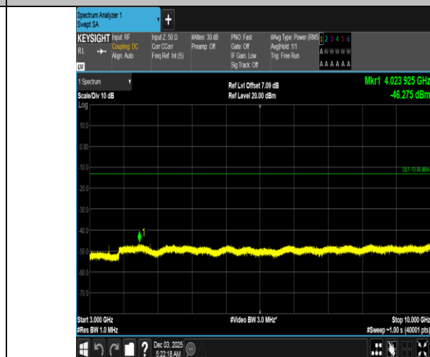
Band5-1.4MHz-16QAM-20643-1RB#0-3000~10000-PASS
