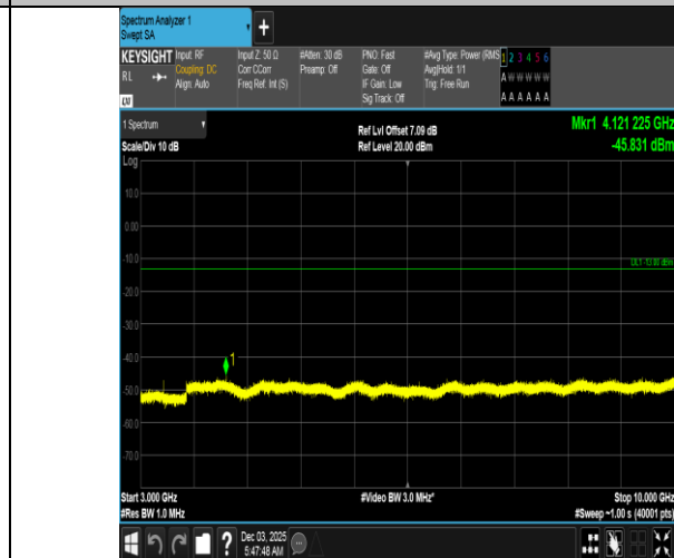
Band5-3MHz-16QAM-20415-1RB#0-3000~10000-PASS
