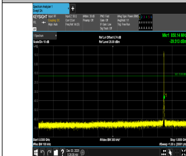
Band5-1.4MHz-QPSK-20643-6RB#0-30~1000-PASS
