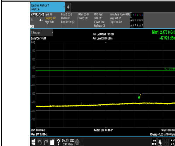
Band5-3MHz-16QAM-20415-1RB#0-1000~3000-PASS
