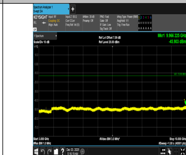
Band5-1.4MHz-16QAM-20525-1RB#0-3000~10000-PASS
