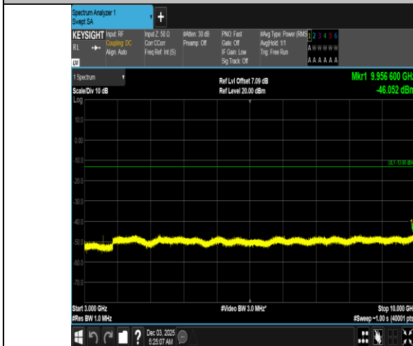
Band5-1.4MHz-16QAM-20643-1RB#5-3000~10000-PASS
