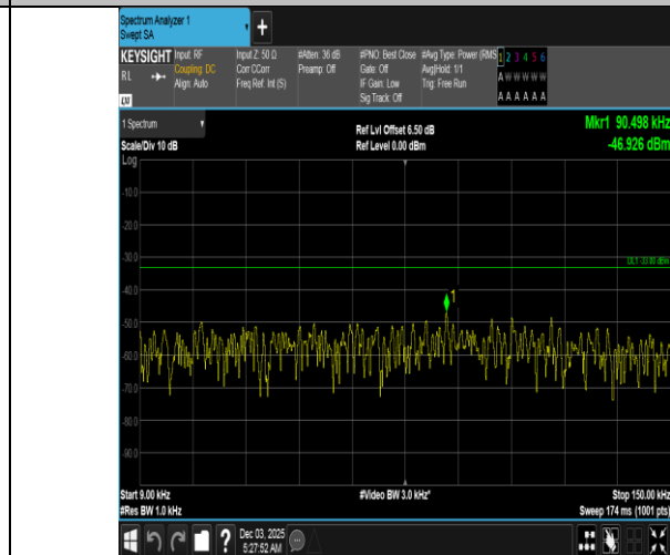
Band5-1.4MHz-16QAM-20643-6RB#0-0.009~0.15-PASS
