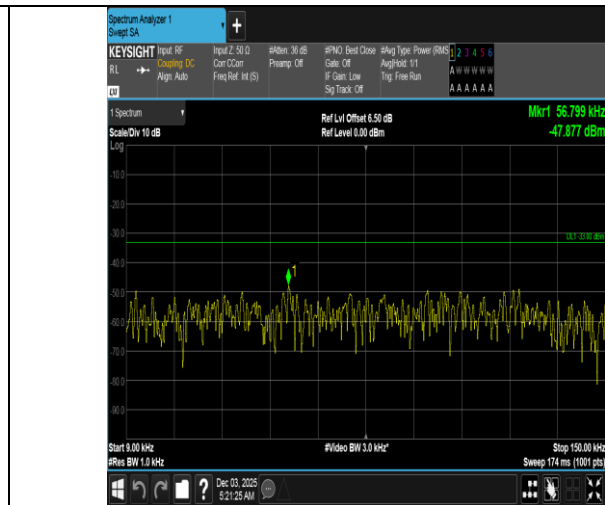
Band5-1.4MHz-16QAM-20643-1RB#0-0.009~0.15-PASS
