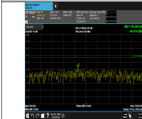
Band5-1.4MHz-QPSK-20643-6RB#0-0.009~0.15-PASS
