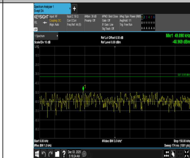
Band5-1.4MHz-16QAM-20525-6RB#0-0.009~0.15-PASS
