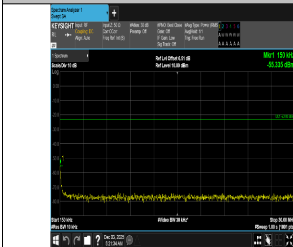
Band5-1.4MHz-16QAM-20643-1RB#0-0.15~30-PASS
