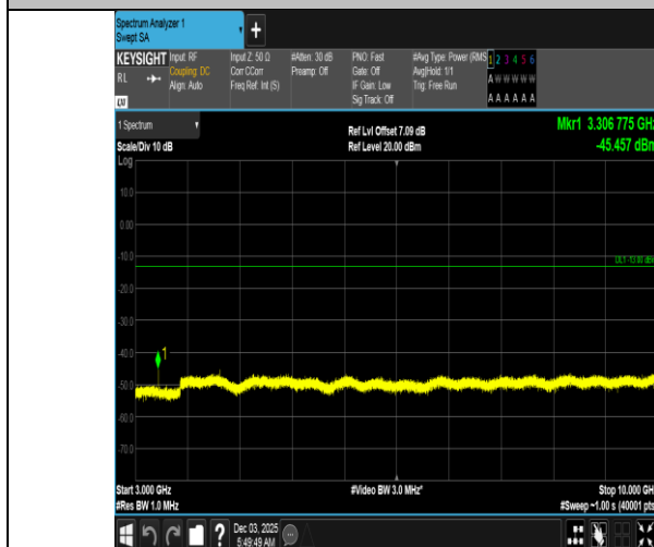
Band5-3MHz-16QAM-20415-1RB#14-3000~10000-PASS
