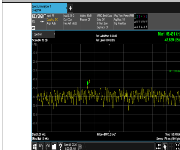
Band5-1.4MHz-QPSK-20643-1RB#0-0.009~0.15-PASS
