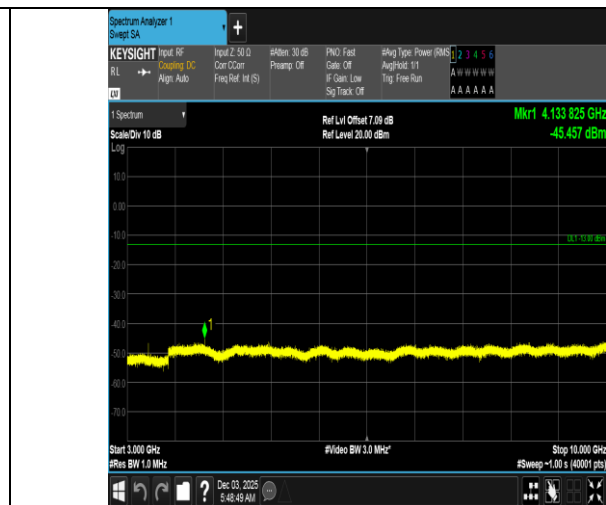
Band5-3MHz-QPSK-20415-1RB#14-3000~10000-PASS
