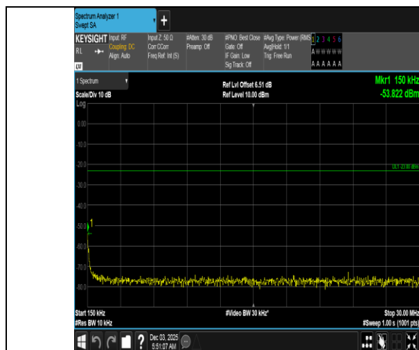
Band5-3MHz-16QAM-20415-15RB#0-0.15~30-PASS
