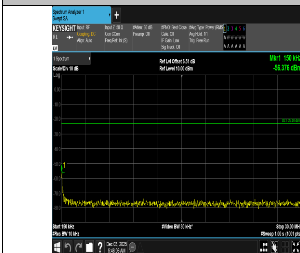
Band5-3MHz-QPSK-20415-1RB#14-0.15~30-PASS
