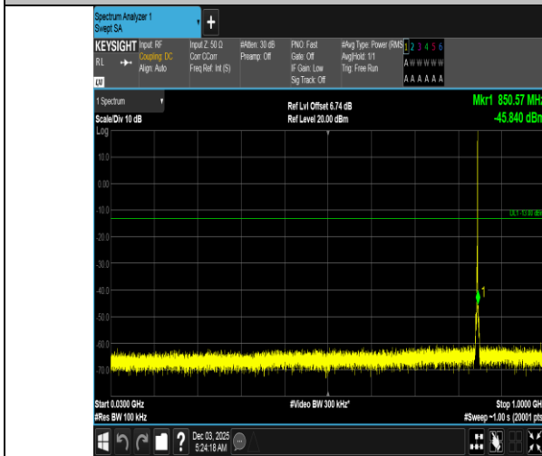
Band5-1.4MHz-16QAM-20643-1RB#5-30~1000-PASS
