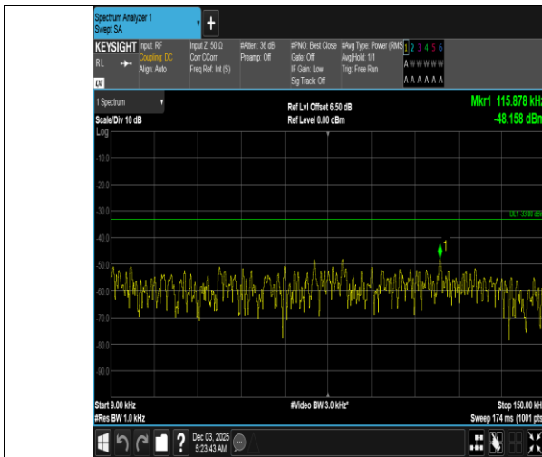
Band5-1.4MHz-16QAM-20643-1RB#5-0.009~0.15-PASS
