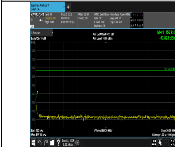
Band5-1.4MHz-QPSK-20643-1RB#5-0.15~30-PASS
