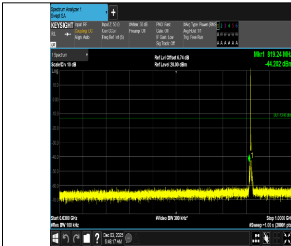
Band5-3MHz-QPSK-20415-1RB#0-30~1000-PASS
