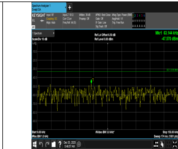
Band5-3MHz-16QAM-20415-1RB#0-0.009~0.15-PASS
