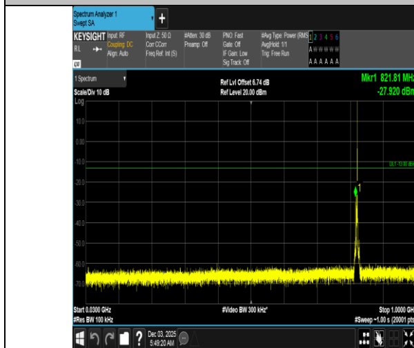
Band5-3MHz-16QAM-20415-1RB#14-30~1000-PASS
