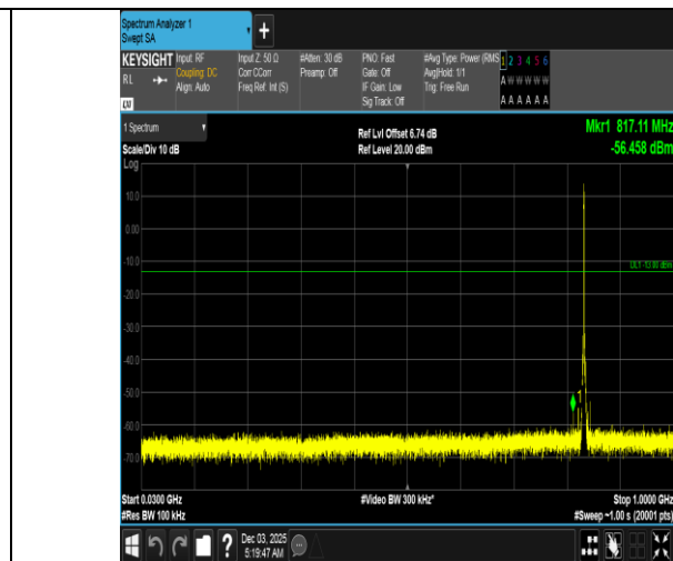
Band5-1.4MHz-16QAM-20525-6RB#0-30~1000-PASS
