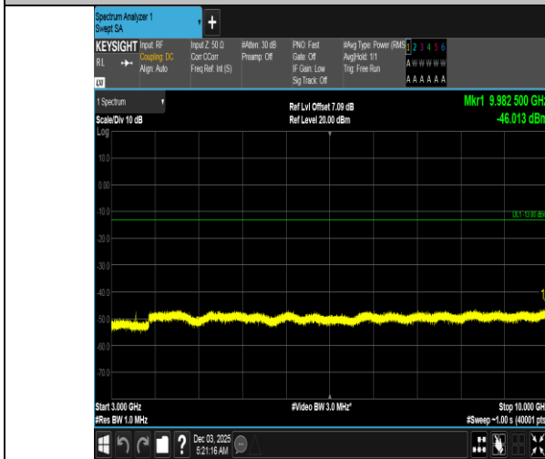
Band5-1.4MHz-QPSK-20643-1RB#0-3000~10000-PASS
