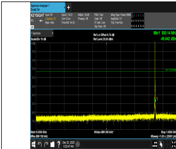
Band5-1.4MHz-QPSK-20643-1RB#0-30~1000-PASS
