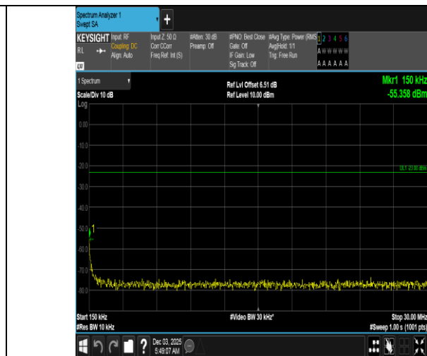
Band5-3MHz-16QAM-20415-1RB#14-0.15~30-PASS
