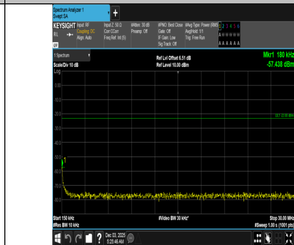
Band5-1.4MHz-QPSK-20643-6RB#0-0.15~30-PASS
