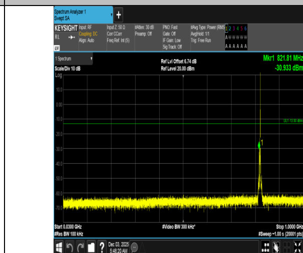
Band5-3MHz-QPSK-20415-1RB#14-30~1000-PASS
