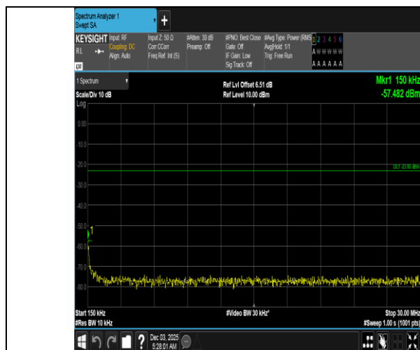
Band5-1.4MHz-16QAM-20643-6RB#0-0.15~30-PASS
