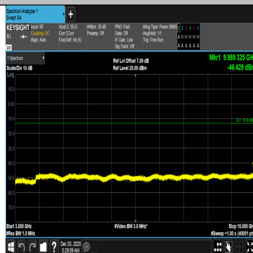
Band5-1.4MHz-16QAM-20643-6RB#0-3000~10000-PASS
