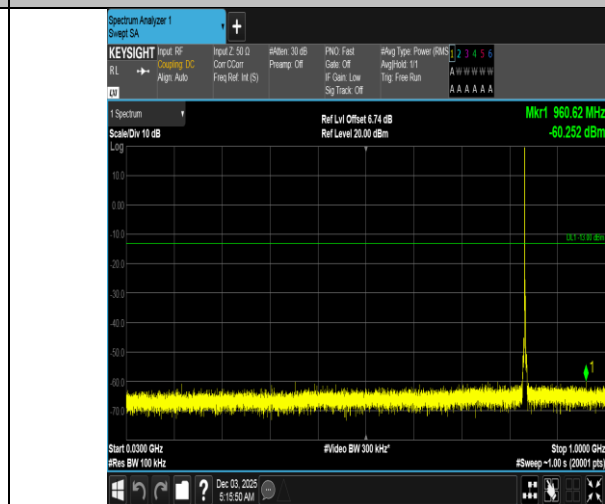
Band5-1.4MHz-16QAM-20525-1RB#0-30~1000-PASS
