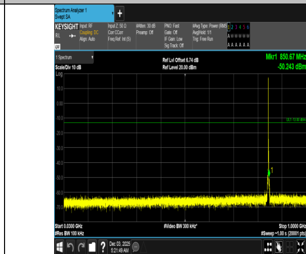
Band5-1.4MHz-16QAM-20643-1RB#0-30~1000-PASS
