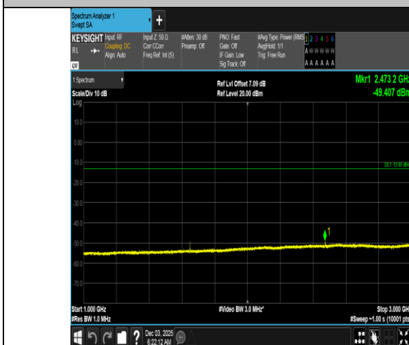
Band5-5MHz-16QAM-20425-1RB#0-1000~3000-PASS
