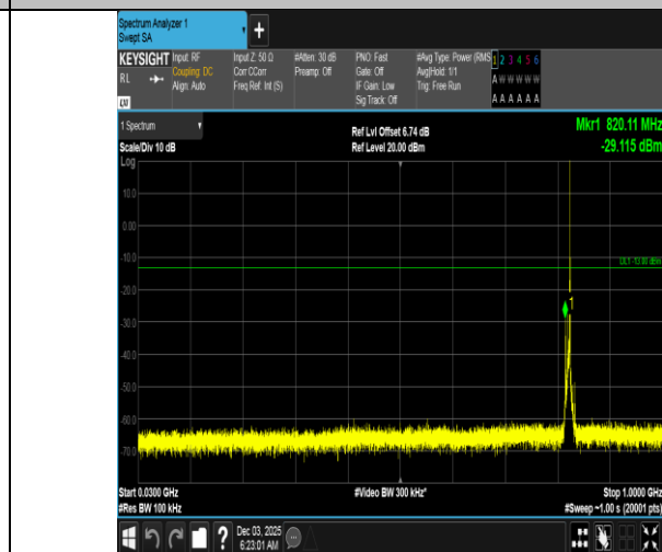
Band5-5MHz-QPSK-20425-1RB#24-30~1000-PASS
