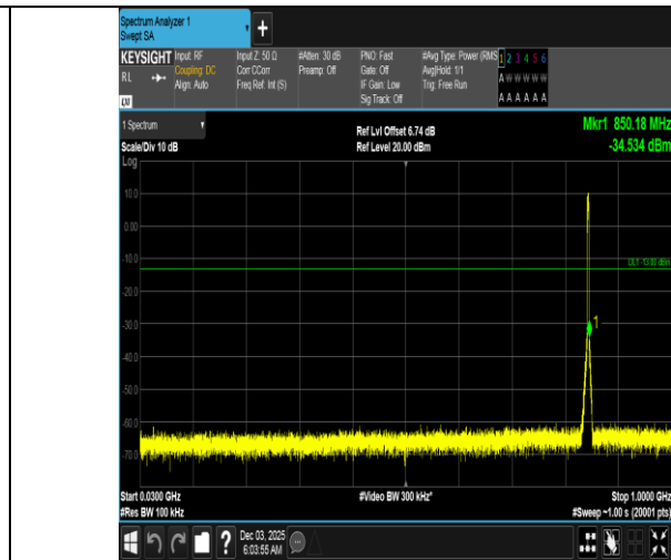
Band5-3MHz-16QAM-20635-15RB#0-30~1000-PASS
