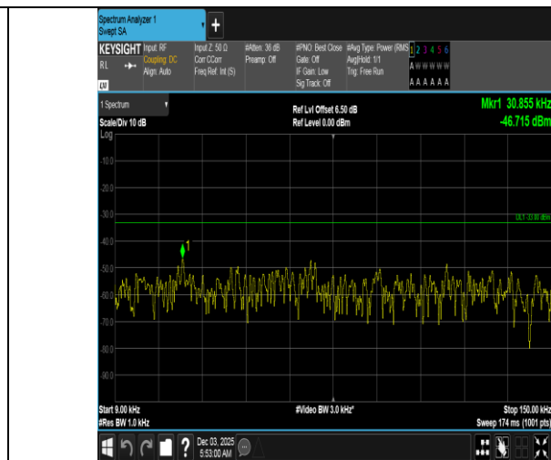
Band5-3MHz-16QAM-20525-1RB#0-0.009~0.15-PASS
