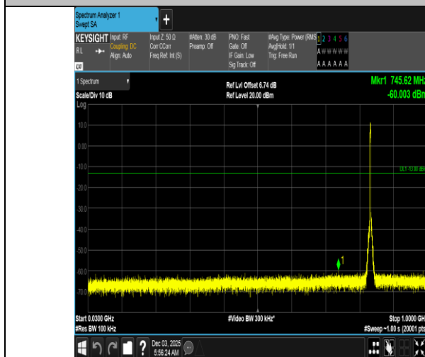
Band5-3MHz-QPSK-20525-15RB#0-30~1000-PASS
