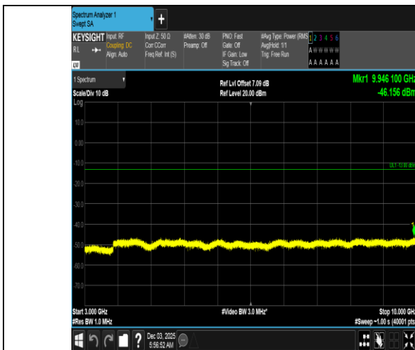
Band5-3MHz-QPSK-20525-15RB#0-3000~10000-PASS
