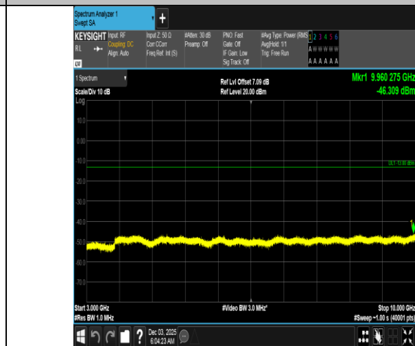
Band5-3MHz-16QAM-20635-15RB#0-3000~10000-PASS
