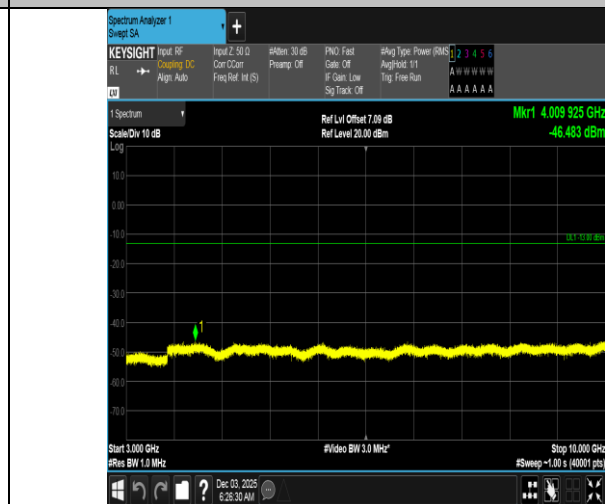
Band5-5MHz-16QAM-20425-25RB#0-3000~10000-PASS
