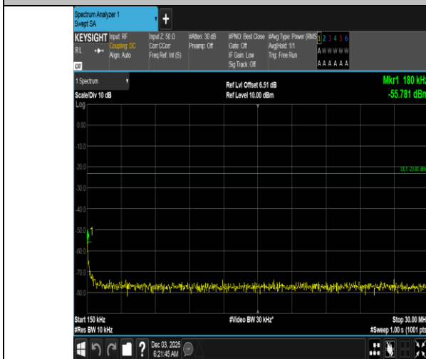
Band5-5MHz-16QAM-20425-1RB#0-0.15~30-PASS
