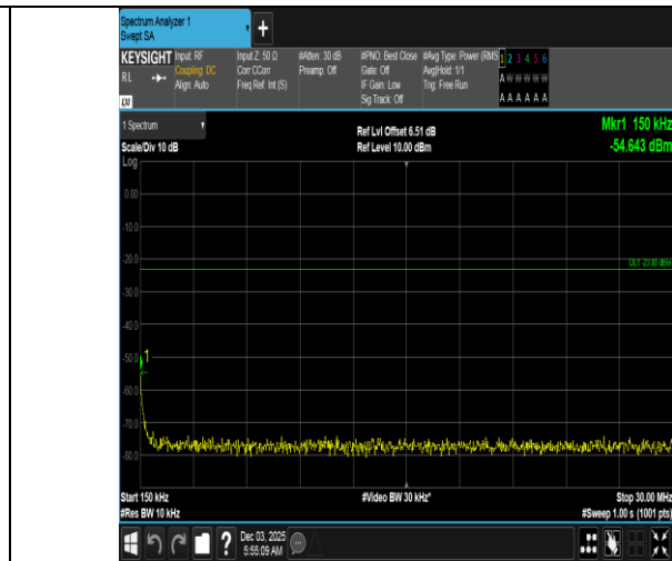
Band5-3MHz-16QAM-20525-1RB#14-0.15~30-PASS
