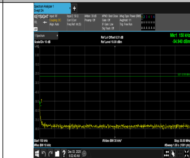
Band5-3MHz-QPSK-20635-15RB#0-0.15~30-PASS
