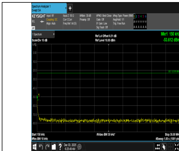
Band5-5MHz-16QAM-20425-25RB#0-0.15~30-PASS
