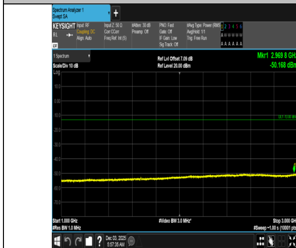
Band5-3MHz-16QAM-20525-15RB#0-1000~3000-PASS
