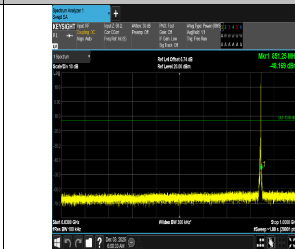
Band5-3MHz-QPSK-20635-1RB#14-30~1000-PASS
