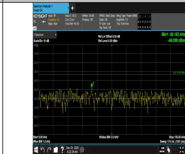
Band5-5MHz-QPSK-20425-1RB#24-0.009~0.15-PASS
