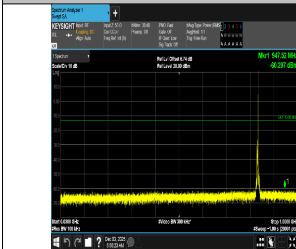
Band5-3MHz-16QAM-20525-1RB#14-30~1000-PASS
