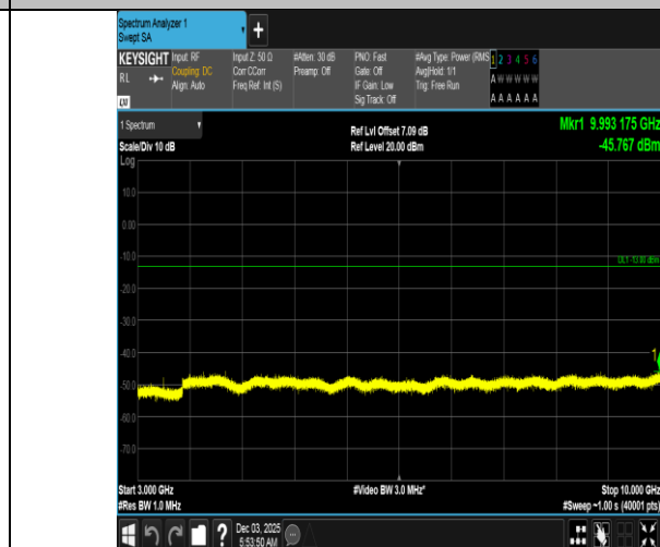
Band5-3MHz-16QAM-20525-1RB#0-3000~10000-PASS
