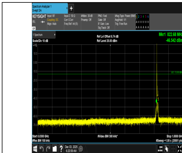
Band5-5MHz-QPSK-20425-1RB#0-30~1000-PASS
