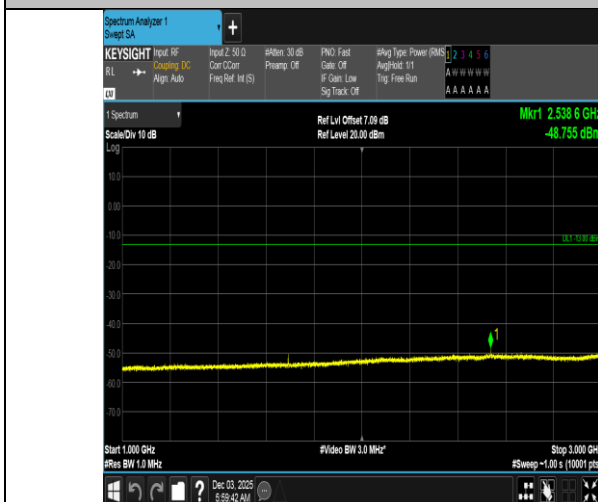
Band5-3MHz-16QAM-20635-1RB#0-1000~3000-PASS
