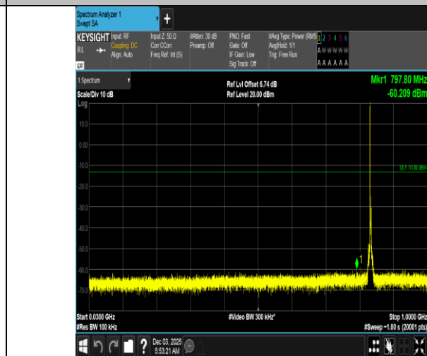
Band5-3MHz-16QAM-20525-1RB#0-30~1000-PASS
