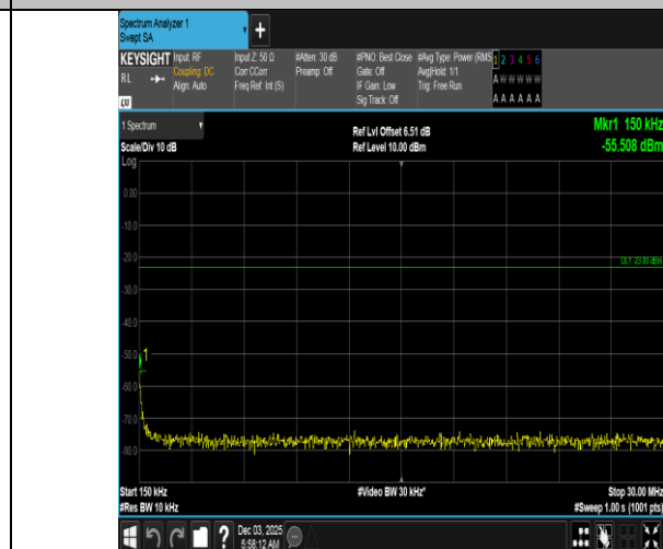
Band5-3MHz-QPSK-20635-1RB#0-0.15~30-PASS
