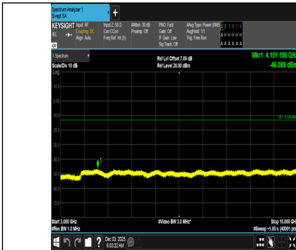
Band5-3MHz-QPSK-20635-15RB#0-3000~10000-PASS
