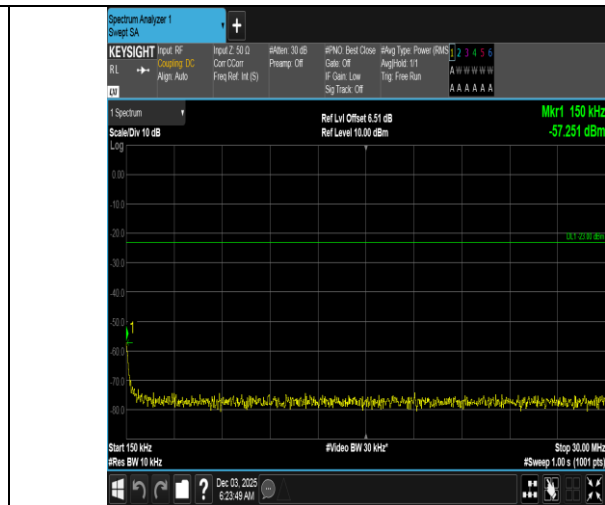
Band5-5MHz-16QAM-20425-1RB#24-0.15~30-PASS
