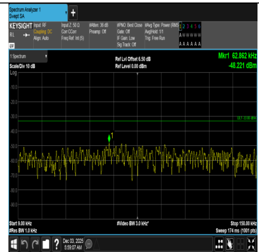
Band5-3MHz-16QAM-20635-1RB#0-0.009~0.15-PASS
