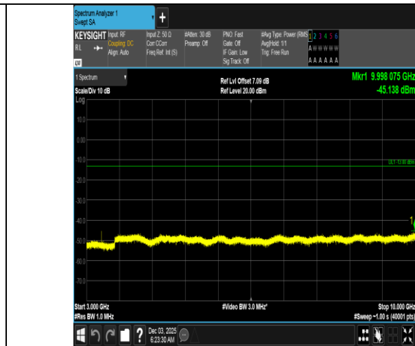
Band5-5MHz-QPSK-20425-1RB#24-3000~10000-PASS
