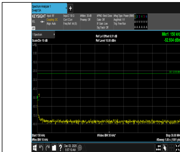
Band5-3MHz-16QAM-20525-15RB#0-0.15~30-PASS
