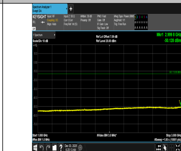
Band5-5MHz-QPSK-20425-25RB#0-1000~3000-PASS
