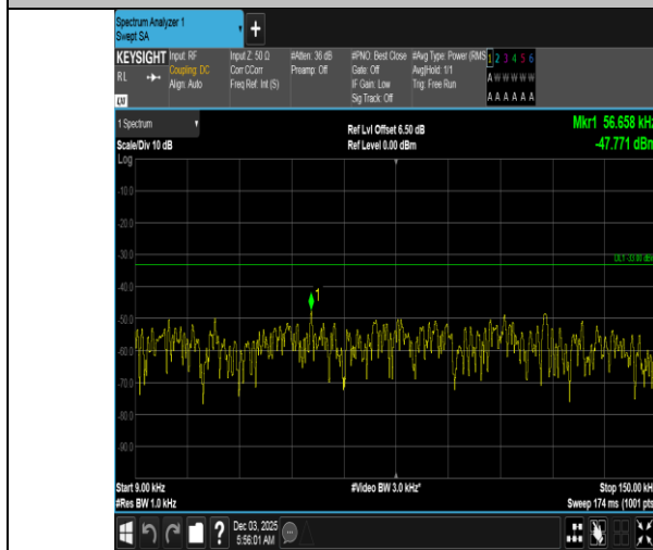
Band5-3MHz-QPSK-20525-15RB#0-0.009~0.15-PASS
