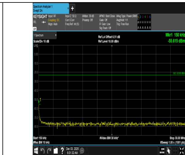
Band5-3MHz-16QAM-20635-1RB#14-0.15~30-PASS
