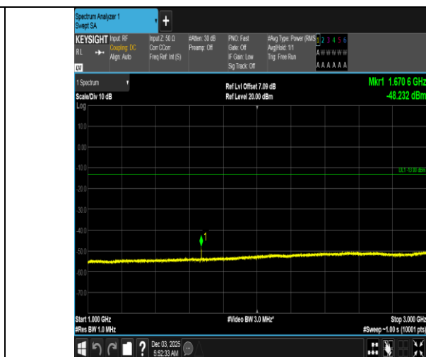
Band5-3MHz-QPSK-20525-1RB#0-1000~3000-PASS
