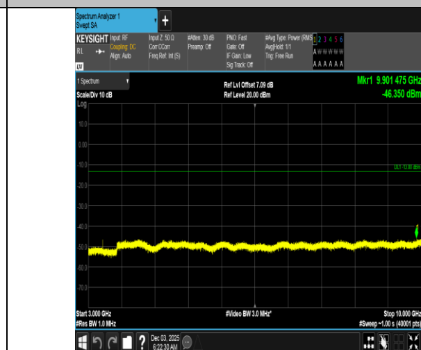
Band5-5MHz-16QAM-20425-1RB#0-3000~10000-PASS
