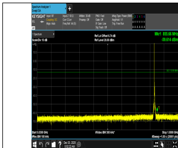
Band5-3MHz-QPSK-20525-1RB#0-30~1000-PASS
