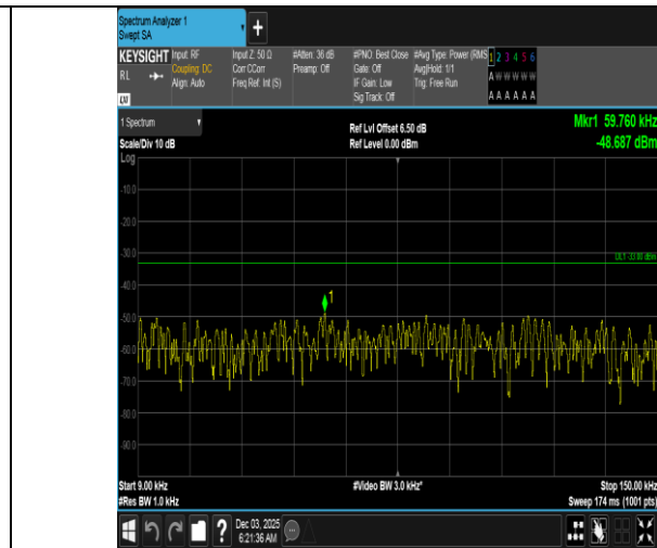
Band5-5MHz-16QAM-20425-1RB#0-0.009~0.15-PASS
