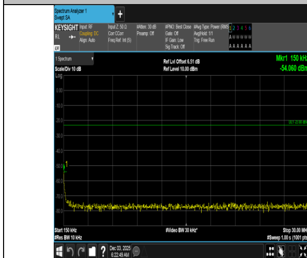
Band5-5MHz-QPSK-20425-1RB#24-0.15~30-PASS
