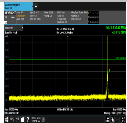
Band5-3MHz-16QAM-20635-1RB#0-30~1000-PASS
