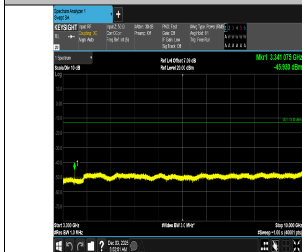
Band5-3MHz-QPSK-20525-1RB#0-3000~10000-PASS
