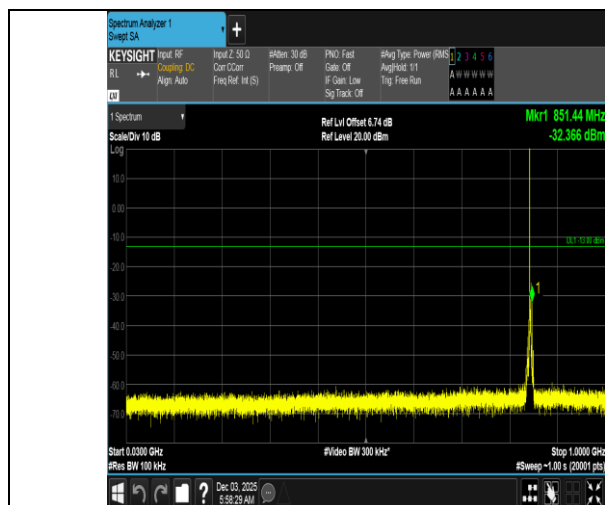
Band5-3MHz-QPSK-20635-1RB#0-30~1000-PASS
