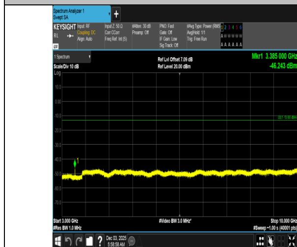
Band5-3MHz-QPSK-20635-1RB#0-3000~10000-PASS
