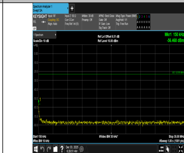
Band5-5MHz-QPSK-20525-1RB#0-0.15~30-PASS
