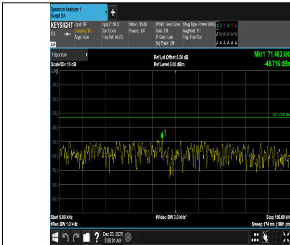
Band5-3MHz-16QAM-20525-1RB#14-0.009~0.15-PASS
