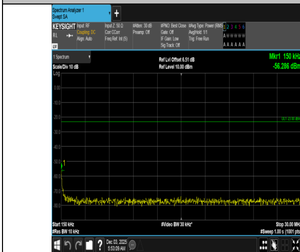
Band5-3MHz-16QAM-20525-1RB#0-0.15~30-PASS
