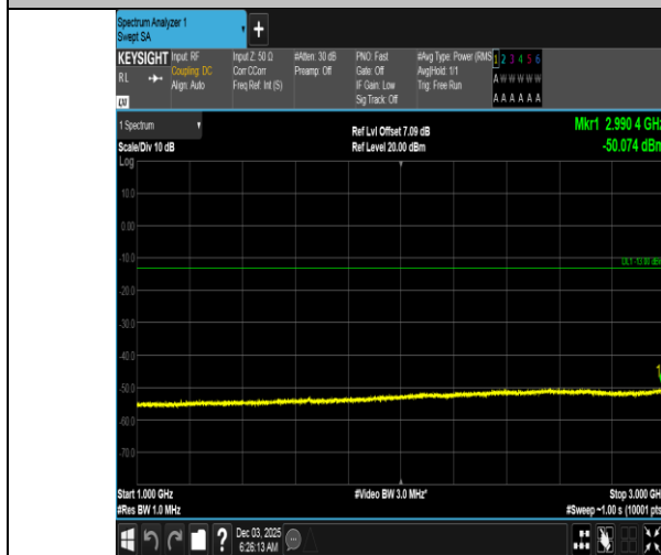
Band5-5MHz-16QAM-20425-25RB#0-1000~3000-PASS
