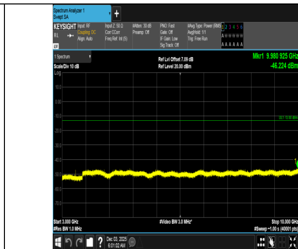
Band5-3MHz-QPSK-20635-1RB#14-3000~10000-PASS
