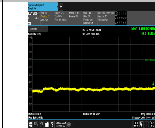
Band5-3MHz-16QAM-20525-15RB#0-3000~10000-PASS
