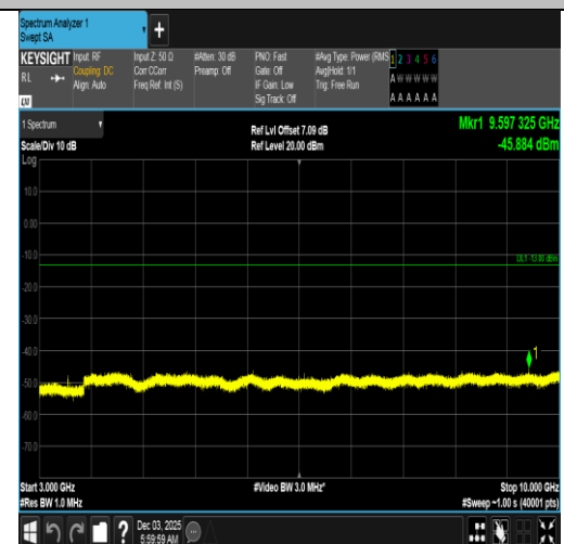
Band5-3MHz-16QAM-20635-1RB#0-3000~10000-PASS
