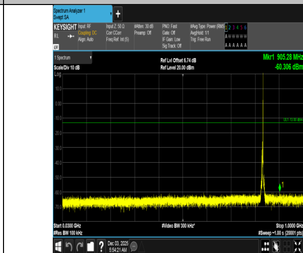
Band5-3MHz-QPSK-20525-1RB#14-30~1000-PASS
