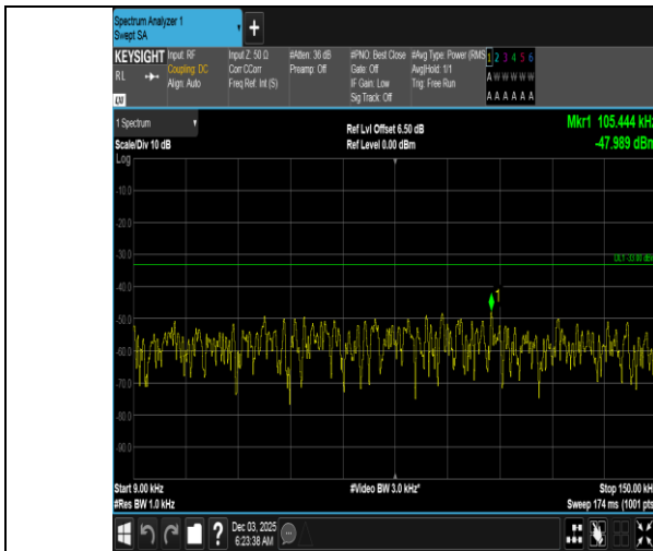
Band5-5MHz-16QAM-20425-1RB#24-0.009~0.15-PASS
