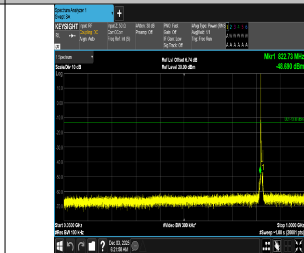
Band5-5MHz-16QAM-20425-1RB#0-30~1000-PASS
