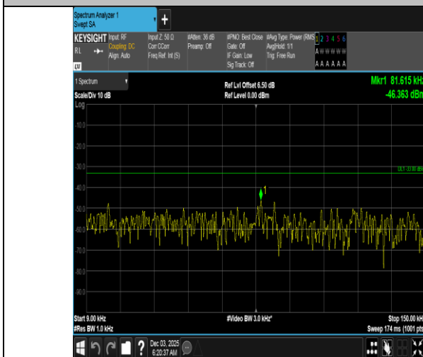
Band5-5MHz-QPSK-20425-1RB#0-0.009~0.15-PASS
