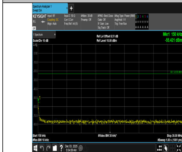
Band5-3MHz-QPSK-20525-1RB#14-0.15~30-PASS
