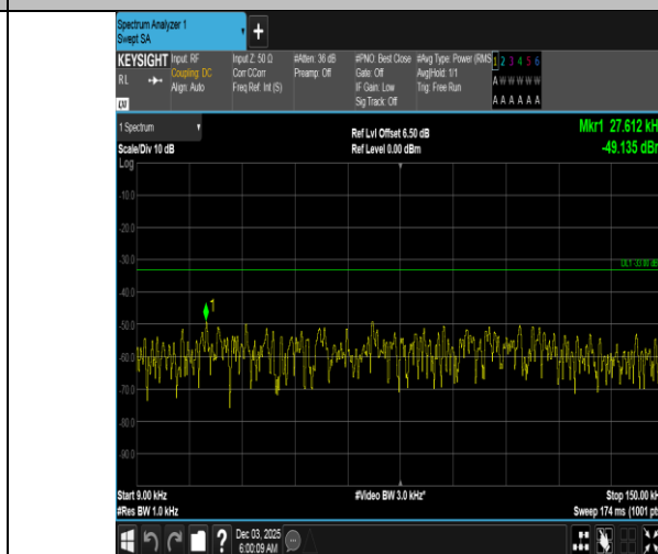
Band5-3MHz-QPSK-20635-1RB#14-0.009~0.15-PASS
