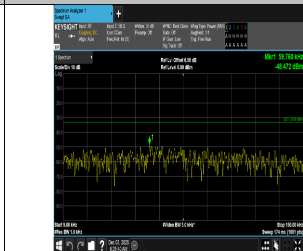
Band5-5MHz-16QAM-20425-25RB#0-0.009~0.15-PASS
