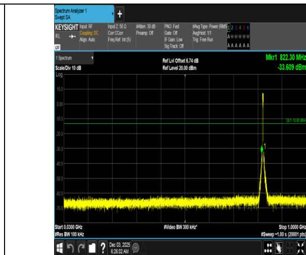
Band5-5MHz-16QAM-20425-25RB#0-30~1000-PASS
