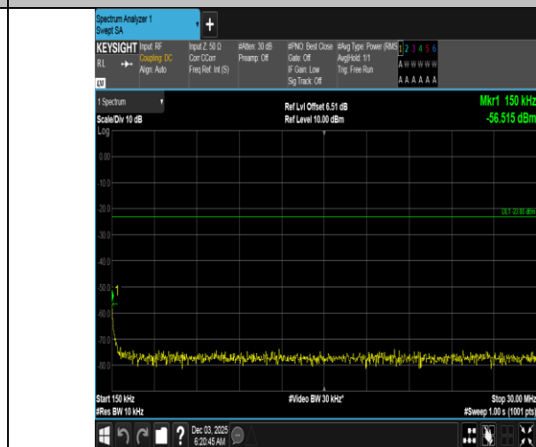
Band5-5MHz-QPSK-20425-1RB#0-0.15~30-PASS
