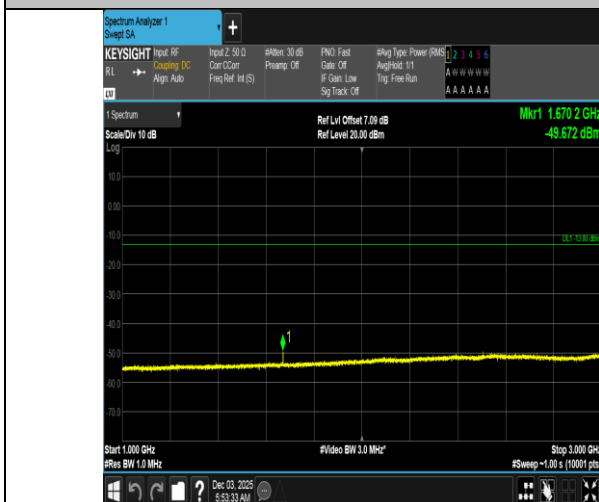
Band5-3MHz-16QAM-20525-1RB#0-1000~3000-PASS
