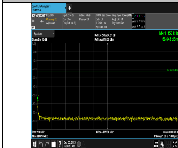
Band5-3MHz-QPSK-20635-1RB#14-0.15~30-PASS
