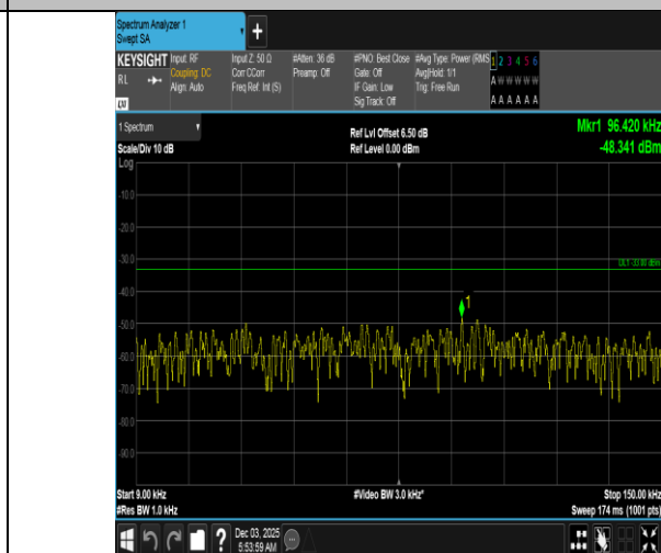
Band5-3MHz-QPSK-20525-1RB#14-0.009~0.15-PASS
