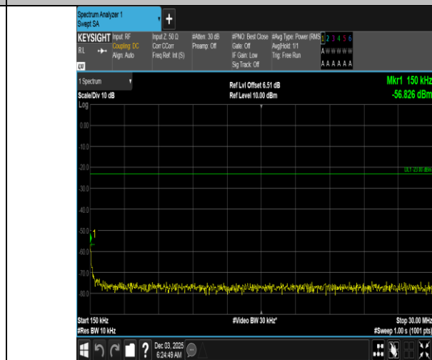
Band5-5MHz-QPSK-20425-25RB#0-0.15~30-PASS
