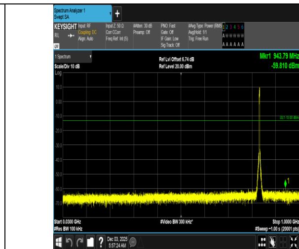
Band5-3MHz-16QAM-20525-15RB#0-30~1000-PASS
