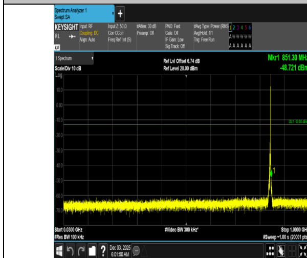
Band5-3MHz-16QAM-20635-1RB#14-30~1000-PASS
