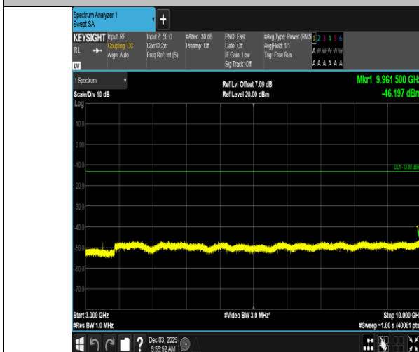
Band5-3MHz-16QAM-20525-1RB#14-3000~10000-PASS
