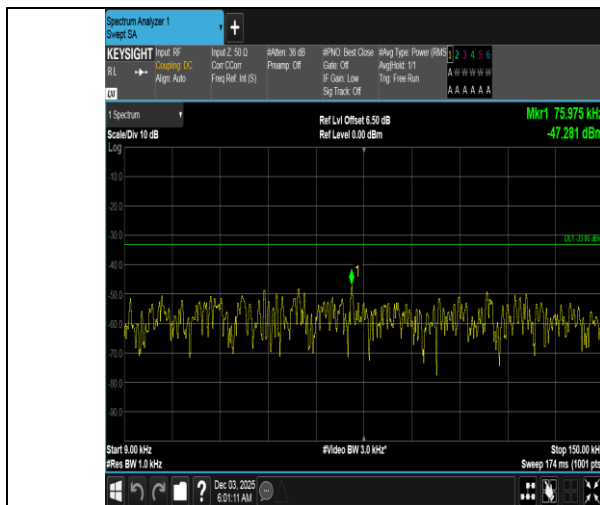
Band5-3MHz-16QAM-20635-1RB#14-0.009~0.15-PASS
