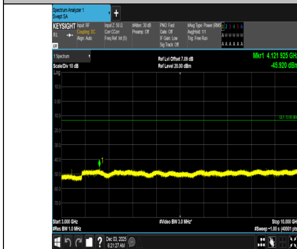
Band5-5MHz-QPSK-20425-1RB#0-3000~10000-PASS
