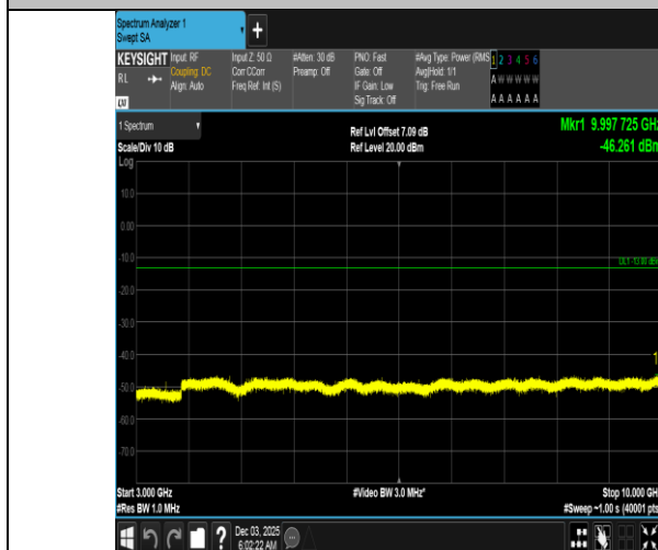
Band5-3MHz-16QAM-20635-1RB#14-3000~10000-PASS
