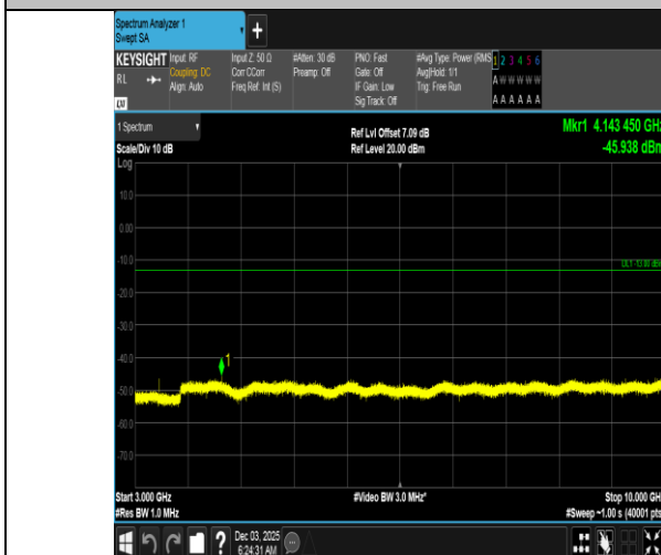
Band5-5MHz-16QAM-20425-1RB#24-3000~10000-PASS
