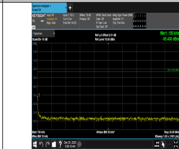
Band5-3MHz-QPSK-20525-15RB#0-0.15~30-PASS
