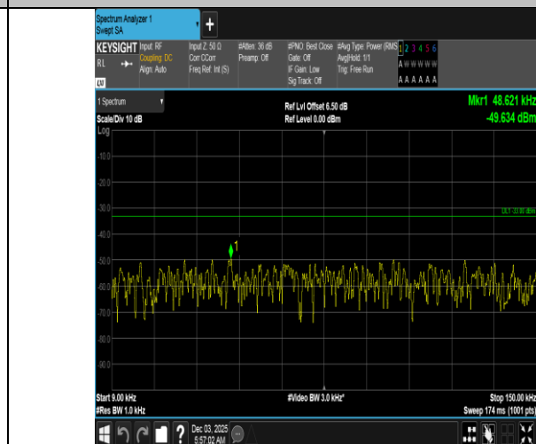
Band5-3MHz-16QAM-20525-15RB#0-0.009~0.15-PASS
