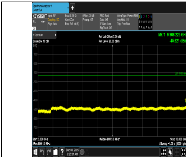
Band5-5MHz-QPSK-20425-25RB#0-3000~10000-PASS
