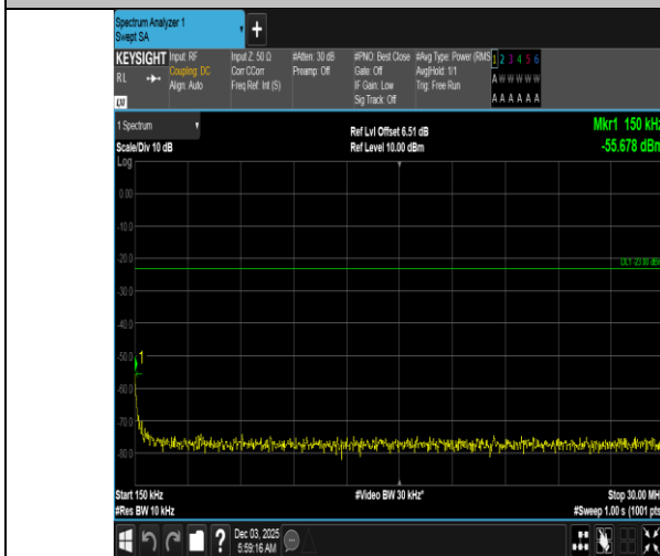
Band5-3MHz-16QAM-20635-1RB#0-0.15~30-PASS
