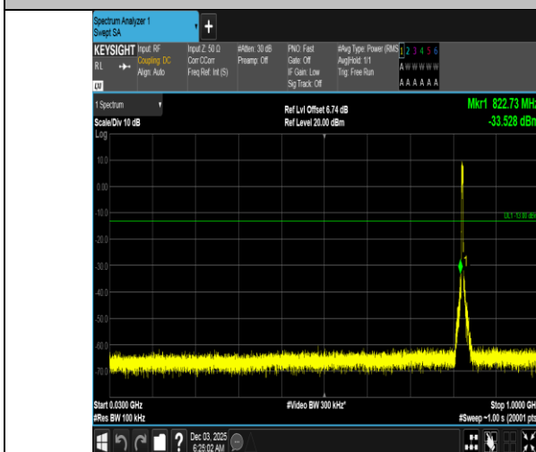
Band5-5MHz-QPSK-20425-25RB#0-30~1000-PASS
