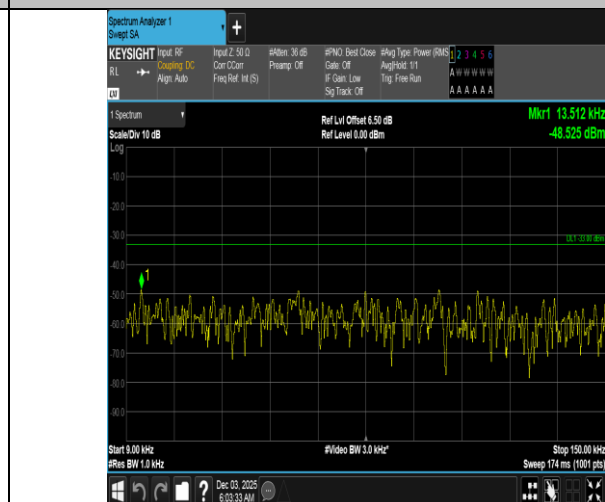
Band5-3MHz-16QAM-20635-15RB#0-0.009~0.15-PASS
