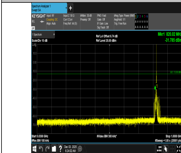
Band5-5MHz-16QAM-20425-1RB#24-30~1000-PASS
