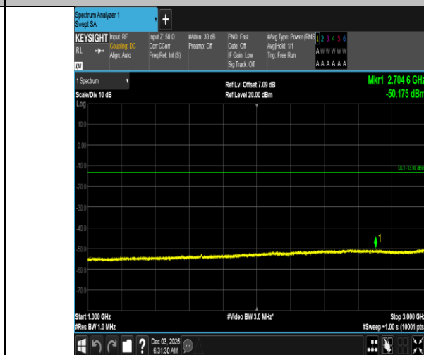
Band5-5MHz-QPSK-20525-25RB#0-1000~3000-PASS
