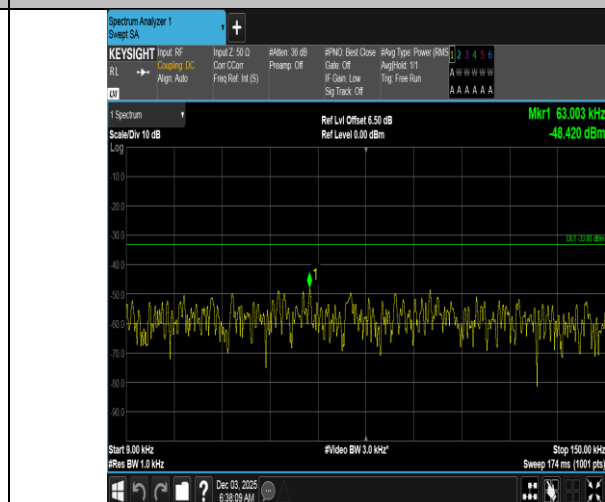
Band5-5MHz-16QAM-20625-25RB#0-0.009~0.15-PASS
