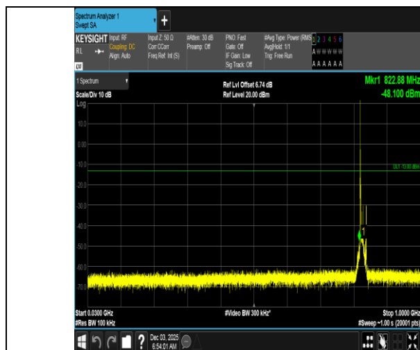
Band5-10MHz-QPSK-20450-1RB#0-30~1000-PASS
