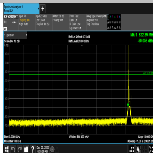
Band5-10MHz-16QAM-20450-1RB#0-30~1000-PASS
