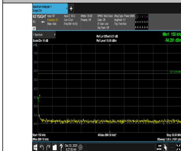
Band5-5MHz-16QAM-20525-1RB#0-0.15~30-PASS
