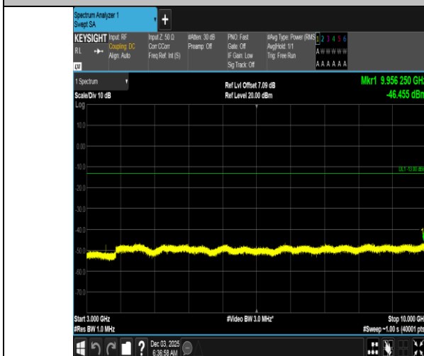
Band5-5MHz-16QAM-20625-1RB#24-3000~10000-PASS
