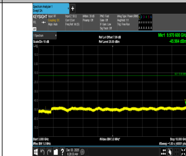
Band5-5MHz-16QAM-20525-1RB#0-3000~10000-PASS
