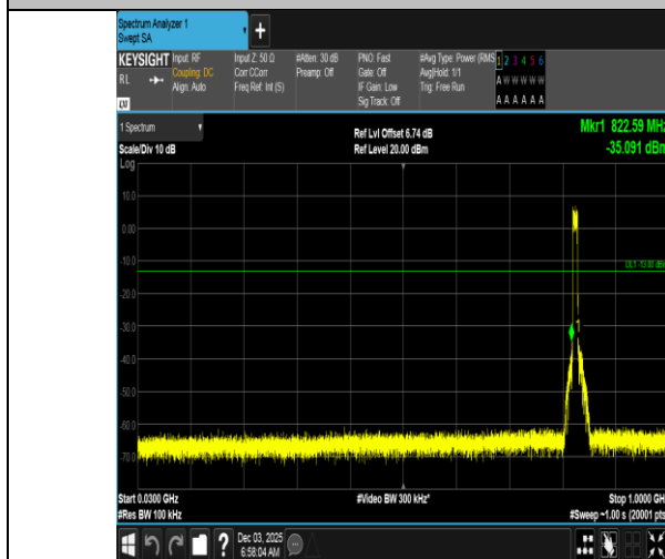
Band5-10MHz-QPSK-20450-50RB#0-30~1000-PASS
