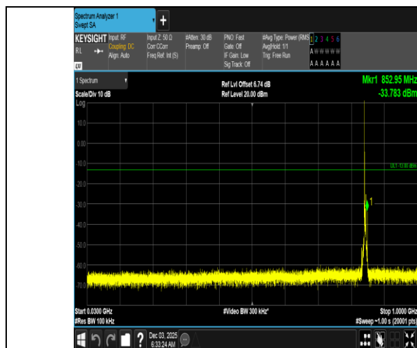
Band5-5MHz-QPSK-20625-1RB#0-30~1000-PASS
