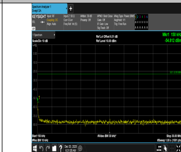
Band5-5MHz-QPSK-20525-25RB#0-0.15~30-PASS
