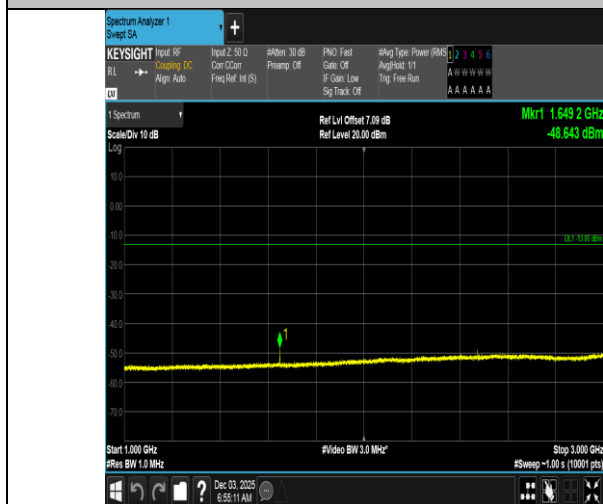
Band5-10MHz-16QAM-20450-1RB#0-1000~3000-PASS
