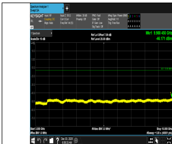
Band5-10MHz-QPSK-20450-50RB#0-3000~10000-PASS
