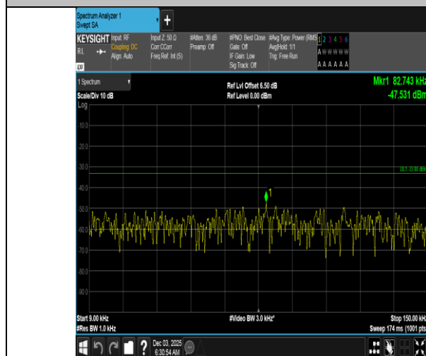
Band5-5MHz-QPSK-20525-25RB#0-0.009~0.15-PASS
