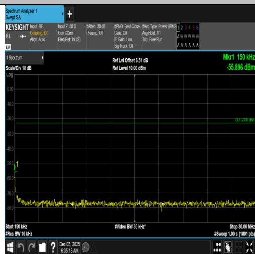
Band5-5MHz-QPSK-20625-1RB#24-0.15~30-PASS
