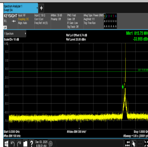
Band5-10MHz-QPSK-20450-1RB#49-30~1000-PASS
