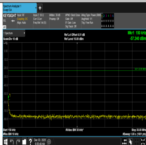
Band5-10MHz-QPSK-20450-1RB#49-0.15~30-PASS
