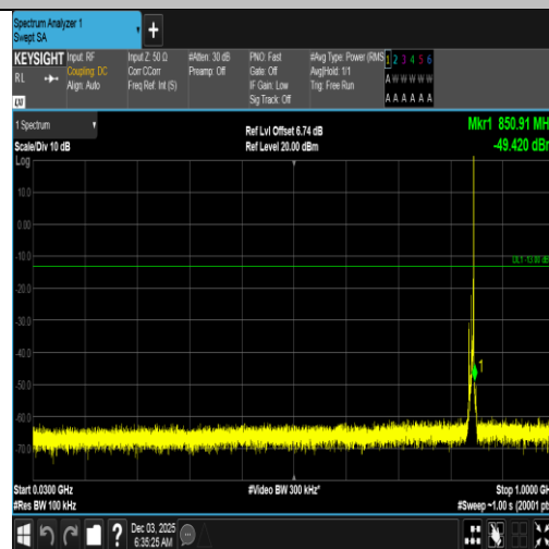
Band5-5MHz-QPSK-20625-1RB#24-30~1000-PASS
