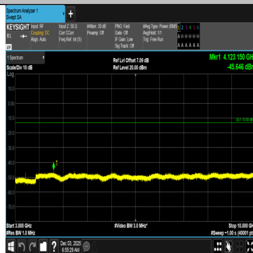
Band5-10MHz-16QAM-20450-1RB#0-3000~10000-PASS
