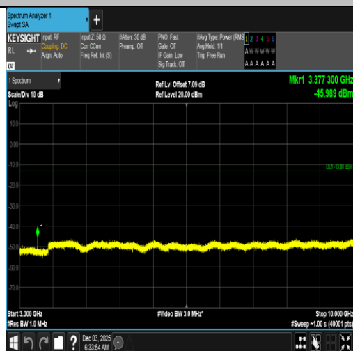
Band5-5MHz-QPSK-20625-1RB#0-3000~10000-PASS
