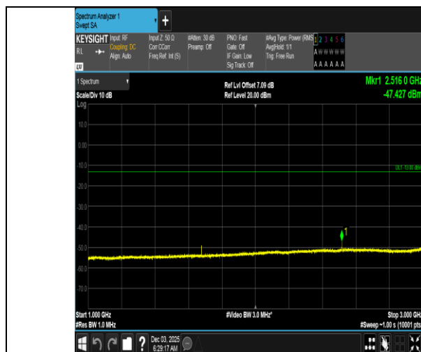
Band5-5MHz-QPSK-20525-1RB#24-1000~3000-PASS
