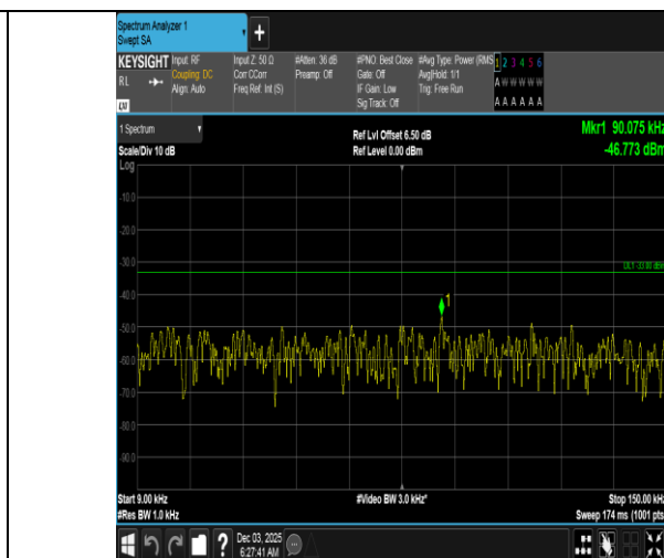
Band5-5MHz-16QAM-20525-1RB#0-0.009~0.15-PASS
