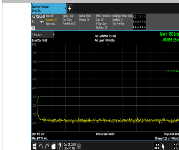
Band5-10MHz-16QAM-20450-1RB#0-0.15~30-PASS
