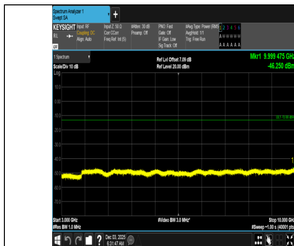
Band5-5MHz-QPSK-20525-25RB#0-3000~10000-PASS
