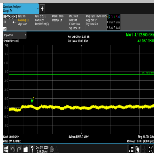
Band5-10MHz-QPSK-20450-1RB#0-3000~10000-PASS
