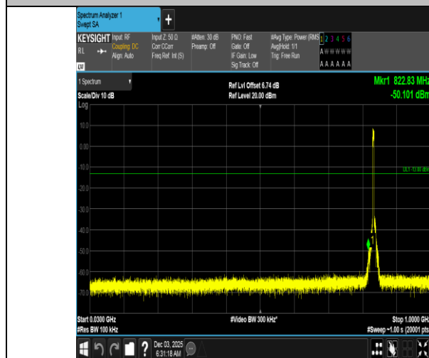
Band5-5MHz-QPSK-20525-25RB#0-30~1000-PASS
