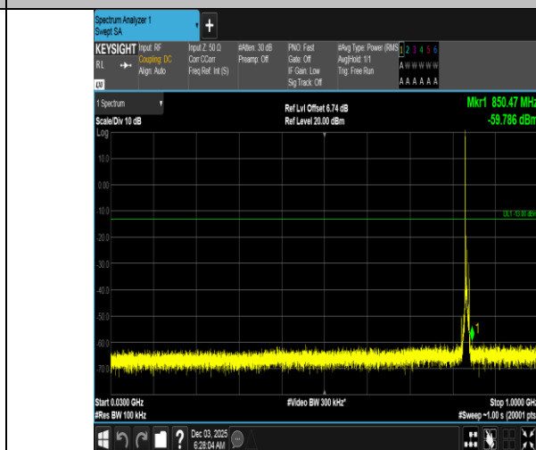
Band5-5MHz-16QAM-20525-1RB#0-30~1000-PASS
