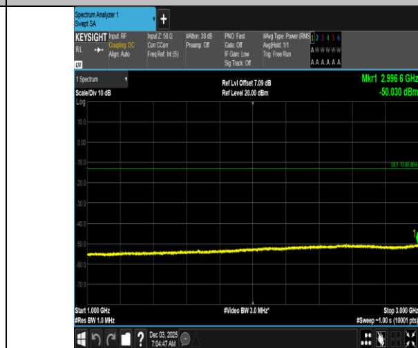
Band5-10MHz-QPSK-20525-50RB#0-1000~3000-PASS
