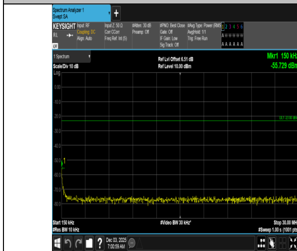
Band5-10MHz-16QAM-20525-1RB#0-0.15~30-PASS
