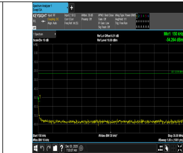
Band5-10MHz-16QAM-20525-1RB#49-0.15~30-PASS
