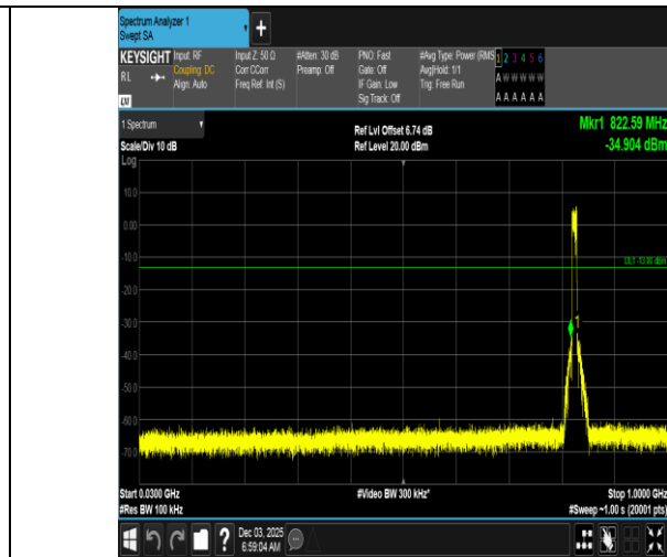
Band5-10MHz-16QAM-20450-50RB#0-30~1000-PASS
