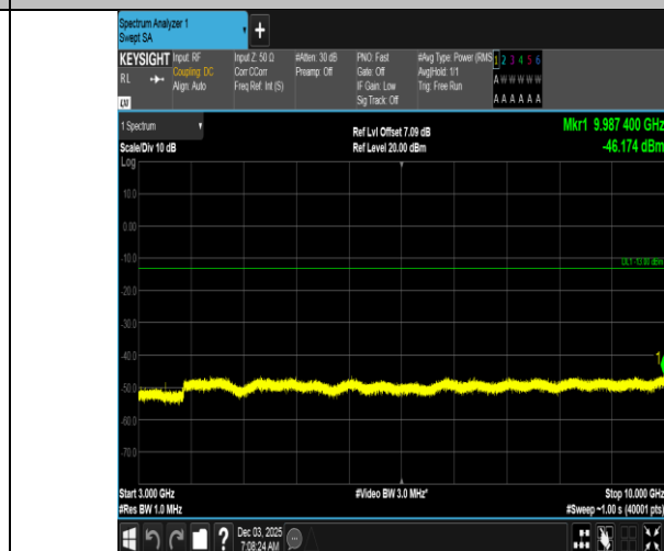
Band5-10MHz-16QAM-20600-1RB#0-3000~10000-PASS
