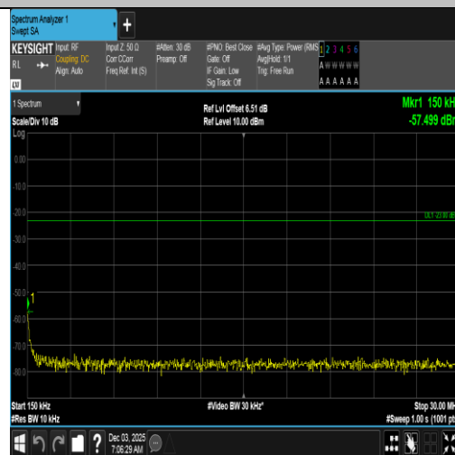
Band5-10MHz-QPSK-20600-1RB#0-0.15~30-PASS
