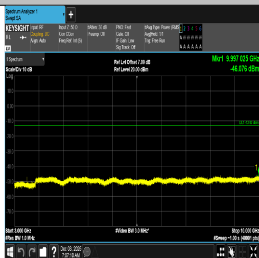
Band5-10MHz-QPSK-20600-1RB#0-3000~10000-PASS
