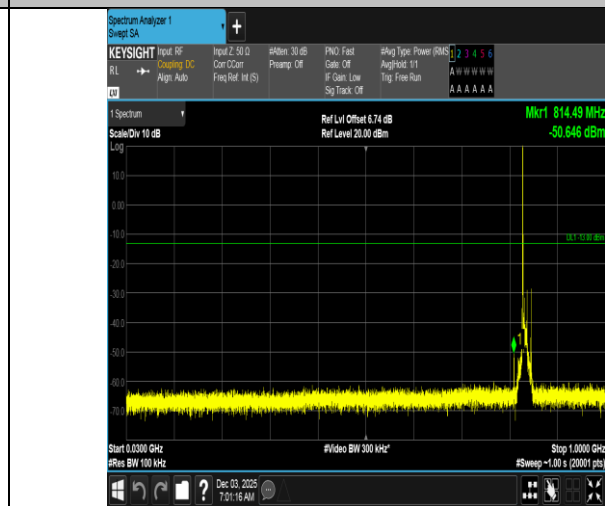
Band5-10MHz-16QAM-20525-1RB#0-30~1000-PASS
