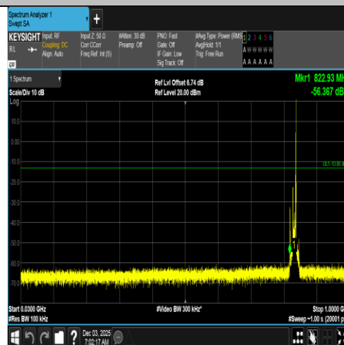
Band5-10MHz-QPSK-20525-1RB#49-30~1000-PASS
