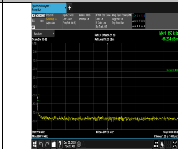
Band5-10MHz-QPSK-20525-50RB#0-0.15~30-PASS
