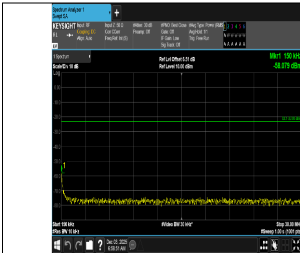
Band5-10MHz-16QAM-20450-50RB#0-0.15~30-PASS
