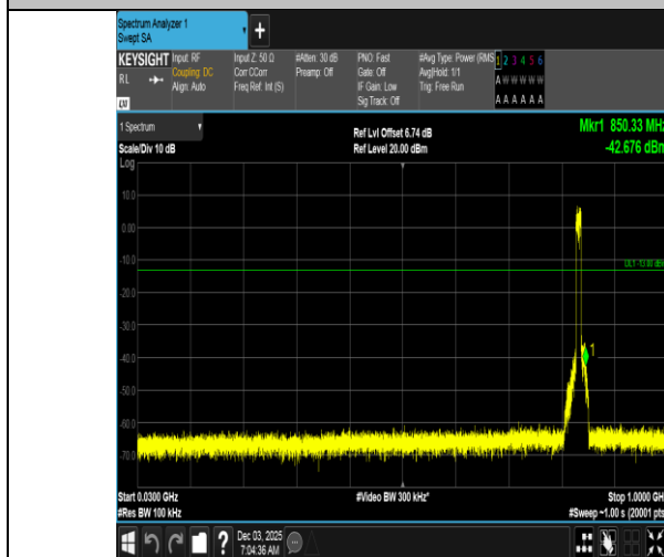
Band5-10MHz-QPSK-20525-50RB#0-30~1000-PASS
