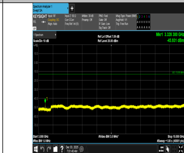
Band5-10MHz-16QAM-20525-1RB#0-3000~10000-PASS
