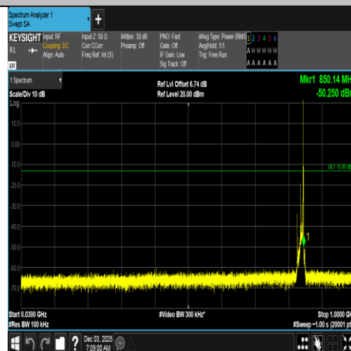
Band5-10MHz-QPSK-20600-1RB#49-30~1000-PASS
