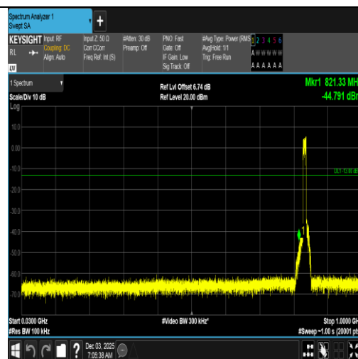
Band5-10MHz-16QAM-20525-50RB#0-30~1000-PASS
