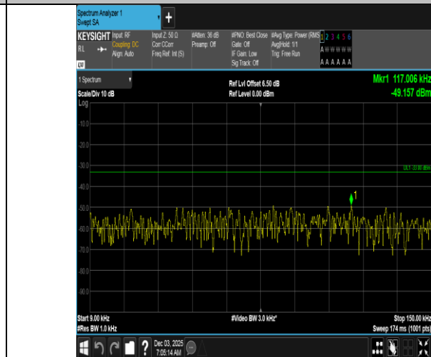
Band5-10MHz-16QAM-20525-50RB#0-0.009~0.15-PASS
