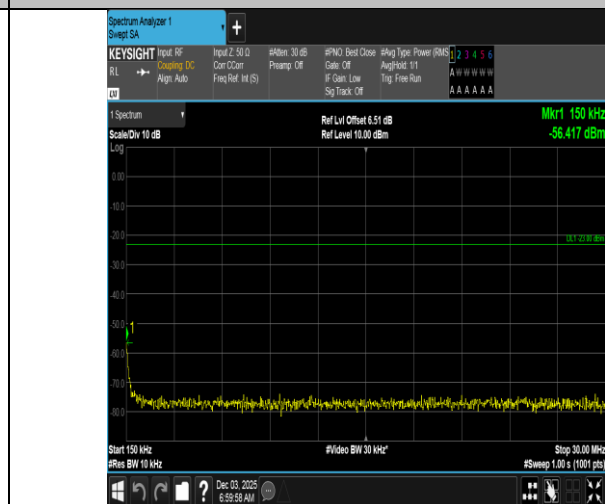
Band5-10MHz-QPSK-20525-1RB#0-0.15~30-PASS
