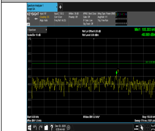
Band5-10MHz-QPSK-20525-1RB#0-0.009~0.15-PASS
