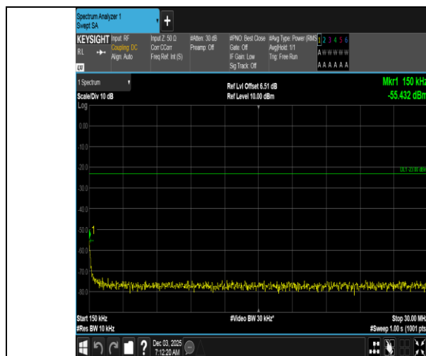
Band5-10MHz-16QAM-20600-50RB#0-0.15~30-PASS
