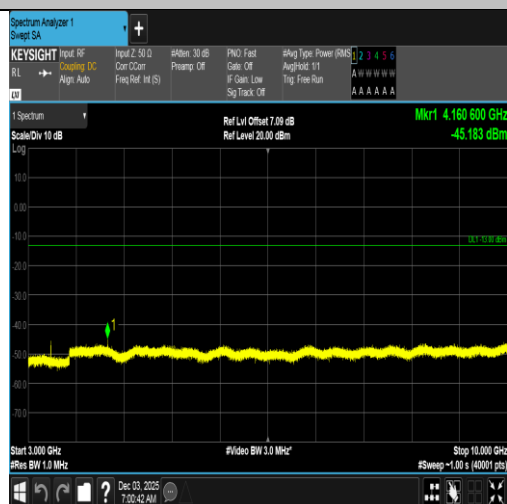
Band5-10MHz-QPSK-20525-1RB#0-3000~10000-PASS
