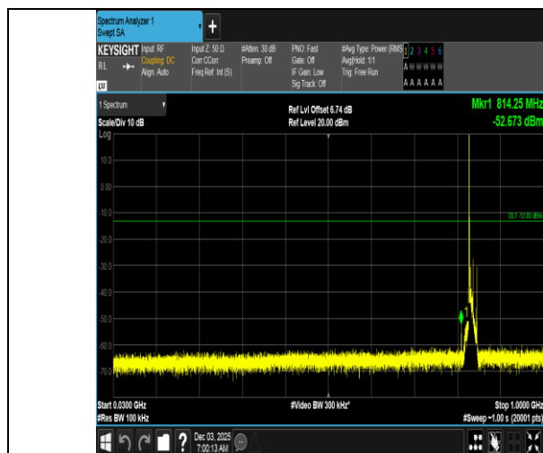
Band5-10MHz-QPSK-20525-1RB#0-30~1000-PASS
