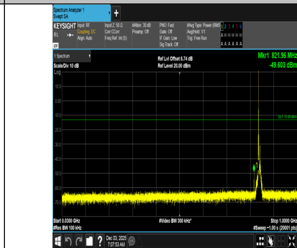
Band5-10MHz-16QAM-20600-1RB#0-30~1000-PASS
