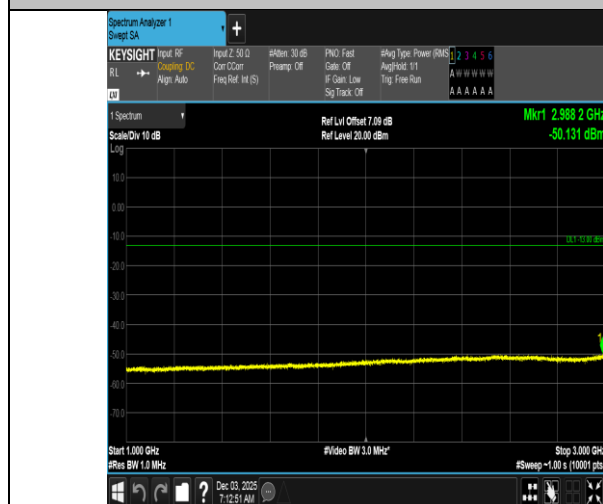
Band5-10MHz-16QAM-20600-50RB#0-1000~3000-PASS
