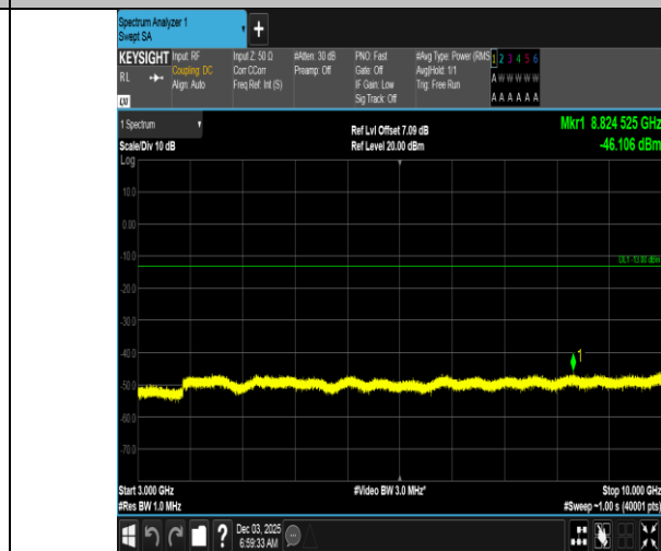
Band5-10MHz-16QAM-20450-50RB#0-3000~10000-PASS
