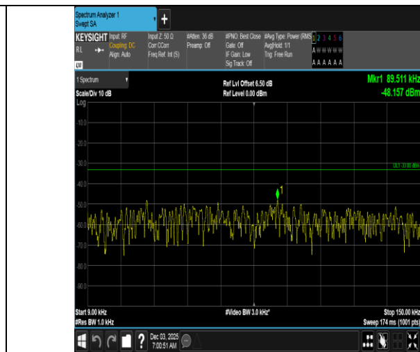
Band5-10MHz-16QAM-20525-1RB#0-0.009~0.15-PASS
