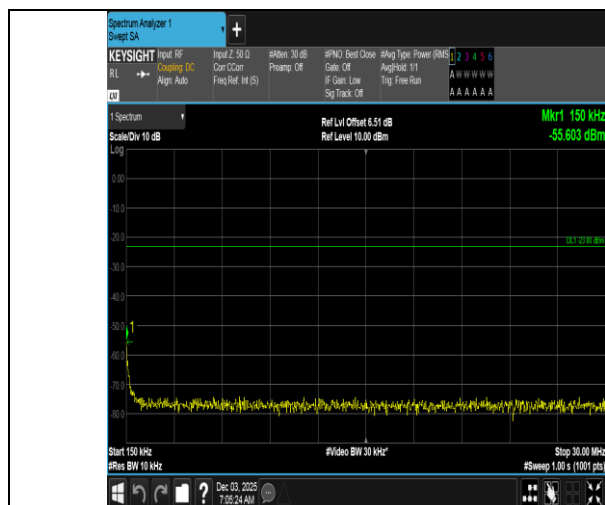
Band5-10MHz-16QAM-20525-50RB#0-0.15~30-PASS
