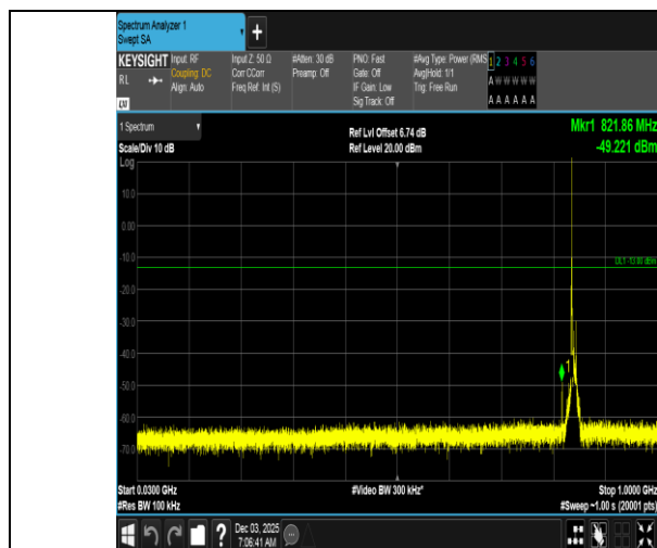
Band5-10MHz-QPSK-20600-1RB#0-30~1000-PASS
