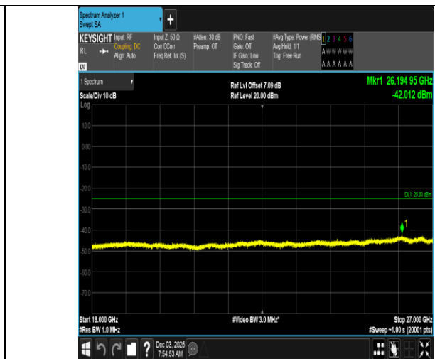
Band7-5MHz-QPSK-20775-25RB#0-18000~27000-PASS
