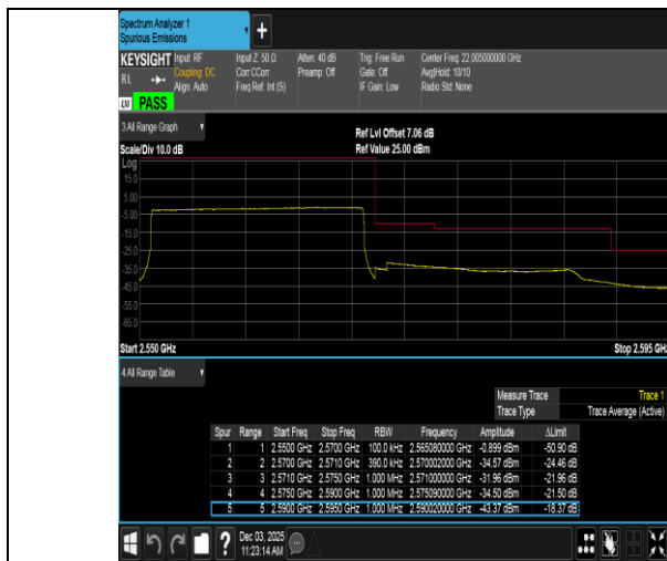
Band7-20MHz-QPSK-21350-100RB#0-PASS
