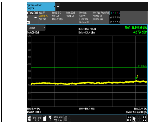
Band7-5MHz-QPSK-20775-1RB#24-18000~27000-PASS
