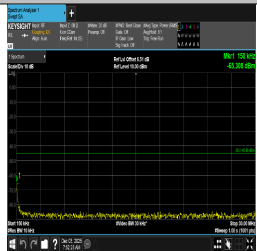
Band7-5MHz-16QAM-20775-1RB#24-0.15~30-PASS
