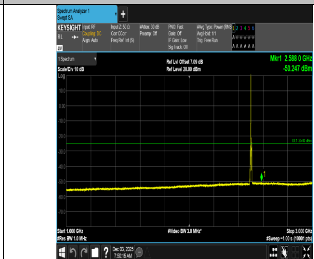
Band7-5MHz-16QAM-20775-1RB#0-1000~3000-PASS
