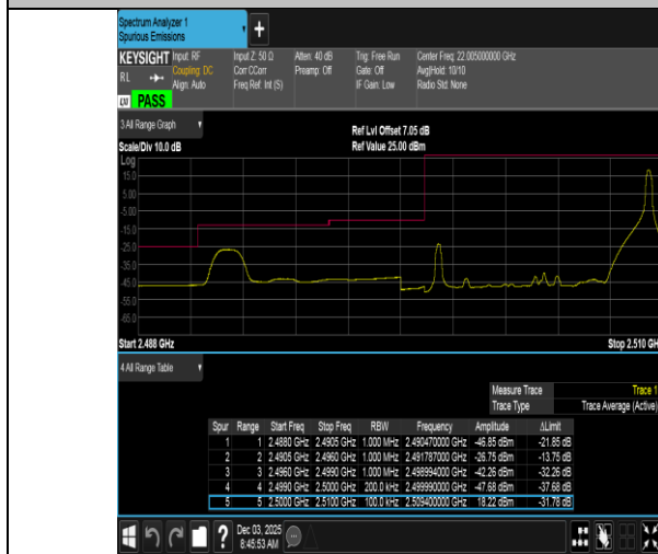
Band7-10MHz-16QAM-20800-1RB#49-PASS
