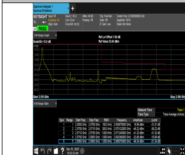
Band7-15MHz-QPSK-21375-1RB#0-PASS
