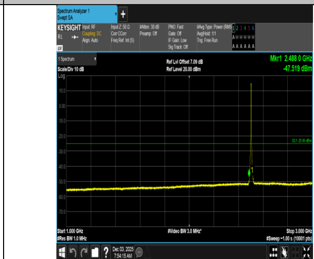
Band7-5MHz-QPSK-20775-25RB#0-1000~3000-PASS
