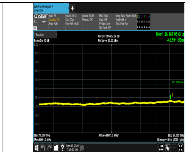
Band7-5MHz-QPSK-20775-1RB#0-18000~27000-PASS
