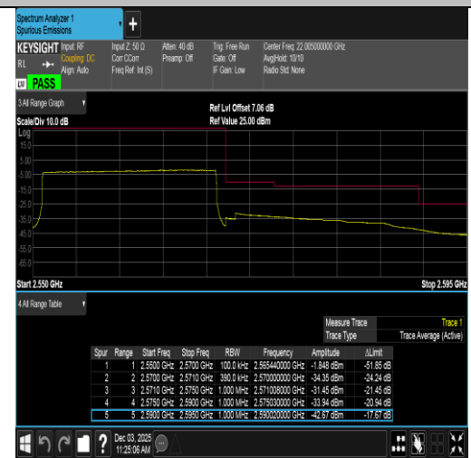
Band7-20MHz-16QAM-21350-100RB#0-PASS
