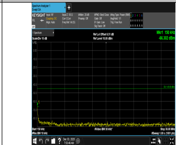
Band7-5MHz-QPSK-20775-25RB#0-0.15~30-PASS
