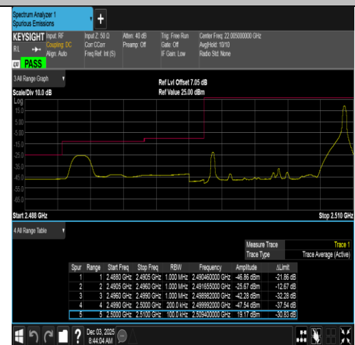
Band7-10MHz-QPSK-20800-1RB#49-PASS
