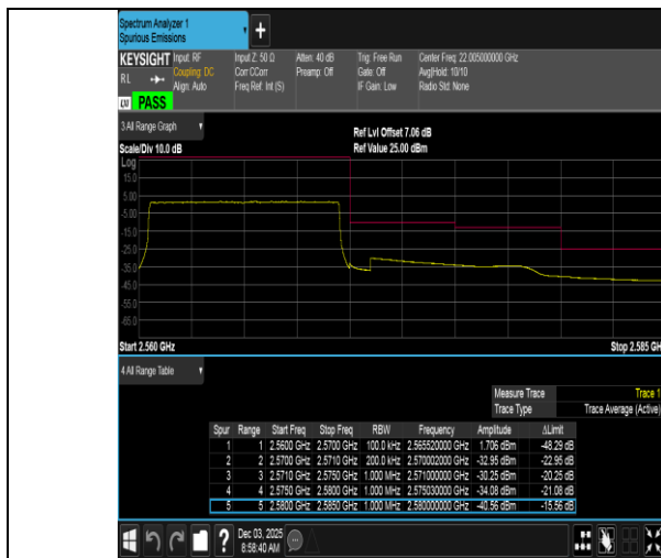
Band7-10MHz-QPSK-21400-50RB#0-PASS
