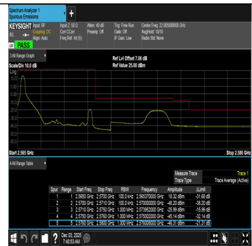
Band7-5MHz-16QAM-21425-1RB#0-PASS
