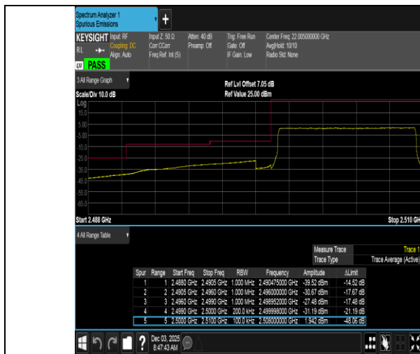
Band7-10MHz-QPSK-20800-50RB#0-PASS
