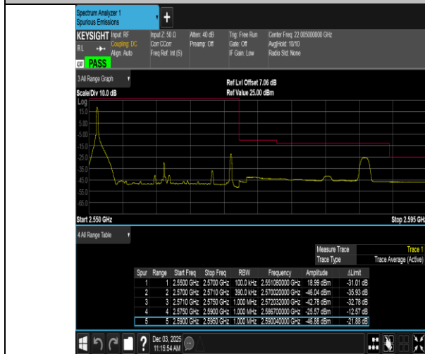
Band7-20MHz-QPSK-21350-1RB#0-PASS
