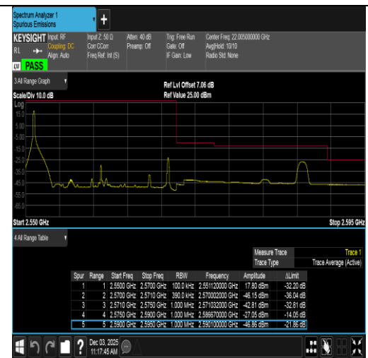
Band7-20MHz-16QAM-21350-1RB#0-PASS
