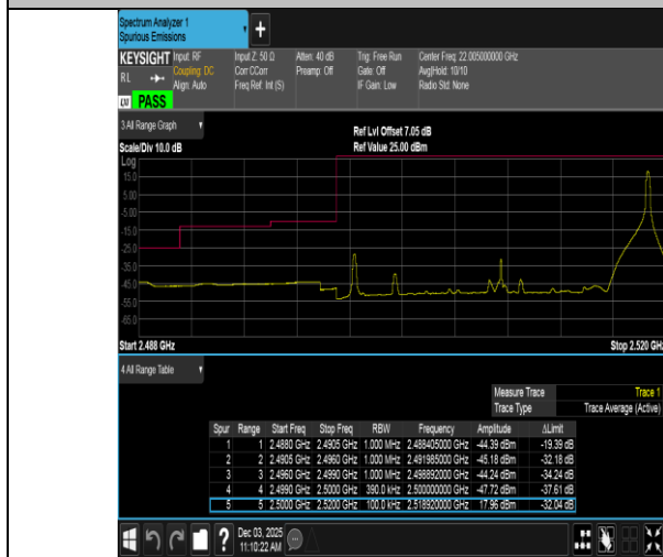
Band7-20MHz-16QAM-20850-1RB#99-PASS
