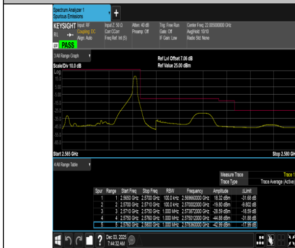
Band7-5MHz-16QAM-21425-1RB#24-PASS
