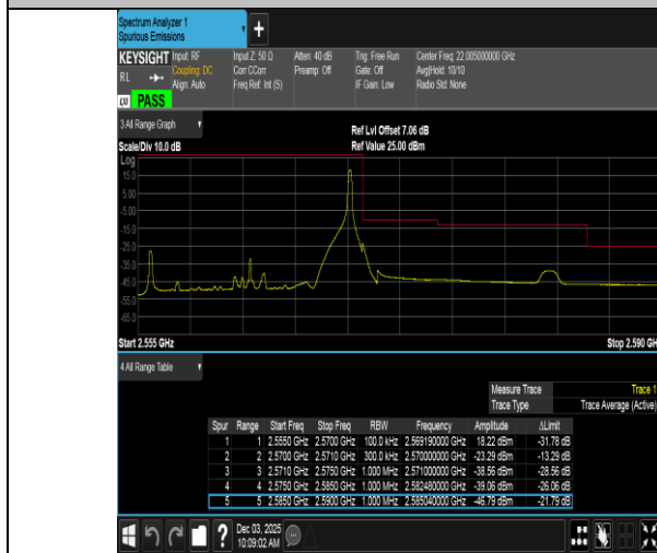
Band7-15MHz-16QAM-21375-1RB#74-PASS
