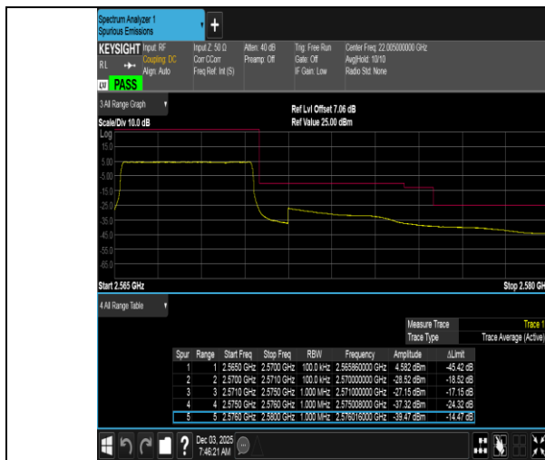
Band7-5MHz-QPSK-21425-25RB#0-PASS
