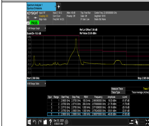
Band7-10MHz-16QAM-21400-1RB#49-PASS
