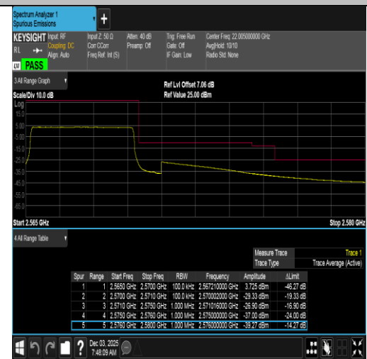
Band7-5MHz-16QAM-21425-25RB#0-PASS
