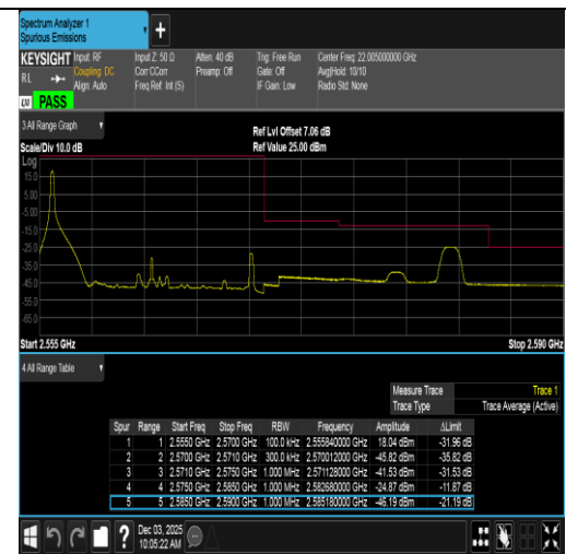
Band7-15MHz-16QAM-21375-1RB#0-PASS
