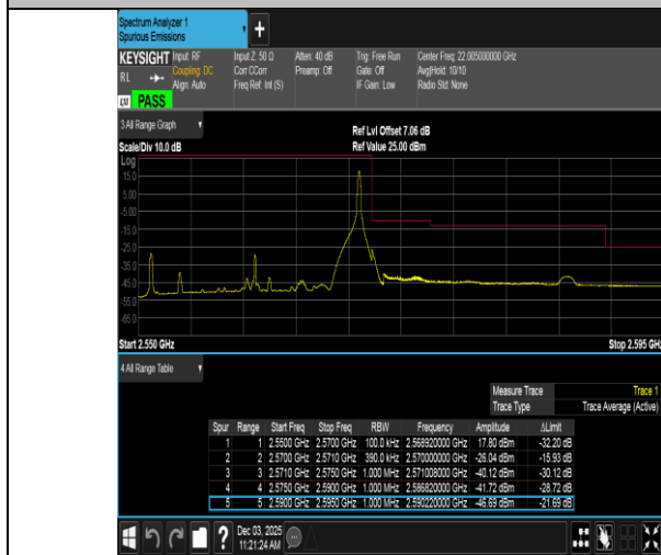
Band7-20MHz-16QAM-21350-1RB#99-PASS
