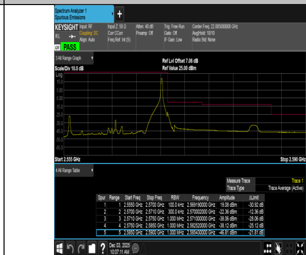
Band7-15MHz-QPSK-21375-1RB#74-PASS
