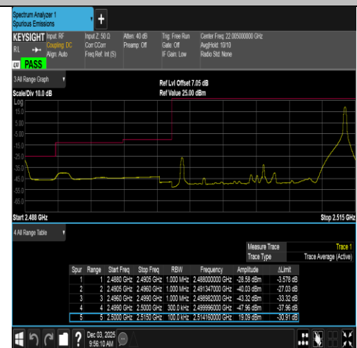
Band7-15MHz-QPSK-20825-1RB#74-PASS
