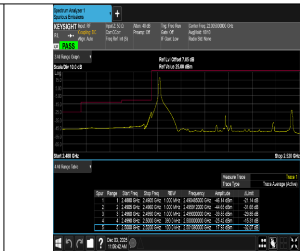
Band7-20MHz-16QAM-20850-1RB#0-PASS
