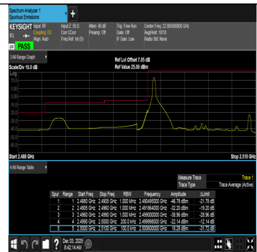
Band7-10MHz-16QAM-20800-1RB#0-PASS
