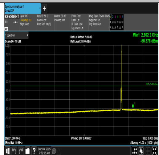
Band7-5MHz-16QAM-20775-1RB#24-1000~3000-PASS
