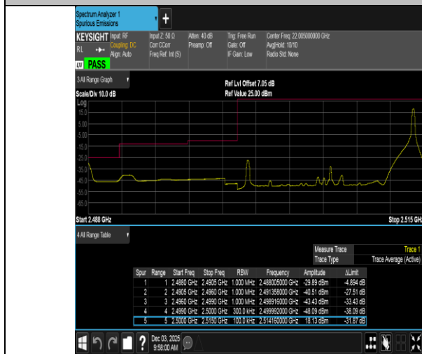
Band7-15MHz-16QAM-20825-1RB#74-PASS
