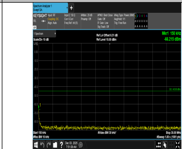
Band7-5MHz-QPSK-20775-1RB#24-0.15~30-PASS
