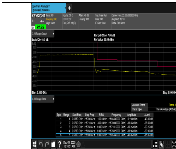
Band7-15MHz-QPSK-21375-75RB#0-PASS
