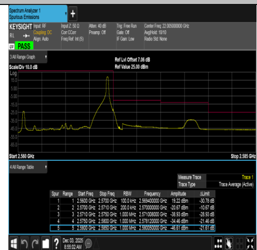
Band7-10MHz-QPSK-21400-1RB#49-PASS
