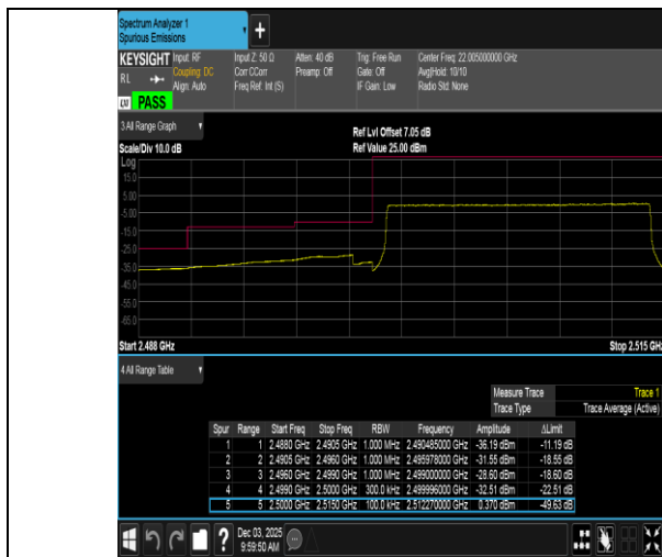
Band7-15MHz-QPSK-20825-75RB#0-PASS
