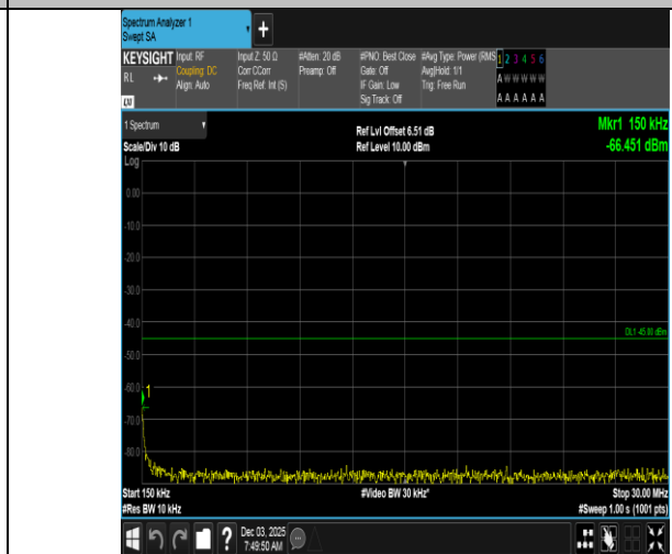
Band7-5MHz-16QAM-20775-1RB#0-0.15~30-PASS
