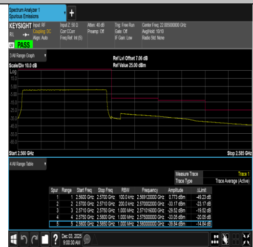
Band7-10MHz-16QAM-21400-50RB#0-PASS
