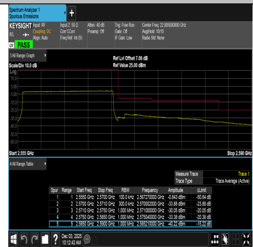
Band7-15MHz-16QAM-21375-75RB#0-PASS
