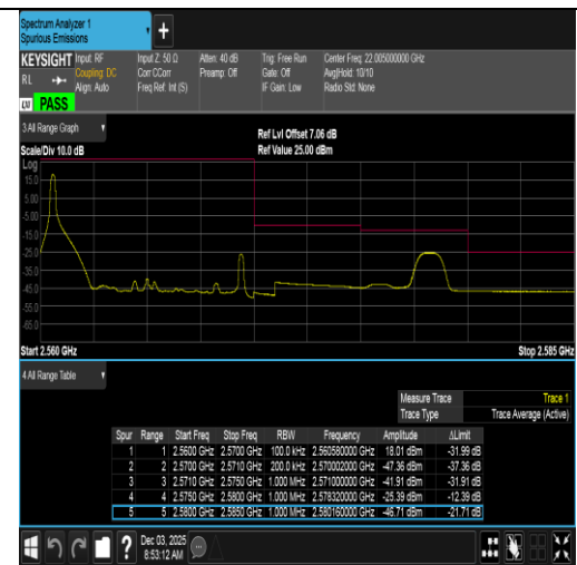
Band7-10MHz-16QAM-21400-1RB#0-PASS
