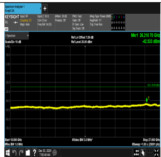
Band7-5MHz-16QAM-20775-1RB#0-18000~27000-PASS
