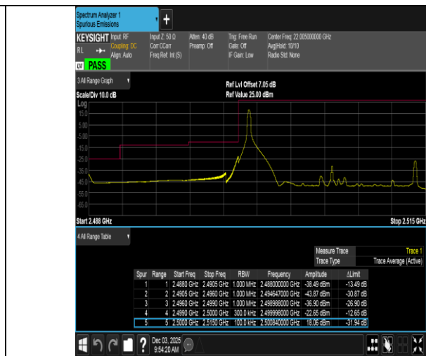
Band7-15MHz-16QAM-20825-1RB#0-PASS
