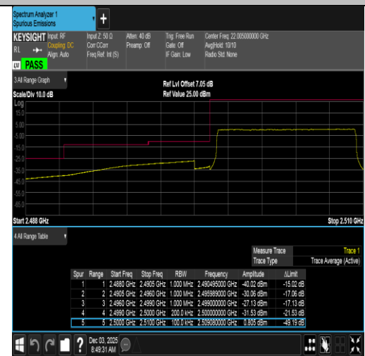
Band7-10MHz-16QAM-20800-50RB#0-PASS
