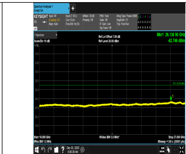
Band7-5MHz-QPSK-21425-1RB#0-18000~27000-PASS
