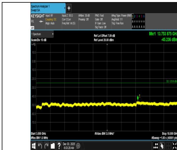
Band7-5MHz-QPSK-21100-25RB#0-3000~18000-PASS
