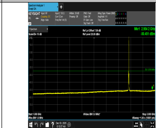
Band7-5MHz-16QAM-21425-1RB#24-1000~3000-PASS
