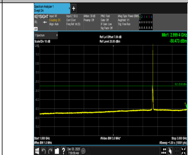
Band7-5MHz-QPSK-21100-1RB#24-1000~3000-PASS
