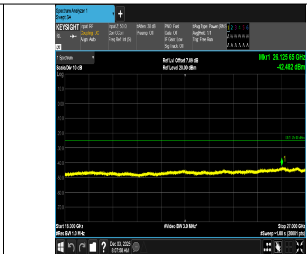
Band7-5MHz-16QAM-21425-1RB#0-18000~27000-PASS
