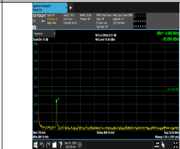
Band7-5MHz-QPSK-21425-1RB#0-0.15~30-PASS
