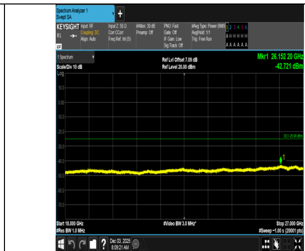
Band7-5MHz-QPSK-21425-1RB#24-18000~27000-PASS
