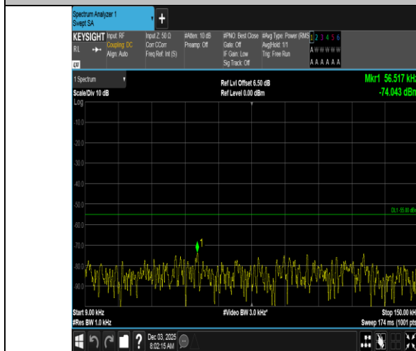
Band7-5MHz-QPSK-21100-25RB#0-0.009~0.15-PASS
