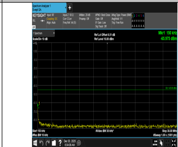
Band7-5MHz-16QAM-21100-25RB#0-0.15~30-PASS
