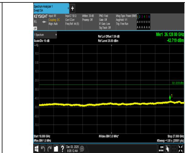
Band7-5MHz-16QAM-21100-25RB#0-18000~27000-PASS
