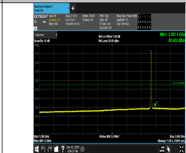
Band7-5MHz-16QAM-21100-25RB#0-1000~3000-PASS
