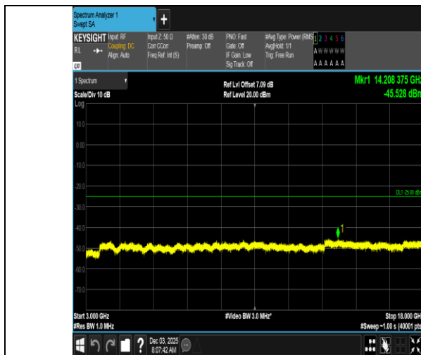
Band7-5MHz-16QAM-21425-1RB#0-3000~18000-PASS
