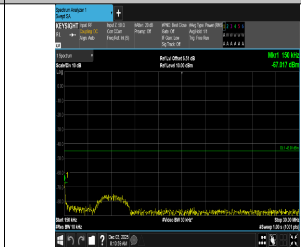
Band7-5MHz-QPSK-21425-25RB#0-0.15~30-PASS
