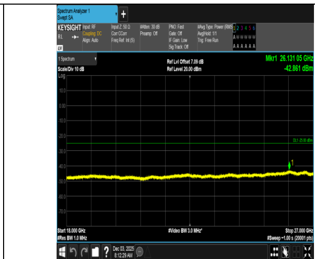
Band7-5MHz-QPSK-21425-25RB#0-18000~27000-PASS
