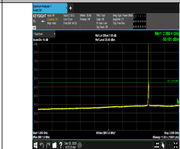
Band7-5MHz-16QAM-21425-1RB#0-1000~3000-PASS
