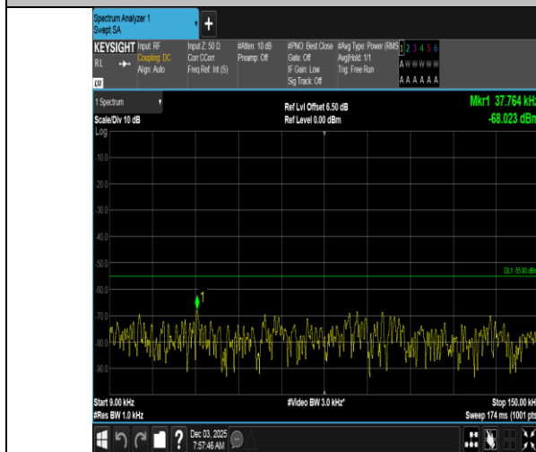
Band7-5MHz-16QAM-21100-1RB#0-0.009~0.15-PASS
