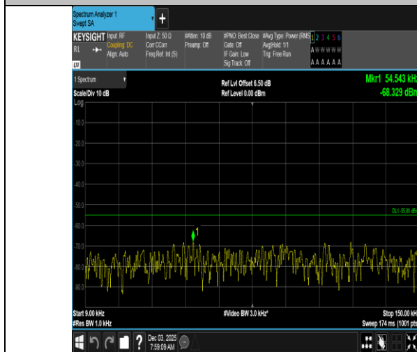
Band7-5MHz-QPSK-21100-1RB#24-0.009~0.15-PASS
