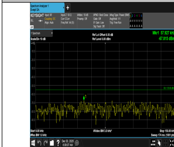
Band7-5MHz-QPSK-21425-1RB#24-0.009~0.15-PASS
