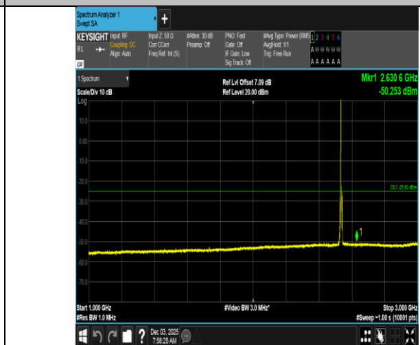
Band7-5MHz-16QAM-21100-1RB#0-1000~3000-PASS
