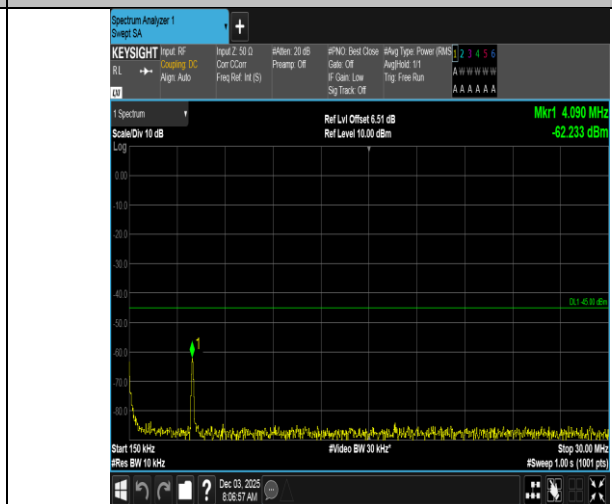
Band7-5MHz-16QAM-21425-1RB#0-0.15~30-PASS
