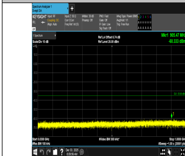
Band7-5MHz-16QAM-21425-1RB#24-30~1000-PASS
