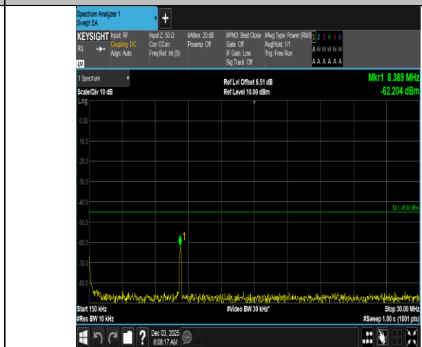
Band7-5MHz-QPSK-21425-1RB#24-0.15~30-PASS
