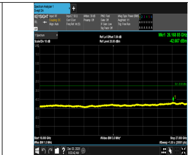
Band7-5MHz-QPSK-21100-25RB#0-18000~27000-PASS
