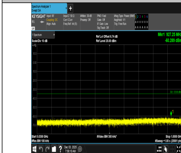
Band7-5MHz-16QAM-21100-1RB#0-30~1000-PASS
