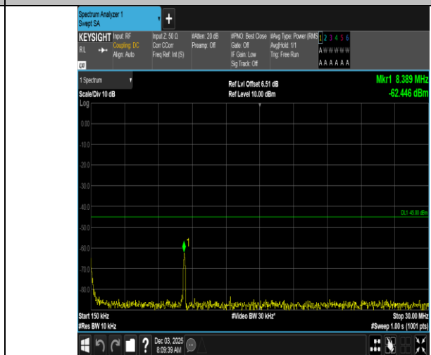
Band7-5MHz-16QAM-21425-1RB#24-0.15~30-PASS
