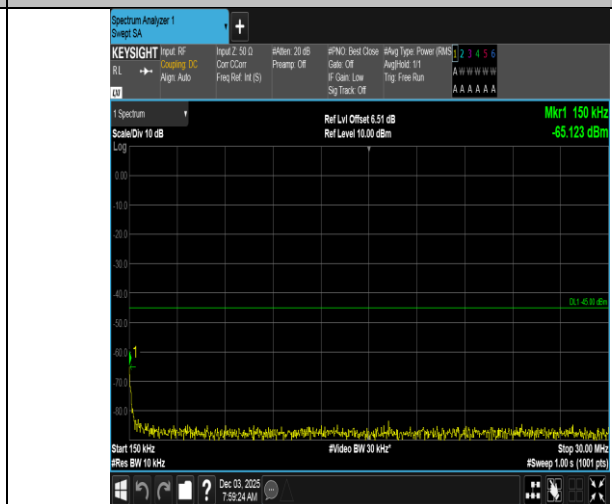
Band7-5MHz-QPSK-21100-1RB#24-0.15~30-PASS
