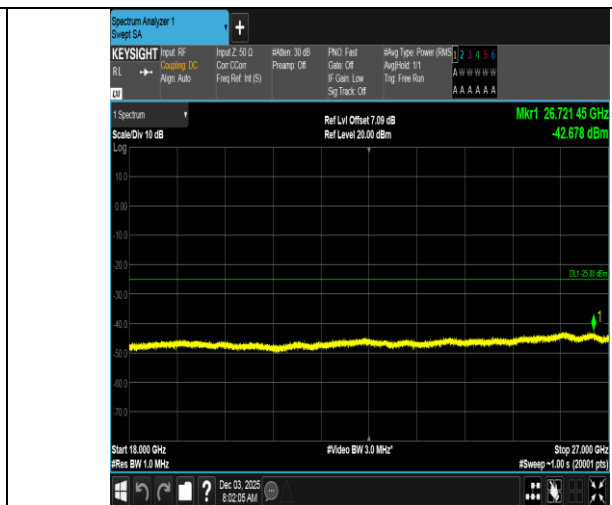
Band7-5MHz-16QAM-21100-1RB#24-18000~27000-PASS
