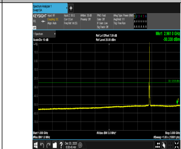
Band7-5MHz-QPSK-21425-1RB#24-1000~3000-PASS
