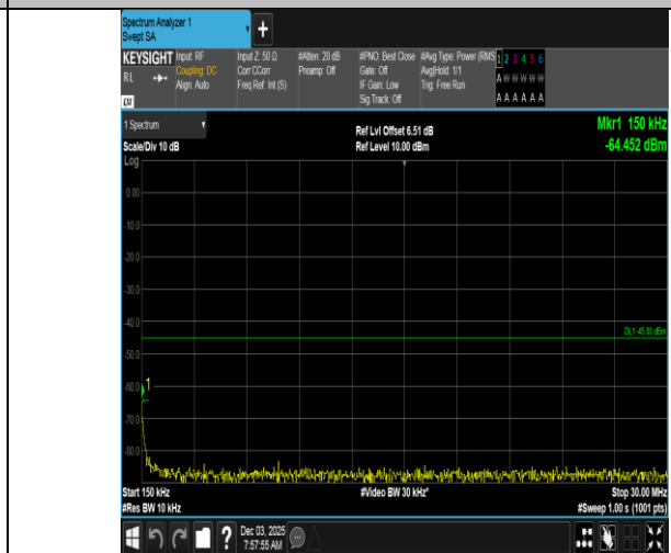
Band7-5MHz-16QAM-21100-1RB#0-0.15~30-PASS
