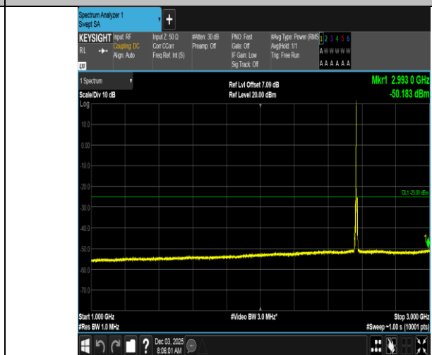
Band7-5MHz-QPSK-21425-1RB#0-1000~3000-PASS
