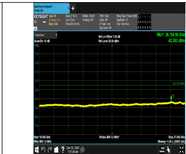
Band7-5MHz-QPSK-21100-1RB#0-18000~27000-PASS
