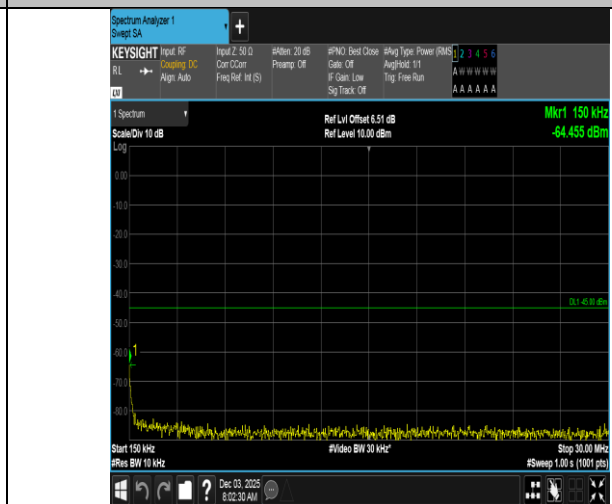
Band7-5MHz-QPSK-21100-25RB#0-0.15~30-PASS
