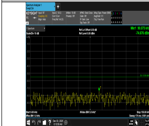
Band7-5MHz-QPSK-21425-25RB#0-0.009~0.15-PASS
