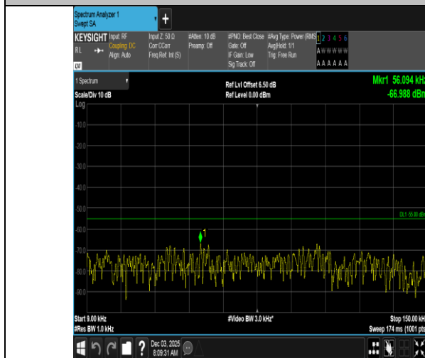
Band7-5MHz-16QAM-21425-1RB#24-0.009~0.15-PASS
