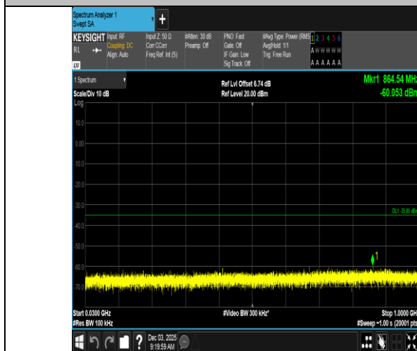
Band7-10MHz-QPSK-21400-1RB#49-30~1000-PASS
