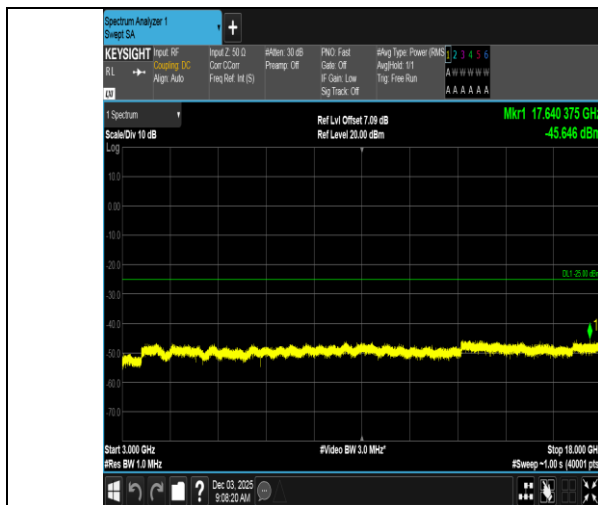
Band7-10MHz-16QAM-20800-50RB#0-3000~18000-PASS
