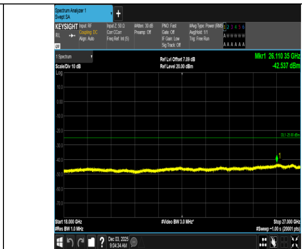
Band7-10MHz-QPSK-20800-1RB#49-18000~27000-PASS
