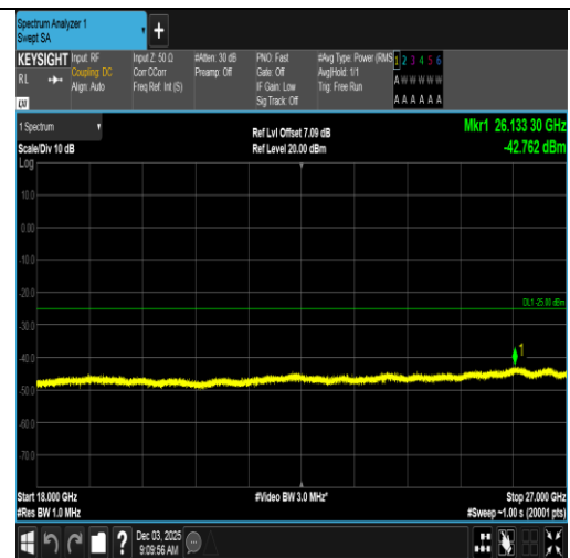
Band7-10MHz-QPSK-21100-1RB#0-18000~27000-PASS
