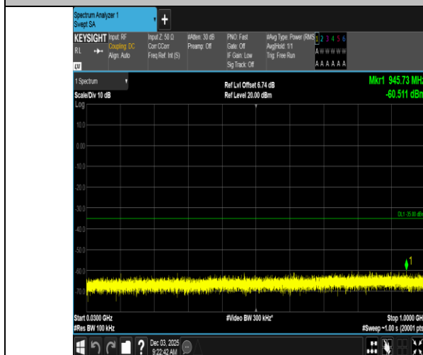
Band7-10MHz-QPSK-21400-50RB#0-30~1000-PASS
