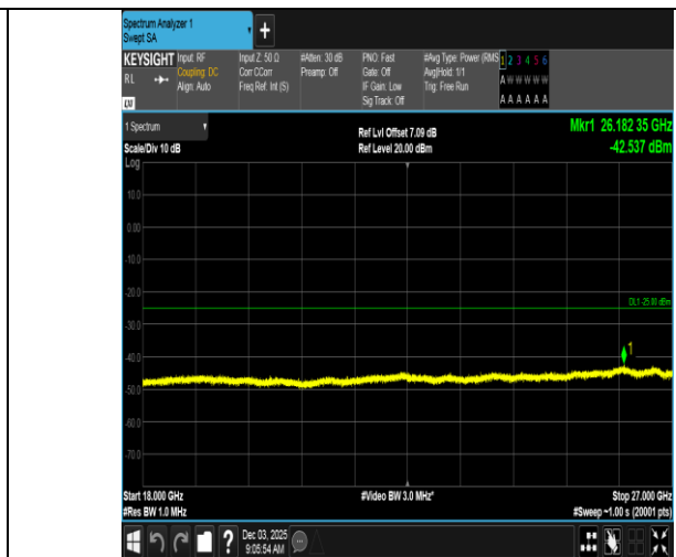
Band7-10MHz-16QAM-20800-1RB#49-18000~27000-PASS
