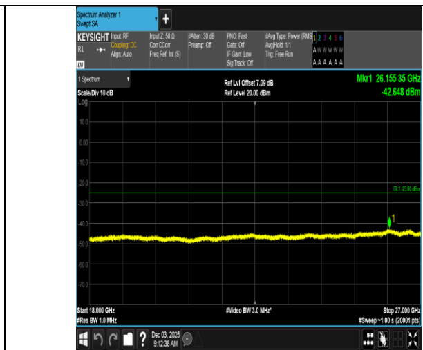
Band7-10MHz-QPSK-21100-1RB#49-18000~27000-PASS
