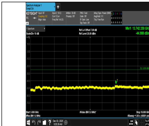
Band7-10MHz-16QAM-20800-1RB#49-3000~18000-PASS
