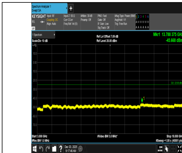
Band7-10MHz-QPSK-21400-1RB#0-3000~18000-PASS
