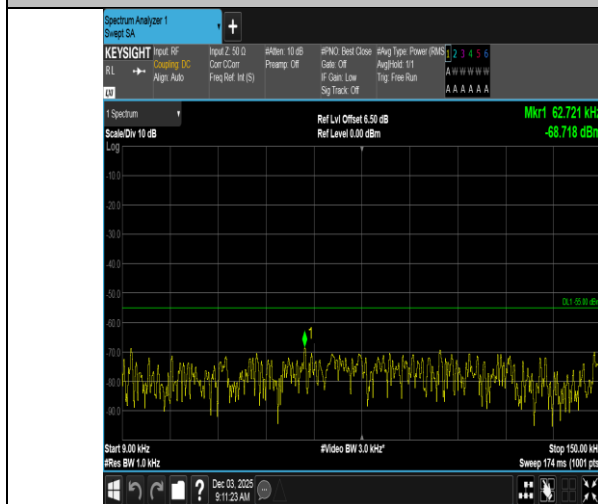
Band7-10MHz-QPSK-21100-1RB#49-0.009~0.15-PASS
