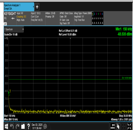
Band7-10MHz-QPSK-21100-1RB#49-0.15~30-PASS
