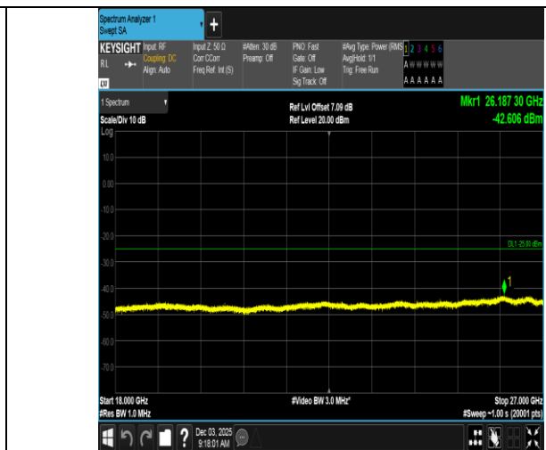
Band7-10MHz-QPSK-21400-1RB#0-18000~27000-PASS
