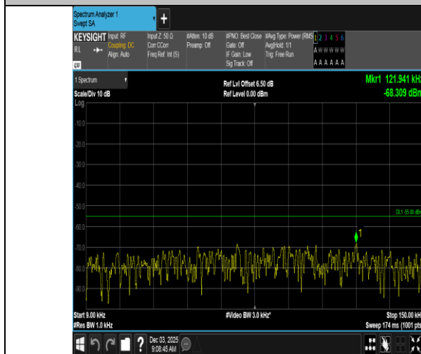
Band7-10MHz-QPSK-21100-1RB#0-0.009~0.15-PASS
