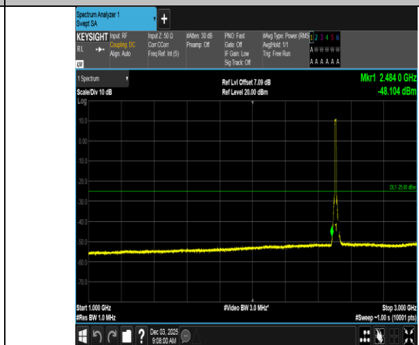
Band7-10MHz-16QAM-20800-50RB#0-1000~3000-PASS
