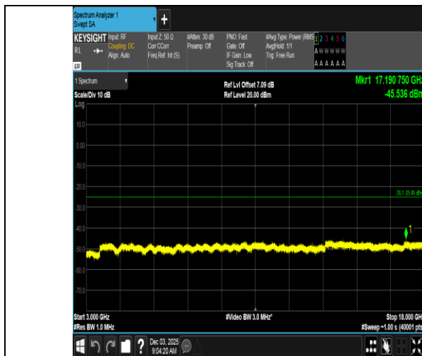
Band7-10MHz-QPSK-20800-1RB#49-3000~18000-PASS
