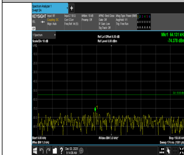
Band7-10MHz-QPSK-21100-50RB#0-0.009~0.15-PASS
