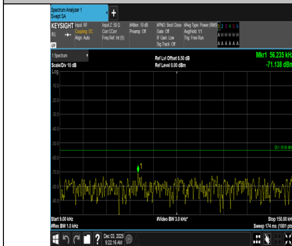
Band7-10MHz-QPSK-21400-50RB#0-0.009~0.15-PASS
