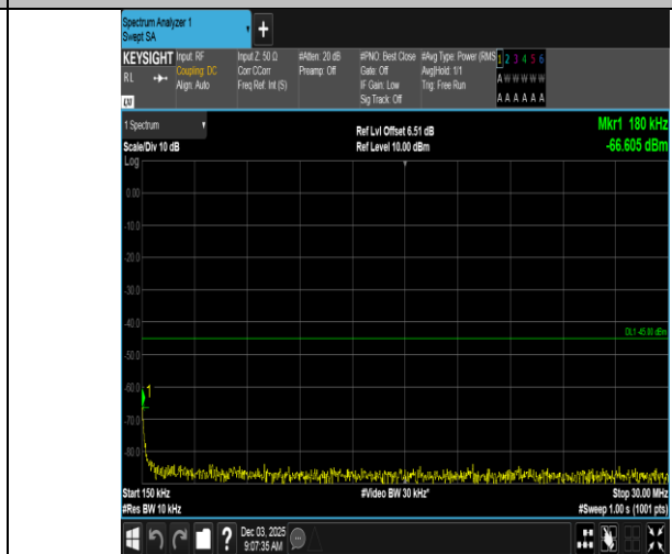
Band7-10MHz-16QAM-20800-50RB#0-0.15~30-PASS
