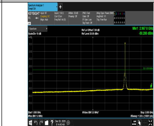
Band7-10MHz-QPSK-21100-50RB#0-1000~3000-PASS
