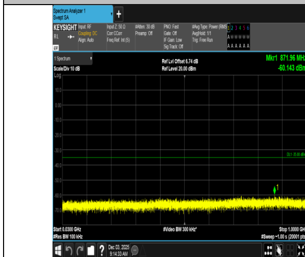
Band7-10MHz-QPSK-21100-50RB#0-30~1000-PASS
