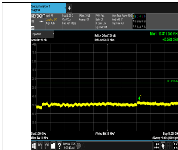
Band7-10MHz-QPSK-21100-1RB#0-3000~18000-PASS
