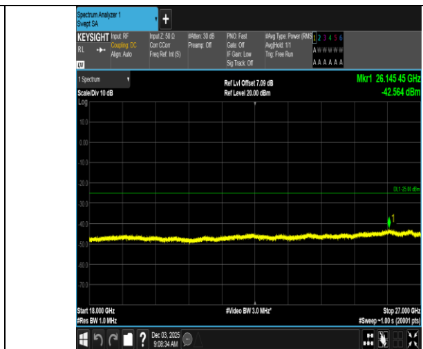
Band7-10MHz-16QAM-20800-50RB#0-18000~27000-PASS
