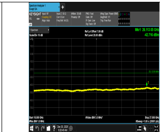
Band7-10MHz-QPSK-21400-1RB#49-18000~27000-PASS
