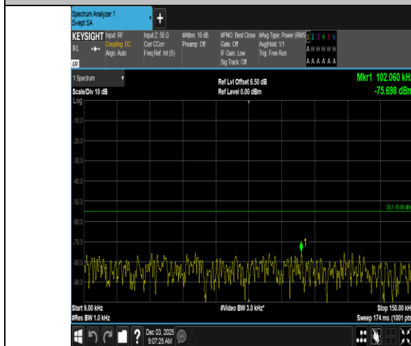
Band7-10MHz-16QAM-20800-50RB#0-0.009~0.15-PASS
