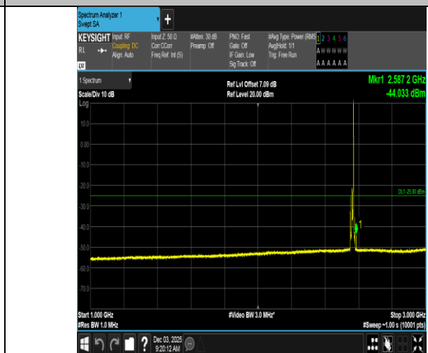
Band7-10MHz-QPSK-21400-1RB#49-1000~3000-PASS
