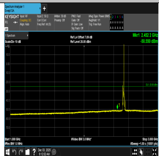
Band7-10MHz-QPSK-21100-1RB#49-1000~3000-PASS
