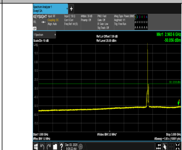
Band7-10MHz-QPSK-21100-1RB#0-1000~3000-PASS
