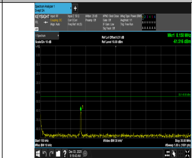
Band7-10MHz-QPSK-21400-1RB#49-0.15~30-PASS
