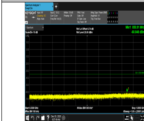
Band7-10MHz-16QAM-20800-50RB#0-30~1000-PASS
