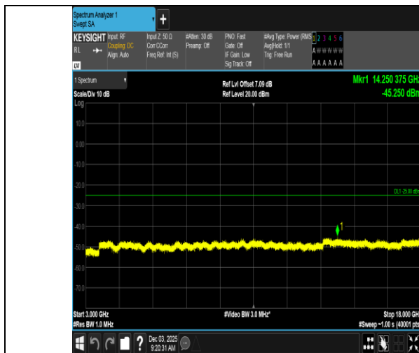
Band7-10MHz-QPSK-21400-1RB#49-3000~18000-PASS
