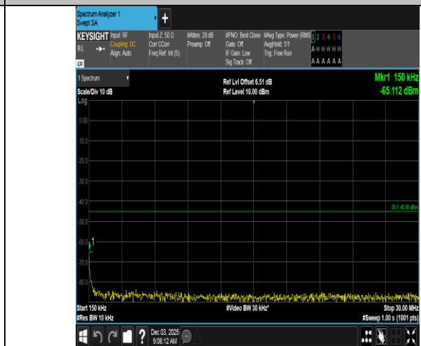
Band7-10MHz-QPSK-20800-50RB#0-0.15~30-PASS
