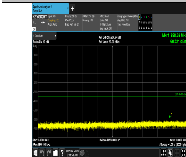
Band7-10MHz-QPSK-21100-1RB#49-30~1000-PASS
