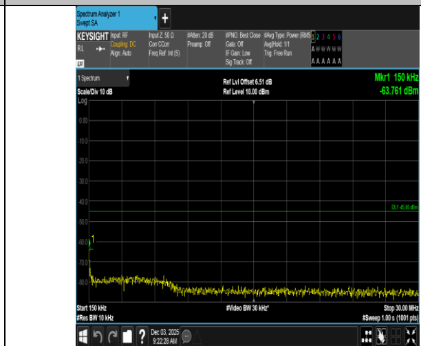
Band7-10MHz-QPSK-21400-50RB#0-0.15~30-PASS
