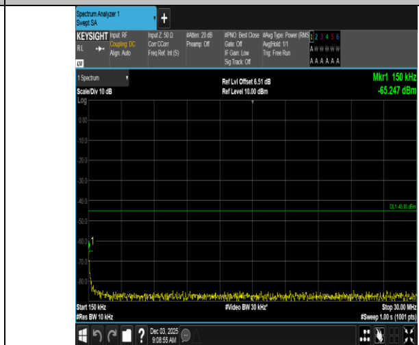
Band7-10MHz-QPSK-21100-1RB#0-0.15~30-PASS
