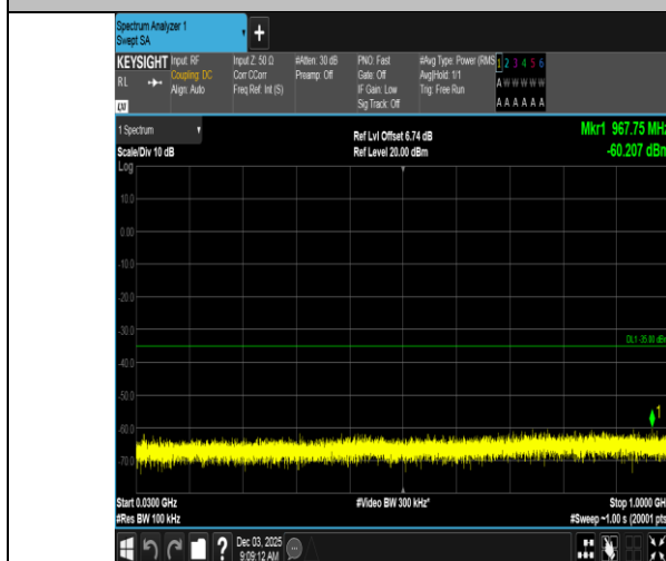
Band7-10MHz-QPSK-21100-1RB#0-30~1000-PASS
