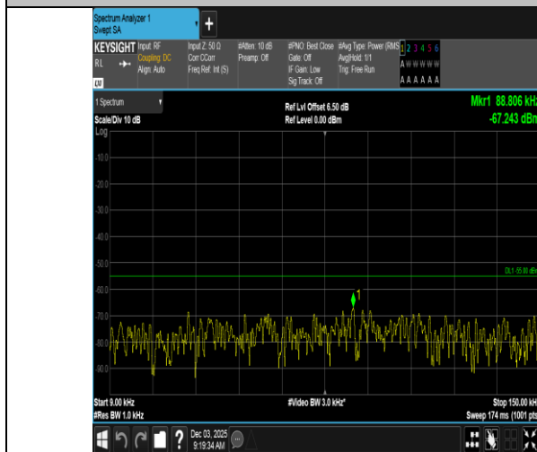
Band7-10MHz-QPSK-21400-1RB#49-0.009~0.15-PASS
