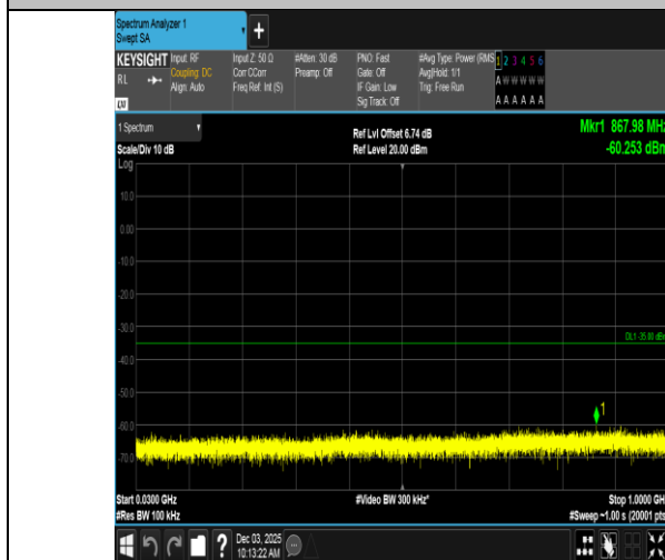
Band7-15MHz-QPSK-20825-1RB#0-30~1000-PASS
