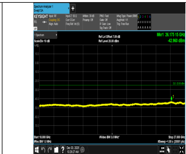
Band7-15MHz-16QAM-21100-75RB#0-18000~27000-PASS
