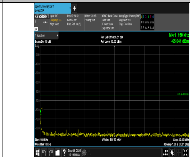
Band7-15MHz-16QAM-20825-75RB#0-0.15~30-PASS
