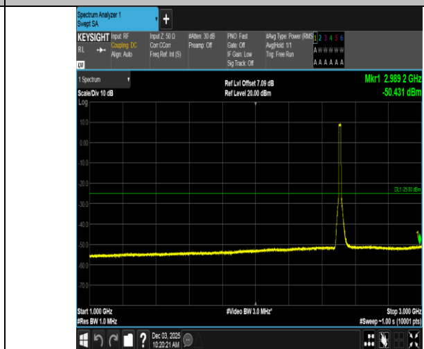
Band7-15MHz-16QAM-20825-75RB#0-1000~3000-PASS
