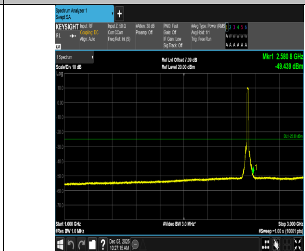
Band7-15MHz-QPSK-21100-75RB#0-1000~3000-PASS
