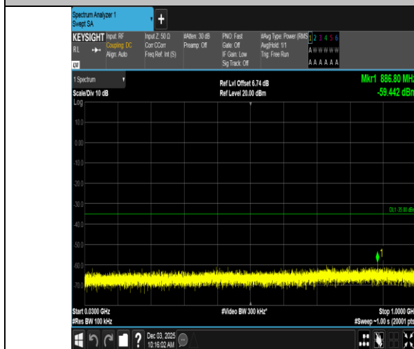
Band7-15MHz-QPSK-20825-1RB#74-30~1000-PASS
