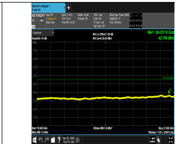
Band7-15MHz-QPSK-21100-75RB#0-18000~27000-PASS
