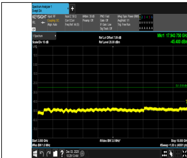
Band7-15MHz-16QAM-21100-75RB#0-3000~18000-PASS
