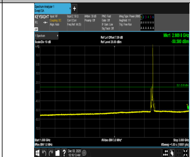
Band7-15MHz-QPSK-20825-1RB#74-1000~3000-PASS
