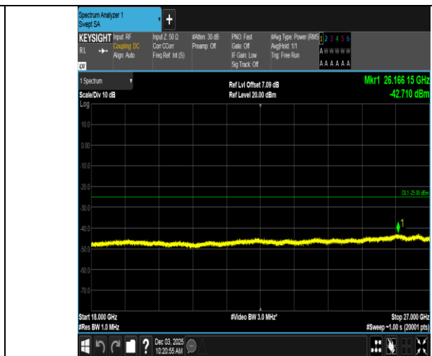
Band7-15MHz-16QAM-20825-75RB#0-18000~27000-PASS
