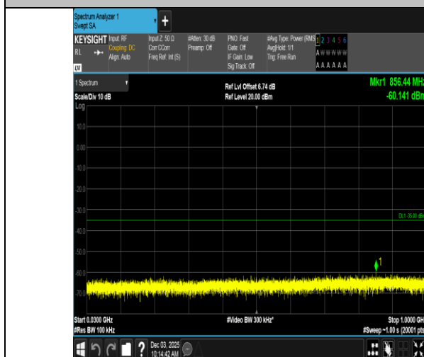
Band7-15MHz-16QAM-20825-1RB#0-30~1000-PASS
