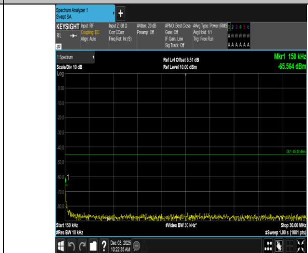
Band7-15MHz-16QAM-21100-1RB#0-0.15~30-PASS
