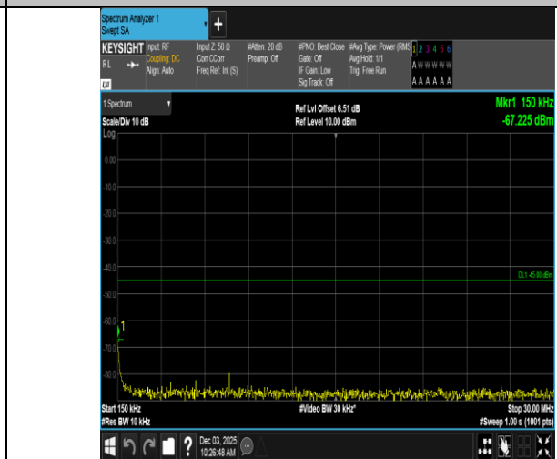
Band7-15MHz-QPSK-21100-75RB#0-0.15~30-PASS
