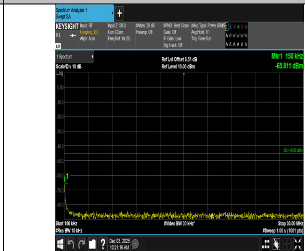
Band7-15MHz-QPSK-21100-1RB#0-0.15~30-PASS
