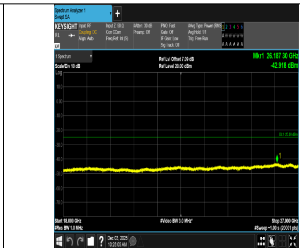
Band7-15MHz-QPSK-21100-1RB#74-18000~27000-PASS
