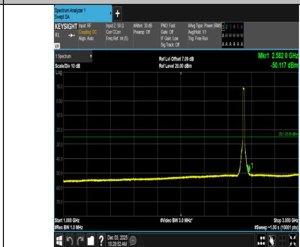
Band7-15MHz-16QAM-21100-75RB#0-1000~3000-PASS
