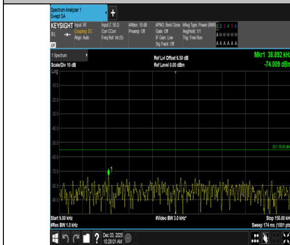
Band7-15MHz-16QAM-21100-75RB#0-0.009~0.15-PASS
