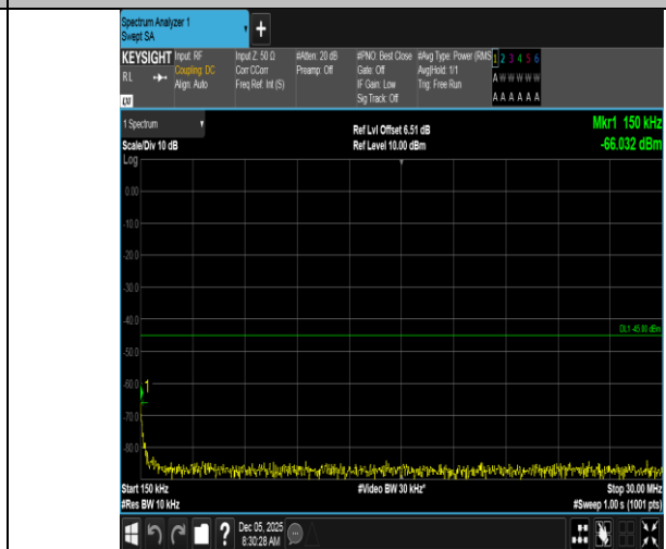
Band7-15MHz-QPSK-21375-1RB#0-0.15~30-PASS
