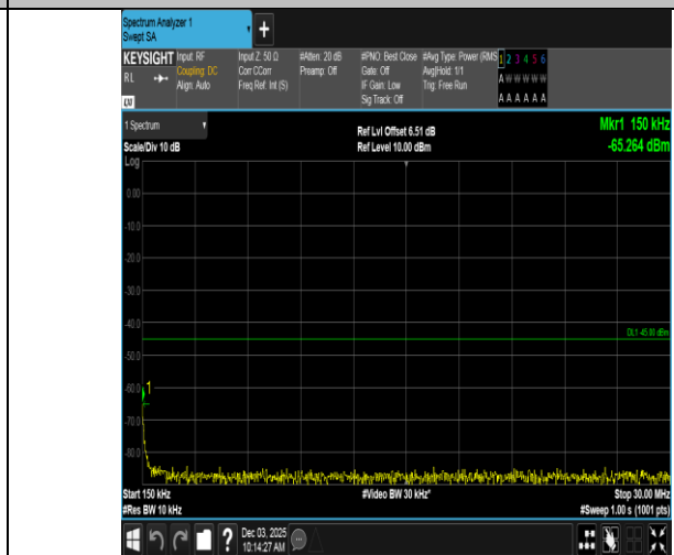
Band7-15MHz-16QAM-20825-1RB#0-0.15~30-PASS
