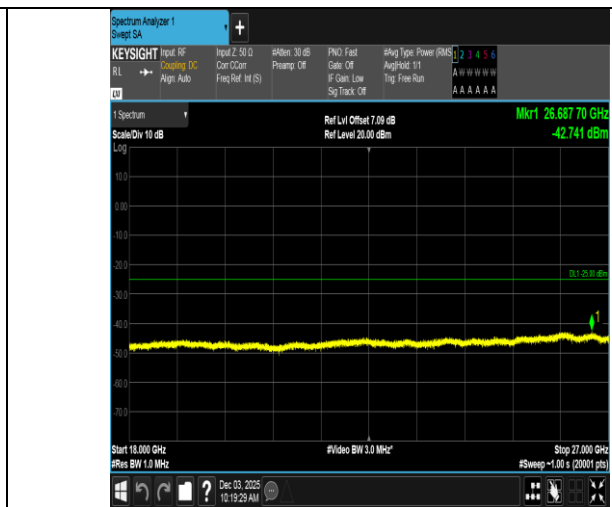
Band7-15MHz-QPSK-20825-75RB#0-18000~27000-PASS
