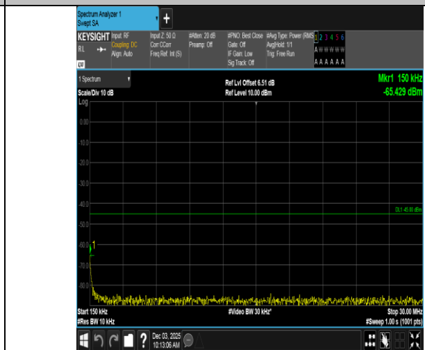
Band7-15MHz-QPSK-20825-1RB#0-0.15~30-PASS
