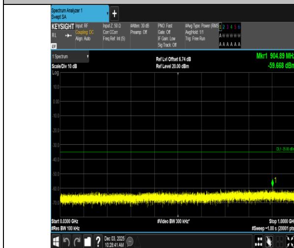
Band7-15MHz-16QAM-21100-75RB#0-30~1000-PASS
