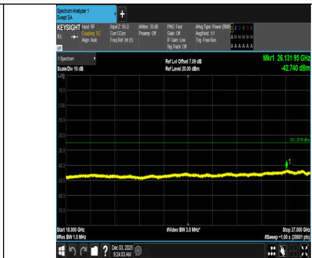
Band7-10MHz-16QAM-21400-50RB#0-18000~27000-PASS
