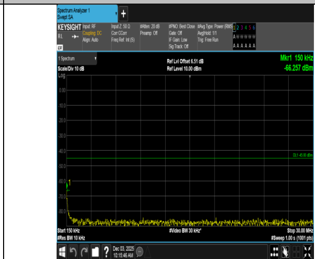
Band7-15MHz-QPSK-20825-1RB#74-0.15~30-PASS
