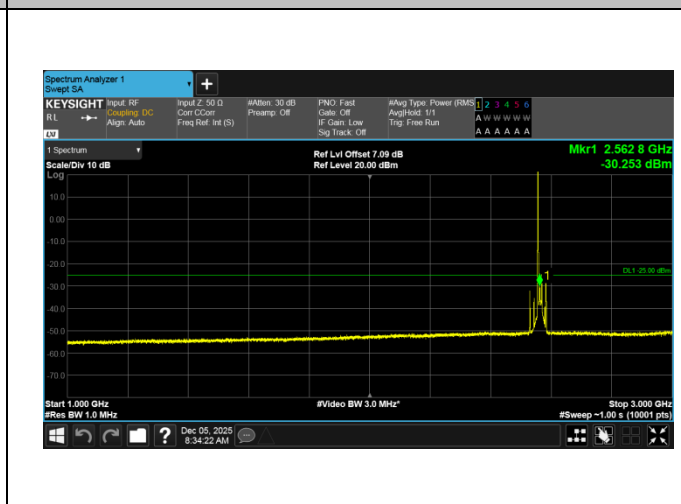
Band7-15MHz-QPSK-21375-1RB#0-1000~3000-PASS
