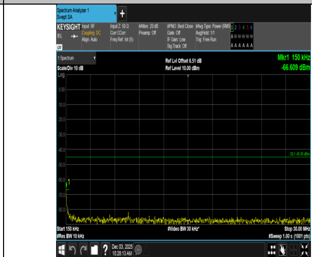
Band7-15MHz-16QAM-21100-75RB#0-0.15~30-PASS
