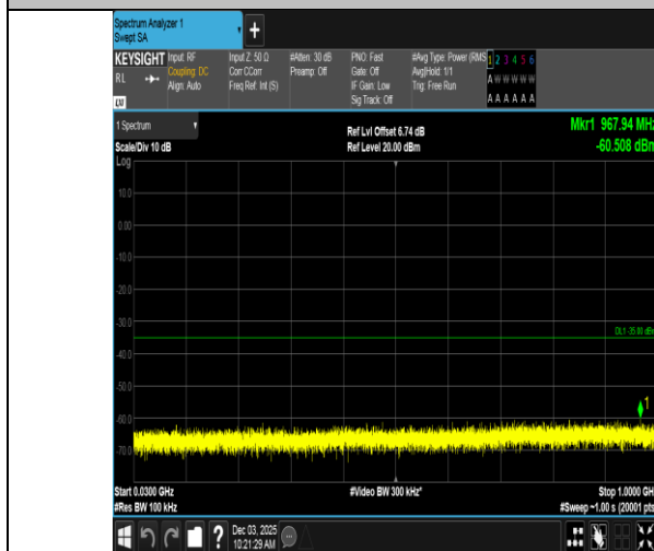
Band7-15MHz-QPSK-21100-1RB#0-30~1000-PASS
