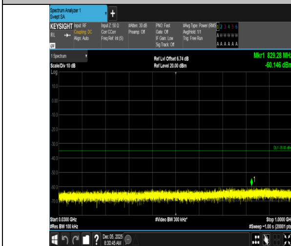
Band7-15MHz-QPSK-21375-1RB#0-30~1000-PASS
