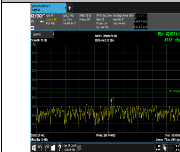
Band7-15MHz-QPSK-21375-1RB#0-0.009~0.15-PASS
