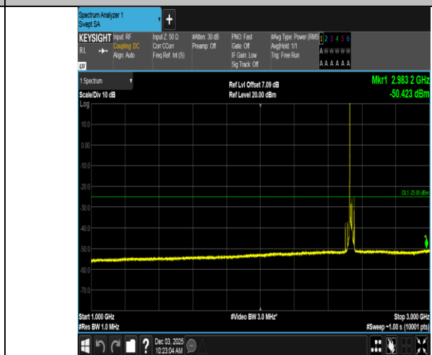
Band7-15MHz-16QAM-21100-1RB#0-1000~3000-PASS
