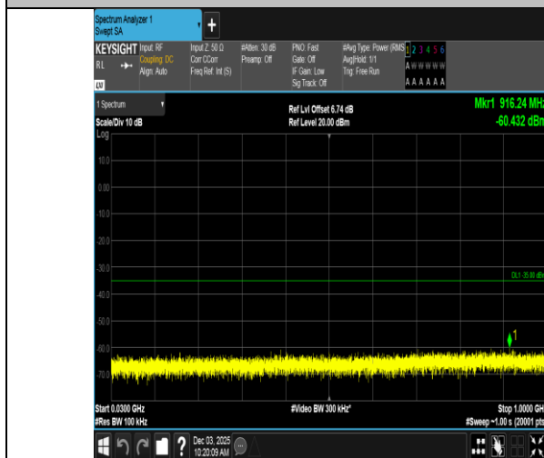
Band7-15MHz-16QAM-20825-75RB#0-30~1000-PASS
