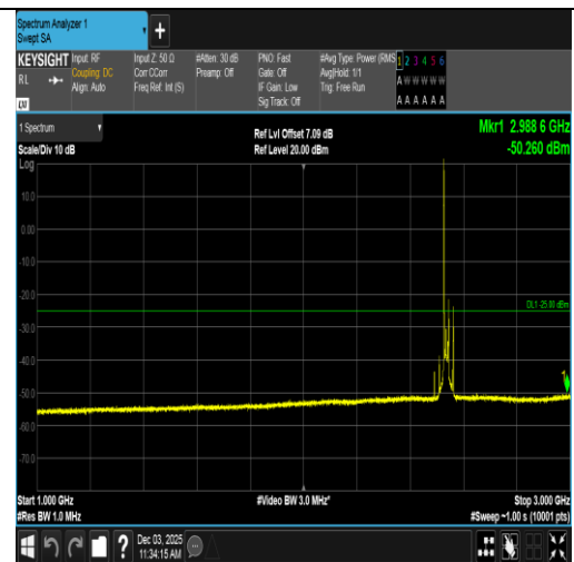
Band7-20MHz-QPSK-21100-1RB#0-1000~3000-PASS
