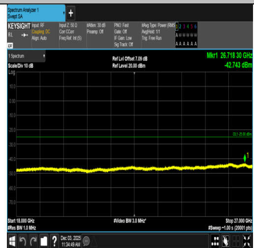
Band7-20MHz-QPSK-21100-1RB#0-18000~27000-PASS
