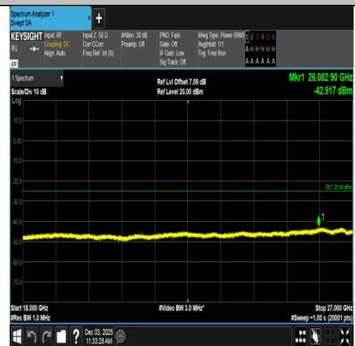
Band7-20MHz-16QAM-20850-100RB#0-18000~27000-PASS
