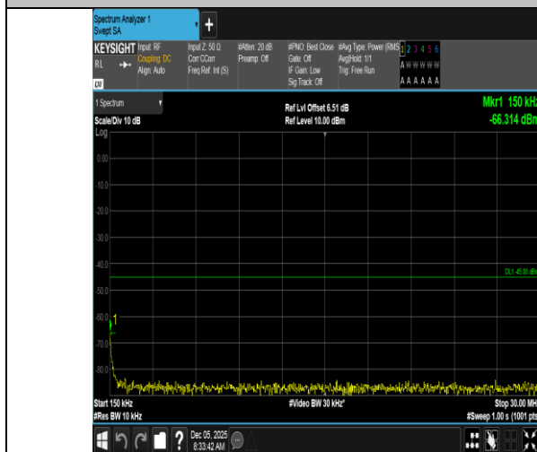
Band7-15MHz-16QAM-21375-1RB#0-0.15~30-PASS
