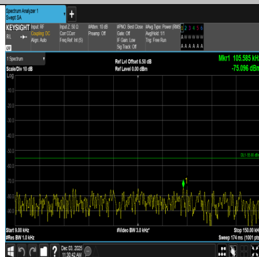
Band7-20MHz-QPSK-20850-100RB#0-0.009~0.15-PASS
