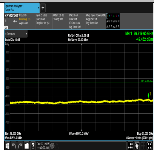
Band7-20MHz-QPSK-21100-100RB#0-18000~27000-PASS
