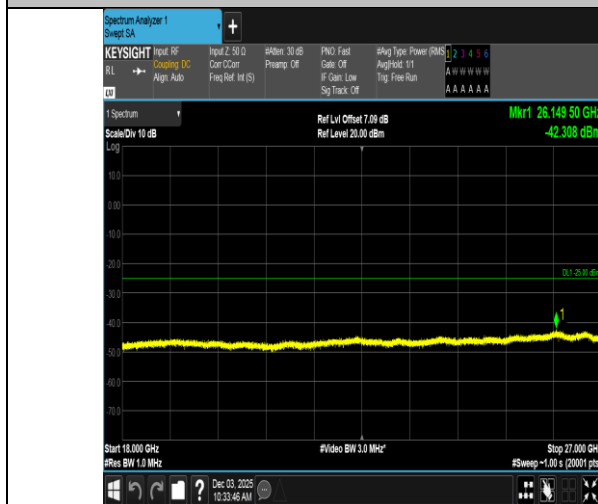
Band7-15MHz-QPSK-21375-1RB#74-18000~27000-PASS
