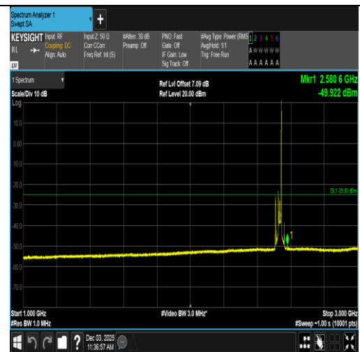
Band7-20MHz-QPSK-21100-1RB#99-1000~3000-PASS
