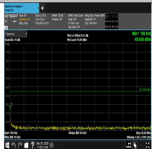
Band7-20MHz-QPSK-20850-1RB#99-0.15~30-PASS
