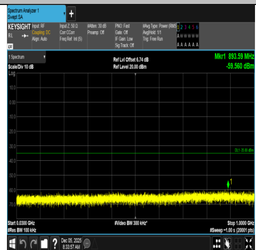
Band7-15MHz-16QAM-21375-1RB#0-30~1000-PASS
