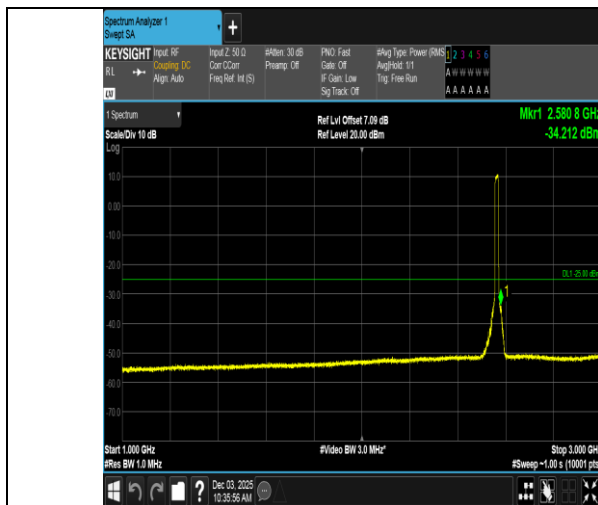
Band7-15MHz-QPSK-21375-75RB#0-1000~3000-PASS
