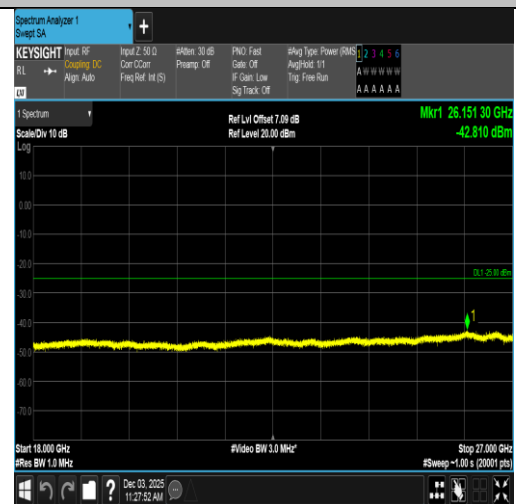
Band7-20MHz-16QAM-20850-1RB#0-18000~27000-PASS
