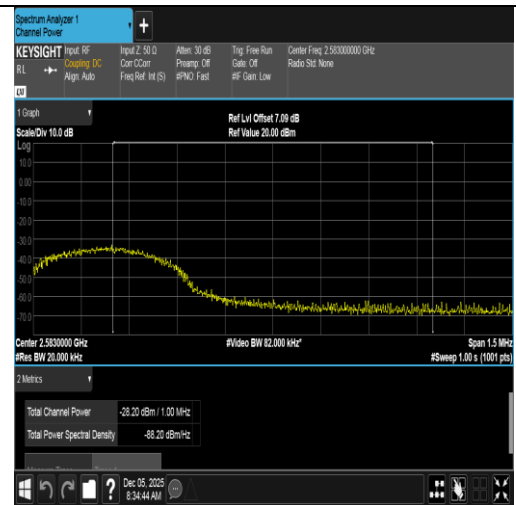
Band7-15MHz-16QAM-21375-1RB#0-1000~3000-PASS
