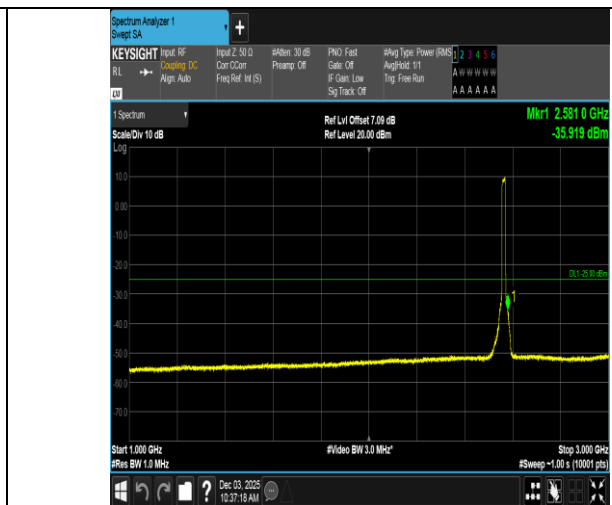
Band7-15MHz-16QAM-21375-75RB#0-1000~3000-PASS
