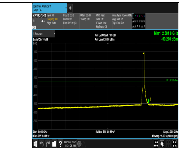
Band7-20MHz-QPSK-20850-100RB#0-1000~3000-PASS
