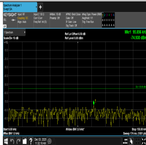
Band7-20MHz-16QAM-20850-100RB#0-0.009~0.15-PASS
