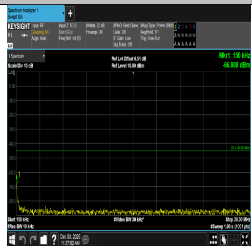
Band7-20MHz-16QAM-21100-1RB#99-0.15~30-PASS
