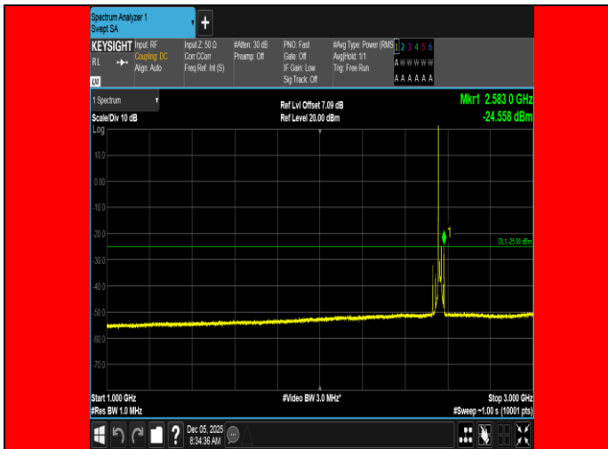
Band7-15MHz-16QAM-21375-1RB#0-1000~3000-FAIL
