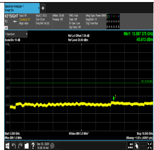
Band7-15MHz-QPSK-21375-75RB#0-3000~18000-PASS
