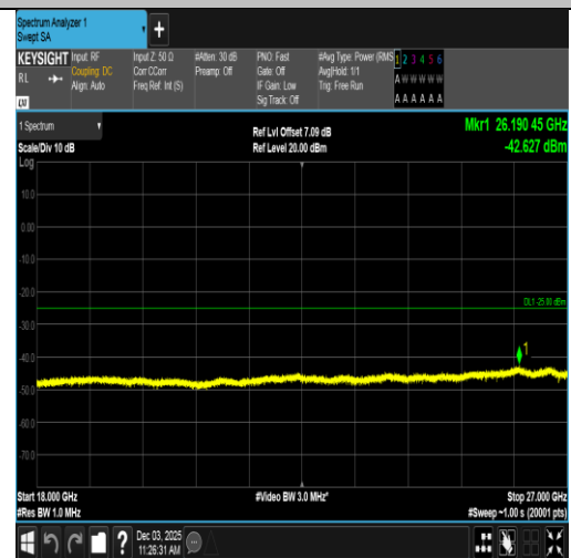
Band7-20MHz-QPSK-20850-1RB#0-18000~27000-PASS
