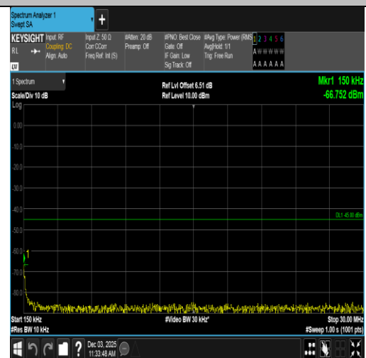
Band7-20MHz-QPSK-21100-1RB#0-0.15~30-PASS
