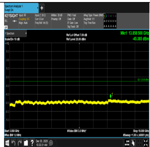
Band7-15MHz-QPSK-21375-1RB#74-3000~18000-PASS
