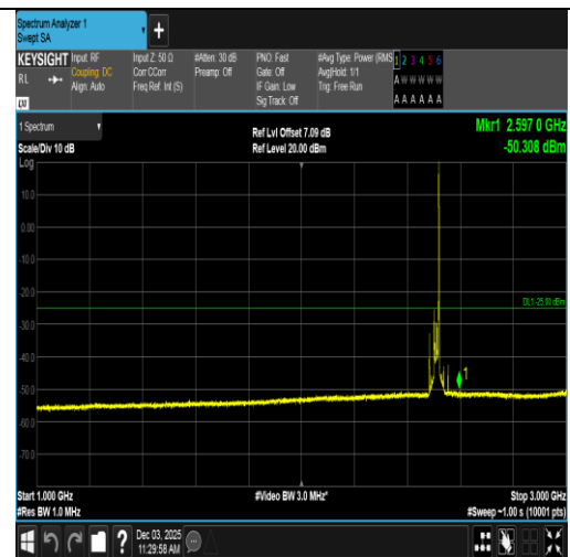
Band7-20MHz-16QAM-20850-1RB#99-1000~3000-PASS
