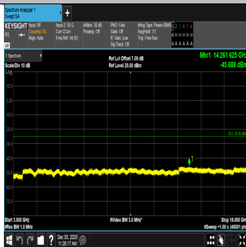
Band7-20MHz-QPSK-20850-1RB#0-3000~18000-PASS
