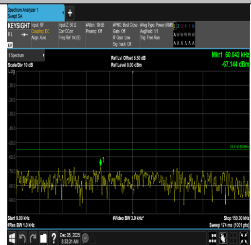
Band7-15MHz-16QAM-21375-1RB#0-0.009~0.15-PASS
