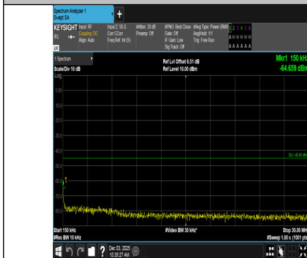
Band7-15MHz-QPSK-21375-75RB#0-0.15~30-PASS
