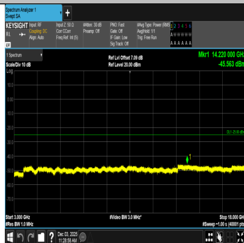
Band7-20MHz-QPSK-20850-1RB#99-3000~18000-PASS
