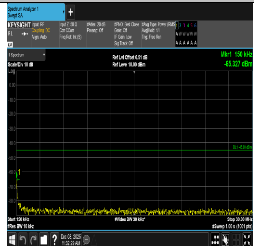
Band7-20MHz-16QAM-20850-100RB#0-0.15~30-PASS
