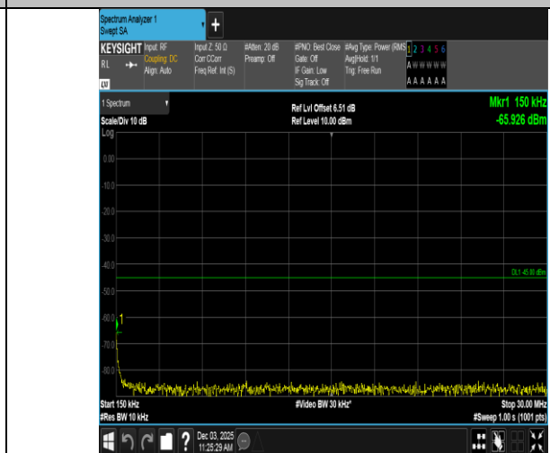
Band7-20MHz-QPSK-20850-1RB#0-0.15~30-PASS
