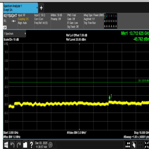
Band7-20MHz-16QAM-21100-1RB#0-3000~18000-PASS
