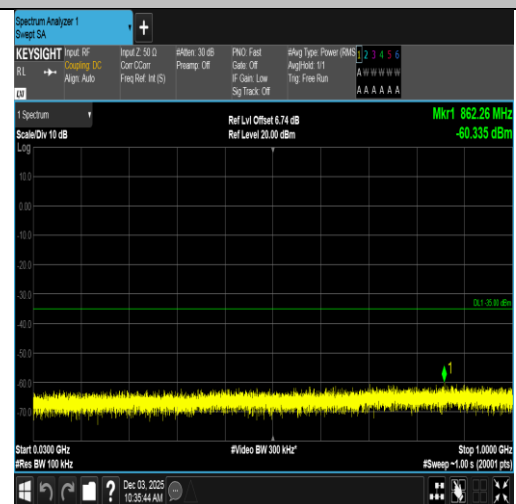
Band7-15MHz-QPSK-21375-75RB#0-30~1000-PASS
