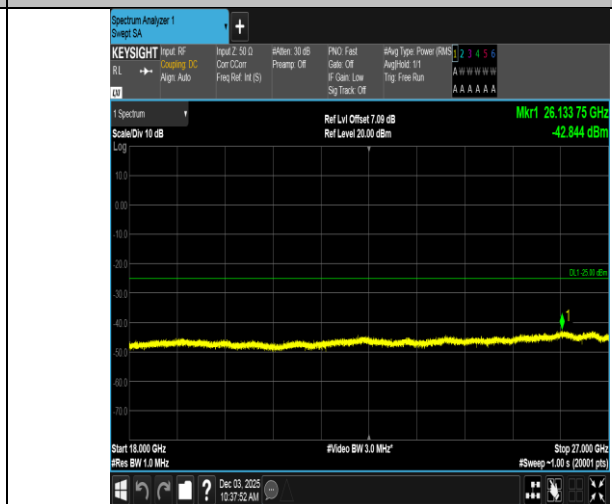
Band7-15MHz-16QAM-21375-75RB#0-18000~27000-PASS
