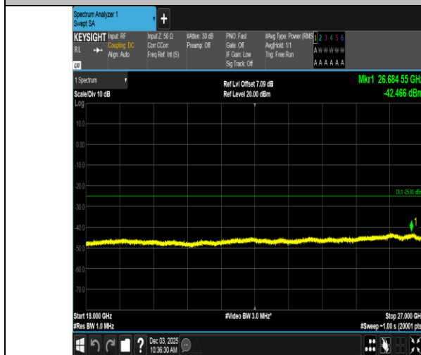
Band7-15MHz-QPSK-21375-75RB#0-18000~27000-PASS
