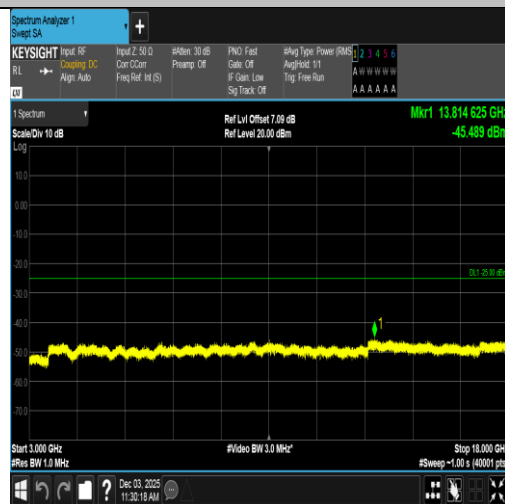
Band7-20MHz-16QAM-20850-1RB#99-3000~18000-PASS
