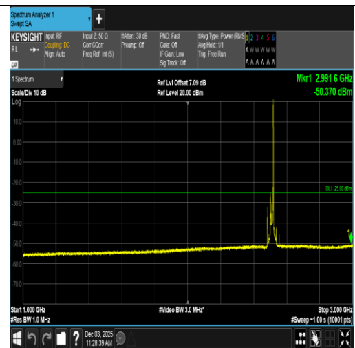
Band7-20MHz-QPSK-20850-1RB#99-1000~3000-PASS
