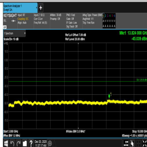
Band7-20MHz-QPSK-21100-1RB#99-3000~18000-PASS
