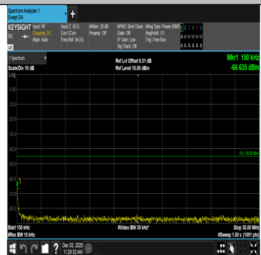
Band7-20MHz-16QAM-20850-1RB#99-0.15~30-PASS
