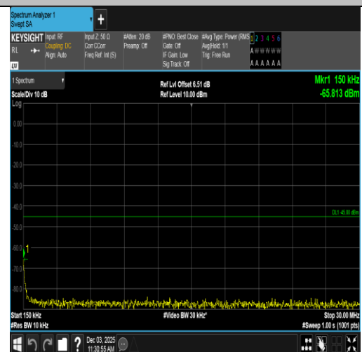
Band7-20MHz-QPSK-20850-100RB#0-0.15~30-PASS
