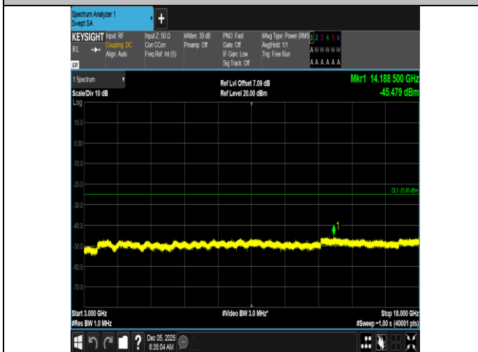
Band7-15MHz-16QAM-21375-1RB#0-3000~18000-PASS
