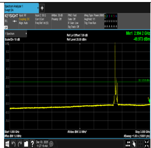
Band7-20MHz-16QAM-20850-1RB#0-1000~3000-PASS
