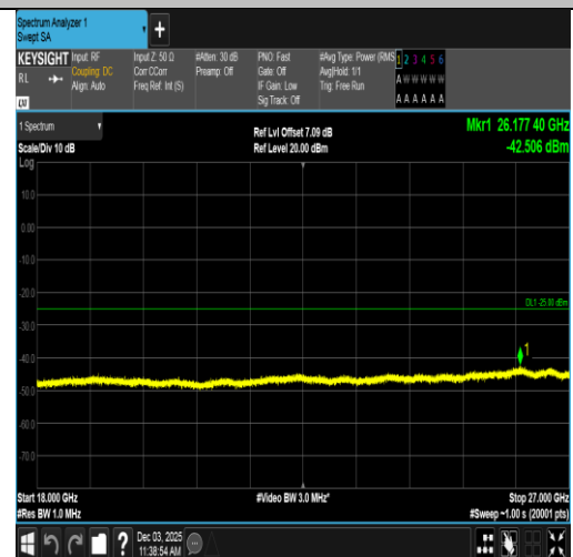
Band7-20MHz-16QAM-21100-1RB#99-18000~27000-PASS
