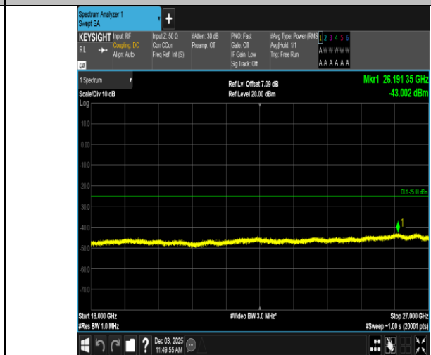
Band7-20MHz-QPSK-21350-100RB#0-18000~27000-PASS
