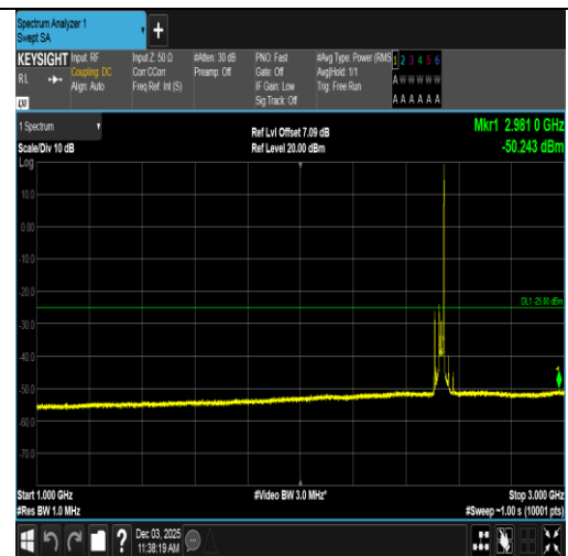
Band7-20MHz-16QAM-21100-1RB#99-1000~3000-PASS
