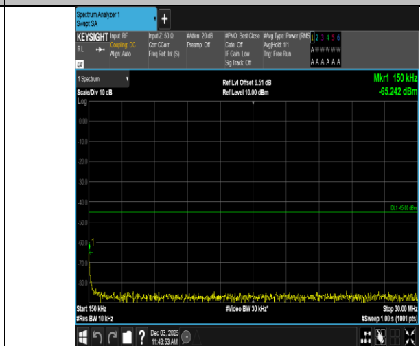
Band7-20MHz-16QAM-21350-1RB#0-0.15~30-PASS
