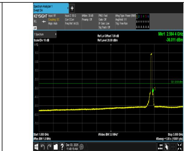
Band7-20MHz-QPSK-21350-100RB#0-1000~3000-PASS
