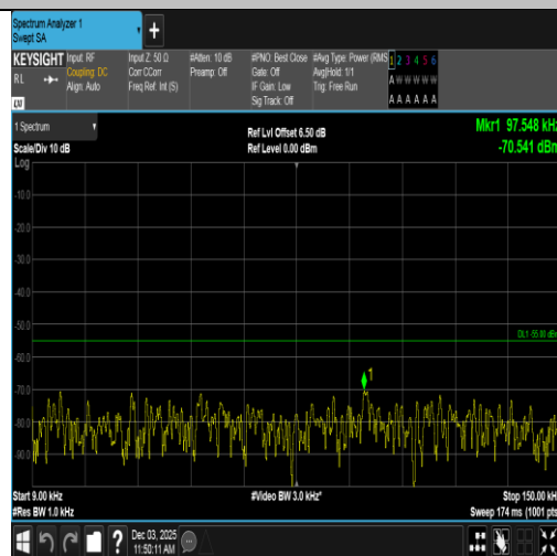
Band7-20MHz-16QAM-21350-100RB#0-0.009~0.15-PASS
