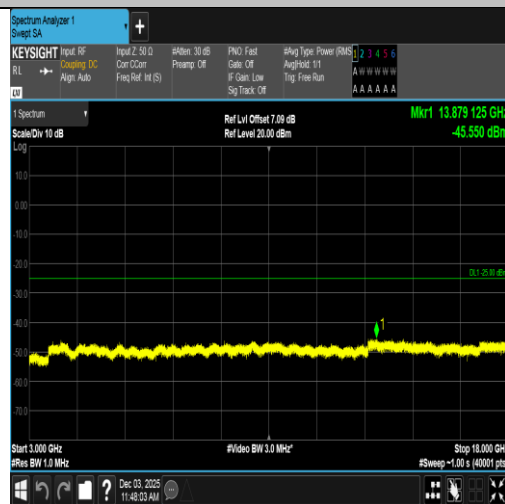
Band7-20MHz-16QAM-21350-1RB#99-3000~18000-PASS
