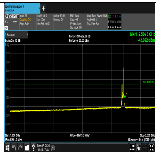
Band7-20MHz-QPSK-21350-1RB#99-1000~3000-PASS
