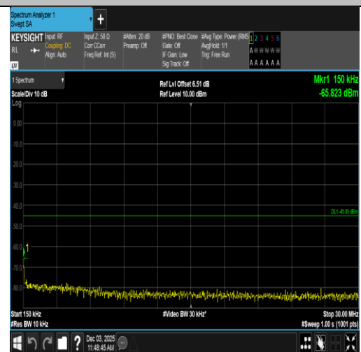
Band7-20MHz-QPSK-21350-100RB#0-0.15~30-PASS
