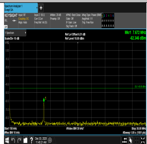
Band7-20MHz-QPSK-21350-1RB#99-0.15~30-PASS
