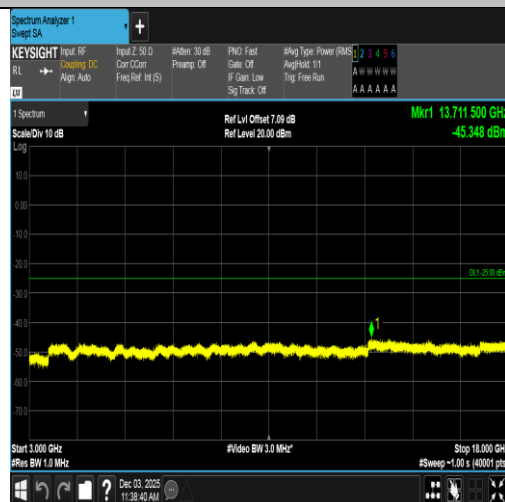
Band7-20MHz-16QAM-21100-1RB#99-3000~18000-PASS
