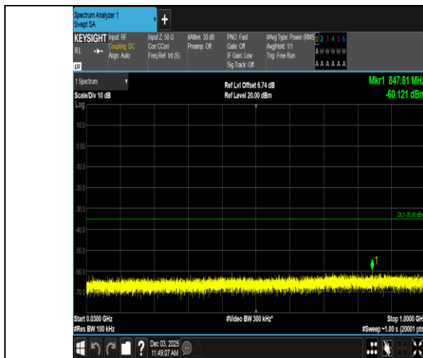
Band7-20MHz-QPSK-21350-100RB#0-30~1000-PASS
