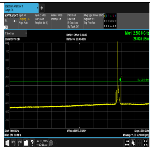
Band7-20MHz-QPSK-21350-1RB#0-1000~3000-PASS
