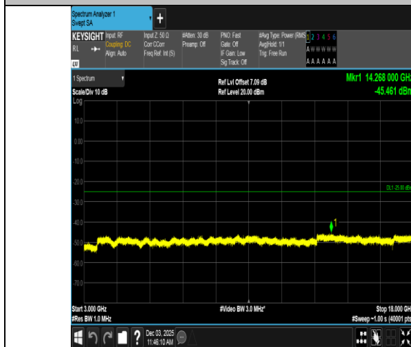
Band7-20MHz-QPSK-21350-1RB#99-3000~18000-PASS
