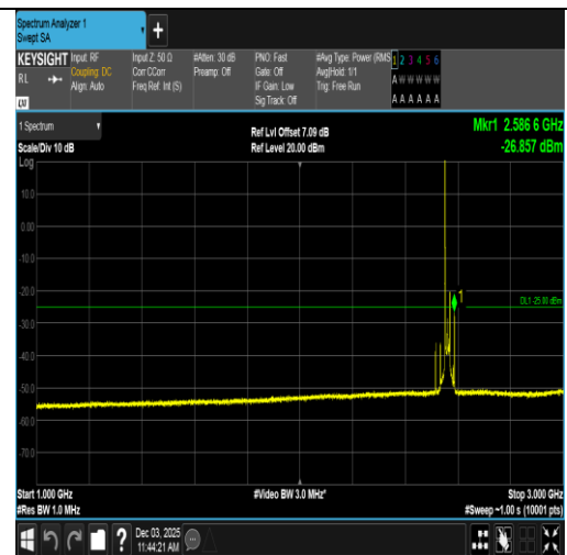
Band7-20MHz-16QAM-21350-1RB#0-1000~3000-PASS
