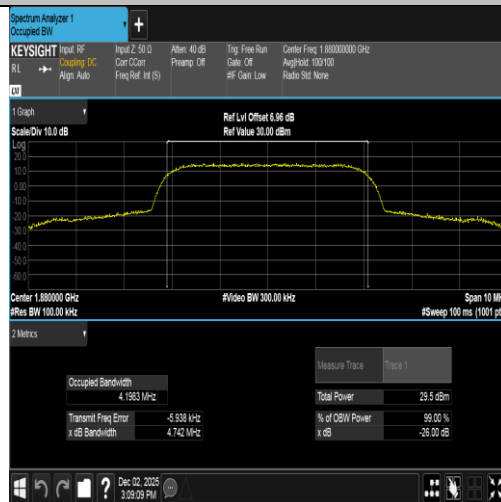
Band2-9400-2-PASS
