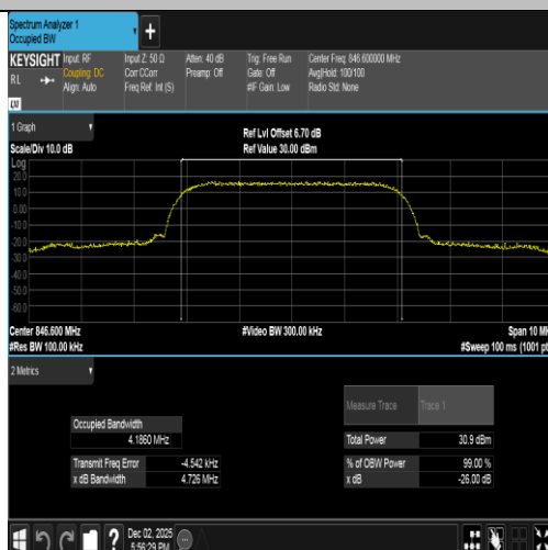
Band5-4233-3-PASS
