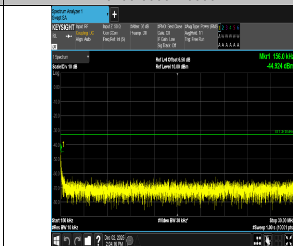
Band2-9538-0.15~30MHz-PASS
