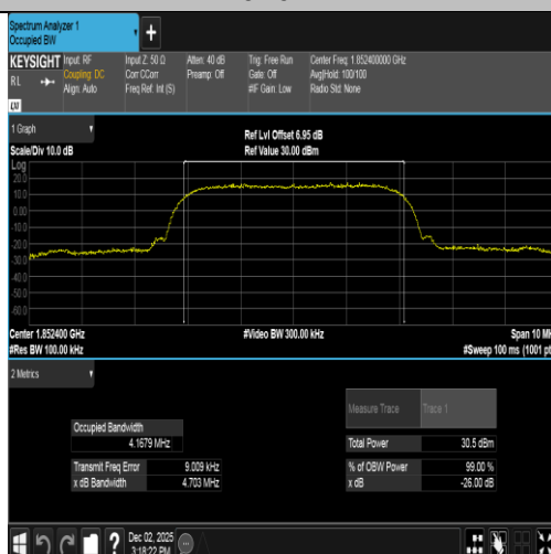
Band2-9262-5-PASS
