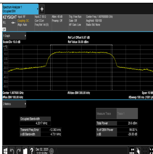
Band2-9538-2-PASS
