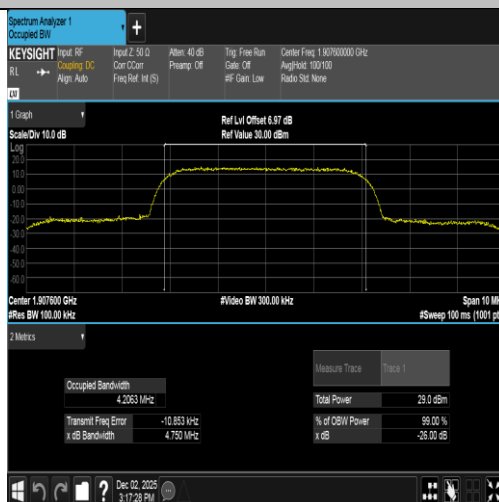
Band2-9538-4-PASS
