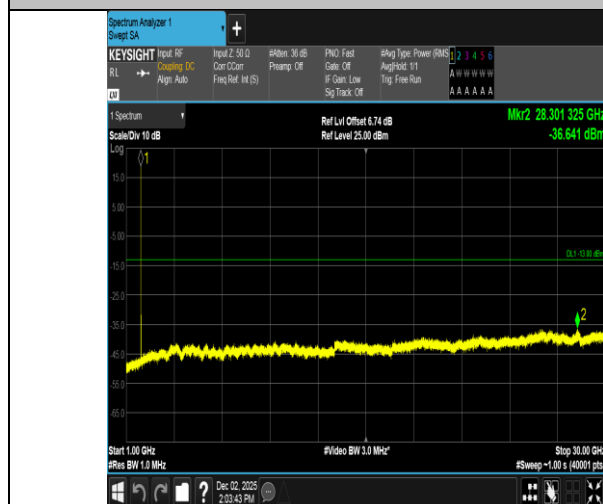
Band2-9400-1000~30000MHz-PASS
