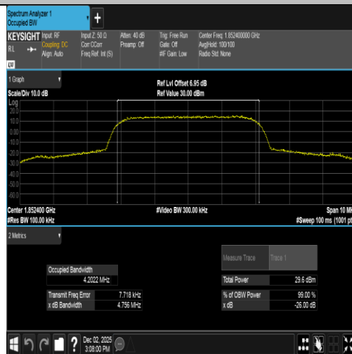
Band2-9262-2-PASS
