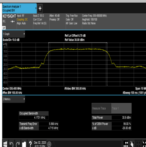
Band5-4182-5-PASS
