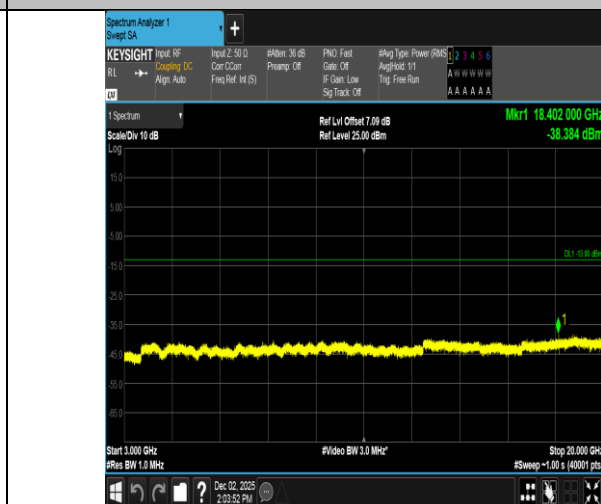
Band2-9400-3000~20000MHz-PASS
