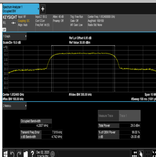
Band2-9262-4-PASS
