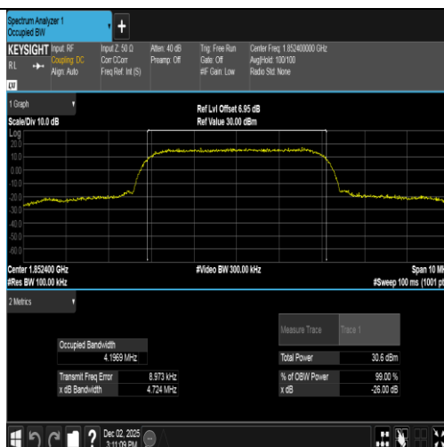
Band2-9262-3-PASS
