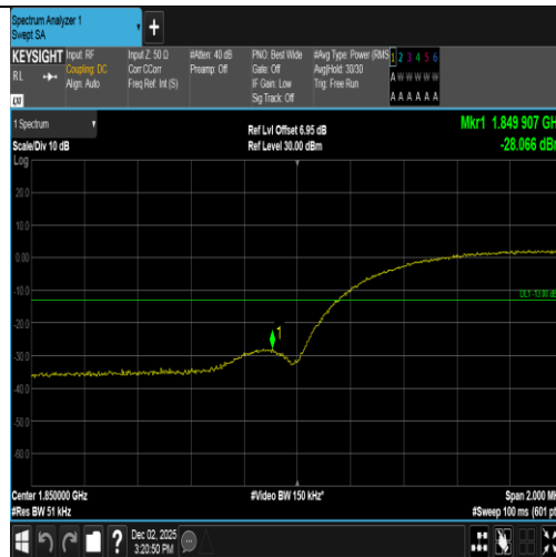
Band2-9262-1-PASS
