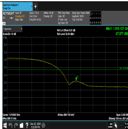
Band2-9538-1-PASS
