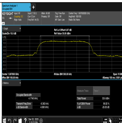
Band2-9538-5-PASS
