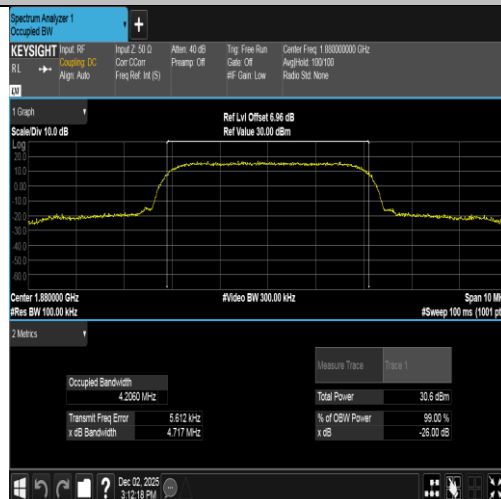
Band2-9400-3-PASS
