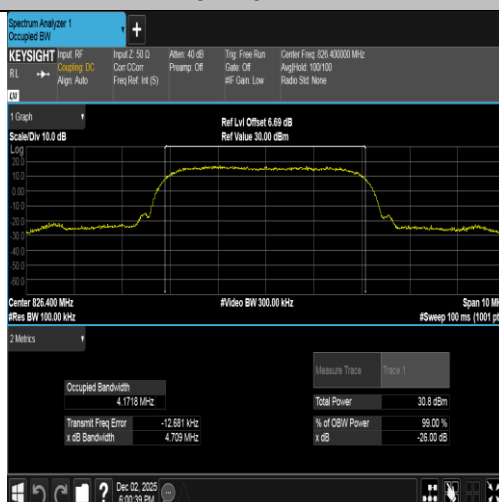
Band5-4132-5-PASS
