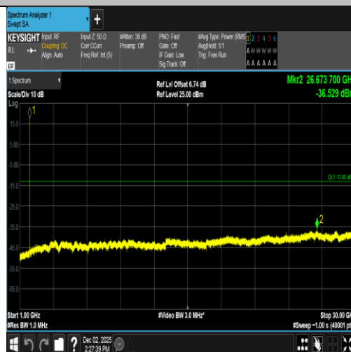
Band2-9262-2-1000~30000MHz-PASS
