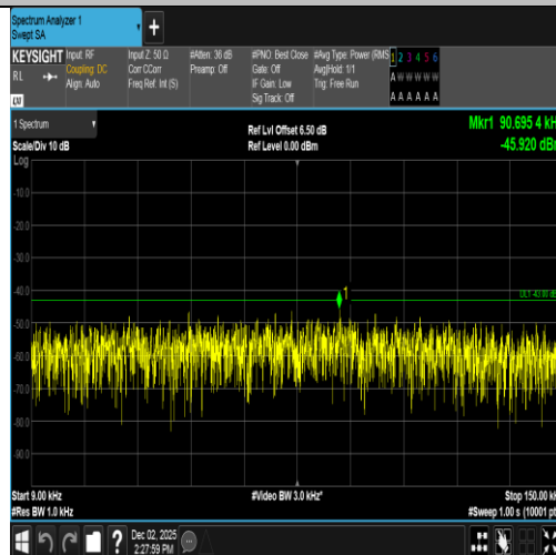
Band2-9400-2-0.009~0.15MHz-PASS
