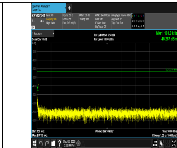
Band5-4233-0.15~30MHz-PASS
