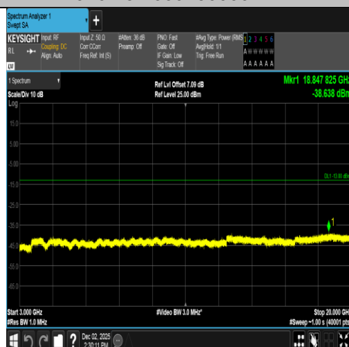
Band2-9262-3-3000~20000MHz-PASS
