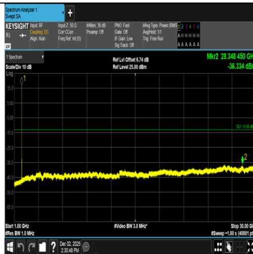
Band2-9400-3-1000~30000MHz-PASS
