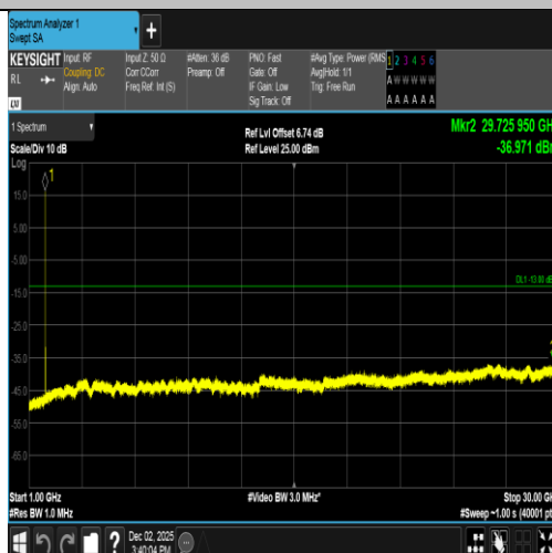
Band2-9400-3-1000~30000MHz-PASS
