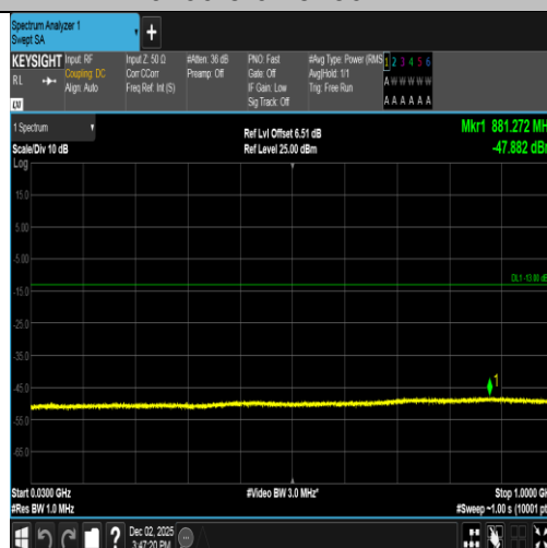
Band2-9400-5-30~1000MHz-PASS
