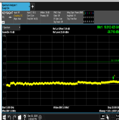
Band2-9262-3-3000~20000MHz-PASS
