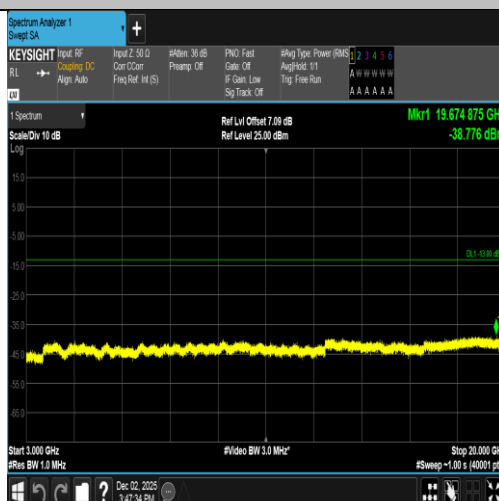
Band2-9400-5-3000~20000MHz-PASS
