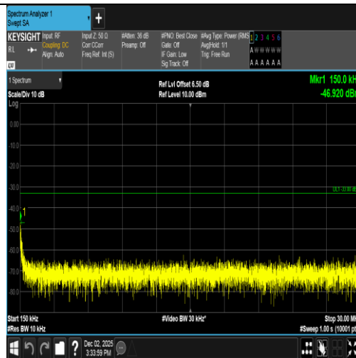
Band2-9262-2-0.15~30MHz-PASS
