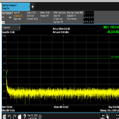
Band5-4233-2-0.15~30MHz-PASS
