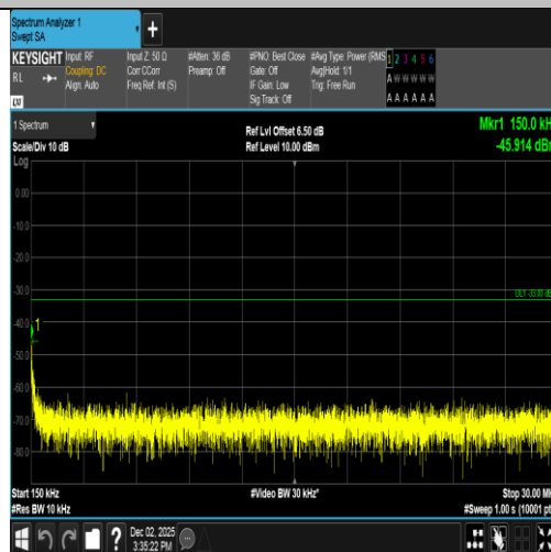
Band2-9400-2-0.15~30MHz-PASS
