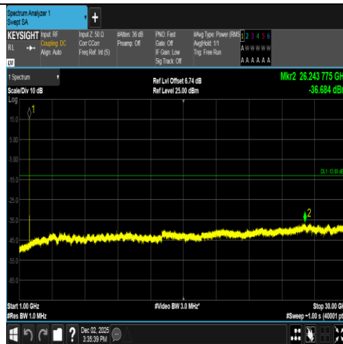
Band2-9400-2-1000~30000MHz-PASS
