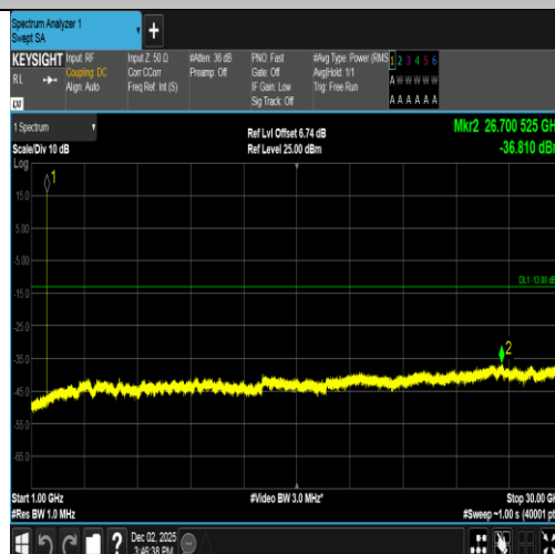
Band2-9262-5-1000~30000MHz-PASS
