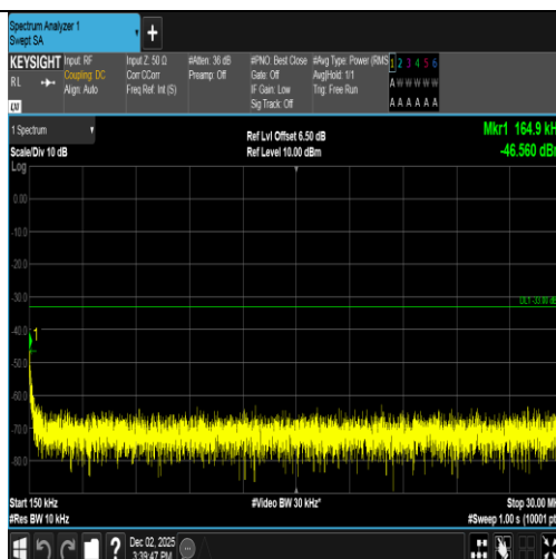
Band2-9400-3-0.15~30MHz-PASS
