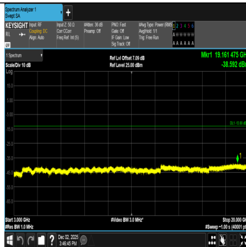
Band2-9262-5-3000~20000MHz-PASS
