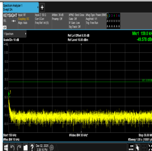
Band2-9262-3-0.15~30MHz-PASS
