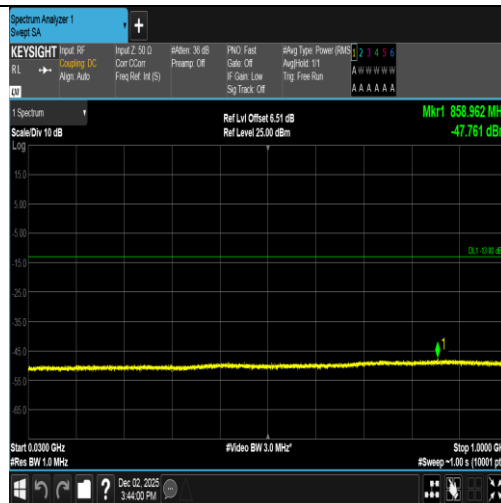
Band2-9400-4-30~1000MHz-PASS
