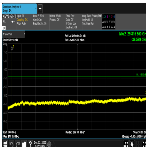
Band2-9400-5-1000~30000MHz-PASS
