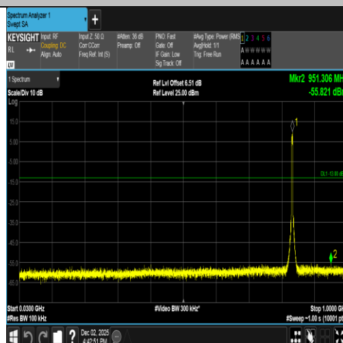
Band5-4182-2-30~1000MHz-PASS
