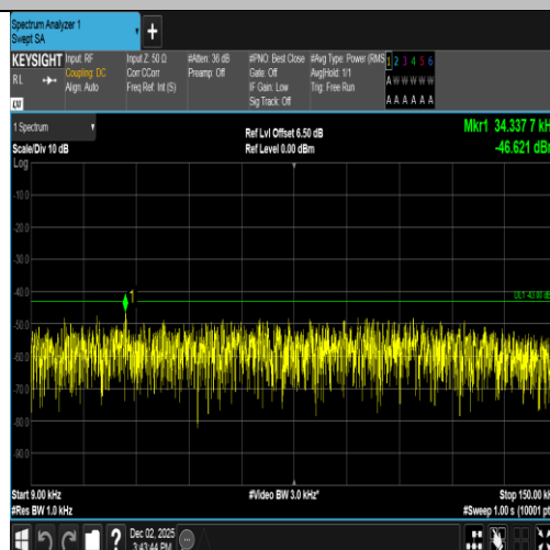
Band2-9400-4-0.009~0.15MHz-PASS
