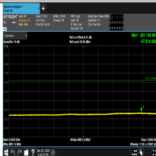
Band2-9400-2-30~1000MHz-PASS
