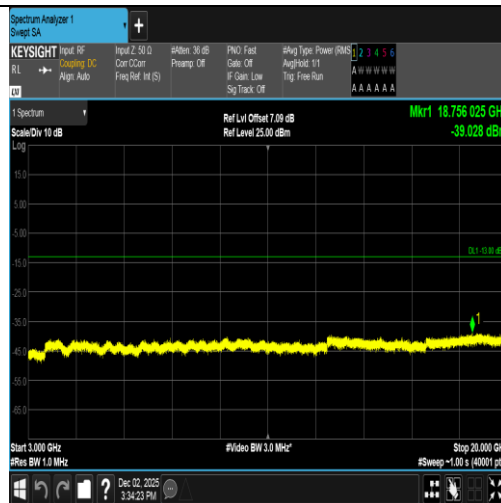
Band2-9262-2-3000~20000MHz-PASS
