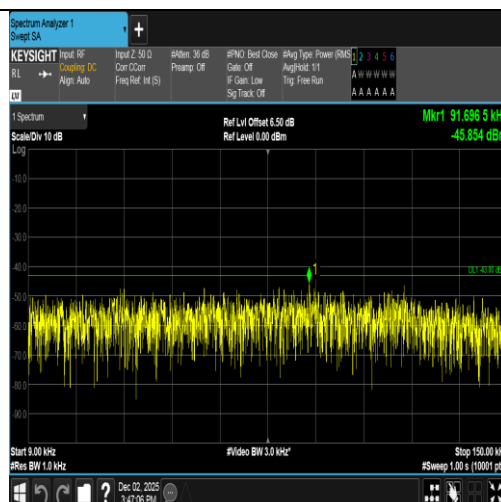
Band2-9400-5-0.009~0.15MHz-PASS
