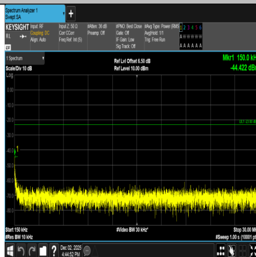
Band5-4182-3-0.15~30MHz-PASS
