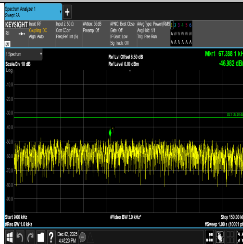
Band5-4233-3-0.009~0.15MHz-PASS
