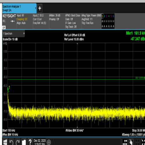
Band2-9262-1-0.15~30MHz-PASS
