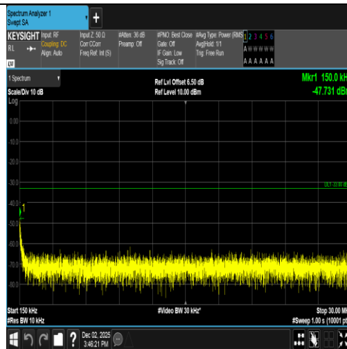
Band2-9262-5-0.15~30MHz-PASS
