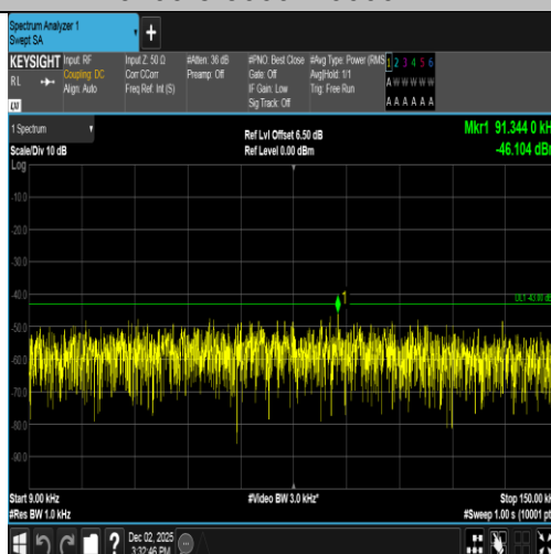
Band2-9538-1-0.009~0.15MHz-PASS
