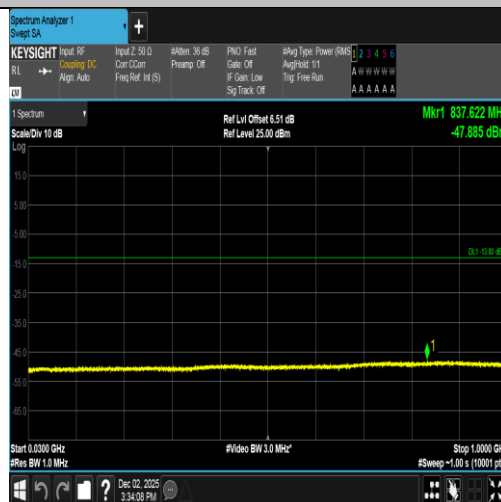
Band2-9262-2-30~1000MHz-PASS
