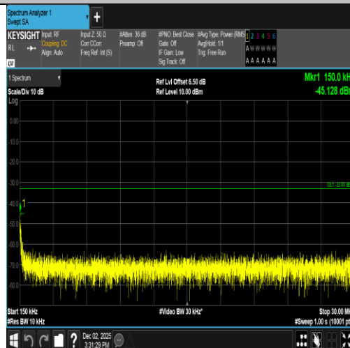
Band2-9400-1-0.15~30MHz-PASS
