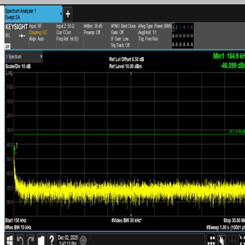
Band2-9400-5-0.15~30MHz-PASS
