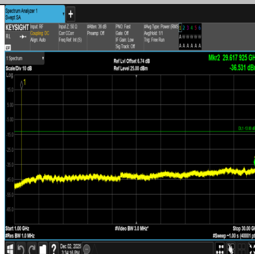
Band2-9262-2-1000~30000MHz-PASS
