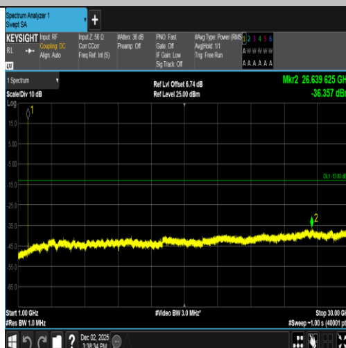
Band2-9262-3-1000~30000MHz-PASS
