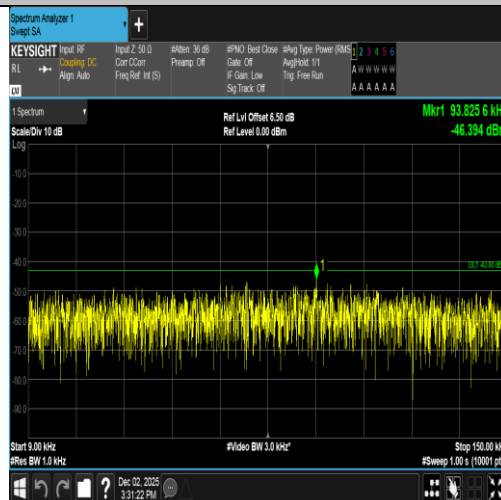
Band2-9400-1-0.009~0.15MHz-PASS
