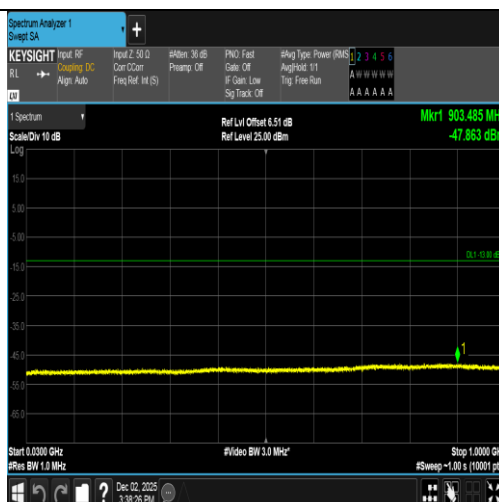
Band2-9262-3-30~1000MHz-PASS
