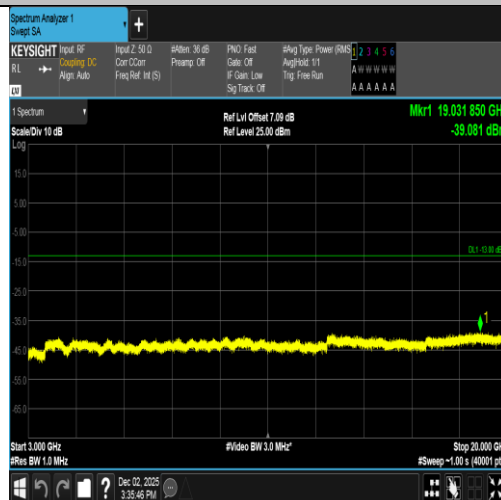
Band2-9400-2-3000~20000MHz-PASS
