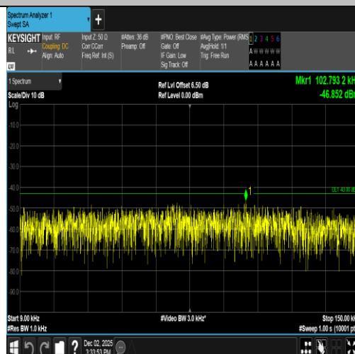
Band2-9262-2-0.009~0.15MHz-PASS
