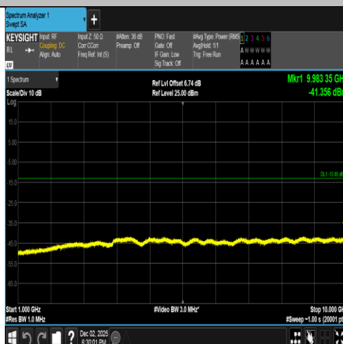
Band5-4132-5-1000~10000MHz-PASS
