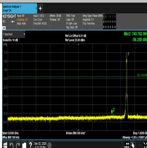
Band5-4233-5-30~1000MHz-PASS
