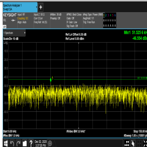
Band2-9538-2-0.009~0.15MHz-PASS
