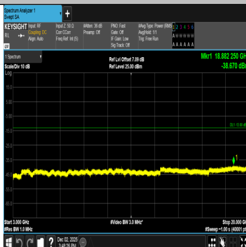
Band2-9538-5-3000~20000MHz-PASS
