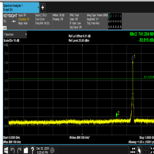
Band5-4233-2-30~1000MHz-PASS
