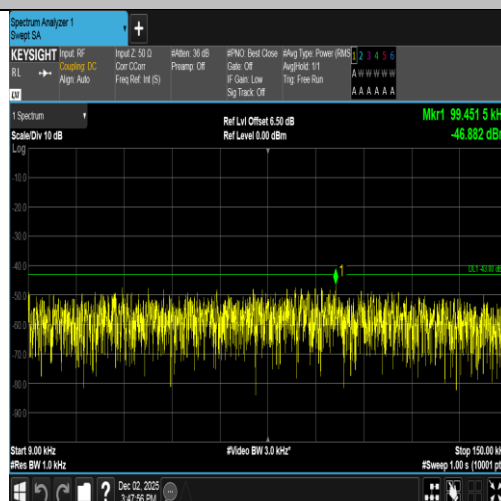
Band2-9538-5-0.009~0.15MHz-PASS
