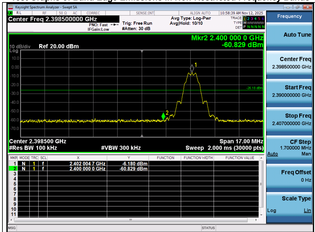
Test_Graph_LE125K_ANT1_2402_1Mbps_Lower Band Edge Emissions
