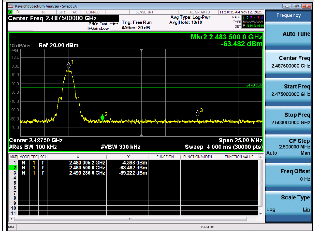
Test_Graph_LE500K_ANT1_2480_1Mbps_Higher Band Edge Emissions
