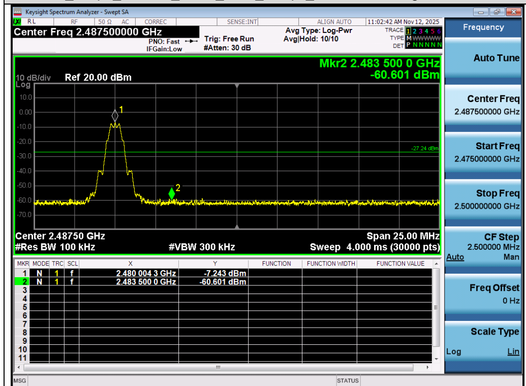
Test_Graph_LE125K_ANT1_2480_1Mbps_Higher Band Edge Emissions
