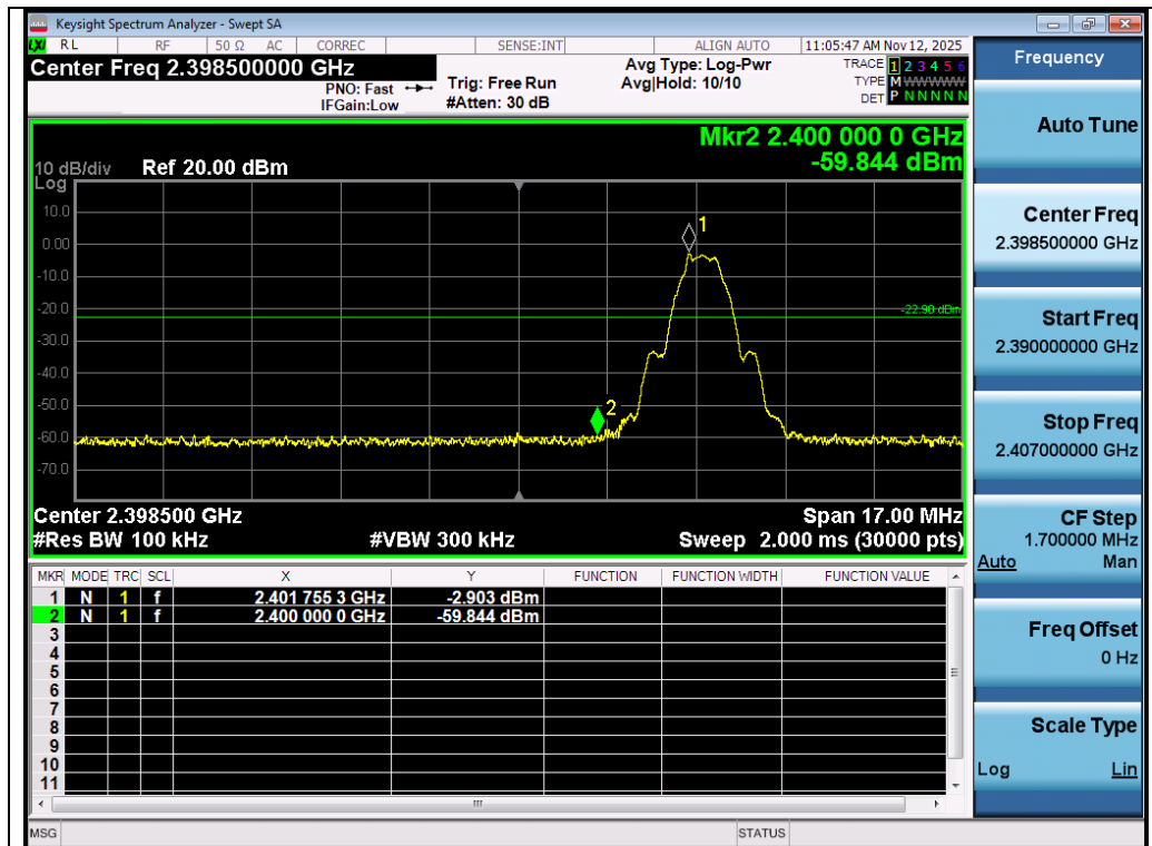
Test_Graph_LE500K_ANT1_2402_1Mbps_Lower Band Edge Emissions
