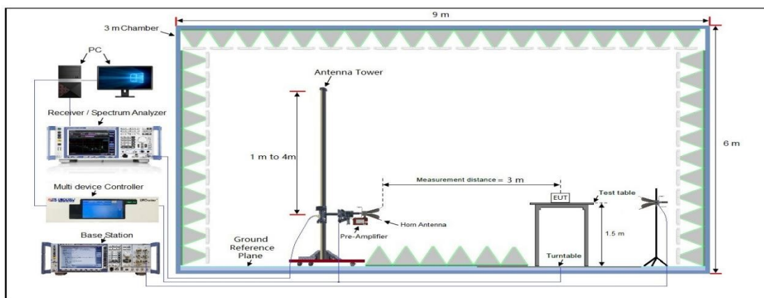
Radiated Emissions Above 1GHz Test setup
