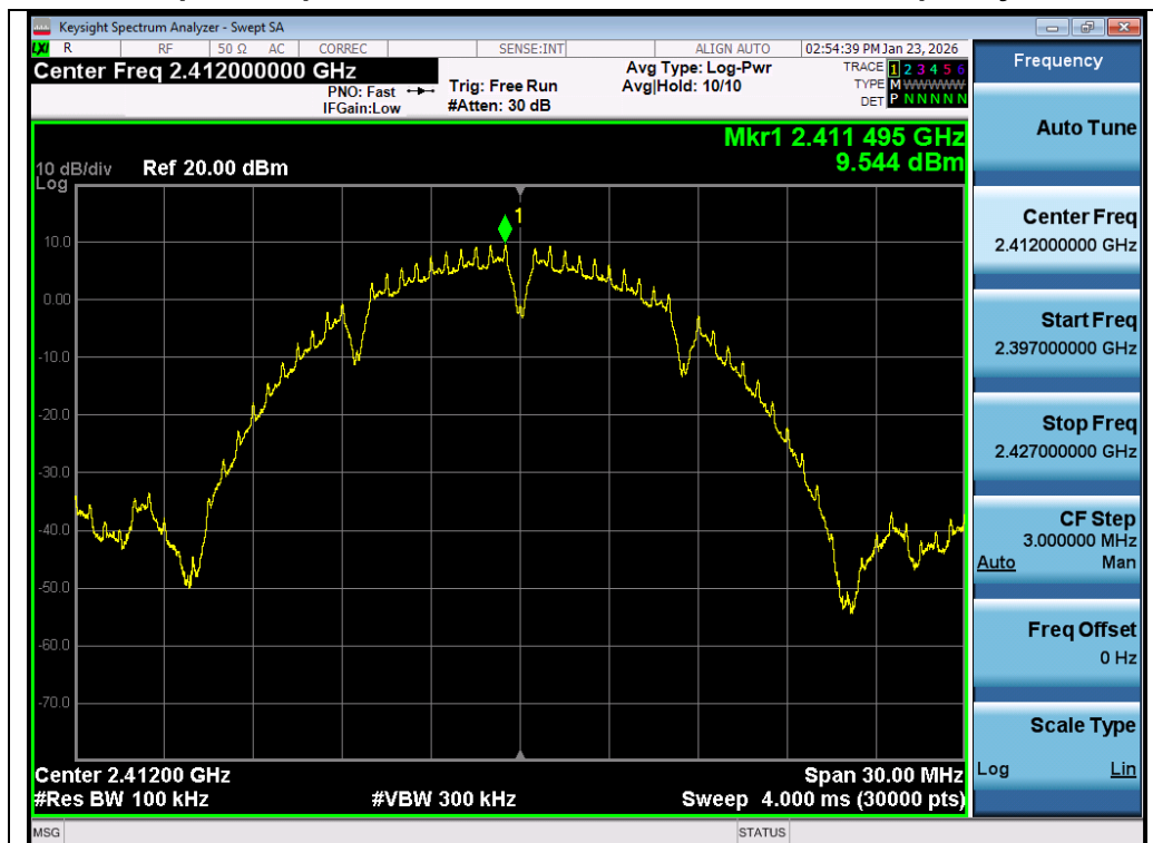
Test_Graph_802.11b_ANT1_2412_1Mbps_Reference Level
