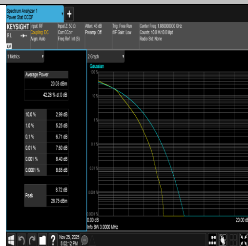
Band2-3MHz-16QAM-18900-15RB#0-PASS
