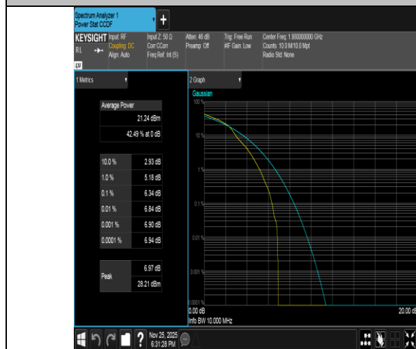
Band2-10MHz-16QAM-18900-1RB#0-PASS
