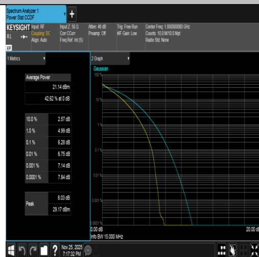
Band2-15MHz-QPSK-18900-75RB#0-PASS
