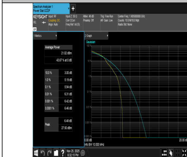
Band2-10MHz-16QAM-19150-1RB#0-PASS
