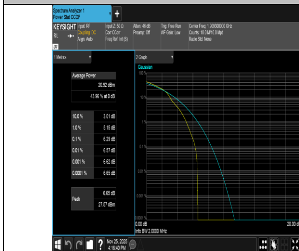
Band2-1.4MHz-16QAM-19193-1RB#0-PASS
