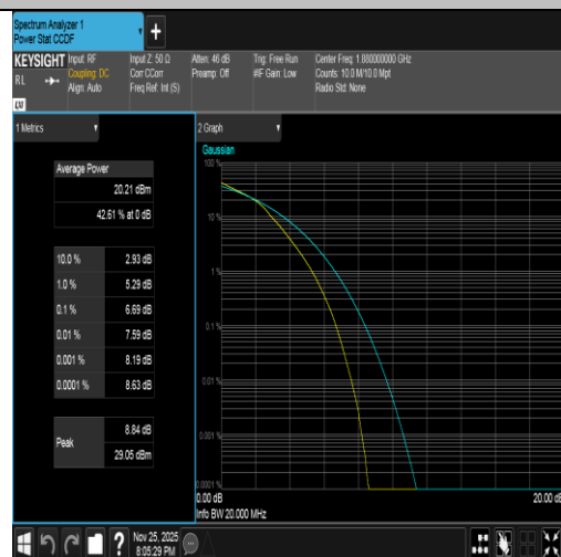
Band2-20MHz-16QAM-18900-100RB#0-PASS
