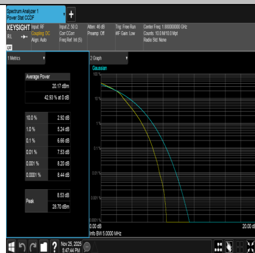
Band2-5MHz-16QAM-18900-25RB#0-PASS
