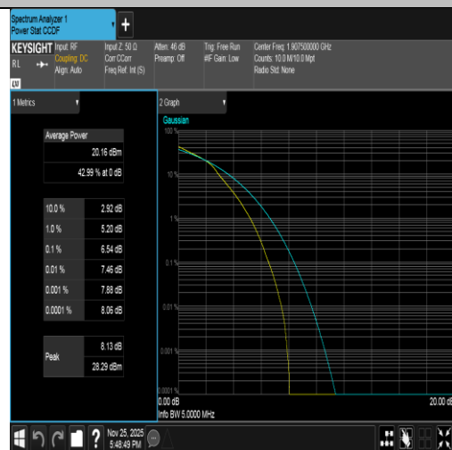
Band2-5MHz-16QAM-19175-25RB#0-PASS
