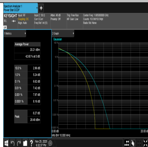
Band2-10MHz-16QAM-19150-50RB#0-PASS
