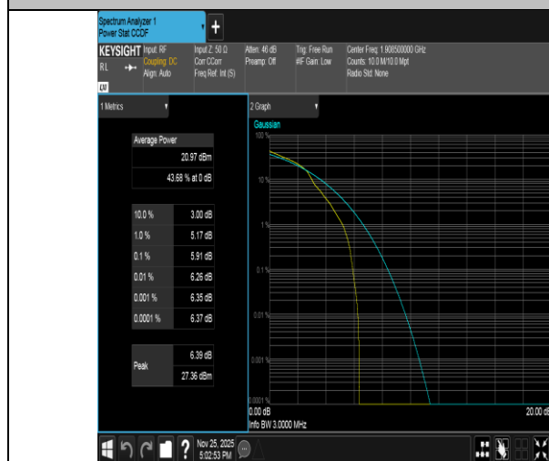
Band2-3MHz-16QAM-19185-1RB#0-PASS
