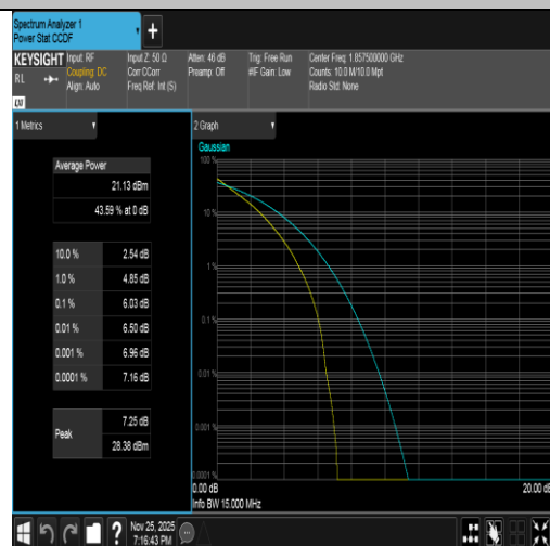
Band2-15MHz-QPSK-18675-75RB#0-PASS
