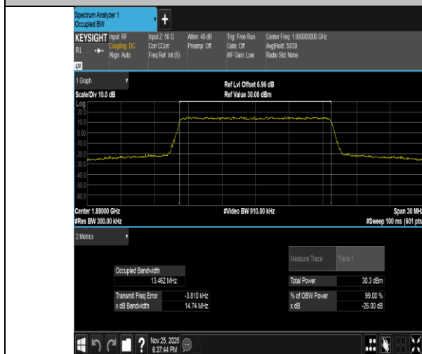
Band2-15MHz-QPSK-18900-75RB#0-PASS
