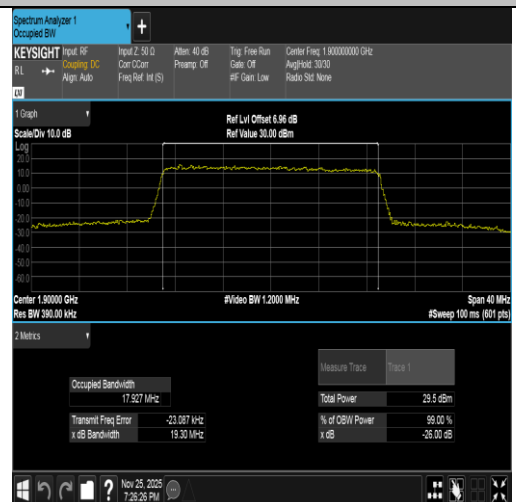
Band2-20MHz-16QAM-19100-100RB#0-PASS
