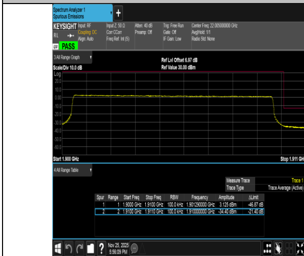
Band2-10MHz-QPSK-19150-50RB#0-PASS
