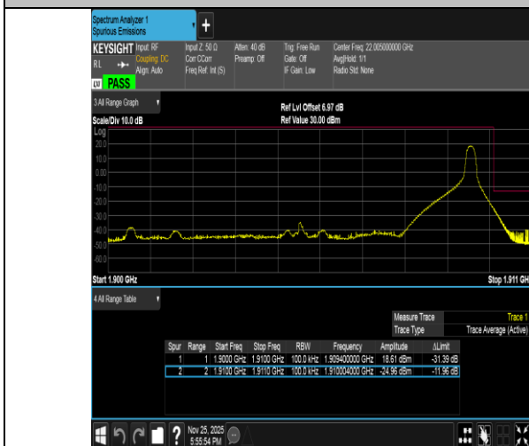
Band2-10MHz-16QAM-19150-1RB#49-PASS
