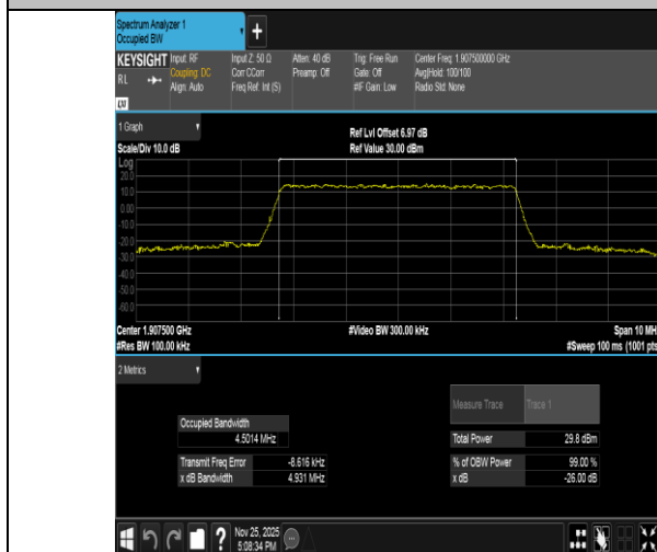
Band2-5MHz-QPSK-19175-25RB#0-PASS
