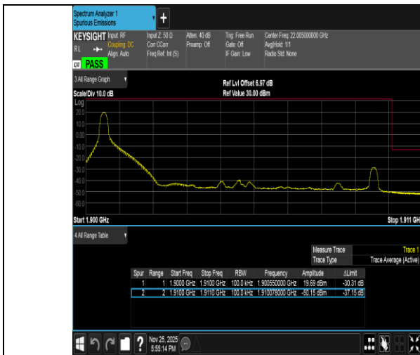
Band2-10MHz-QPSK-19150-1RB#0-PASS
