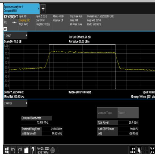
Band2-15MHz-16QAM-19125-75RB#0-PASS
