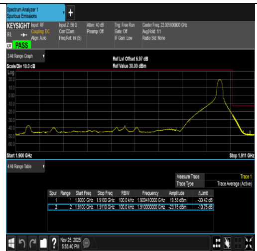
Band2-10MHz-QPSK-19150-1RB#49-PASS
