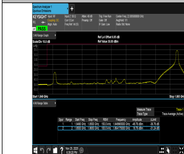
Band2-15MHz-16QAM-18675-1RB#74-PASS
