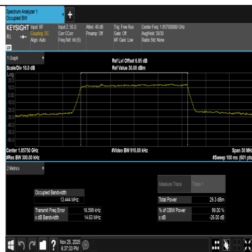
Band2-15MHz-16QAM-18675-75RB#0-PASS
