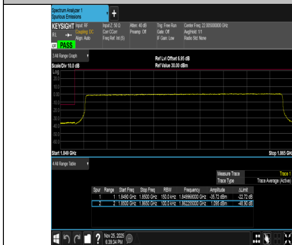
Band2-15MHz-QPSK-18675-75RB#0-PASS
