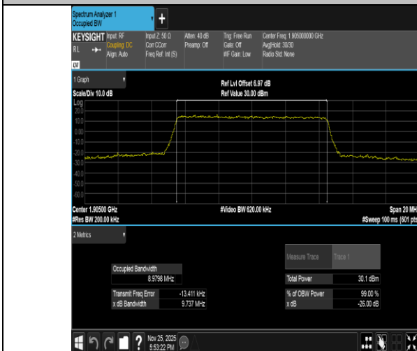
Band2-10MHz-QPSK-19150-50RB#0-PASS
