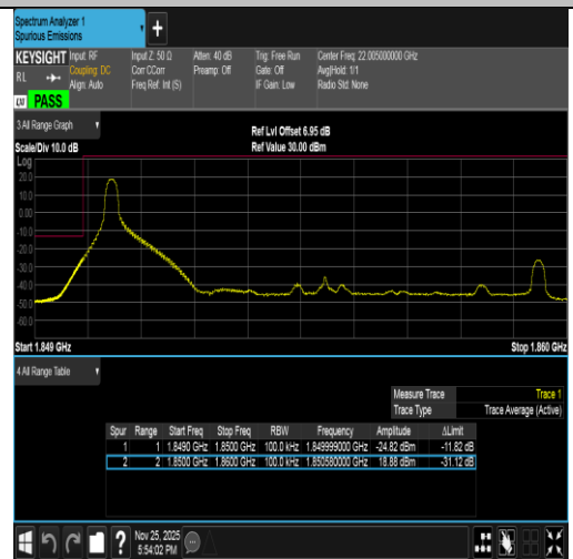
Band2-10MHz-16QAM-18650-1RB#0-PASS
