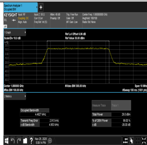
Band2-5MHz-16QAM-18900-25RB#0-PASS
