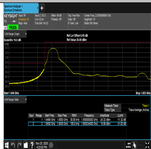
Band2-3MHz-16QAM-18615-1RB#0-PASS
