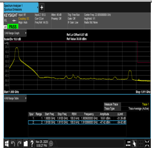
Band2-10MHz-16QAM-19150-1RB#0-PASS
