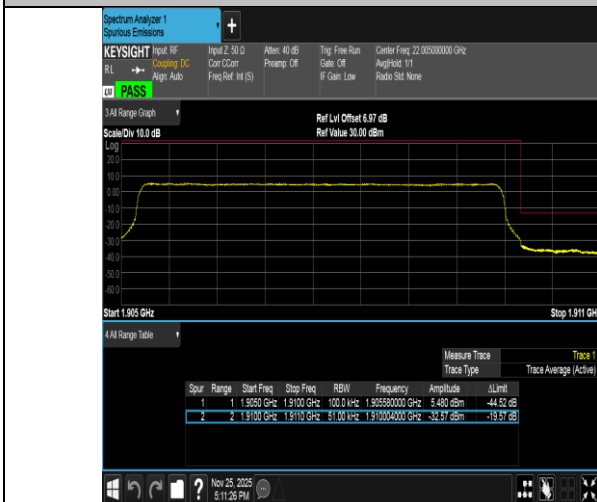
Band2-5MHz-QPSK-19175-25RB#0-PASS
