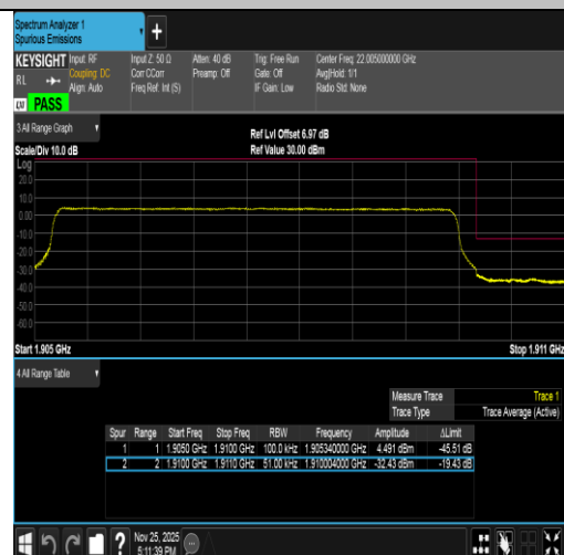
Band2-5MHz-16QAM-19175-25RB#0-PASS
