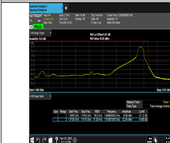
Band2-5MHz-16QAM-19175-1RB#24-PASS
