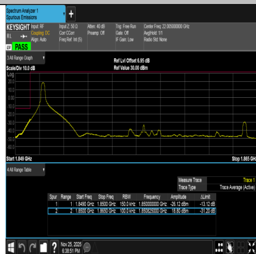
Band2-15MHz-16QAM-18675-1RB#0-PASS
