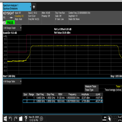
Band2-5MHz-16QAM-18625-25RB#0-PASS
