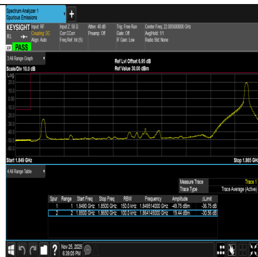
Band2-15MHz-QPSK-18675-1RB#74-PASS
