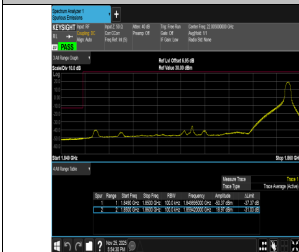
Band2-10MHz-16QAM-18650-1RB#49-PASS
