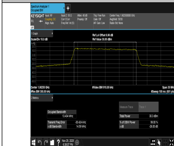
Band2-15MHz-QPSK-19125-75RB#0-PASS
