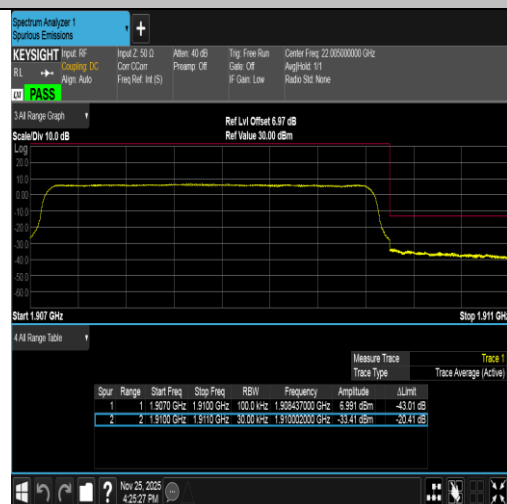
Band2-3MHz-16QAM-19185-15RB#0-PASS
