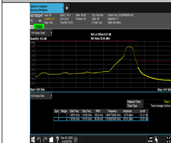
Band2-3MHz-16QAM-19185-1RB#14-PASS
