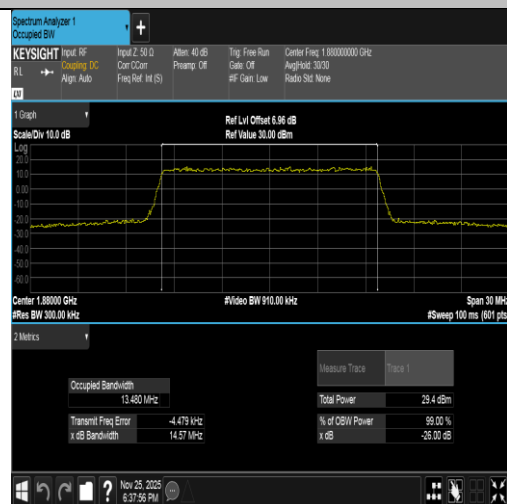
Band2-15MHz-16QAM-18900-75RB#0-PASS
