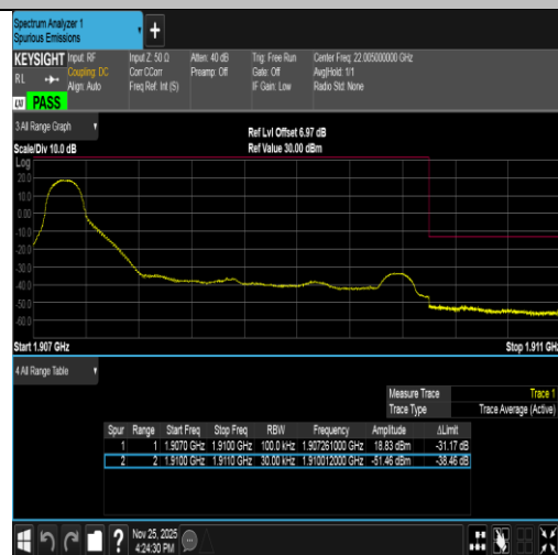
Band2-3MHz-16QAM-19185-1RB#0-PASS
