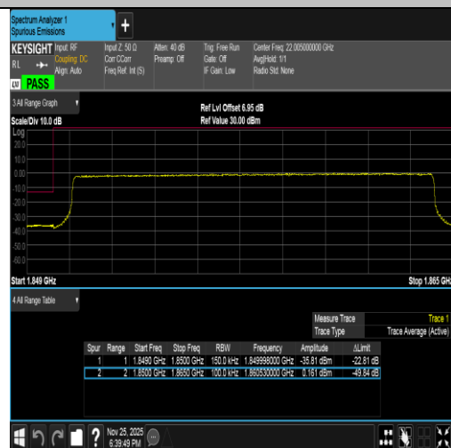
Band2-15MHz-16QAM-18675-75RB#0-PASS
