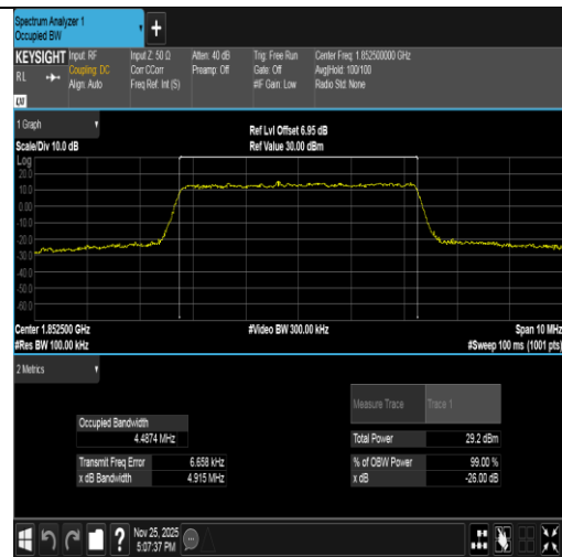
Band2-5MHz-16QAM-18625-25RB#0-PASS
