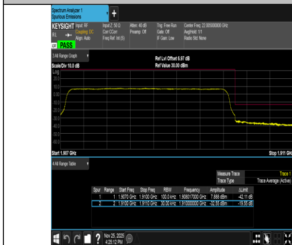
Band2-3MHz-QPSK-19185-15RB#0-PASS
